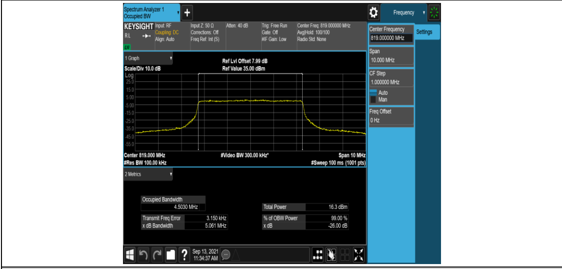
Band26-5MHz-QPSK-26740-25RB#0
