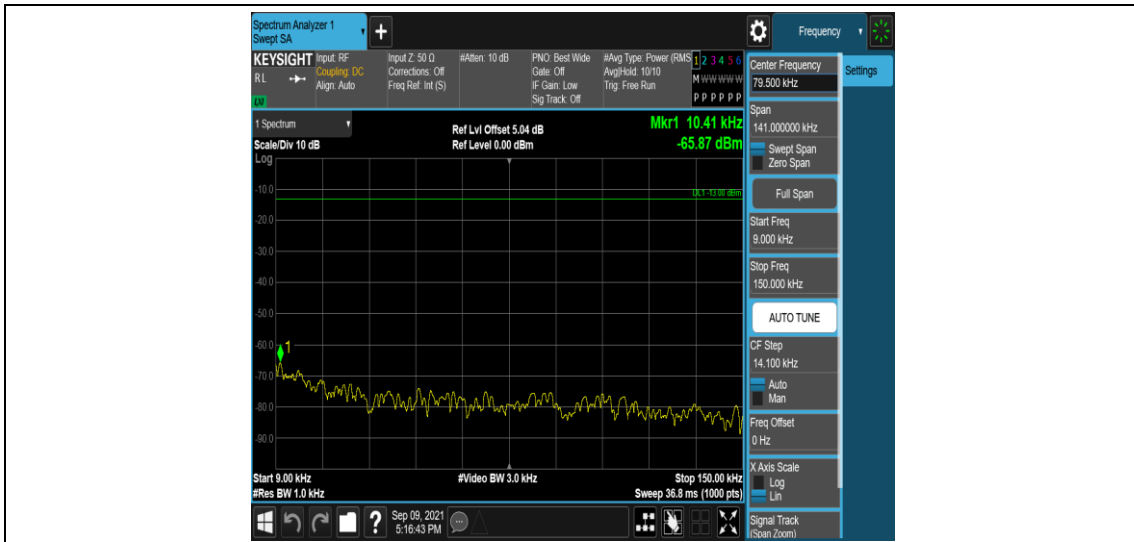
Band25-15MHz-16QAM-26615-1RB#0-Range1:0.009~0.15MHz
