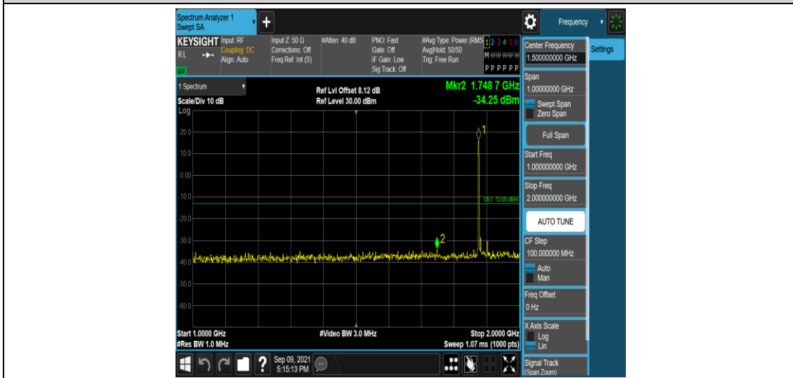
Band25-15MHz-16QAM-26365-1RB#0-Range4:1000~2000MHz
