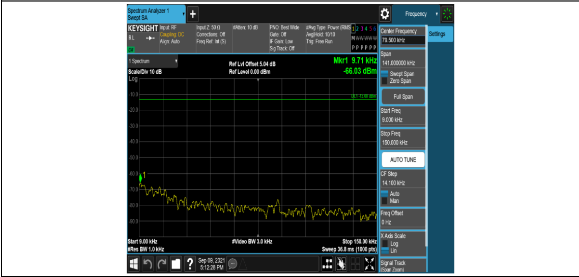
Band25-15MHz-16QAM-26115-1RB#0-Range1:0.009~0.15MHz
