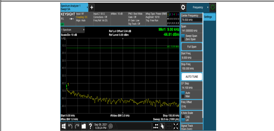
Band25-20MHz-16QAM-26365-1RB#0-Range1:0.009~0.15MHz
