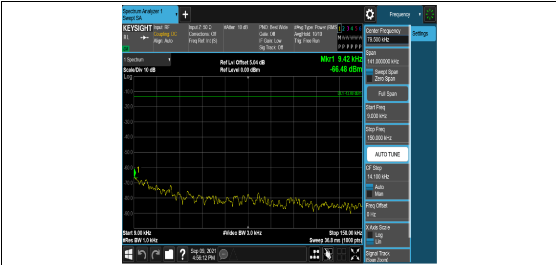
Band25-10MHz-16QAM-26640-1RB#0-Range1:0.009~0.15MHz
