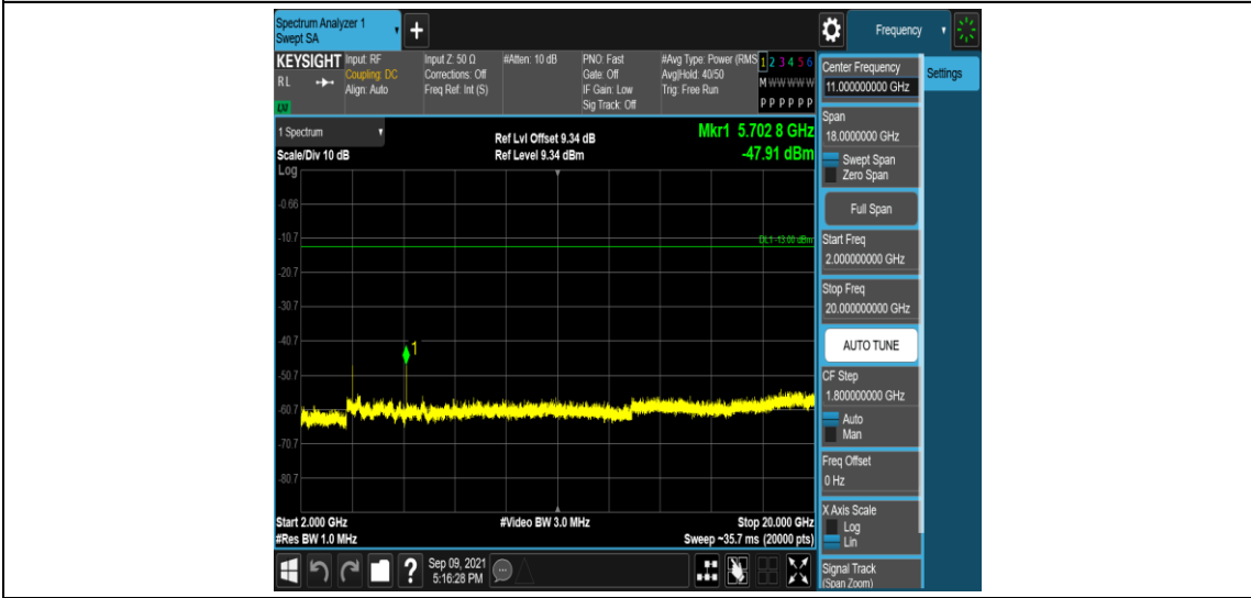
Band25-15MHz-QPSK-26615-1RB#0-Range5:2000~20000MHz
