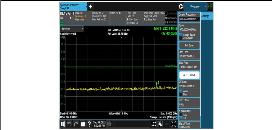
Band25-20MHz-QPSK-26140-1RB#0-Range3:30~1000MHz
