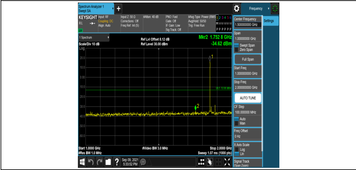
Band25-20MHz-16QAM-26140-1RB#0-Range4:1000~2000MHz
