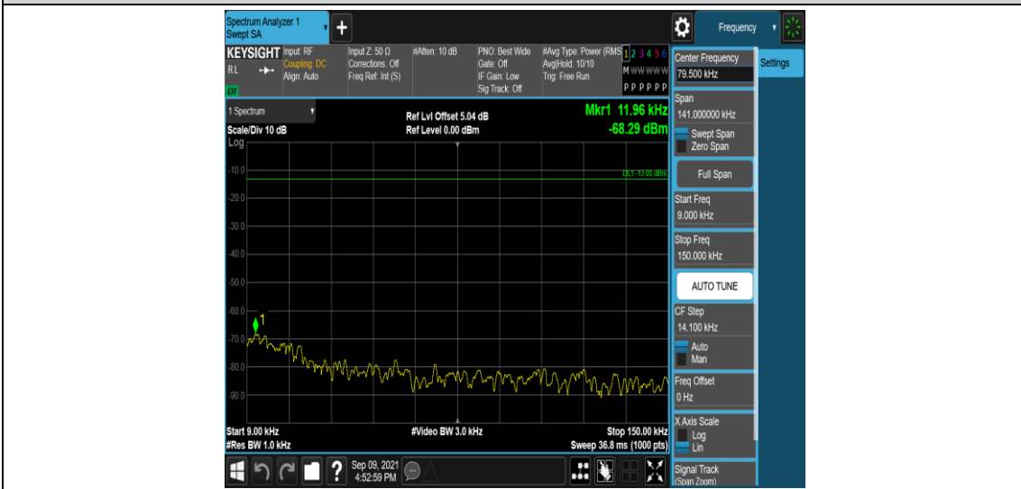
Band25-10MHz-QPSK-26365-1RB#0-Range1:0.009~0.15MHz
