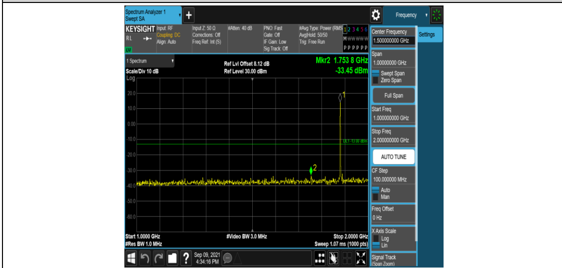
Band25-5MHz-16QAM-26365-1RB#0-Range4:1000~2000MHz
