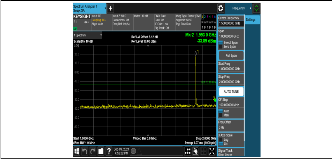
Band25-10MHz-16QAM-26090-1RB#0-Range4:1000~2000MHz
