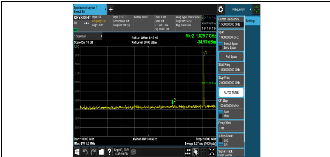
Band25-5MHz-QPSK-26665-1RB#0-Range4:1000~2000MHz
