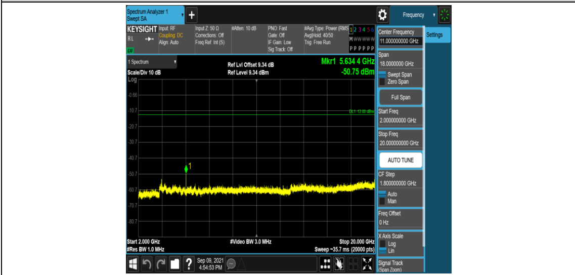
Band25-10MHz-16QAM-26365-1RB#0-Range5:2000~20000MHz
