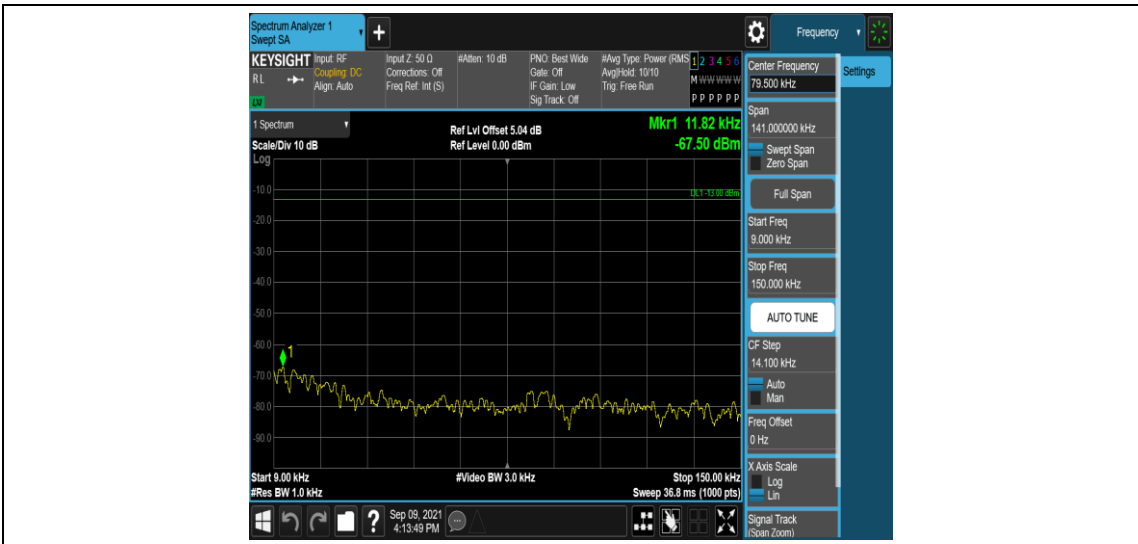
Band25-3MHz-QPSK-26675-1RB#0-Range1:0.009~0.15MHz
