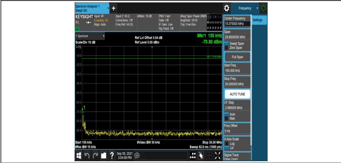
Band25-1.4MHz-16QAM-26683-1RB#0-Range2:0.15~30MHz
