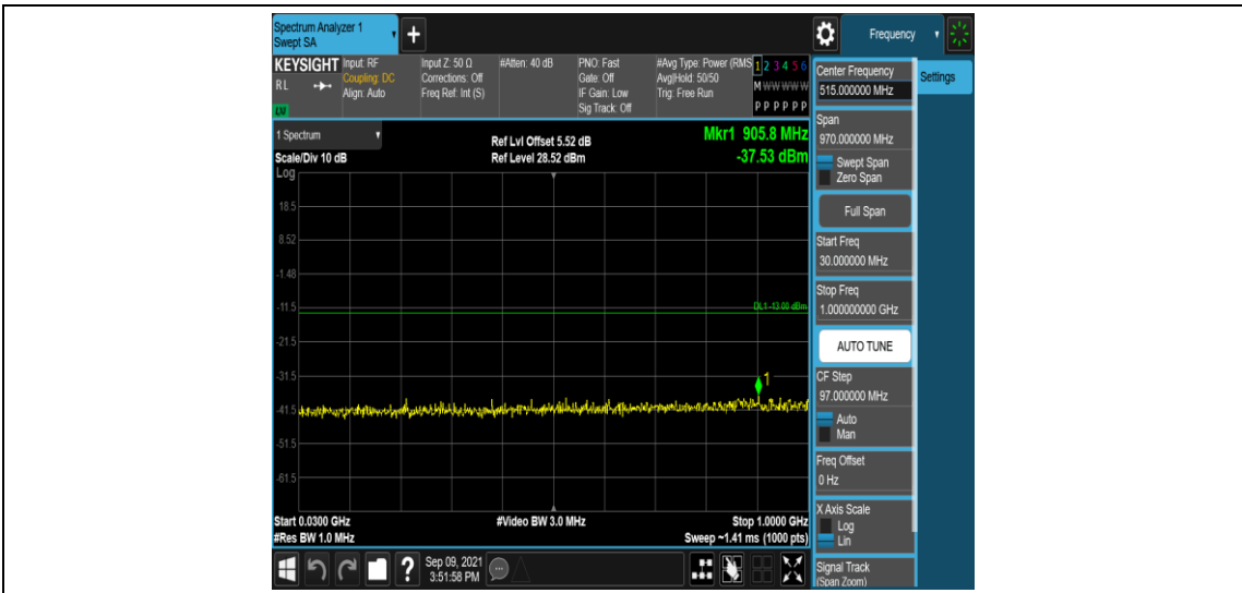
Band25-1.4MHz-QPSK-26365-1RB#0-Range3:30~1000MHz
