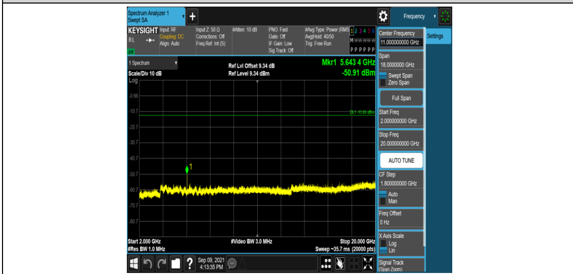
Band25-3MHz-16QAM-26365-1RB#0-Range5:2000~20000MHz
