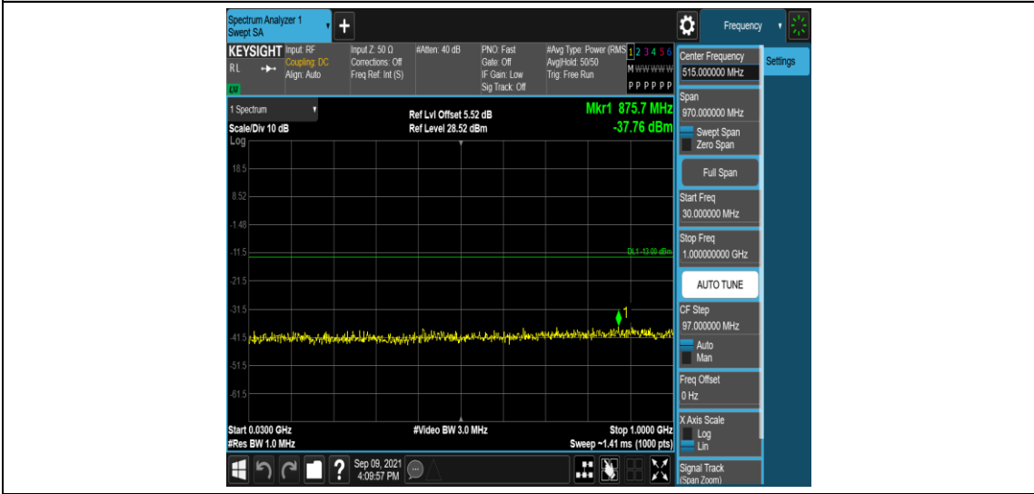
Band25-3MHz-QPSK-26055-1RB#0-Range3:30~1000MHz
