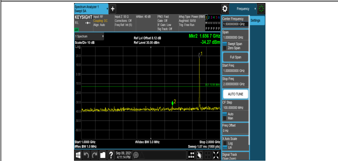
Band25-3MHz-16QAM-26055-1RB#0-Range4:1000~2000MHz
