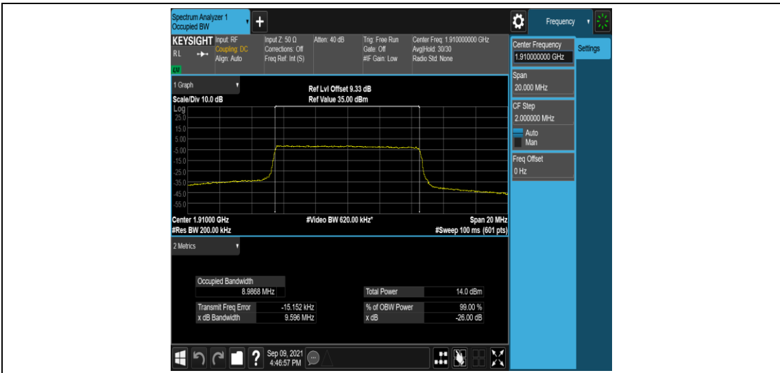
Band25-10MHz-16QAM-26640-50RB#0
