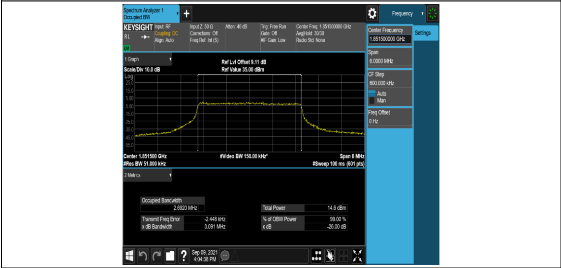
Band25-3MHz-QPSK-26055-15RB#0
