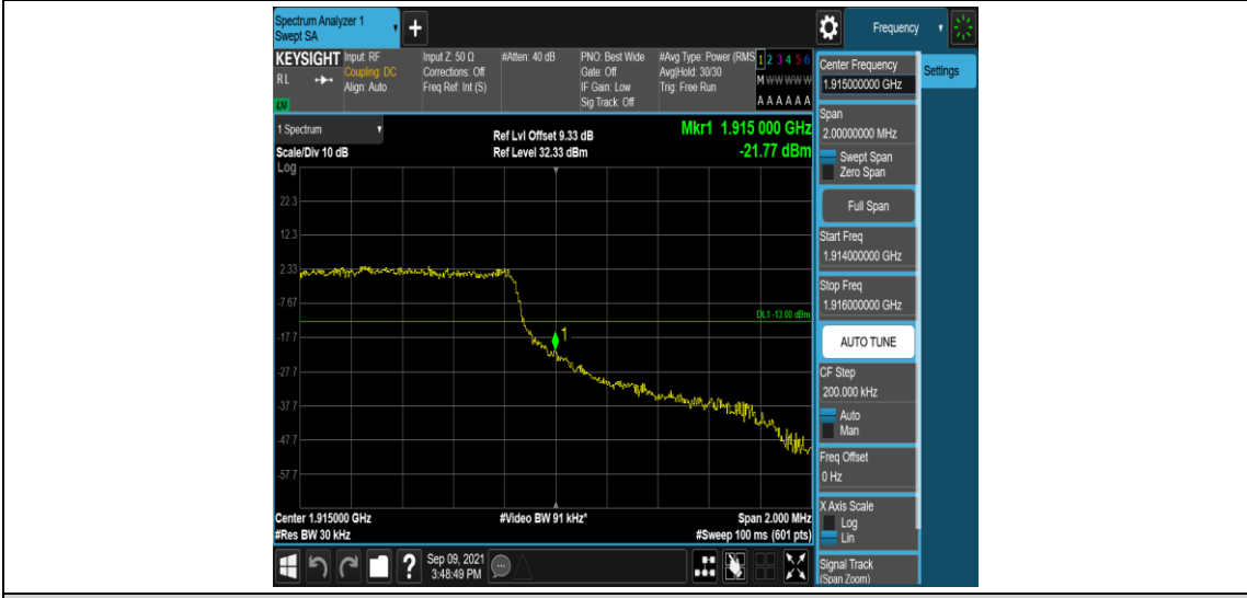
Band25-1.4MHz-QPSK-26683-6RB#0
