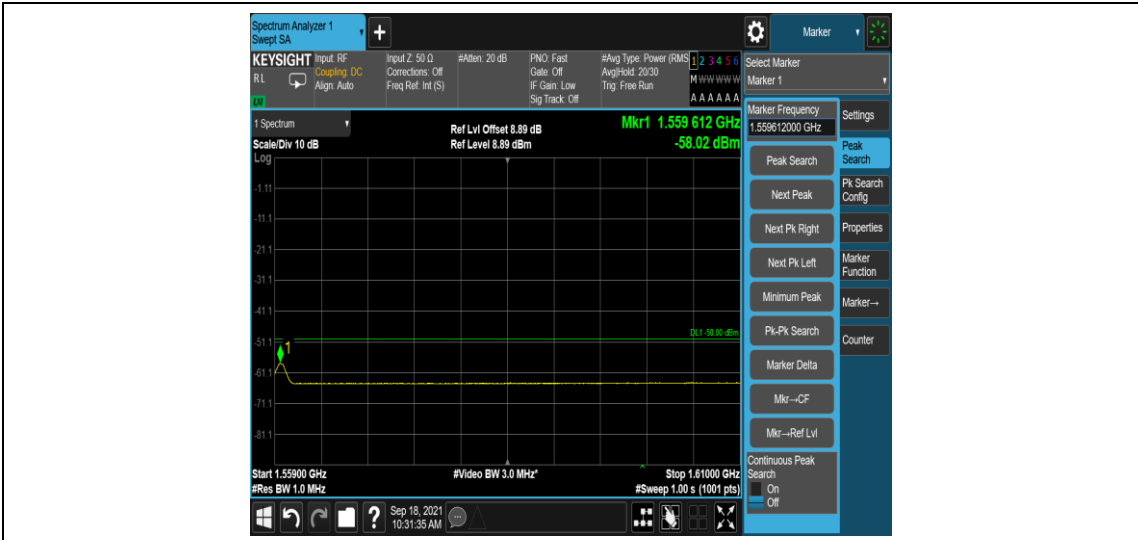
Band13-5MHz-16QAM-23230-1RB#0-Range7:1559~1610MHz
