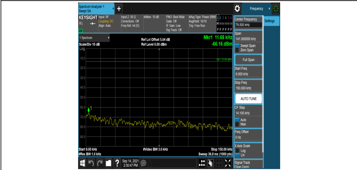
Band13-5MHz-16QAM-23255-1RB#0-Range1:0.009~0.15MHz
