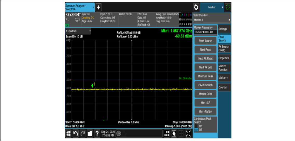
Band13-5MHz-16QAM-23255-1RB#0-Range7:1559~1610MHz
