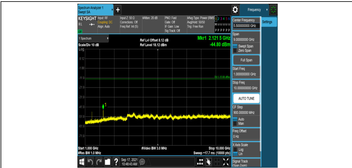
Band12-1.4MHz-QPSK-23095-1RB#0-Range4:1000~10000MHz
