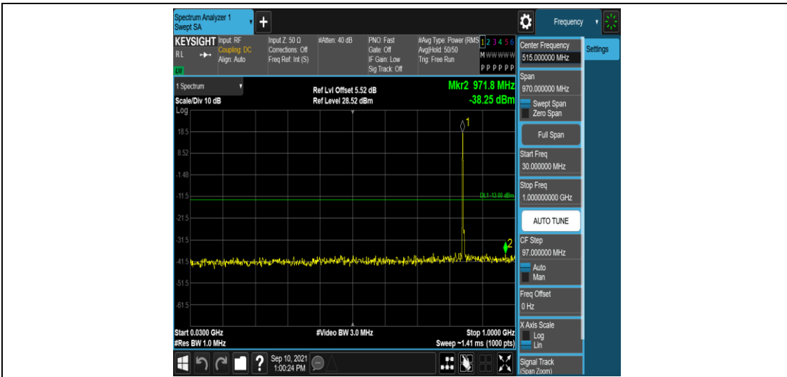
Band5-5MHz-QPSK-20625-1RB#0-Range3:30~1000MHz
