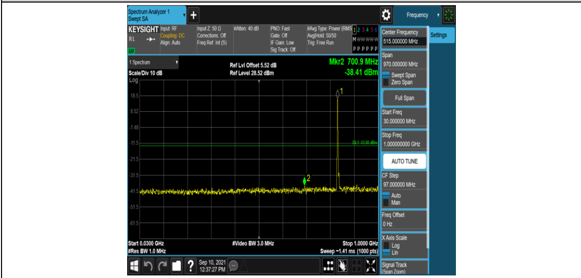
Band5-3MHz-16QAM-20525-1RB#0-Range3:30~1000MHz
