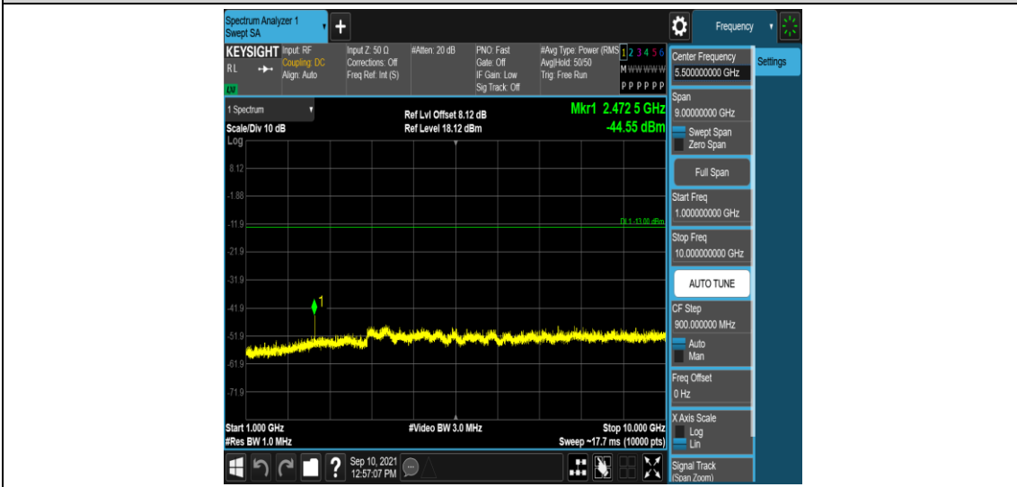
Band5-5MHz-QPSK-20425-1RB#0-Range4:1000~10000MHz
