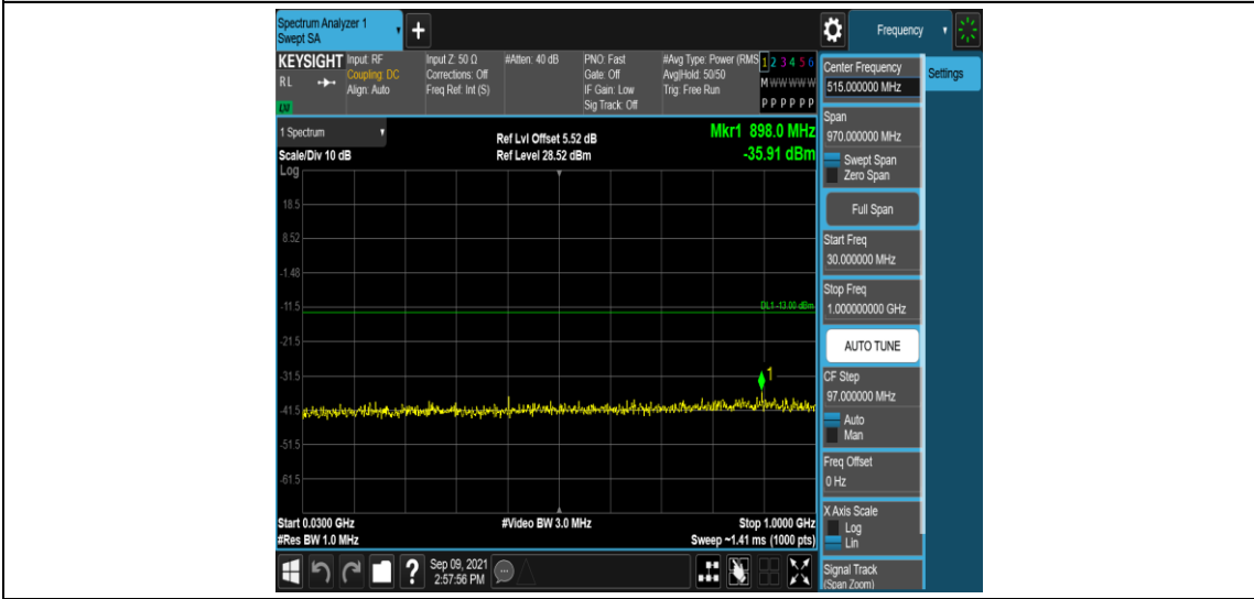
Band4-15MHz-QPSK-2025-1RB#0-Range3:30~1000MHz
