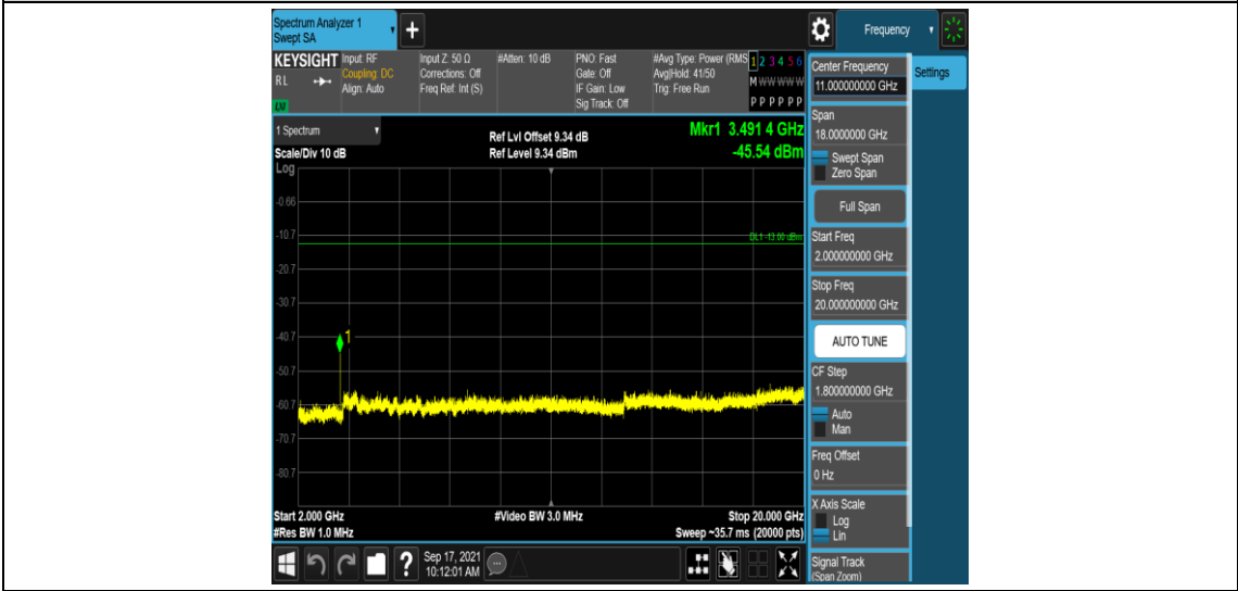
Band4-10MHz-16QAM-20350-1RB#0-Range5:2000~20000MHz
