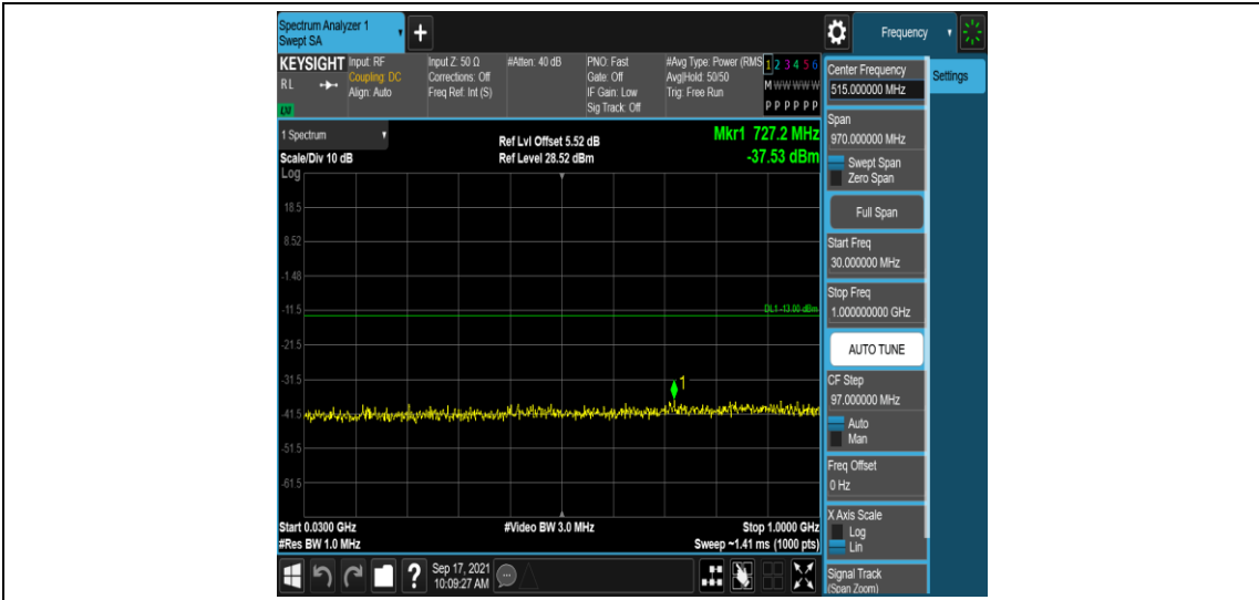
Band4-10MHz-16QAM-20175-1RB#0-Range3:30~1000MHz
