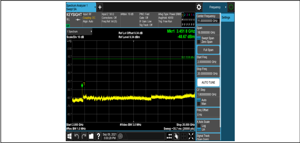
Band4-15MHz-QPSK-20175-1RB#0-Range5:2000~20000MHz
