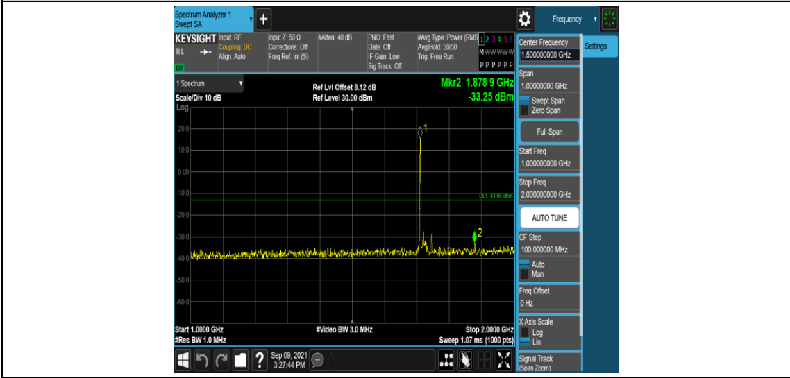
Band4-20MHz-16QAM-20050-1RB#0-Range4:1000~2000MHz
