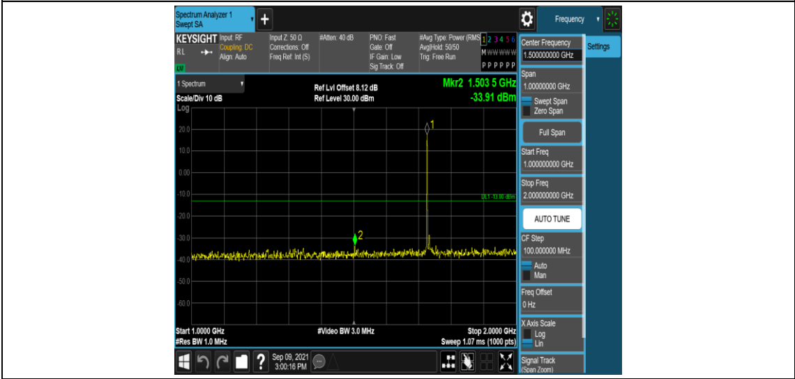
Band4-15MHz-QPSK-20175-1RB#0-Range4:1000~2000MHz
