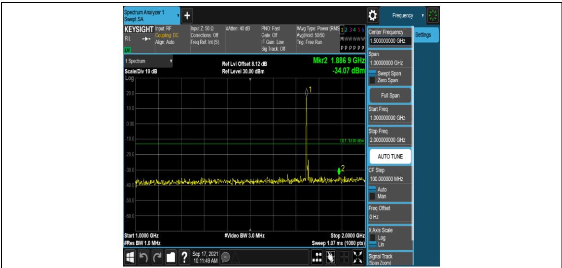
Band4-10MHz-16QAM-20350-1RB#0-Range4: 1000~2000MHz
