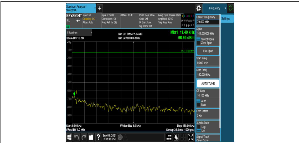
Band4-15MHz-QPSK-20325-1RB#0-Range1:0.009~0.15MHz
