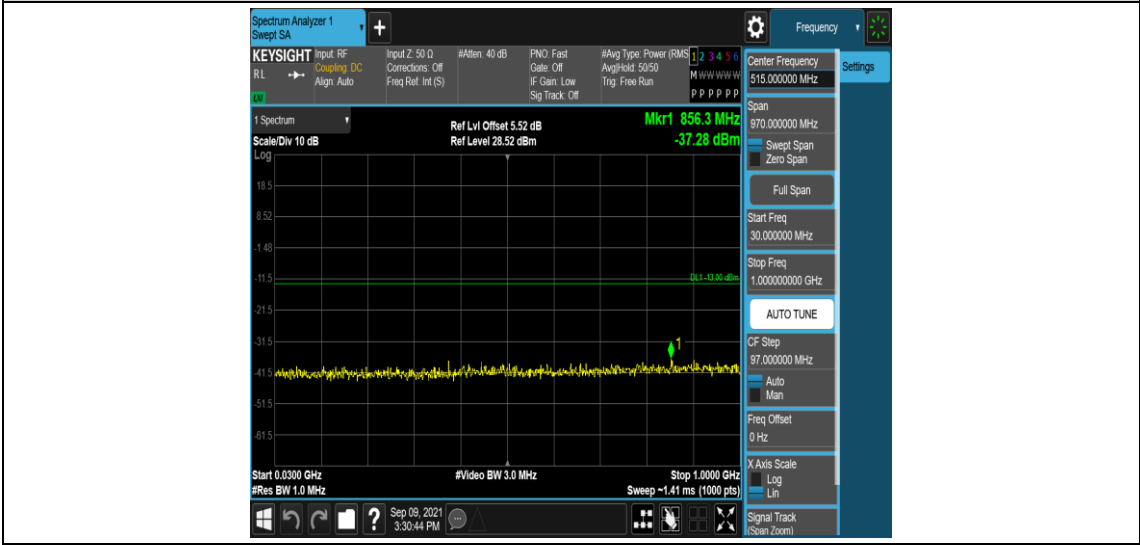
Band4-20MHz-QPSK-20300-1RB#0-Range3:30~1000MHz
