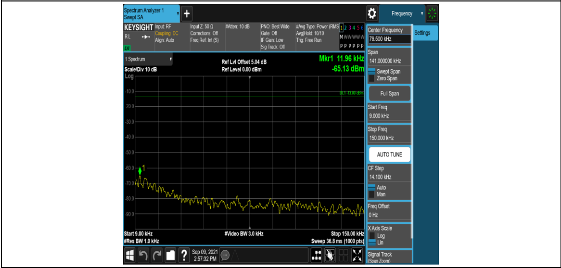
Band4-15MHz-QPSK-20025-1RB#0-Range1:0.009~0.15MHz
