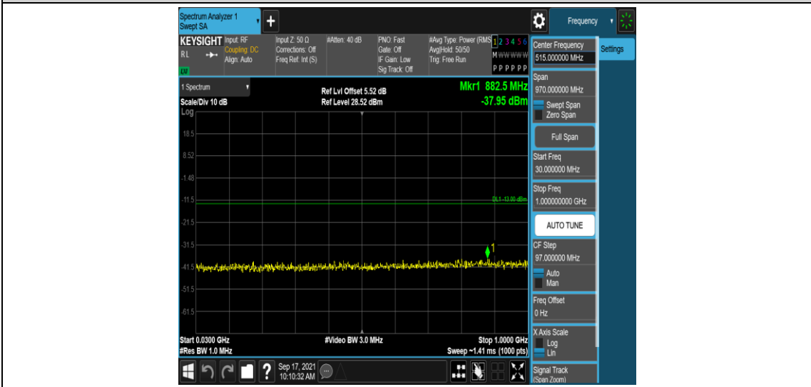
Band4-10MHz-QPSK-20350-1RB#0-Range3:30~1000MHz
