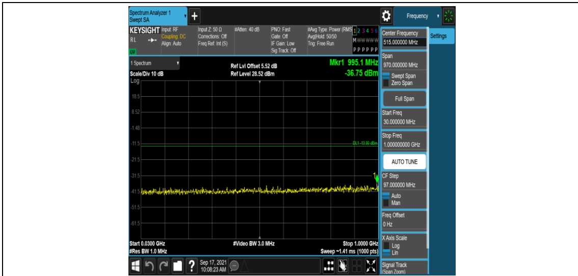
Band4-10MHz-QPSK-20175-1RB#0-Range3:30~1000MHz
