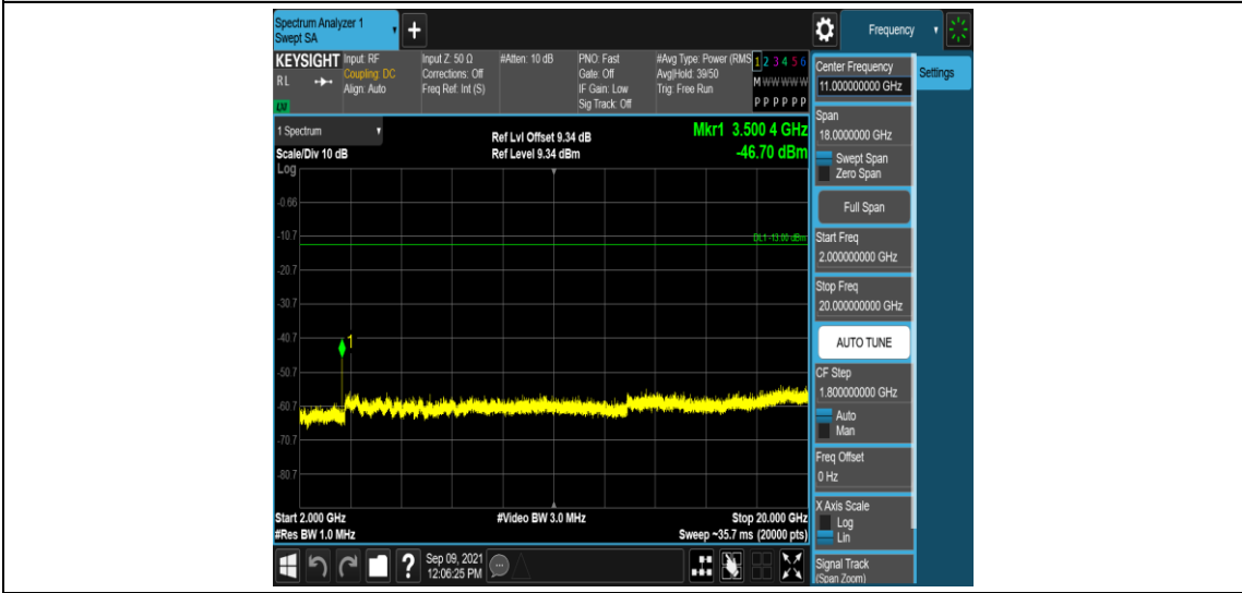
Band4-5MHz-16QAM-20375-1RB#0-Range5:2000~20000MHz
