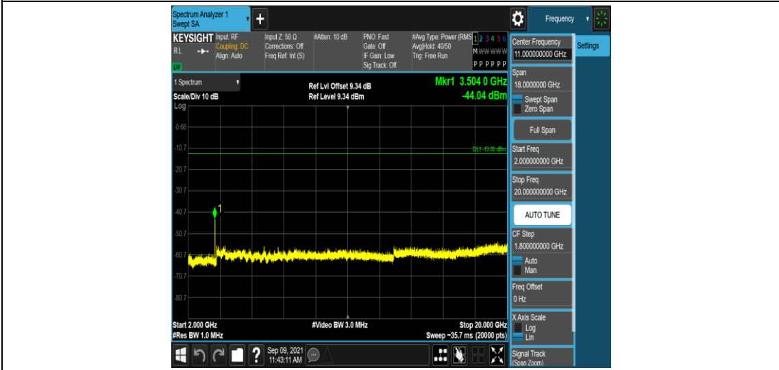
Band4-3MHz-16QAM-20385-1RB#0-Range5:2000~20000MHz
