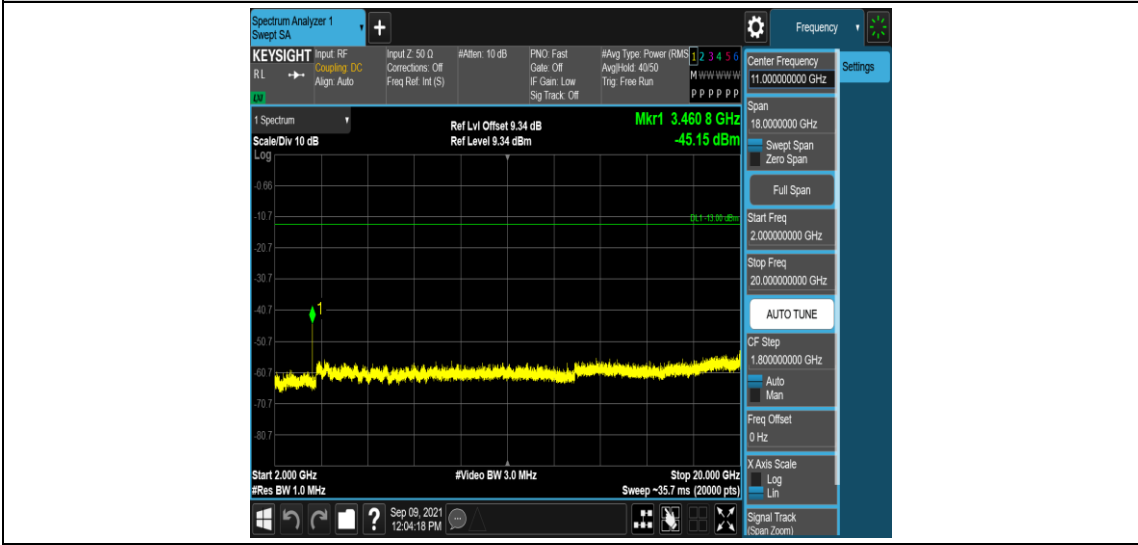
Band4-5MHz-16QAM-20175-1RB#0-Range5:2000~20000MHz
