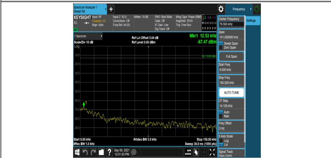
Band4-5MHz-16QAM-19975-1RB#0-Range1:0.009~0.15MHz
