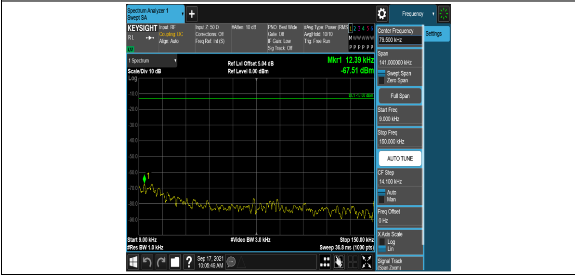
Band4-10MHz-QPSK-20000-1RB#0-Range1:0.009~0.15MHz
