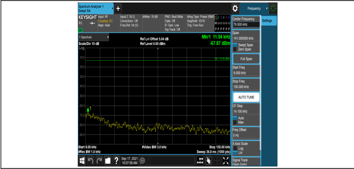
Band4-10MHz-QPSK-20175-1RB#0-Range1:0.009~0.15MHz
