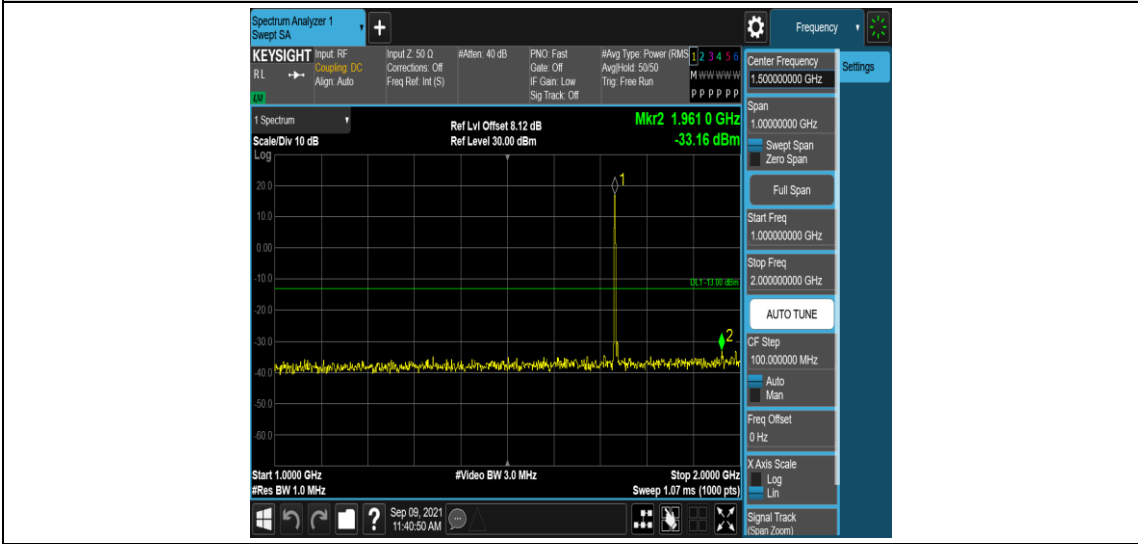
Band4-3MHz-16QAM-20175-1RB#0-Range4:1000~2000MHz
