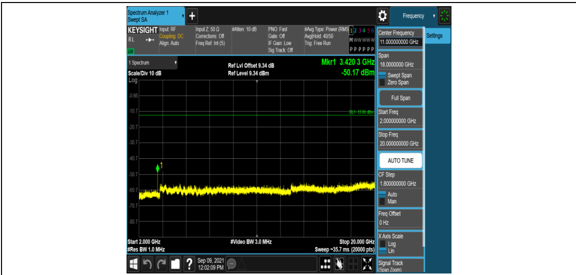
Band4-5MHz-16QAM-19975-1RB#0-Range5:2000~20000MHz
