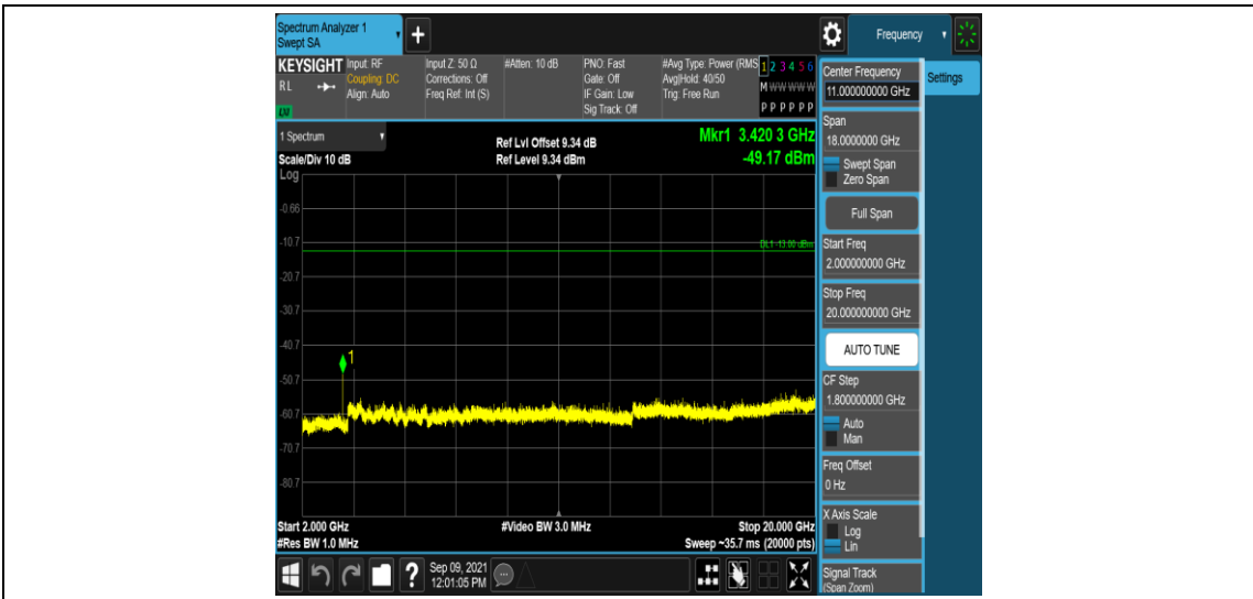
Band4-5MHz-QPSK-19975-1RB#0-Range5:2000~20000MHz
