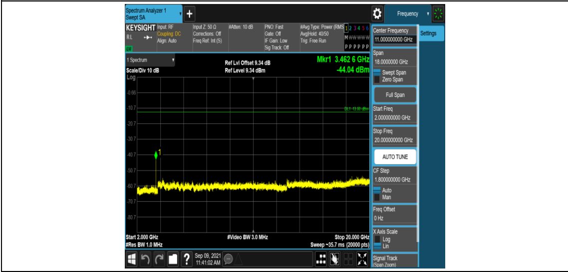
Band4-3MHz-16QAM-20175-1RB#0-Range5:2000~20000MHz
