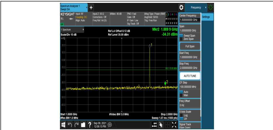
Band4-5MHz-16QAM-20375-1RB#0-Range4:1000~2000MHz
