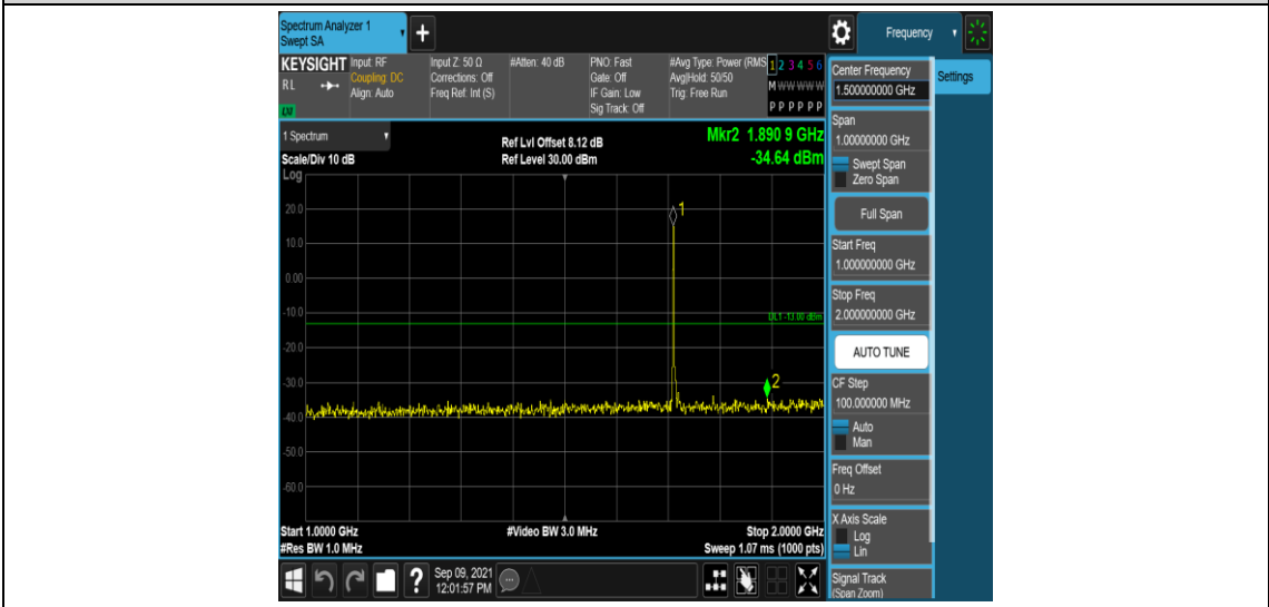
Band4-5MHz-16QAM-19975-1RB#0-Range4:1000~2000MHz
