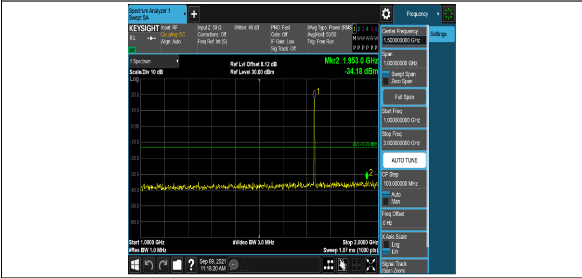
Band4-1.4MHz-16QAM-20175-1RB#0-Range4:1000~2000MHz
