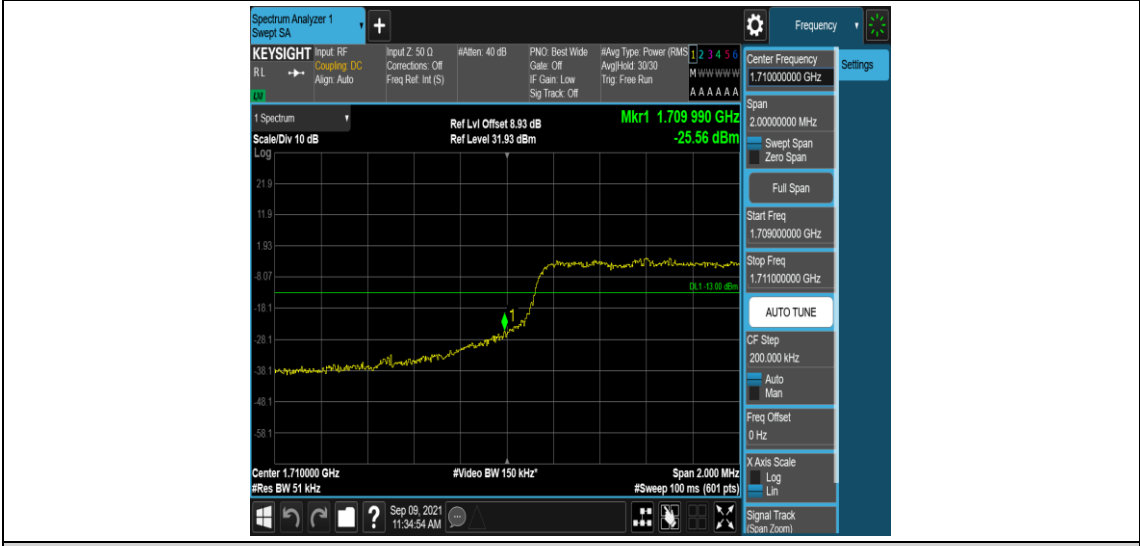
Band4-3MHz-16QAM-19965-15RB#0
