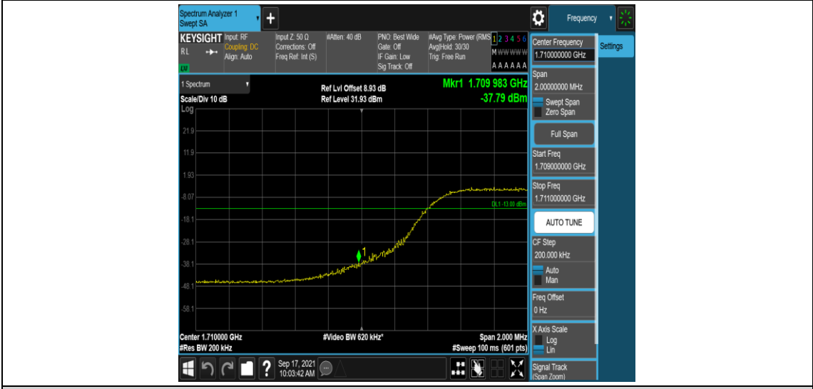
Band4-10MHz-16QAM-20000-50RB#0
