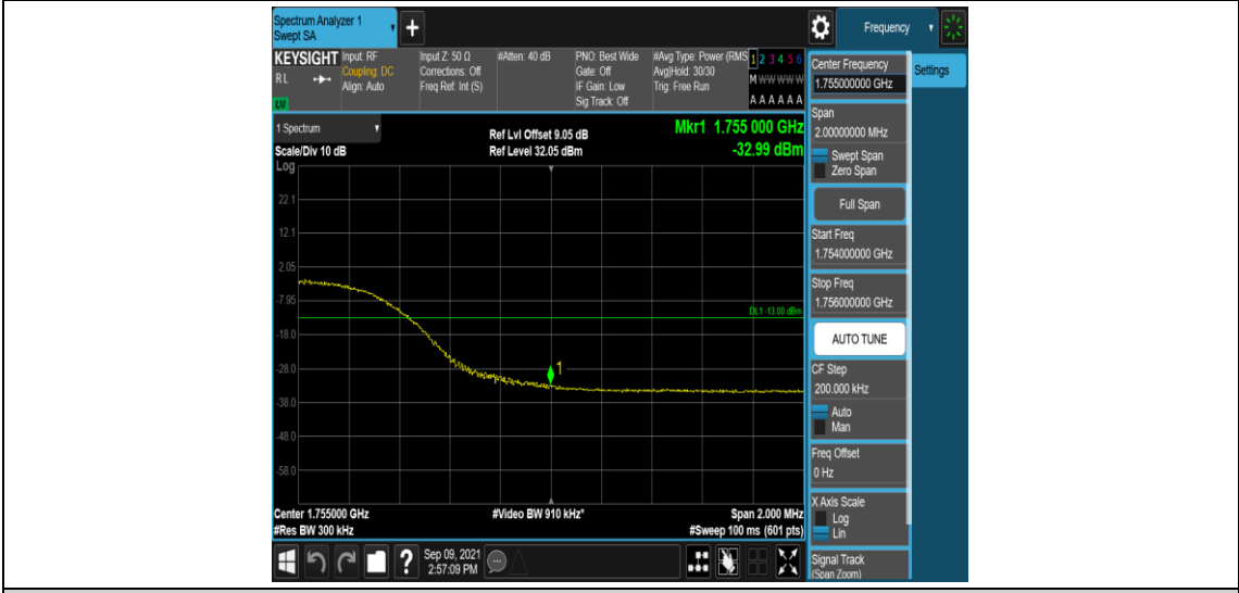
Band4-15MHz-16QAM-20325-75RB#0
