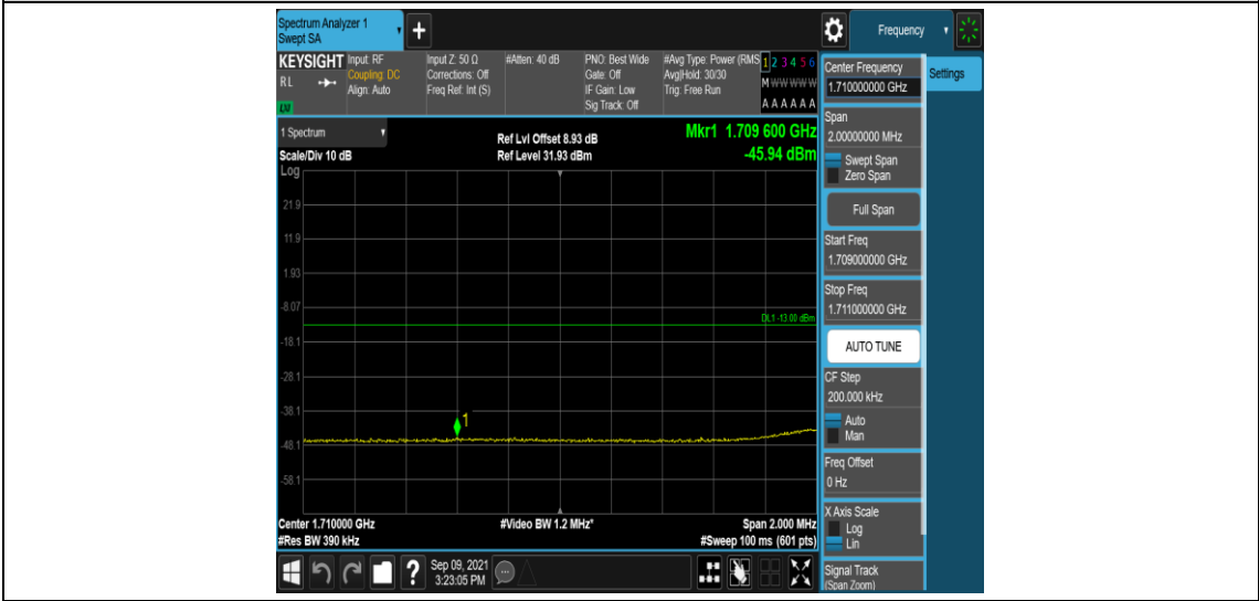
Band4-20MHz-16QAM-20050-1RB#99
