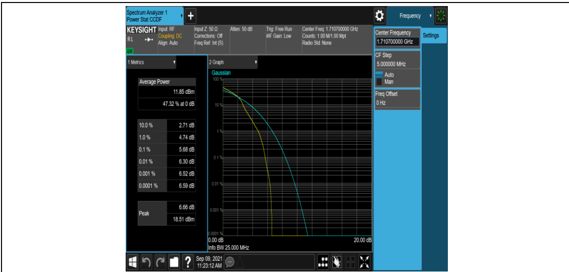
Band4-1.4MHz-16QAM-19957-1RB#0
