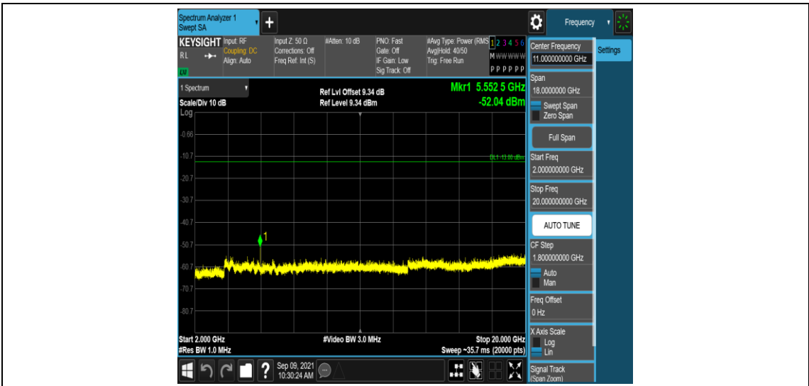
Band2-15MHz-16QAM-18675-1RB#0-Range5:2000~20000MHz
