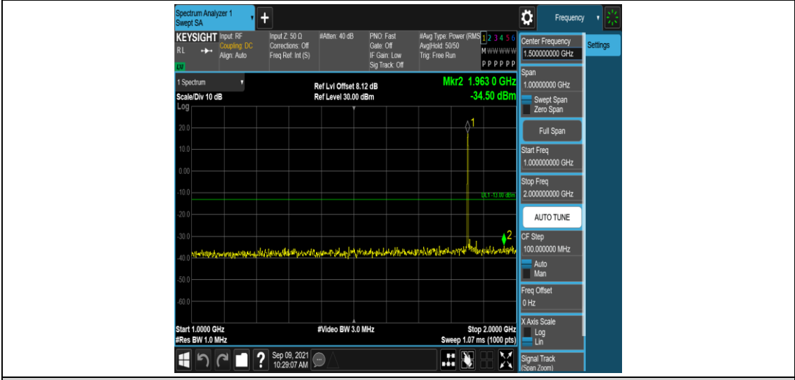
Band2-15MHz-QPSK-18675-1RB#0-Range4:1000~2000MHz
