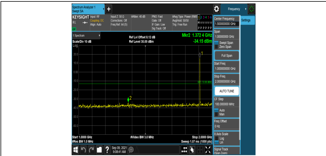
Band2-1.4MHz-16QAM-19193-1RB#0-Range4:1000~2000MHz
