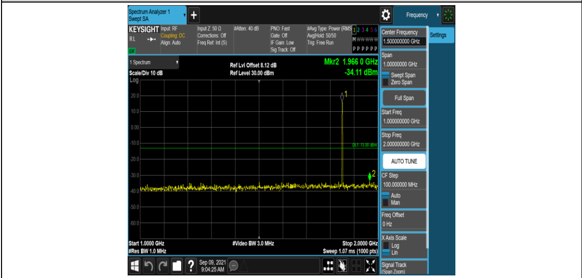
Band2-1.4MHz-16QAM-18607-1RB#0-Range4:1000~2000MHz
