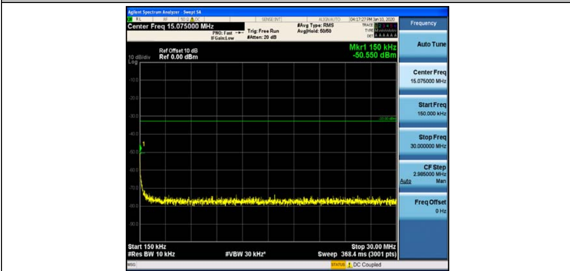
Band25_1.4MHz_16QAM_26365_1RB#0
