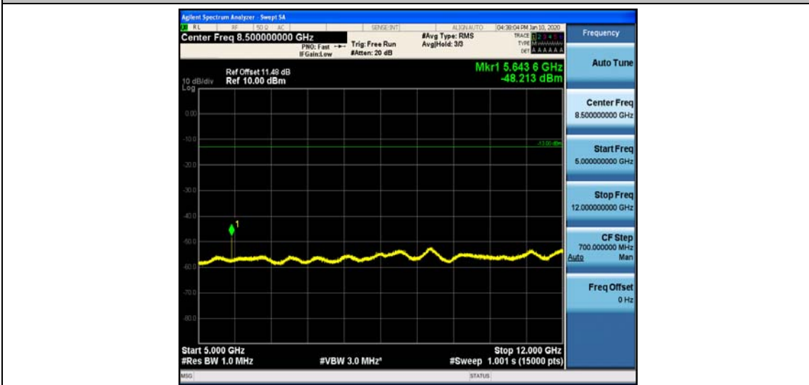
Band25_3MHz_QPSK_26365_1RB#0
