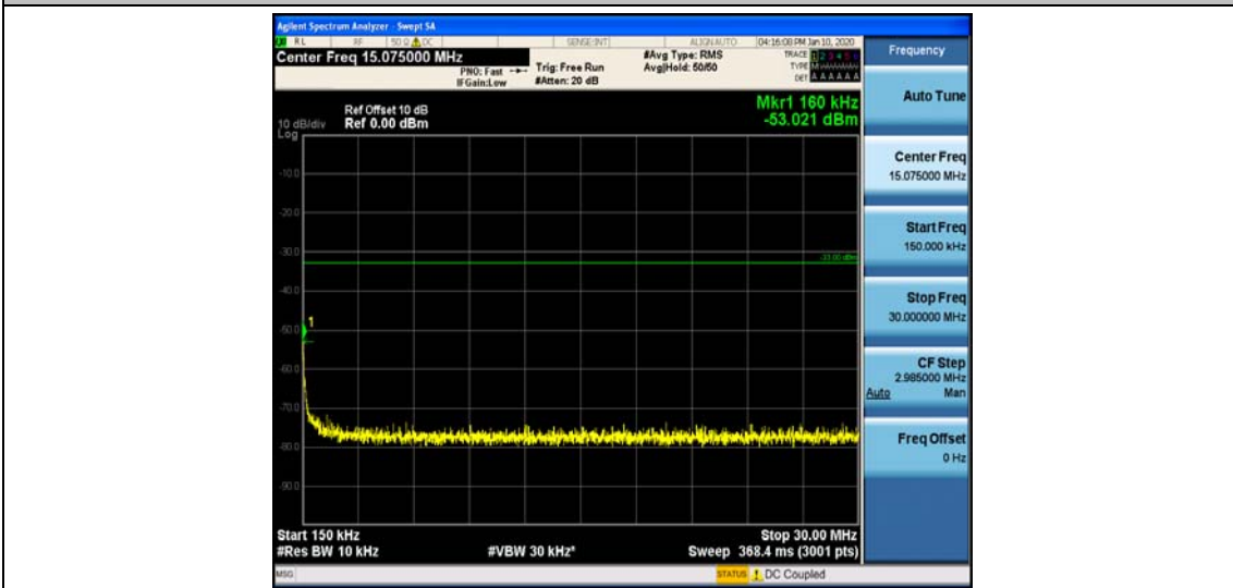
Band25_1.4MHz_QPSK_26365_1RB#0
