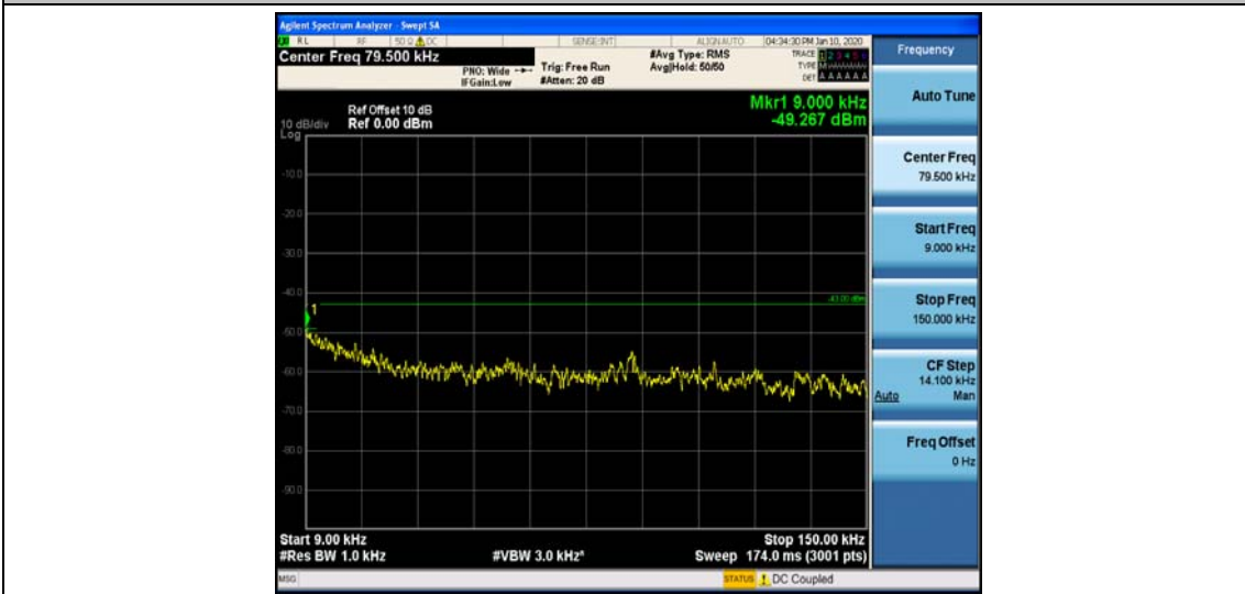
Band25_3MHz_QPSK_24055_1RB#0
