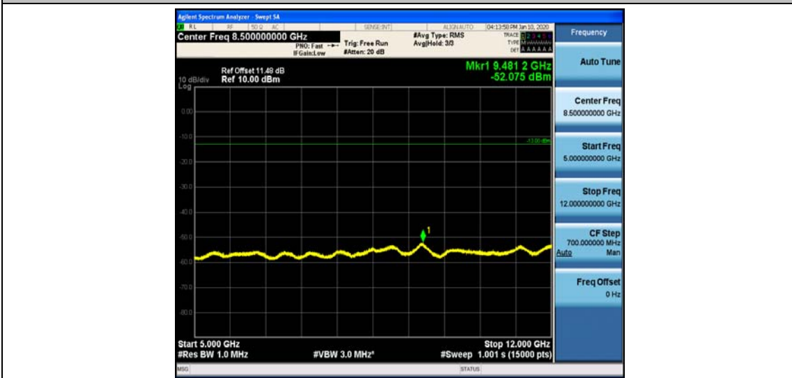
Band25_1.4MHz_QPSK_24047_1RB#0
