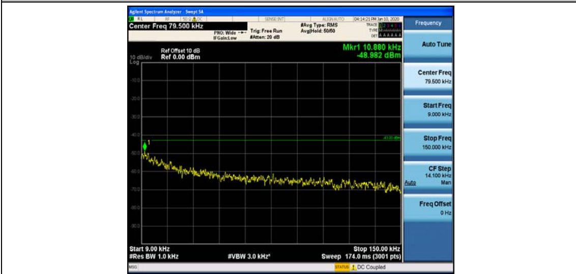
Band25_1.4MHz_16QAM_24047_1RB#0
