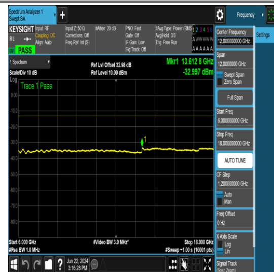
NTNV_N78-3700-3800_PC2_30_40_L_TID20_NS _01_0.009_0.15_#1
