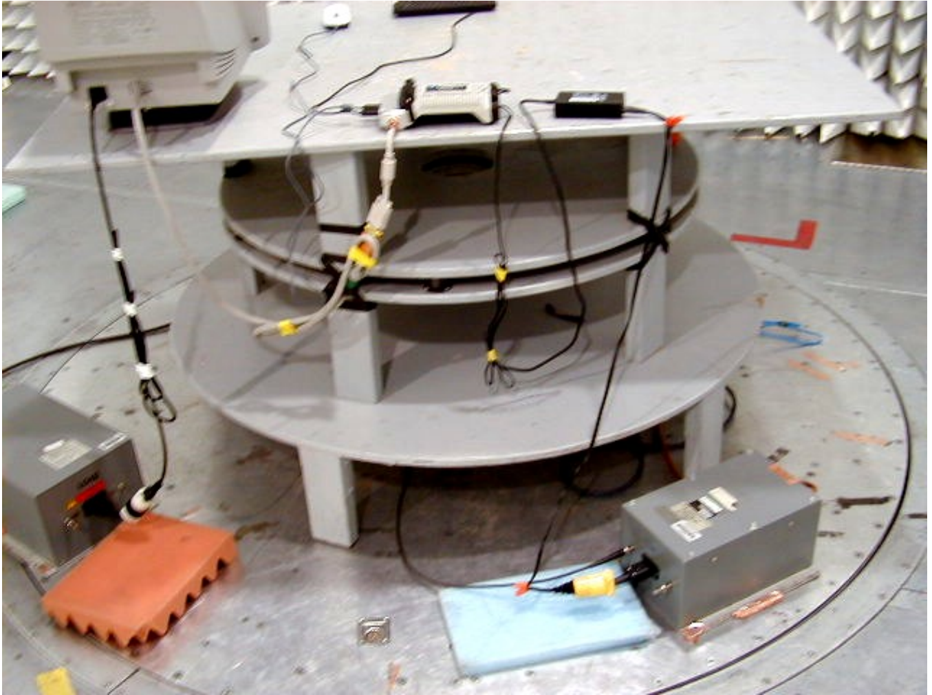
Conducted Emissions Test Configuration
