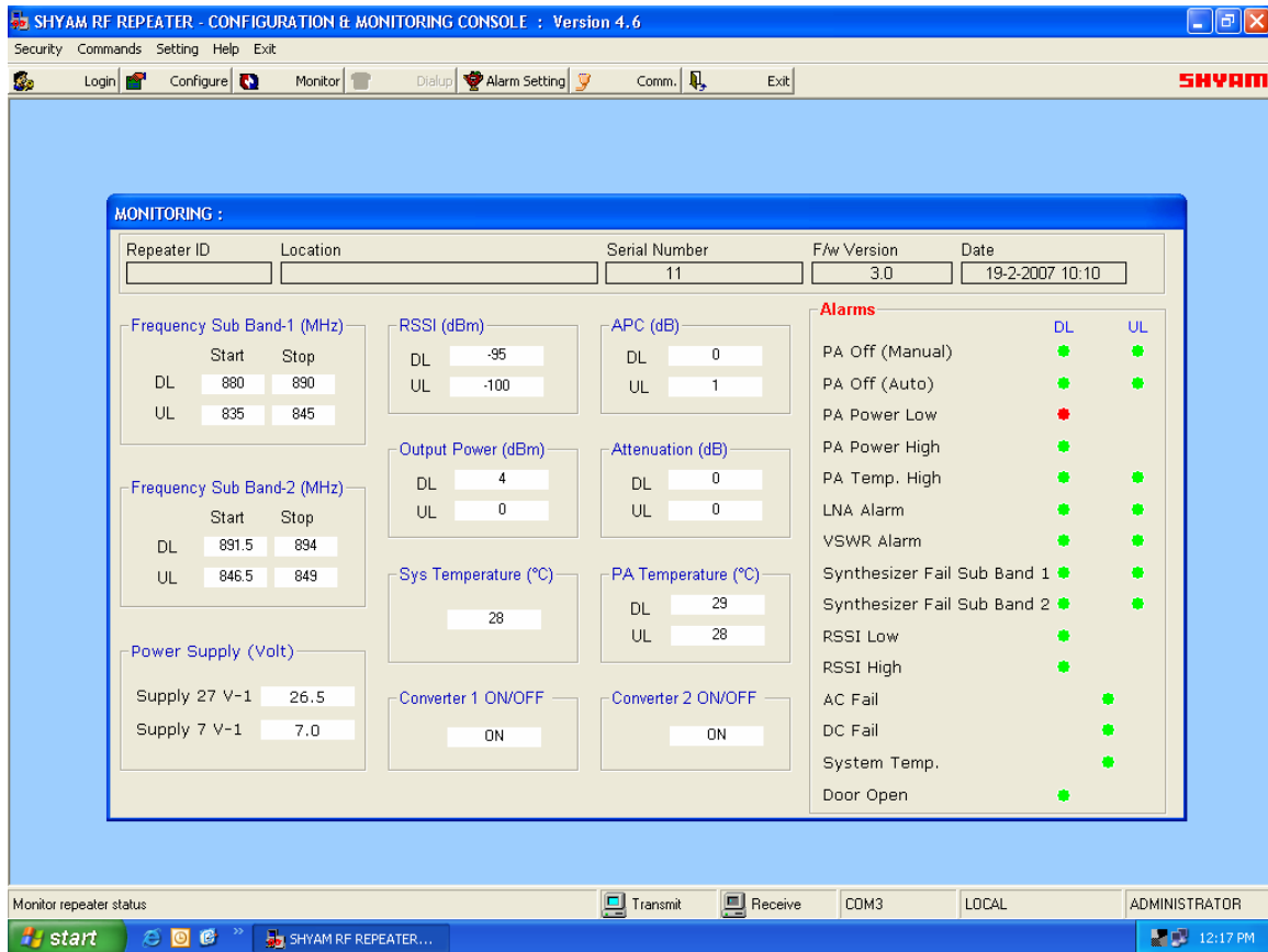
Figure 5: Monitoring Window
