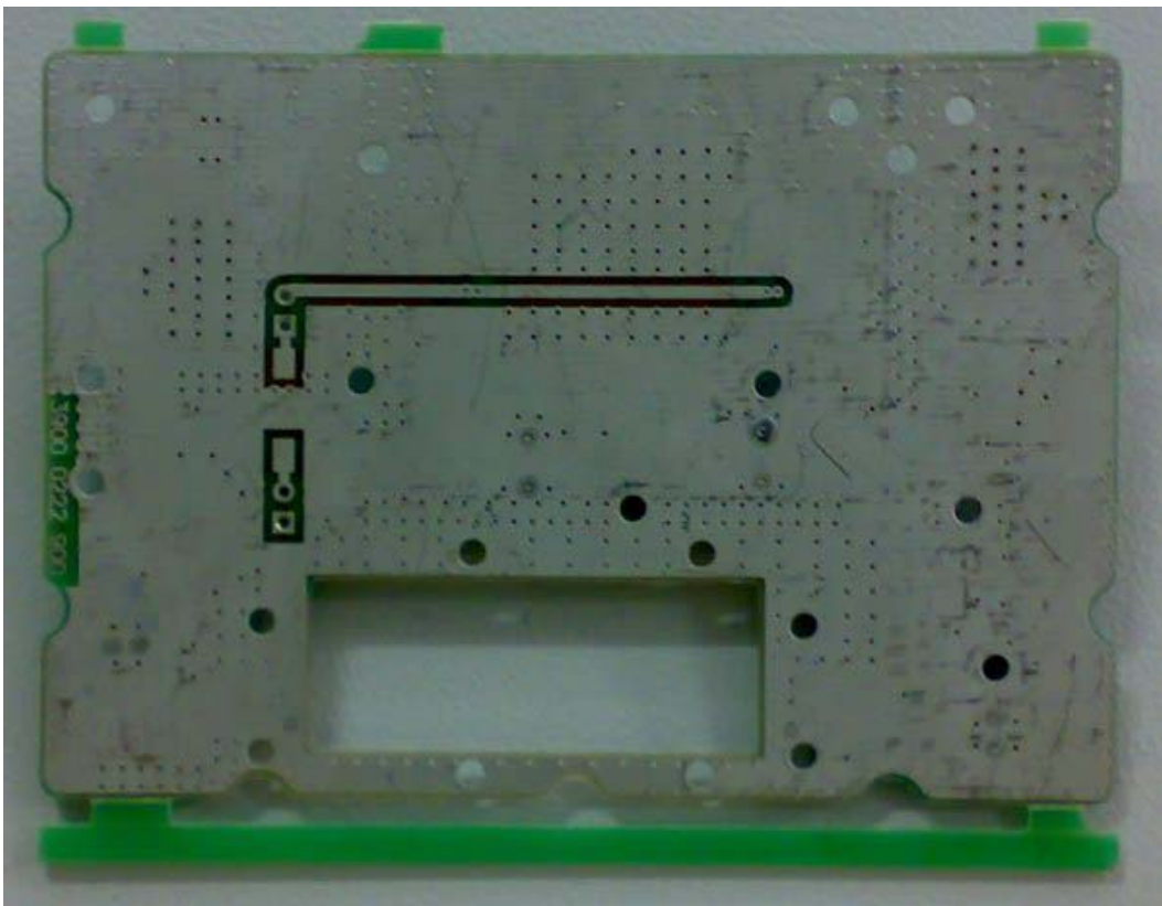
LNA& Converter Foil Side
