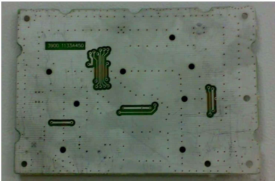
LNA PCB View
