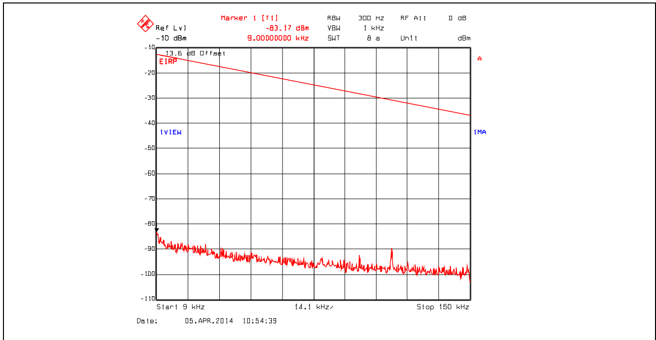
Plot 5.4.4.3.26. Conducted Spurious Emissions – Restricted Bands 802.11g, 9 Mbps, 2462 MHz, 9 kHz - 150 kHz, Peak Detector with Band (Notch) Reject Filter
