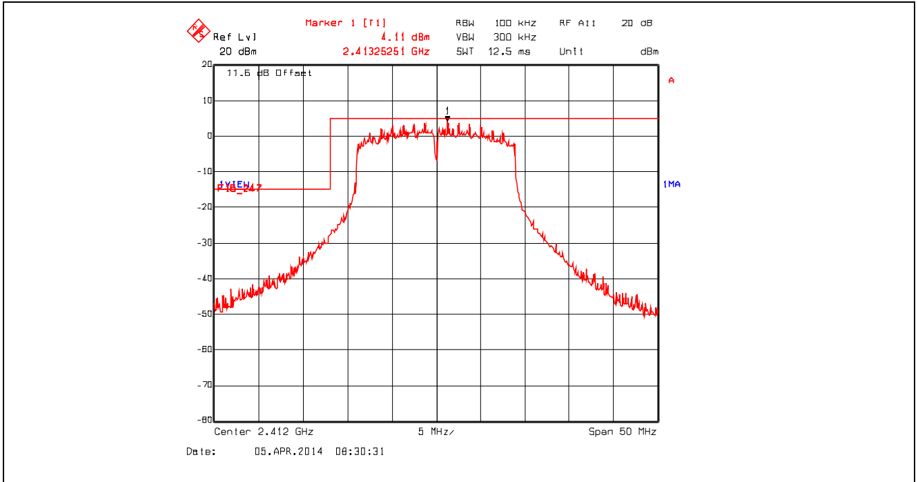
Plot 5.4.4.1.5. Band-Edge RF Conducted Emissions, Lower Band-edge, 2412 MHz, 802.11n 800ns, 65 Mbps
