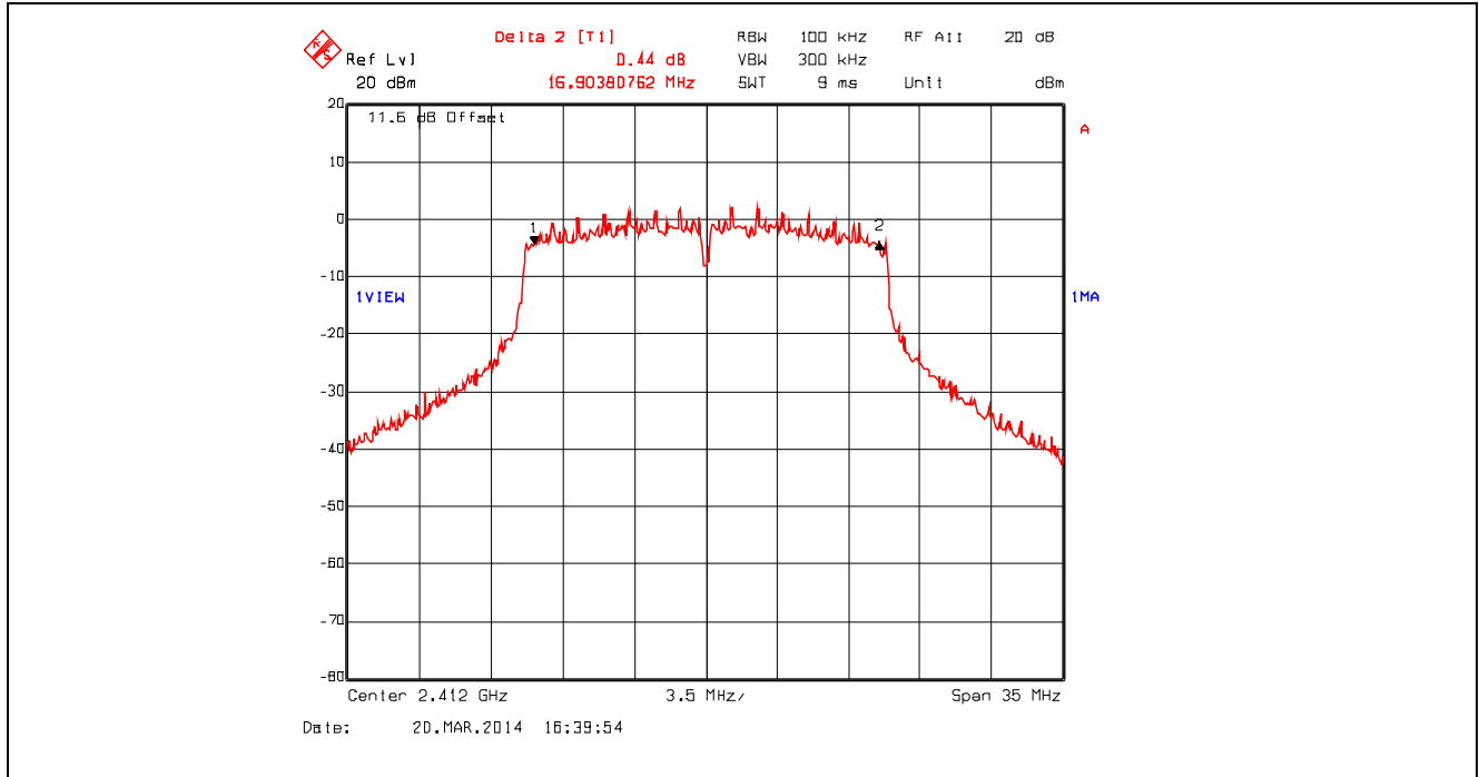
Plot 5.2.4.31. 6 dB Bandwidth, 802.11n 800ns, 65 Mbps 64-QAM 5/6, 2412 MHz
