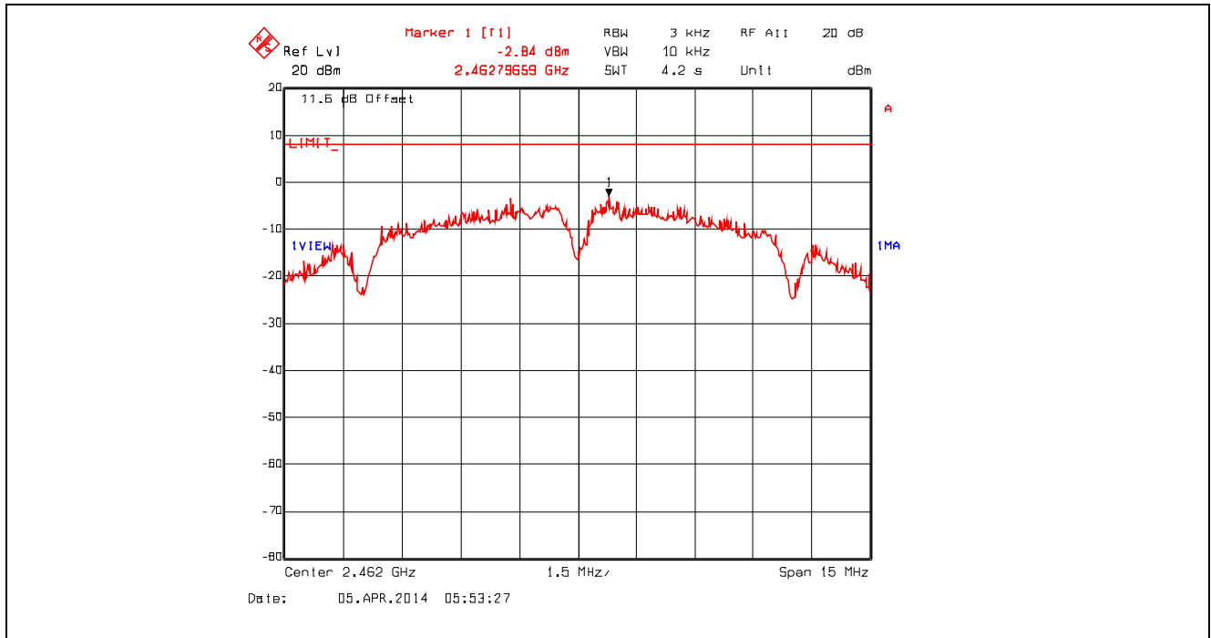
Plot 5.6.4.3. Power Spectral Density, 802.11b, 1 Mbps DBPSK, 2462 MHz
