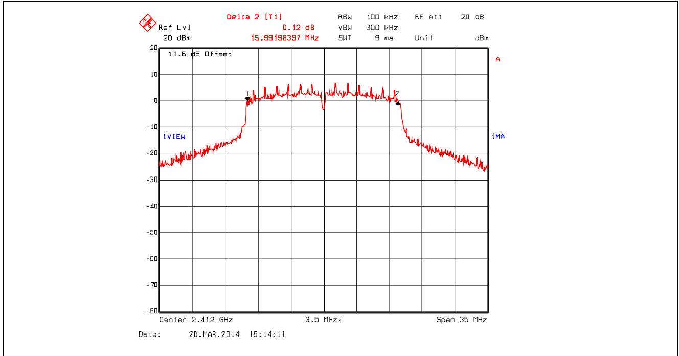
Plot 5.2.4.10. 6 dB Bandwidth, 802.11g, 9 Mbps BPSK, 2412 MHz
