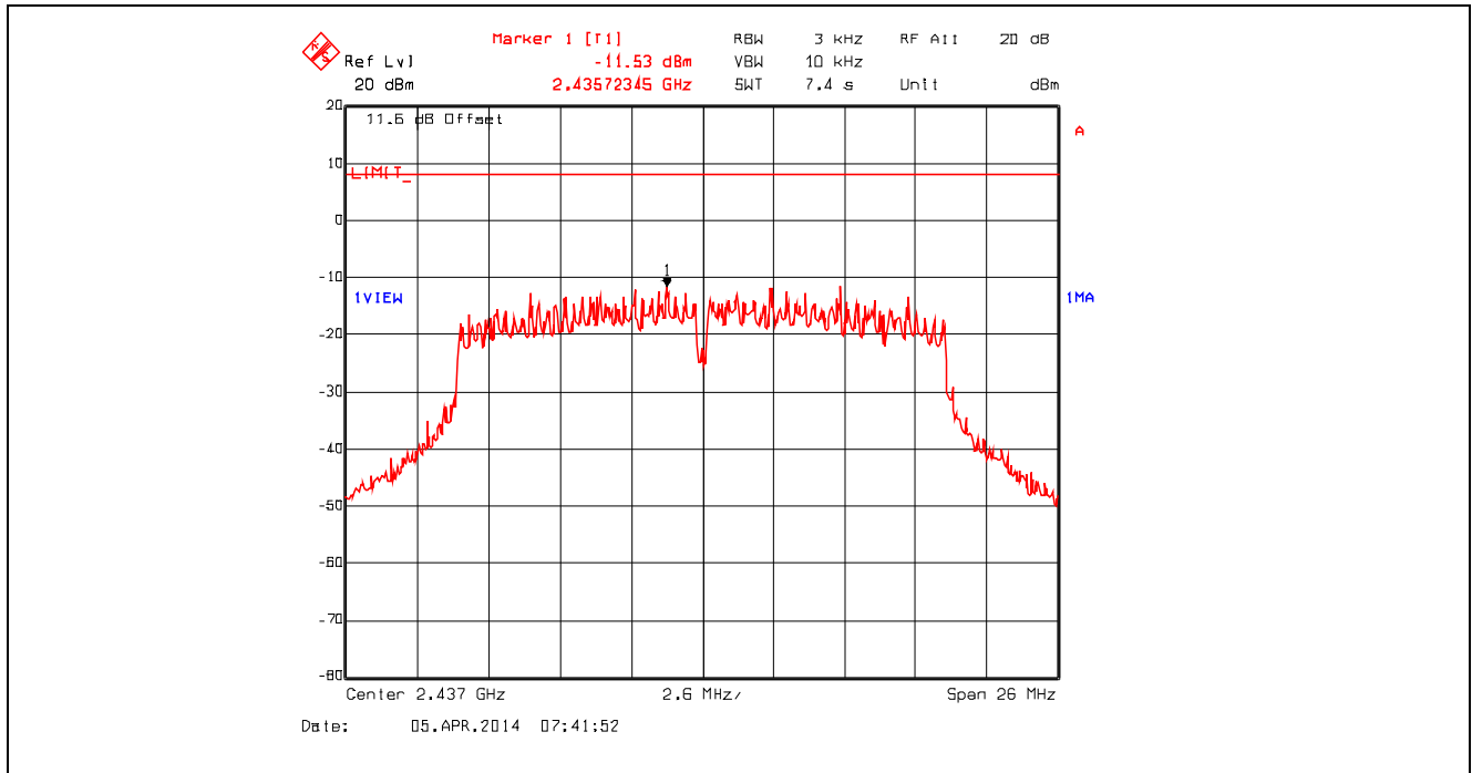
Plot 5.6.4.32. Power Spectral Density, 802.11n 800ns, 65 Mbps 64-QAM 5/6, 2437 MHz
