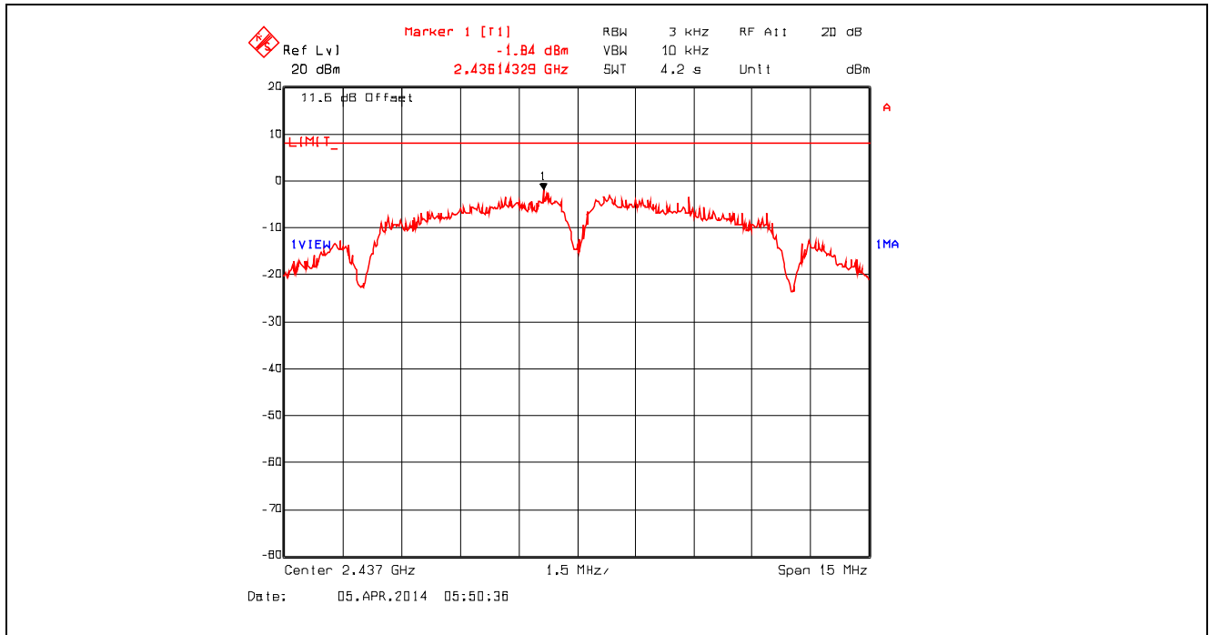
Plot 5.6.4.2. Power Spectral Density, 802.11b, 1 Mbps DBPSK, 2437 MHz
