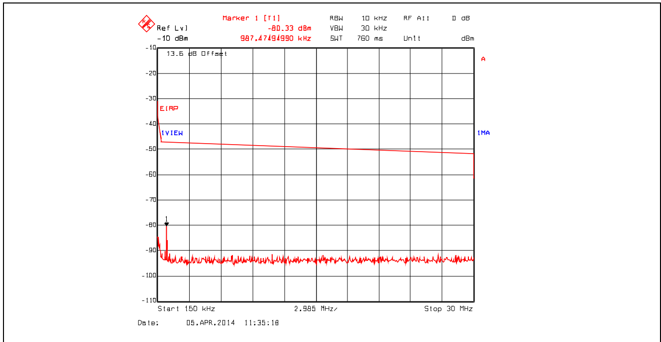
Plot 5.4.4.3.42. Conducted Spurious Emissions – Restricted Bands 802.11n, 6.5 Mbps, 2462 MHz, 150 kHz - 30 MHz, Peak Detector with Band (Notch) Reject Filter
