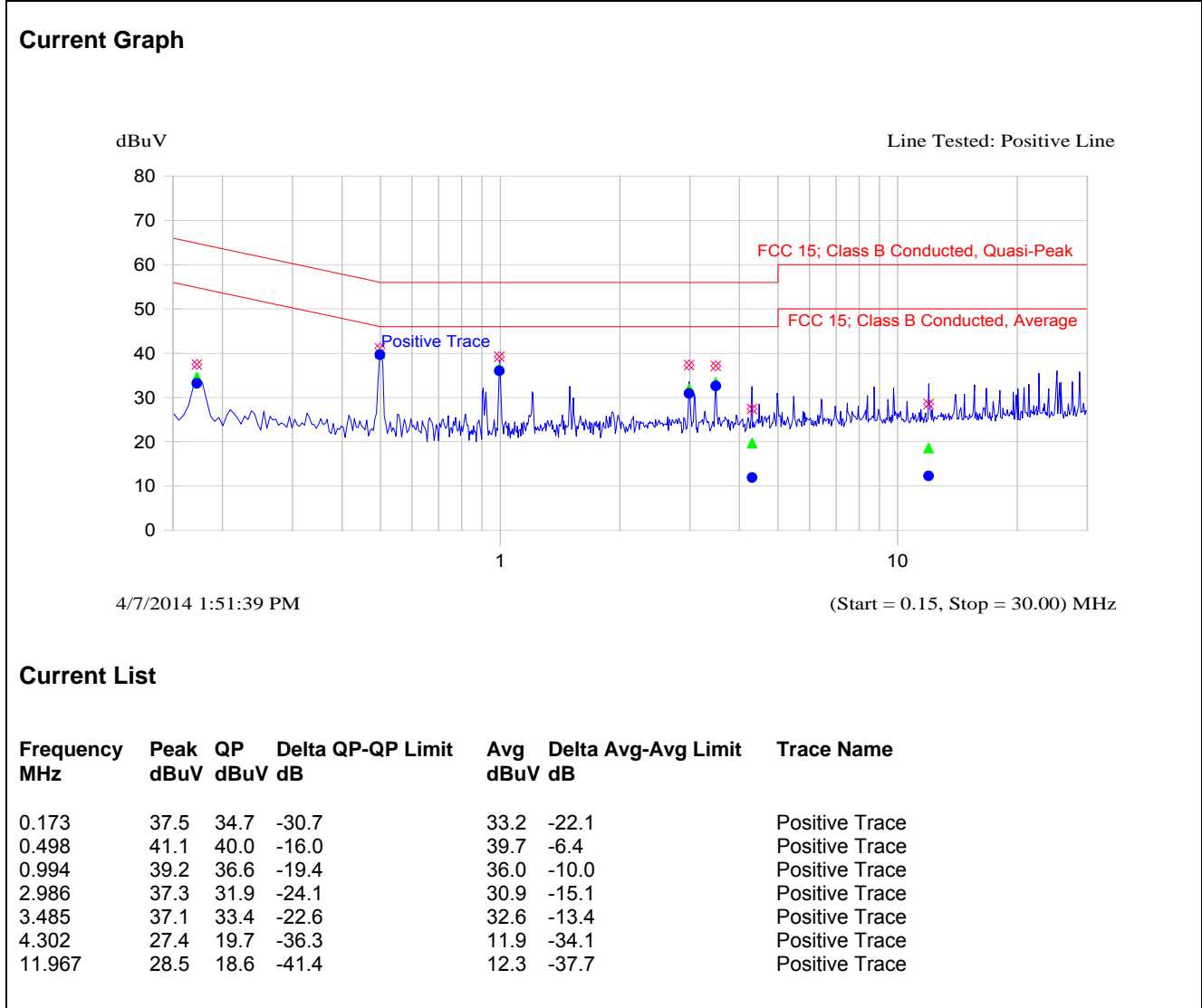
Plot 5.1.4.3. Power Line Conducted Emissions; Line Voltage: 24 V DC; Line Tested: Positive, Tx Mode
