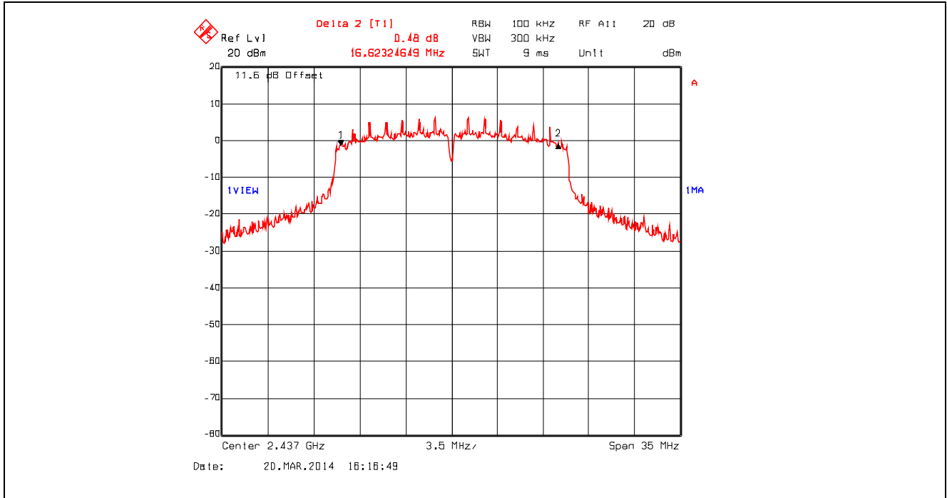
Plot 5.2.4.23. 6 dB Bandwidth, 802.11n 800ns, 6.5 Mbps BPSK1/2, 2437 MHz
