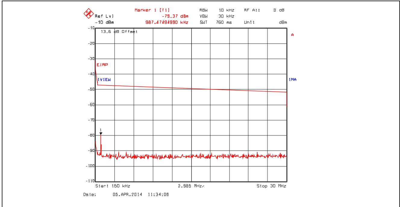
Plot 5.4.4.3.37. Conducted Spurious Emissions – Restricted Bands 802.11n, 6.5 Mbps, 2437 MHz, 150 kHz - 30 MHz, Peak Detector with Band (Notch) Reject Filter
