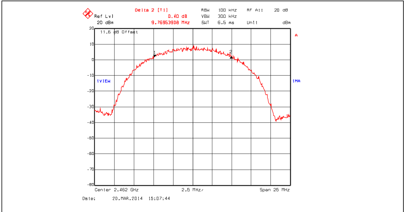
Plot 5.2.4.9. 6 dB Bandwidth, 802.11b, 11 Mbps CCK, 2462 MHz
