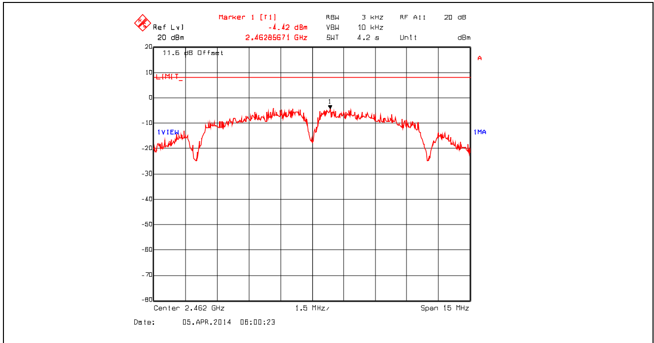
Plot 5.6.4.6. Power Spectral Density, 802.11b, 2 Mbps DQPSK, 2462 MHz
