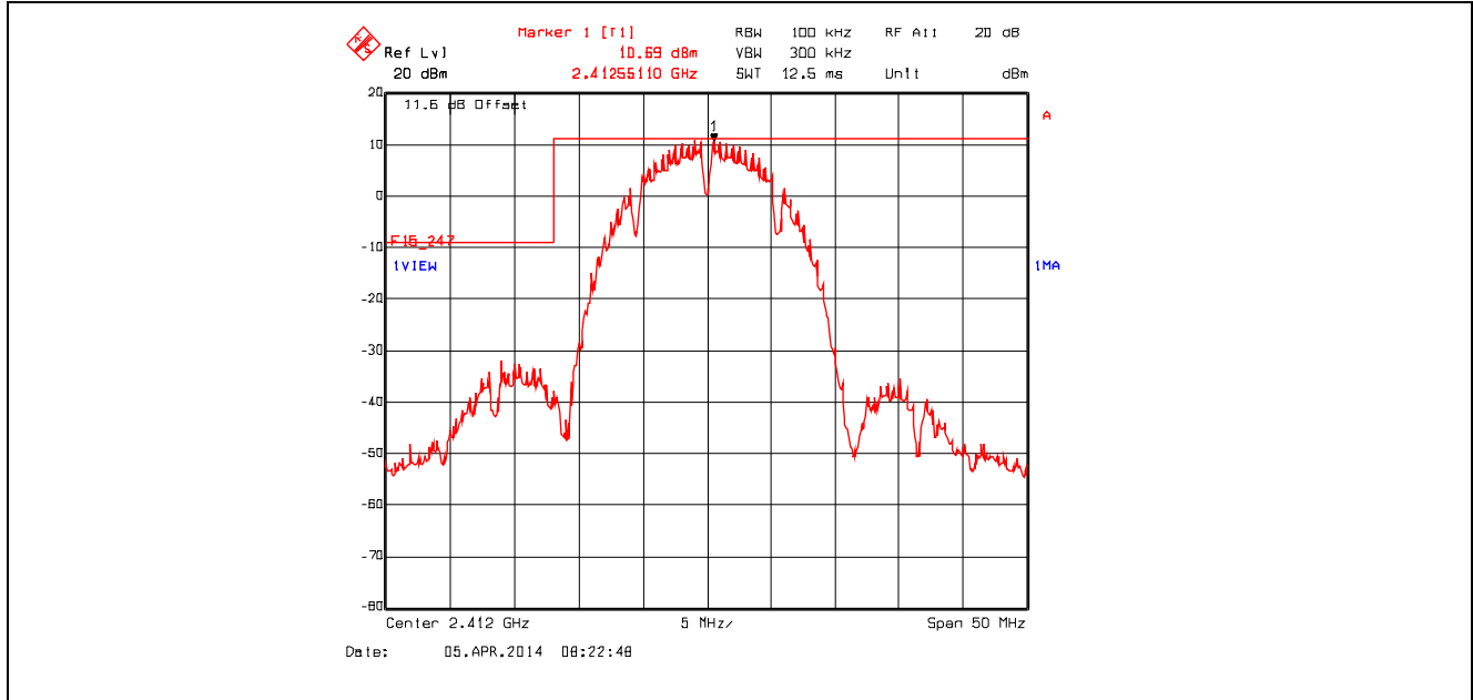
Plot 5.4.4.1.1. Band-Edge RF Conducted Emissions, Lower Band-edge, 2412 MHz, 802.11b, 1 Mbps
