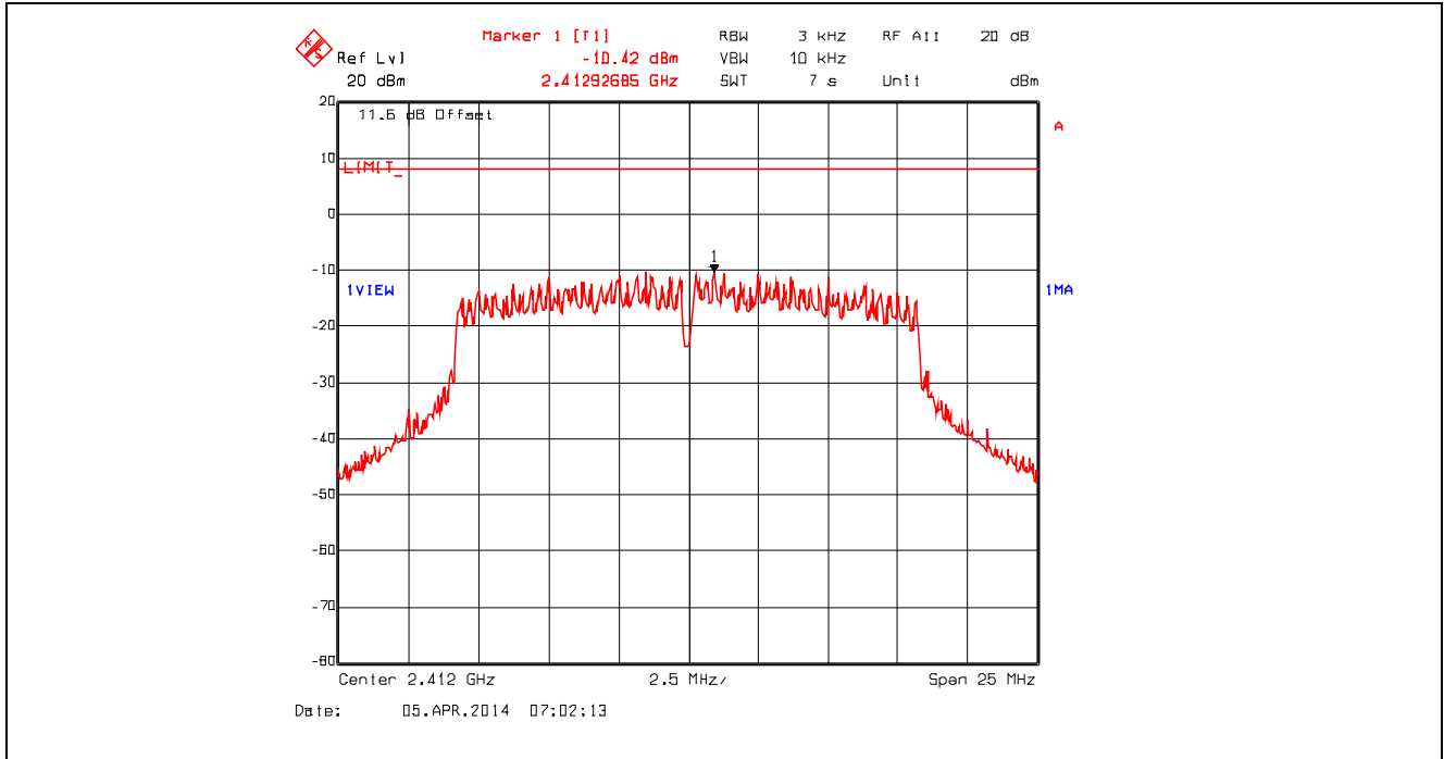
Plot 5.6.4.19. Power Spectral Density, 802.11g, 54 Mbps 64-QAM, 2412 MHz
