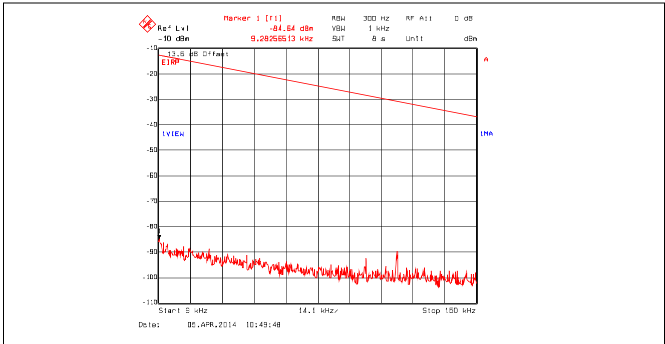
Plot 5.4.4.3.16. Conducted Spurious Emissions – Restricted Bands 802.11g, 9 Mbps, 2412 MHz, 9 kHz - 150 kHz, Peak Detector with Band (Notch) Reject Filter
