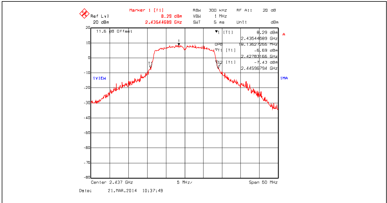
Plot 5.2.4.44. 99% Occupied Bandwidth, 802.11g, 9 Mbps BPSK, 2437 MHz
