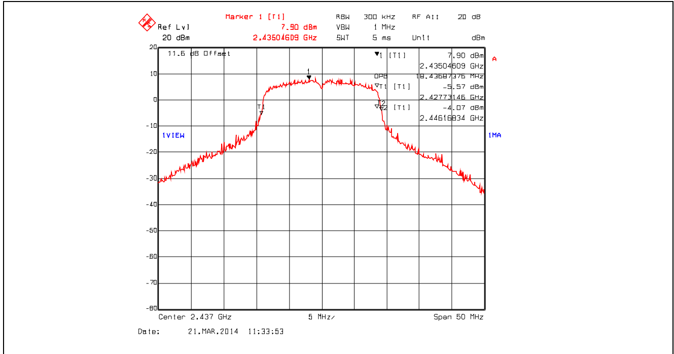
Plot 5.2.4.59. 99% Occupied Bandwidth, 802.11n 800ns, 19.5 Mbps QPSK 3/4, 2437 MHz
