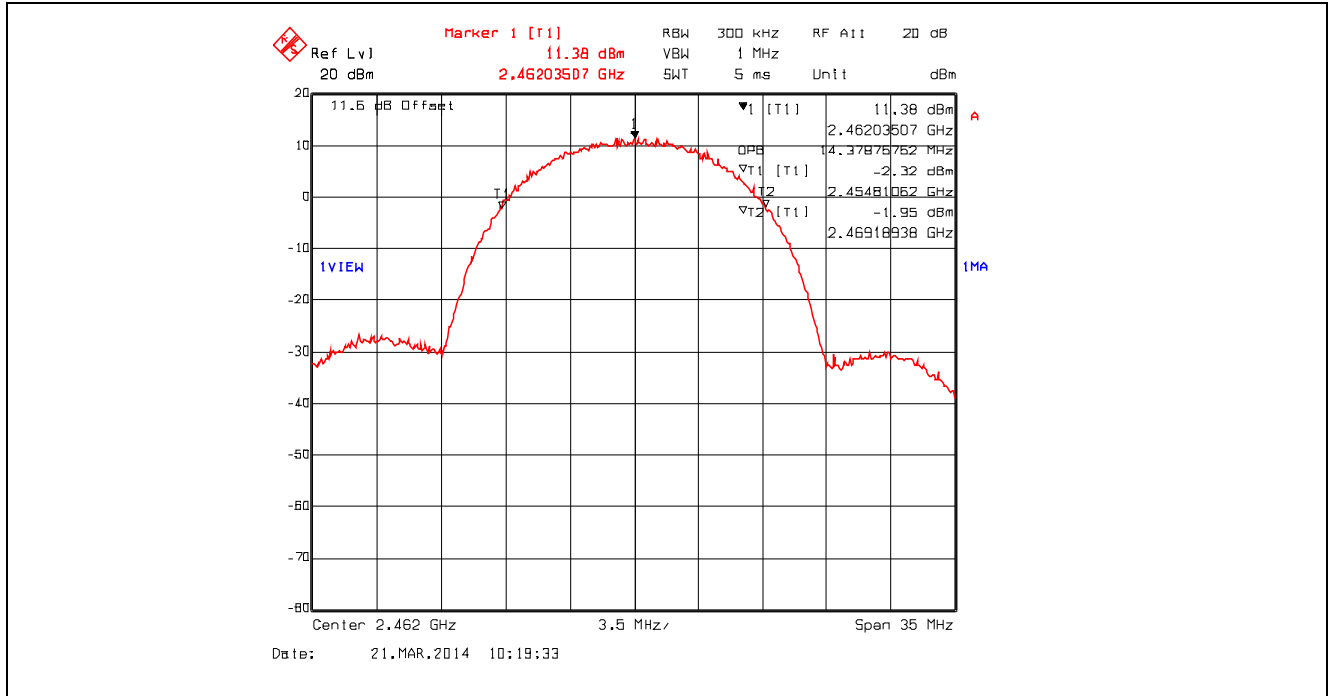
Plot 5.2.4.42. 99% Occupied Bandwidth, 802.11b, 11 Mbps CCK, 2462 MHz
