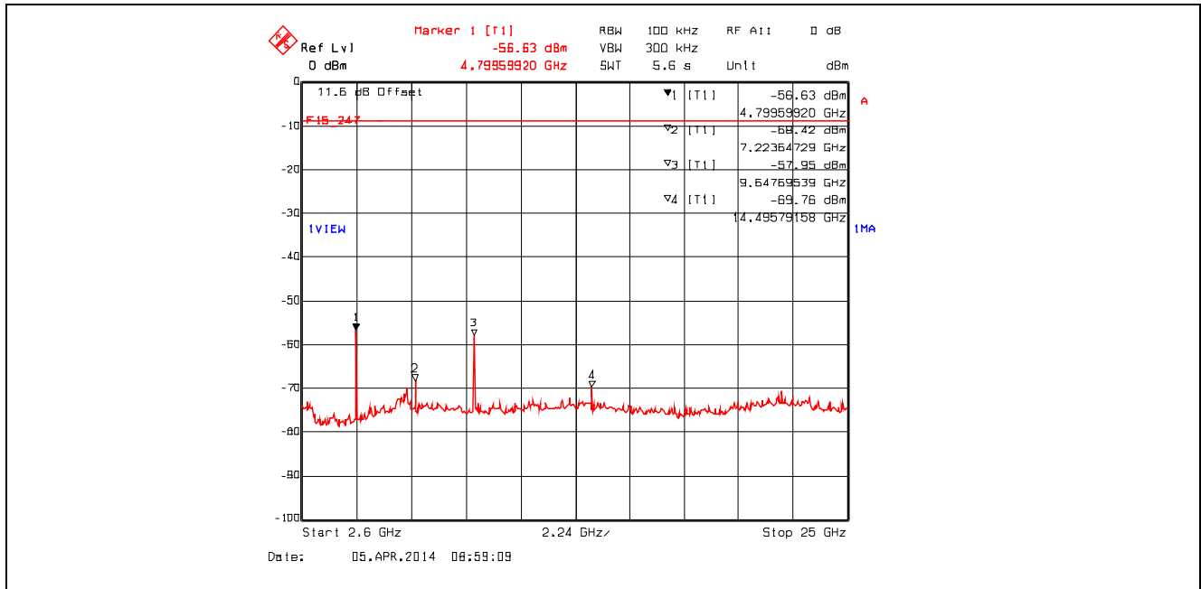
Plot 5.4.4.2.2. Conducted Spurious Emissions - Non Restricted Frequency Bands 802.11b, 2412 MHz, 1 Mbps, 2.6 GHz - 25 GHz
