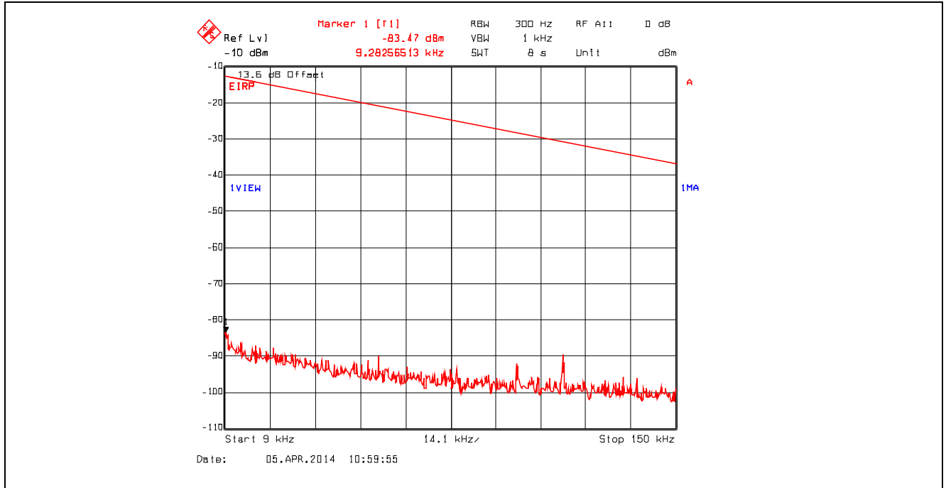
Plot 5.4.4.3.36. Conducted Spurious Emissions – Restricted Bands 802.11n, 6.5 Mbps, 2437 MHz, 9 kHz - 150 kHz, Peak Detector with Band (Notch) Reject Filter
