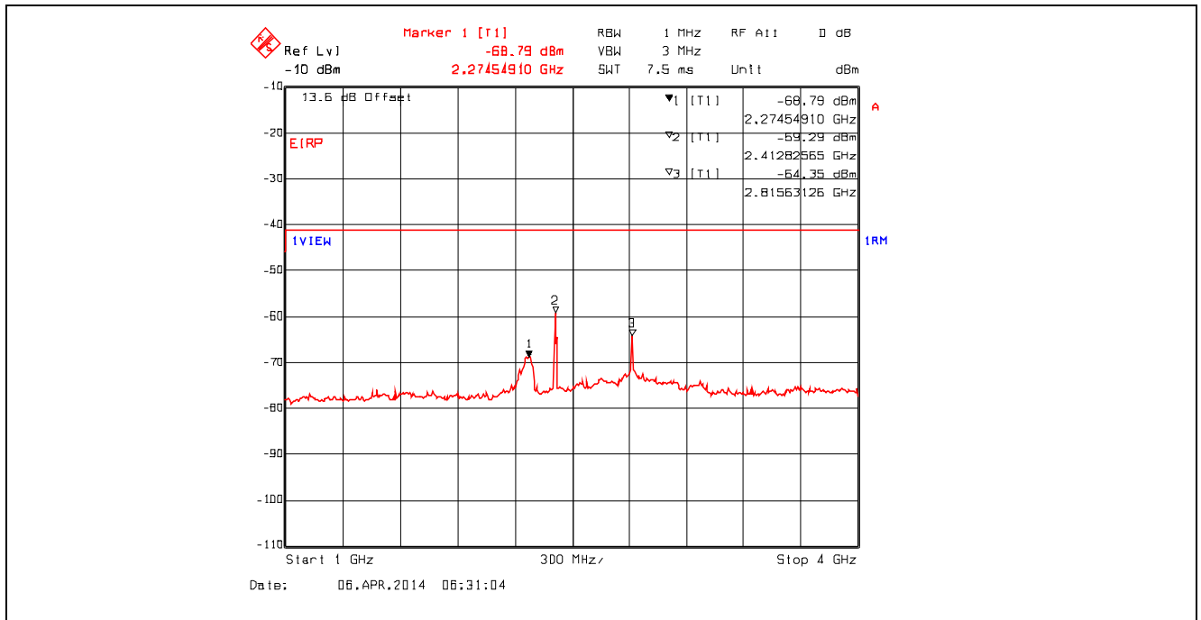
Plot 5.4.4.3.4. Conducted Spurious Emissions – Restricted Bands 802.11b, 1 Mbps, 2412 MHz, 1 GHz - 4 GHz, RMS Detector with Band (Notch) Reject Filter
