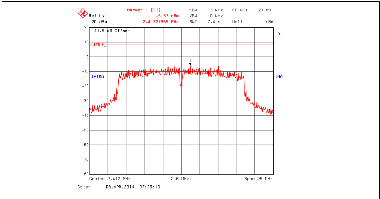
Plot 5.6.4.22. Power Spectral Density, 802.11n 800ns, 6.5 Mbps BPSK1/2, 2412 MHz
