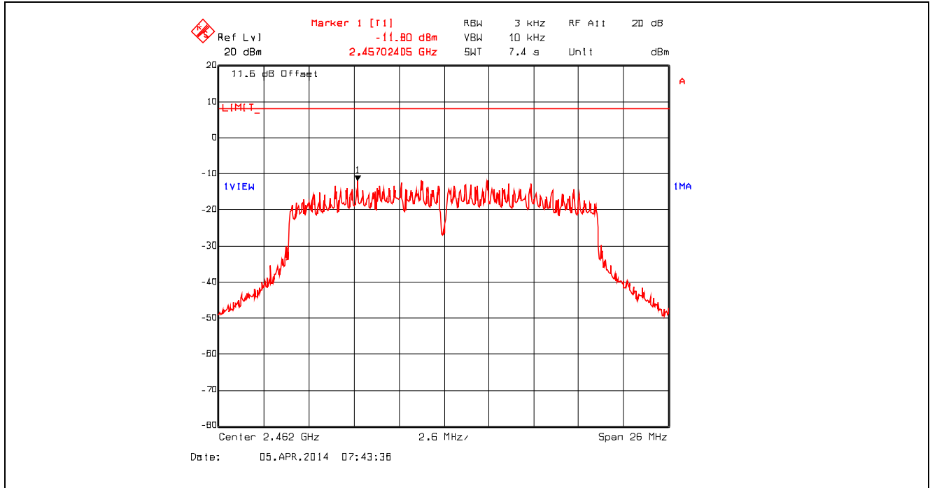
Plot 5.6.4.33. Power Spectral Density, 802.11n 800ns, 65 Mbps 64-QAM 5/6, 2462 MHz
