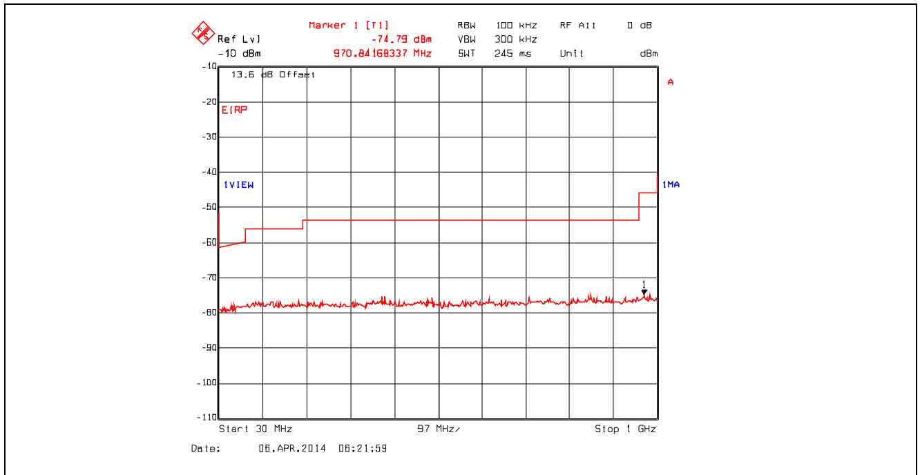
Plot 5.4.4.3.8. Conducted Spurious Emissions – Restricted Bands, Bands 802.11b, 1 Mbps, 2437 MHz, 30 MHz - 1 GHz, Peak Detector with Band (Notch) Reject Filter
