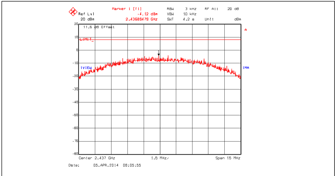
Plot 5.6.4.8. Power Spectral Density, 802.11b, 11 Mbps CCK, 2437 MHz
