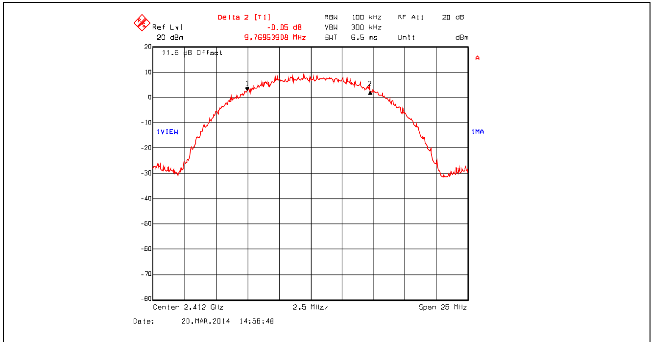
Plot 5.2.4.7. 6 dB Bandwidth, 802.11b, 11 Mbps CCK, 2412 MHz
