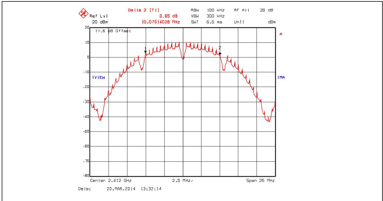
Plot 5.2.4.1. 6 dB Bandwidth, 802.11b, 1 Mbps DBPSK, 2412 MHz
