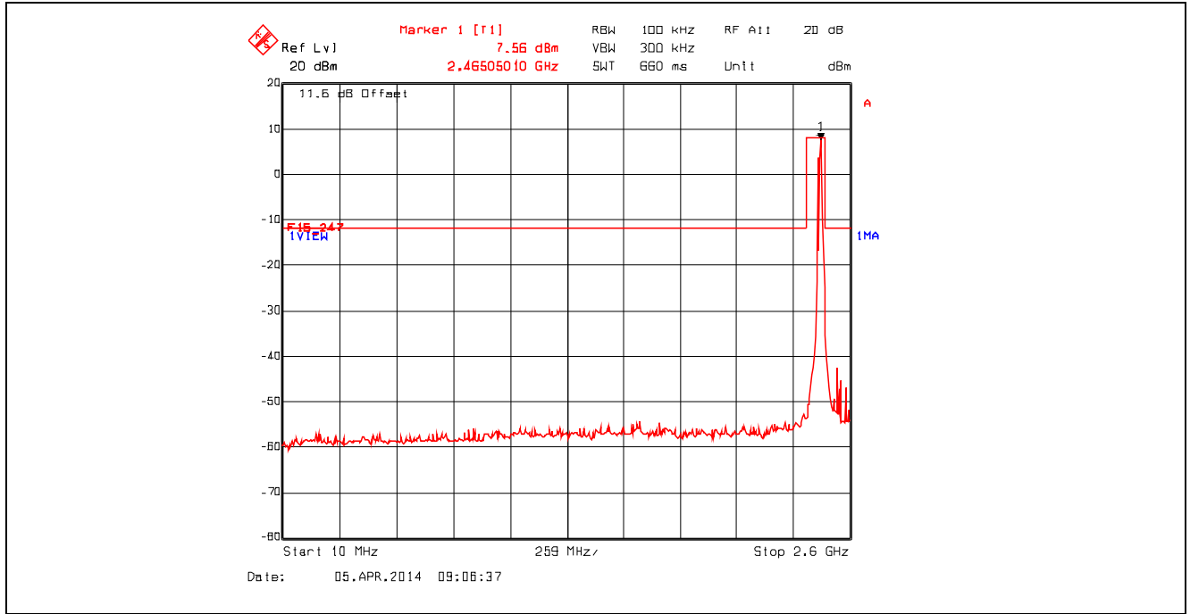
Plot 5.4.4.2.11. Conducted Spurious Emissions - Non Restricted Frequency Bands 802.11g, 2462 MHz, 9 Mbps, 10 MHz - 2.6 GHz
