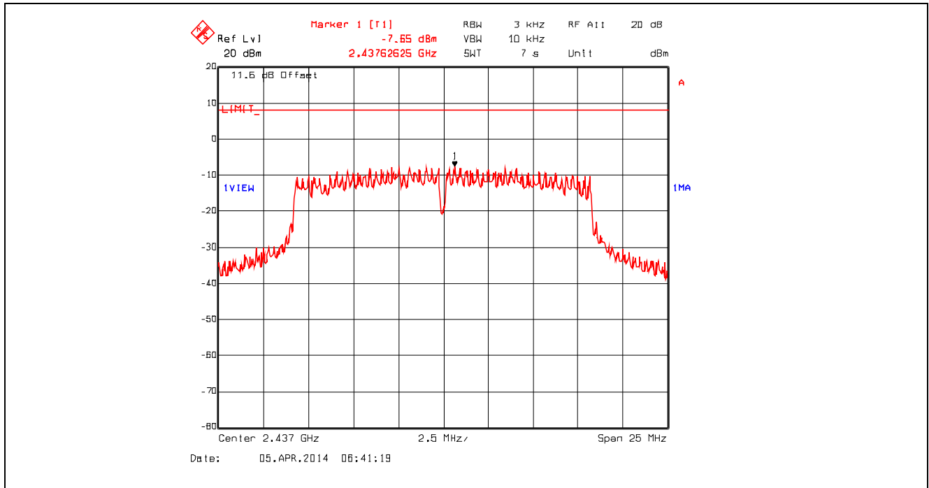
Plot 5.6.4.11. Power Spectral Density, 802.11g, 9 Mbps BPSK, 2437 MHz
