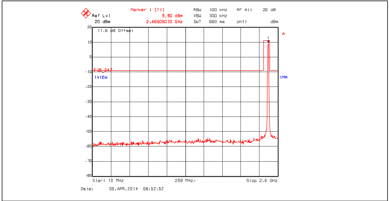
Plot 5.4.4.2.5. Conducted Spurious Emissions - Non Restricted Frequency Bands 802.11b, 2462 MHz, 1 Mbps, 10 MHz - 2.6 GHz
