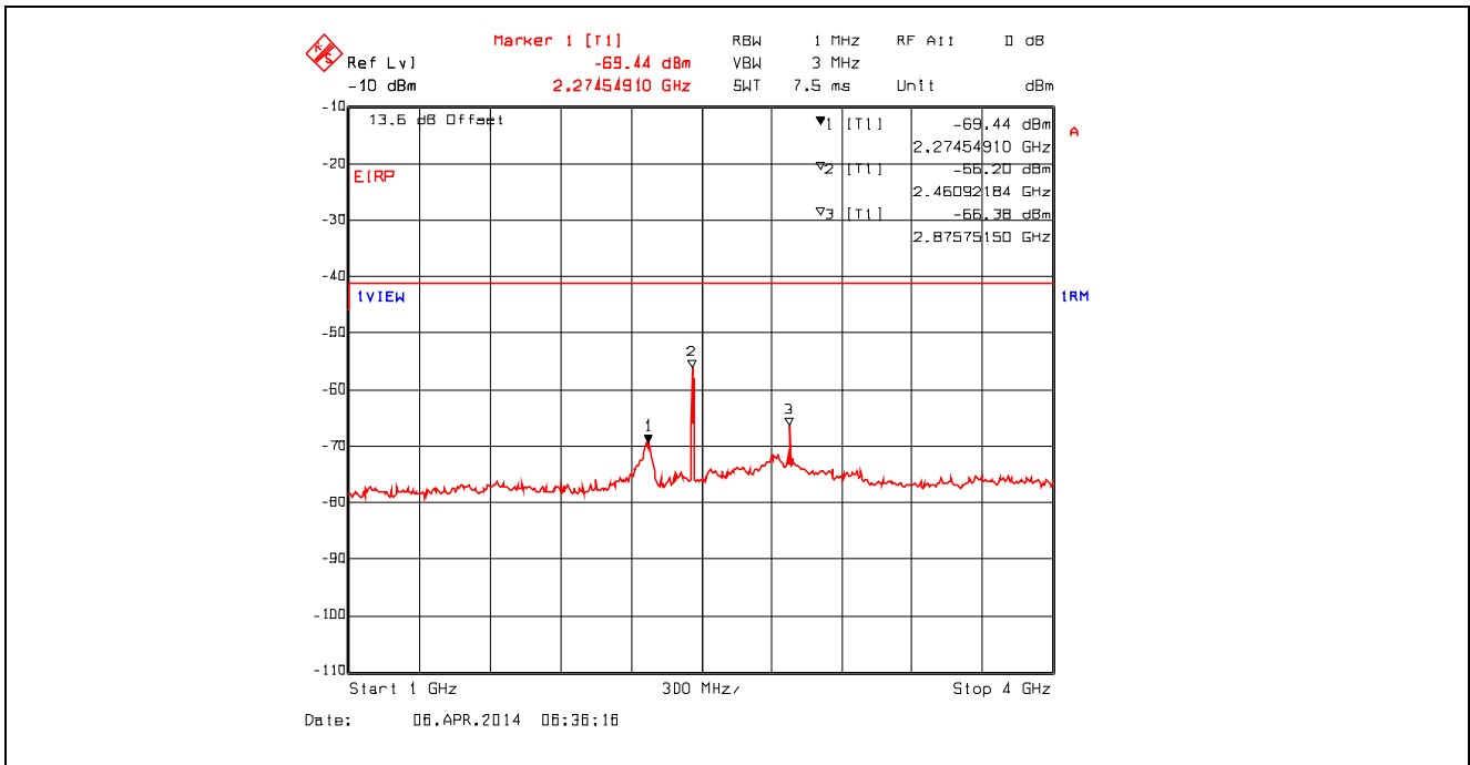
Plot 5.4.4.3.14. Conducted Spurious Emissions – Restricted Bands 802.11b, 1 Mbps, 2462 MHz, 1 GHz - 4 GHz, RMS Detector with Band (Notch) Reject Filter
