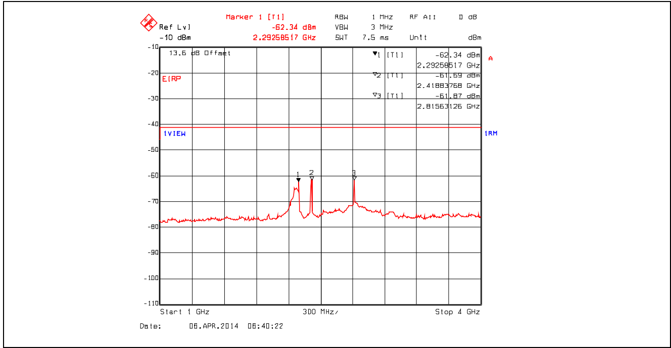
Plot 5.4.4.3.19. Conducted Spurious Emissions – Restricted Bands 802.11g, 9 Mbps, 2412 MHz, 1 GHz - 4 GHz, RMS Detector with Band (Notch) Reject Filter
