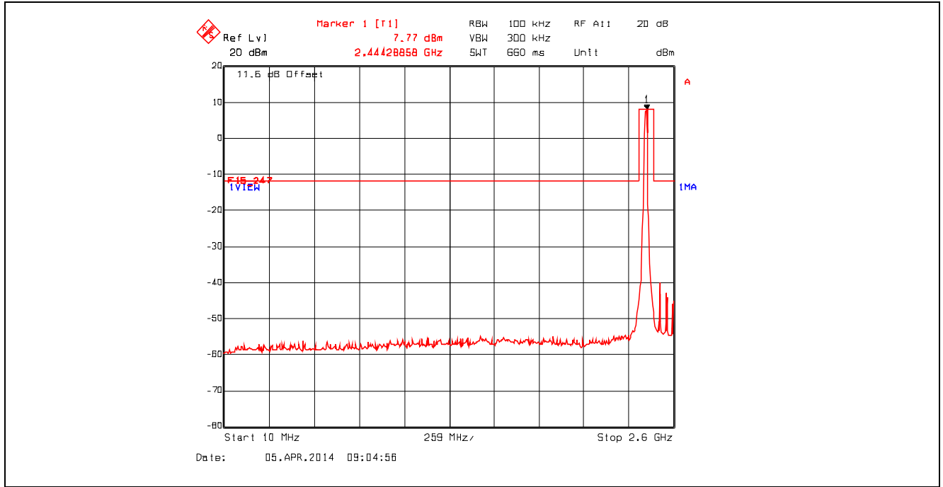
Plot 5.4.4.2.9. Conducted Spurious Emissions - Non Restricted Frequency Bands 802.11g, 2437 MHz, 9 Mbps, 10 MHz - 2.6 GHz
