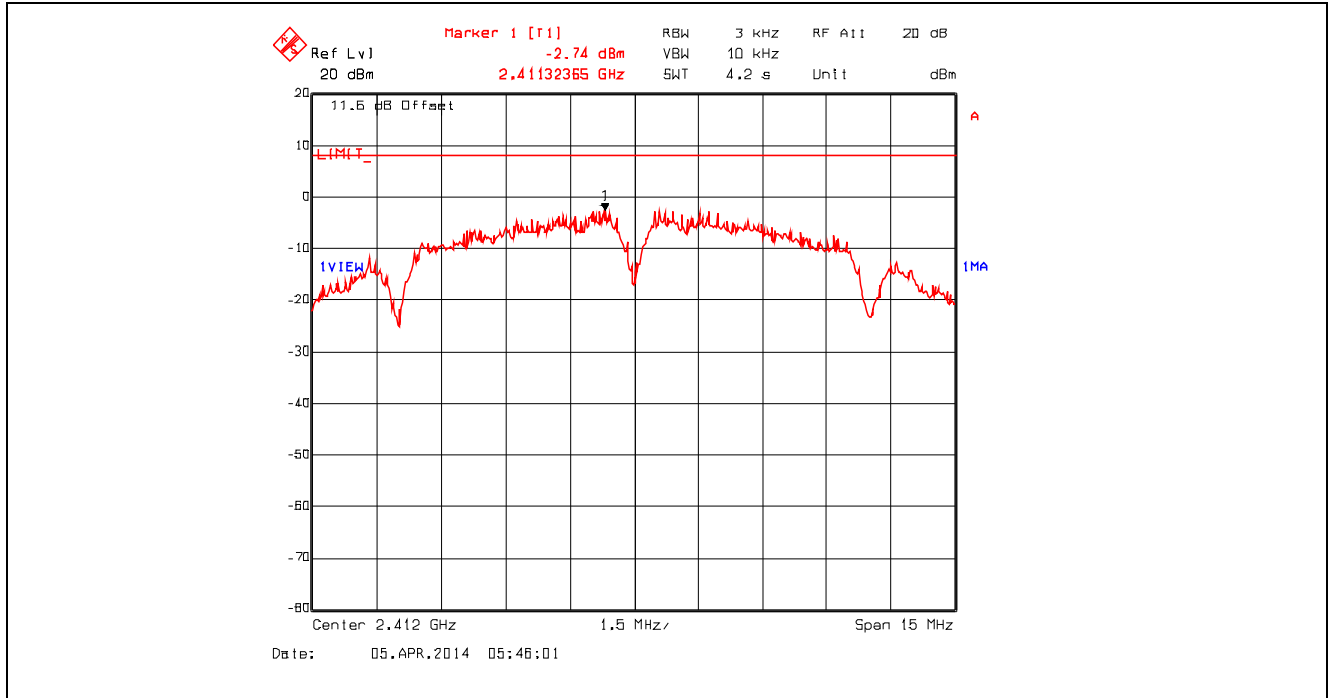
Plot 5.6.4.1. Power Spectral Density, 802.11b, 1 Mbps DBPSK, 2412 MHz
