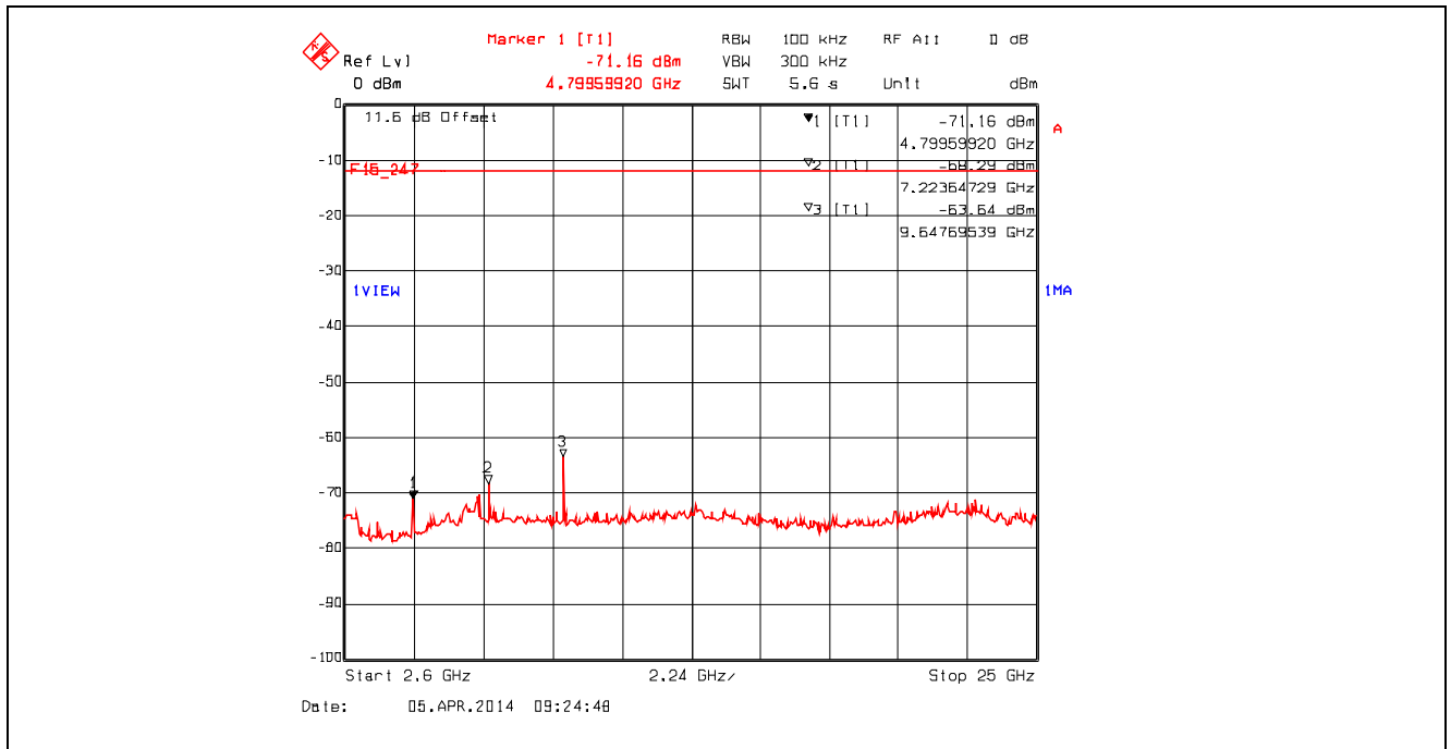
Plot 5.4.4.2.14. Conducted Spurious Emissions - Non Restricted Frequency Bands 802.11n, 2412 MHz, 6.5 Mbps, 2.6 GHz - 25 GHz
