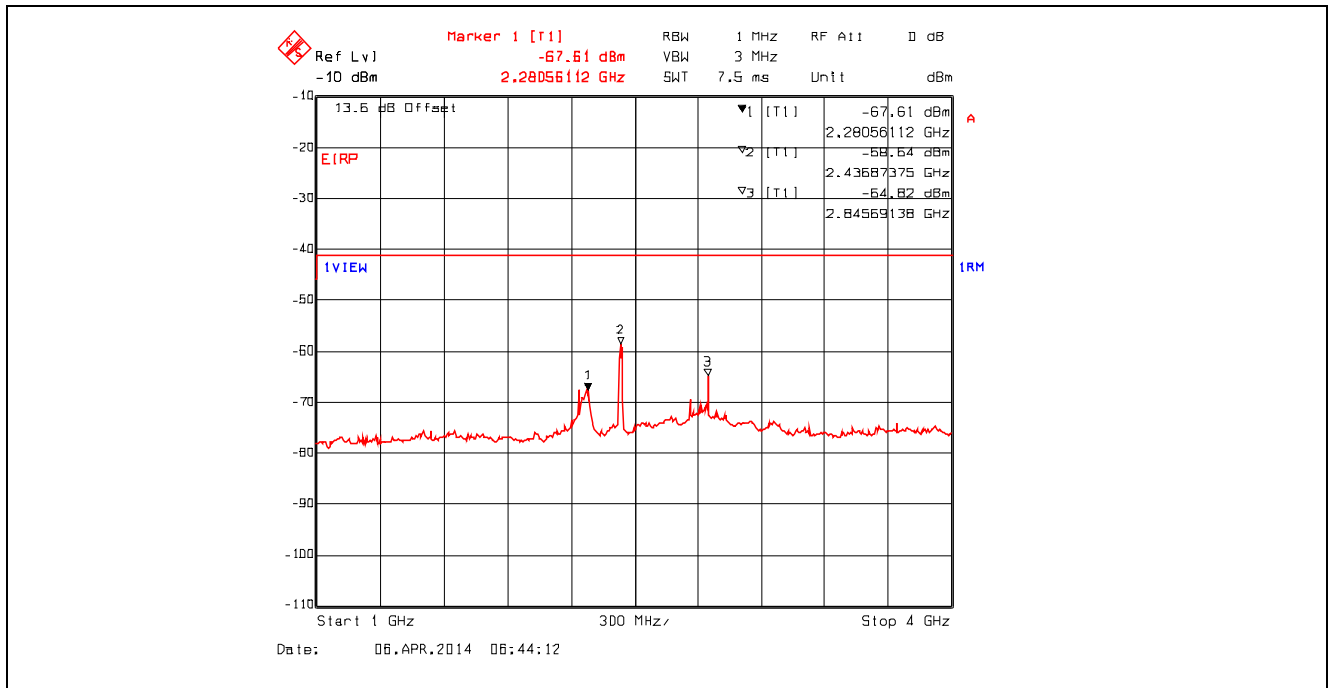
Plot 5.4.4.3.24. Conducted Spurious Emissions – Restricted Bands 802.11g, 9 Mbps, 2437 MHz, 1 GHz - 4 GHz, RMS Detector with Band (Notch) Reject Filter
