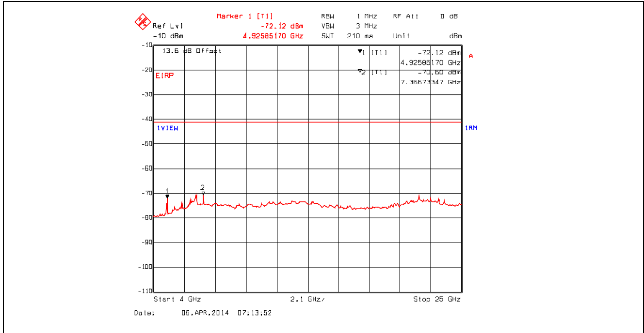
Plot 5.4.4.3.15. Conducted Spurious Emissions – Restricted Bands 802.11b, 1 Mbps, 2462 MHz, 4 GHz - 25 GHz, RMS Detector with High Pass Filter
