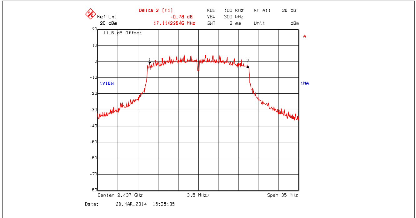
Plot 5.2.4.29. 6 dB Bandwidth, 802.11n 800ns, 39 Mbps 16-QAM 3/4, 2437 MHz
