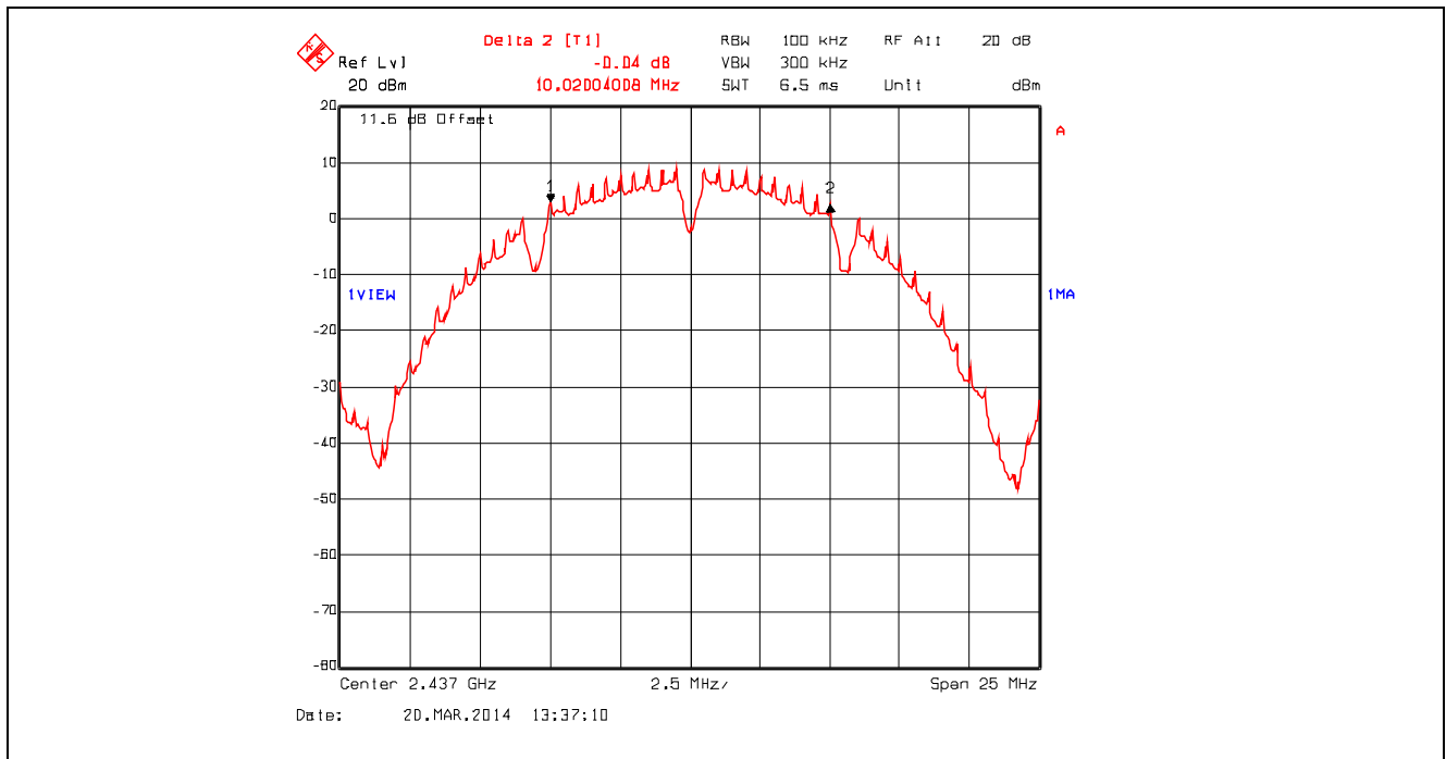
Plot 5.2.4.2. 6 dB Bandwidth, 802.11b, 1 Mbps DBPSK, 2437 MHz
