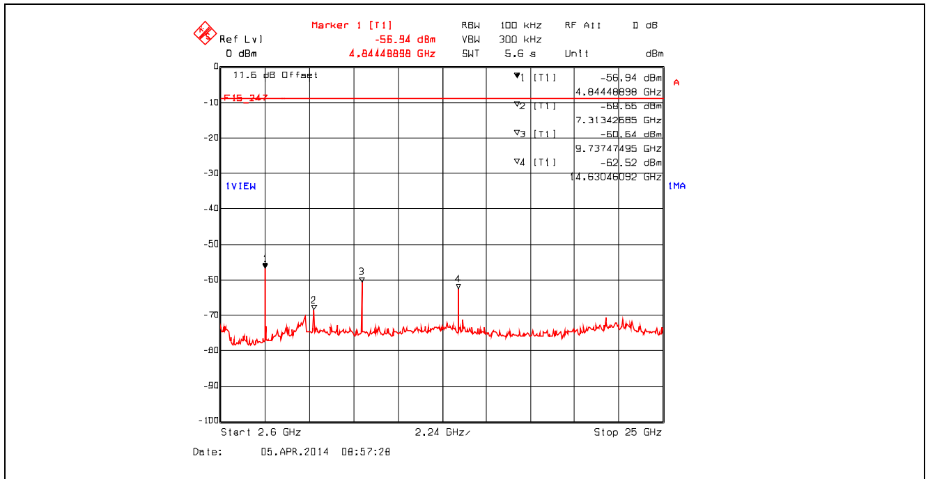
Plot 5.4.4.2.4. Conducted Spurious Emissions - Non Restricted Frequency Bands 802.11b, 2437 MHz, 1 Mbps, 2.6 GHz - 25 GHz
