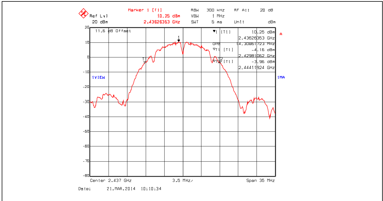
Plot 5.2.4.38. 99% Occupied Bandwidth, 802.11b, 2 Mbps DQPSK, 2437 MHz
