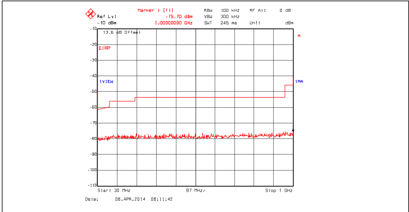
Plot 5.4.4.3.23. Conducted Spurious Emissions – Restricted Bands, Bands 802.11g, 9 Mbps, 2437 MHz, 30 MHz - 1 GHz, Peak Detector with Band (Notch) Reject Filter
