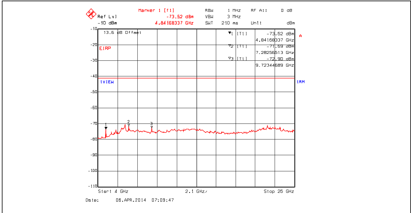
Plot 5.4.4.3.25. Conducted Spurious Emissions – Restricted Bands 802.11g, 9 Mbps, 2437 MHz, 4 GHz - 25 GHz, RMS Detector with High Pass Filter
