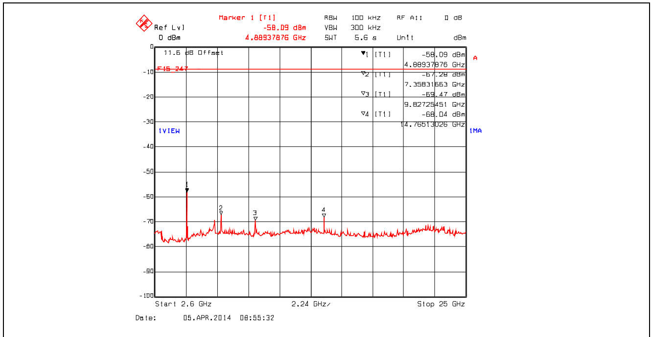
Plot 5.4.4.2.6. Conducted Spurious Emissions - Non Restricted Frequency Bands 802.11b, 2462 MHz, 1 Mbps, 2.6 GHz - 25 GHz
