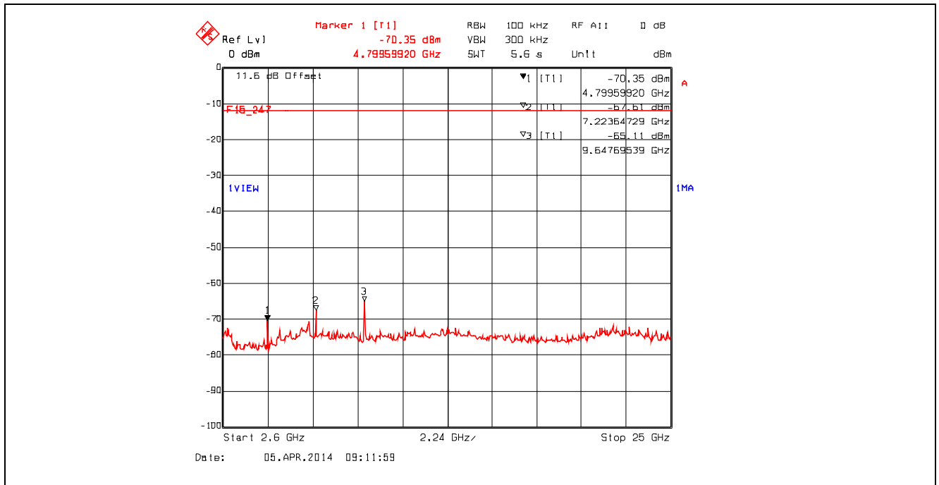
Plot 5.4.4.2.8. Conducted Spurious Emissions - Non Restricted Frequency Bands 802.11g, 2412 MHz, 9 Mbps, 2.6 GHz - 25 GHz
