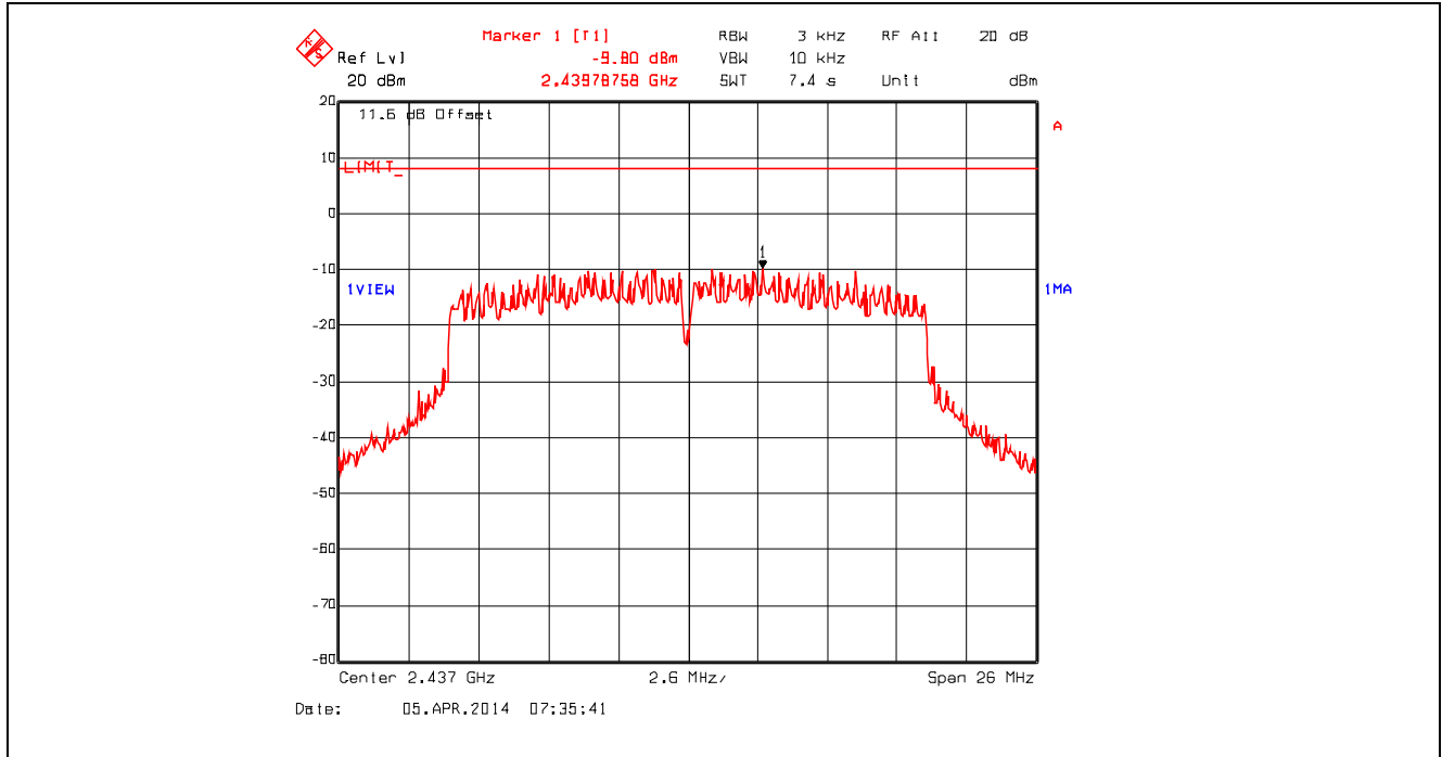
Plot 5.6.4.29. Power Spectral Density, 802.11n 800ns, 39 Mbps 16-QAM 3/4, 2437 MHz
