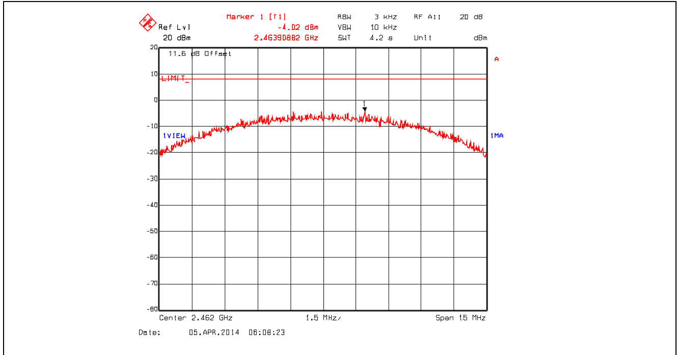
Plot 5.6.4.9. Power Spectral Density, 802.11b, 11 Mbps CCK, 2462 MHz
