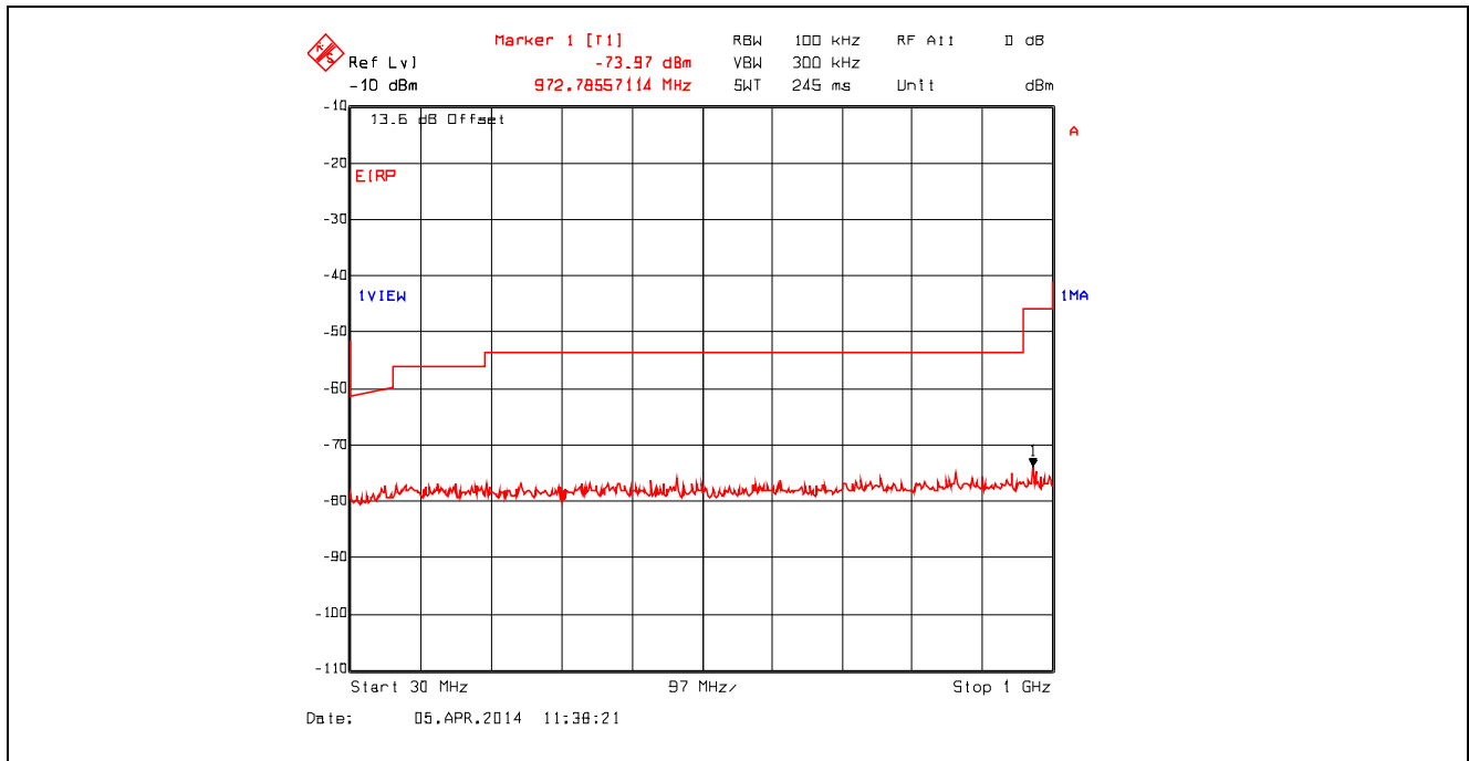
Plot 5.4.4.3.38. Conducted Spurious Emissions – Restricted Bands, Bands 802.11n, 6.5 Mbps, 2437 MHz, 30 MHz - 1 GHz, Peak Detector with Band (Notch) Reject Filter
