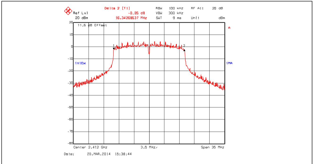
Plot 5.2.4.16. 6 dB Bandwidth, 802.11g, 36 Mbps 16-QAM, 2412 MHz
