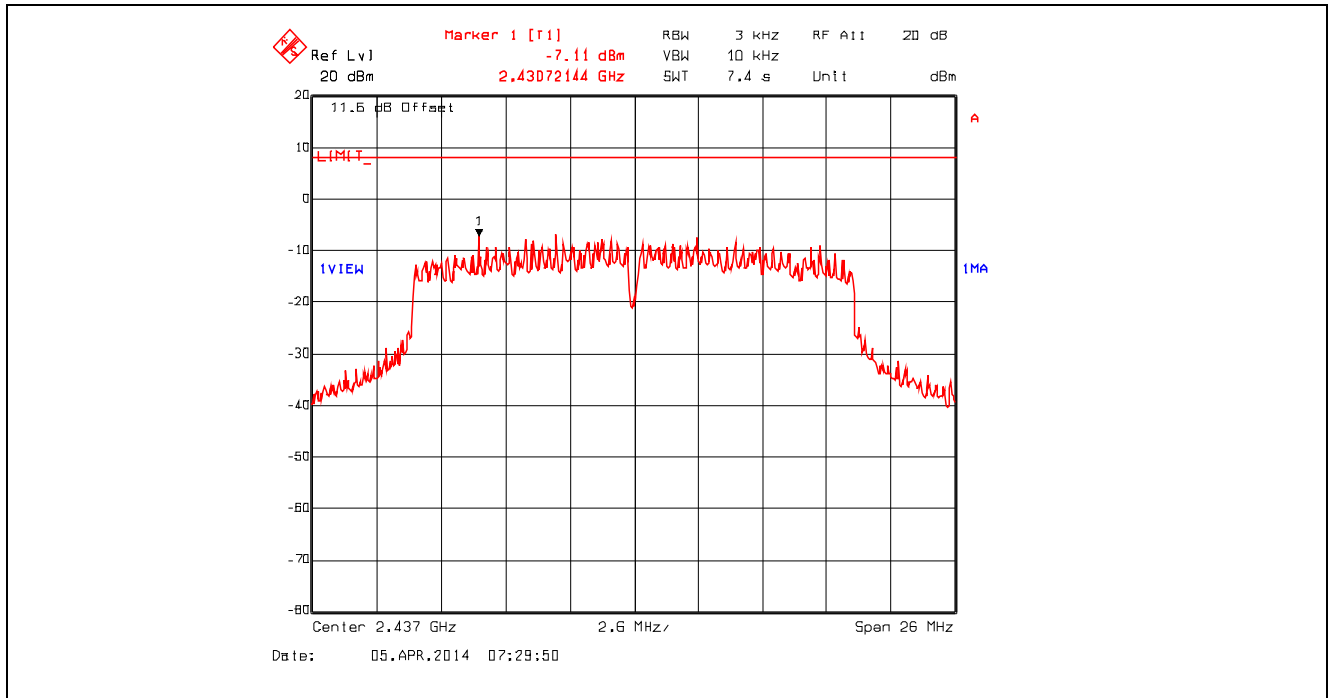
Plot 5.6.4.26. Power Spectral Density, 802.11n 800ns, 19.5 Mbps QPSK 3/4, 2437 MHz
