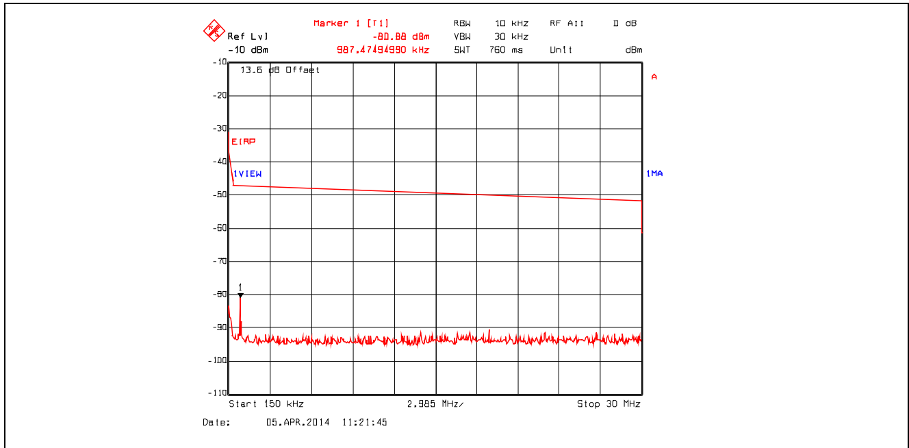
Plot 5.4.4.3.2. Conducted Spurious Emissions – Restricted Bands 802.11b, 1 Mbps, 2412 MHz, 150 kHz - 30 MHz, Peak Detector with Band (Notch) Reject Filter
