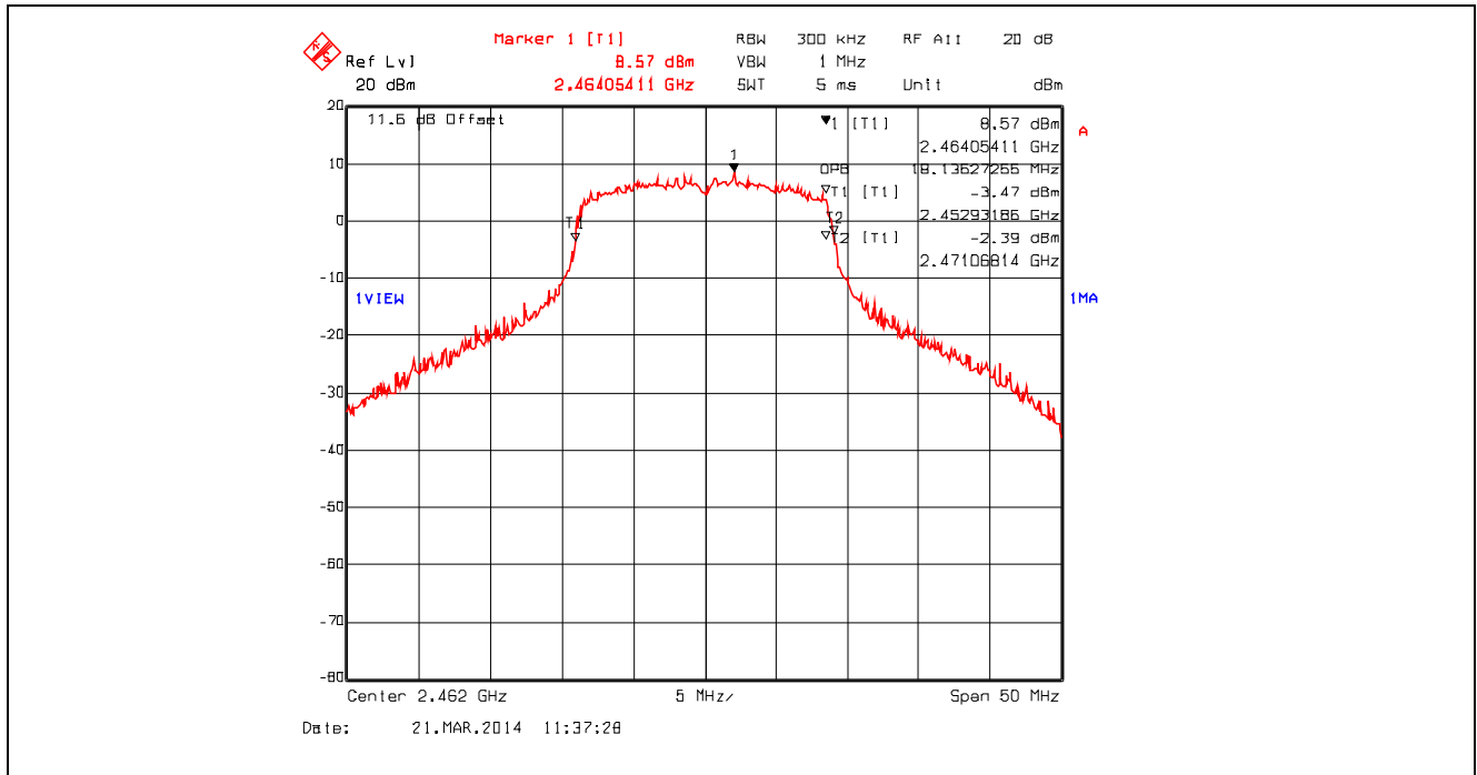
Plot 5.2.4.60. 99% Occupied Bandwidth, 802.11n 800ns, 19.5 Mbps QPSK 3/4, 2462 MHz
