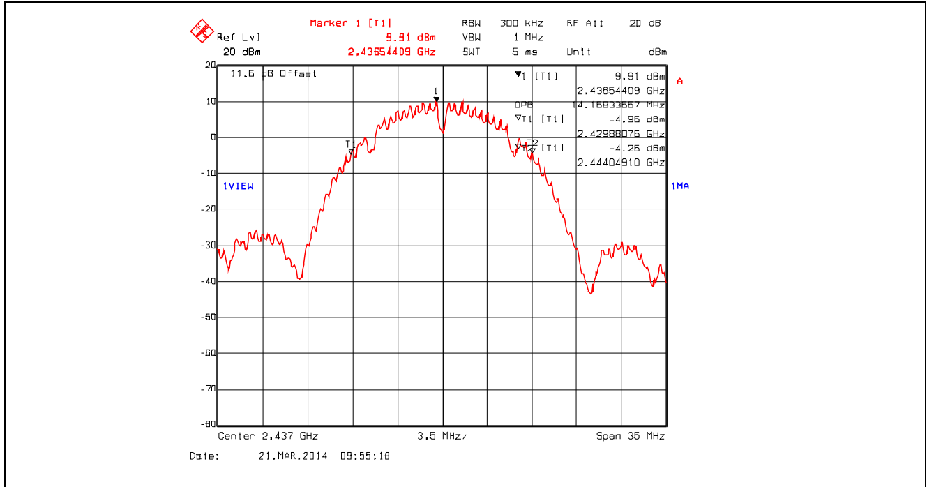
Plot 5.2.4.35. 99% Occupied Bandwidth, 802.11b, 1 Mbps DBPSK, 2437 MHz
