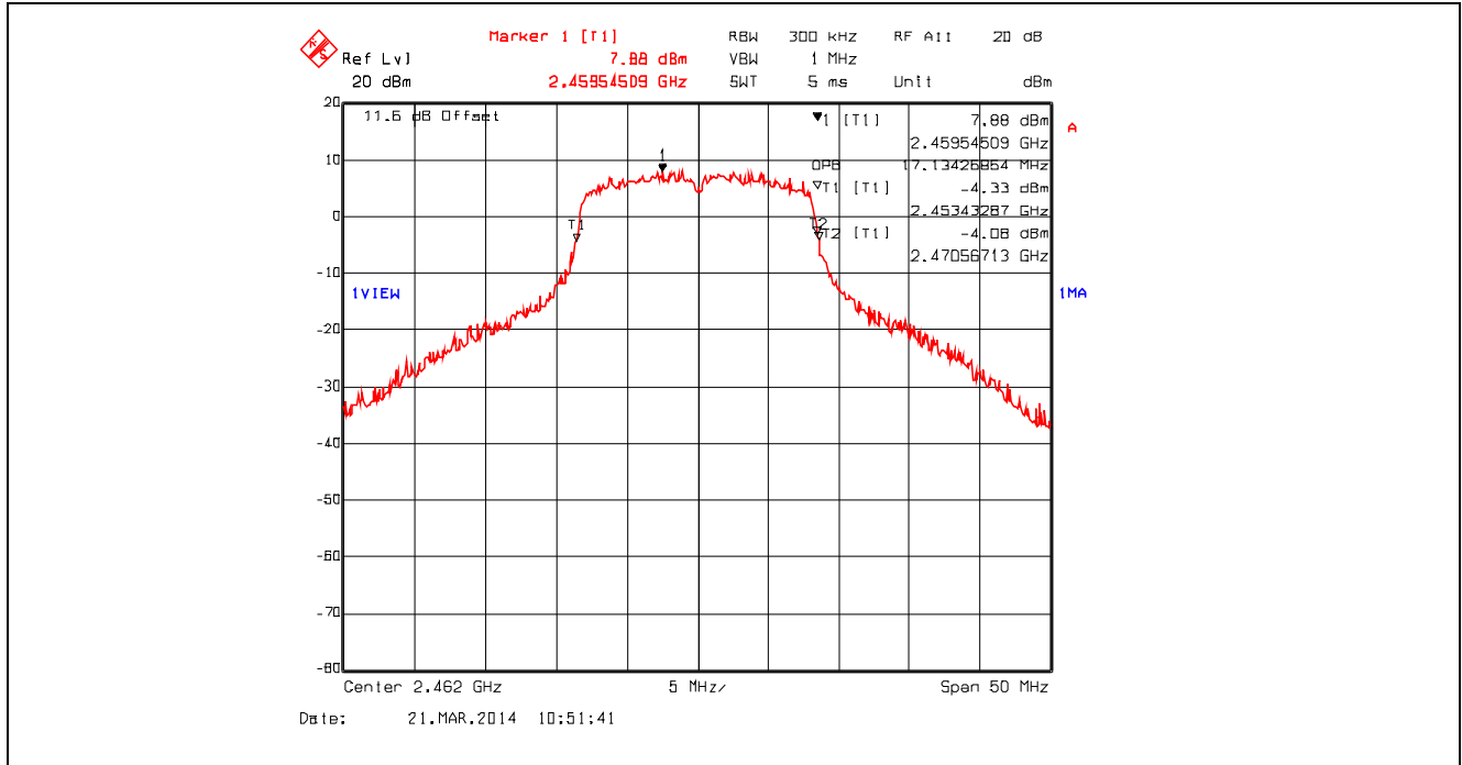
Plot 5.2.4.48. 99% Occupied Bandwidth, 802.11g, 18 Mbps QPSK, 2462 MHz
