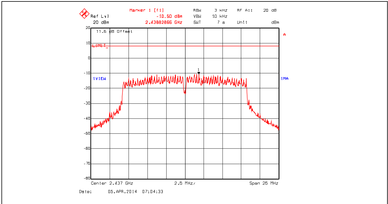
Plot 5.6.4.20. Power Spectral Density, 802.11g, 54 Mbps 64-QAM, 2437 MHz
