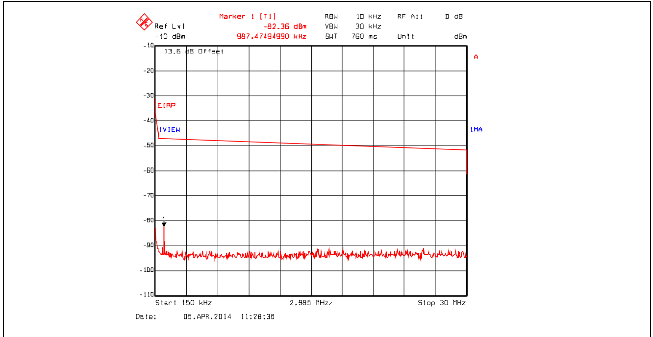
Plot 5.4.4.3.27. Conducted Spurious Emissions – Restricted Bands 802.11g, 9 Mbps, 2462 MHz, 150 kHz - 30 MHz, Peak Detector with Band (Notch) Reject Filter
