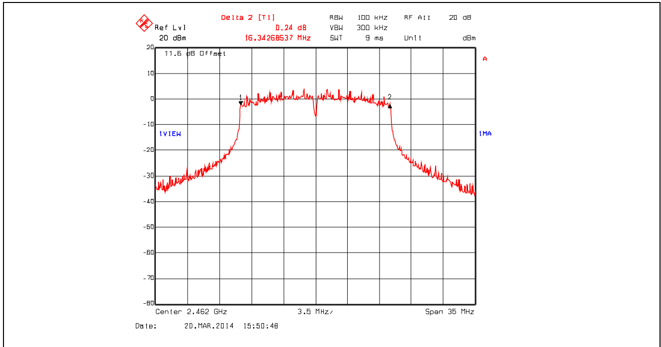
Plot 5.2.4.18. 6 dB Bandwidth, 802.11g, 36 Mbps 16-QAM, 2462 MHz
