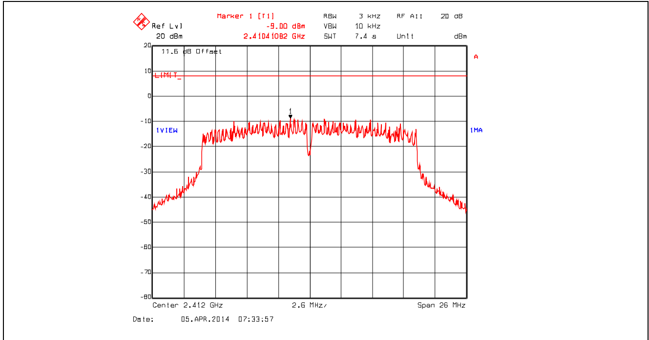
Plot 5.6.4.28. Power Spectral Density, 802.11n 800ns, 39 Mbps 16-QAM 3/4, 2412 MHz
