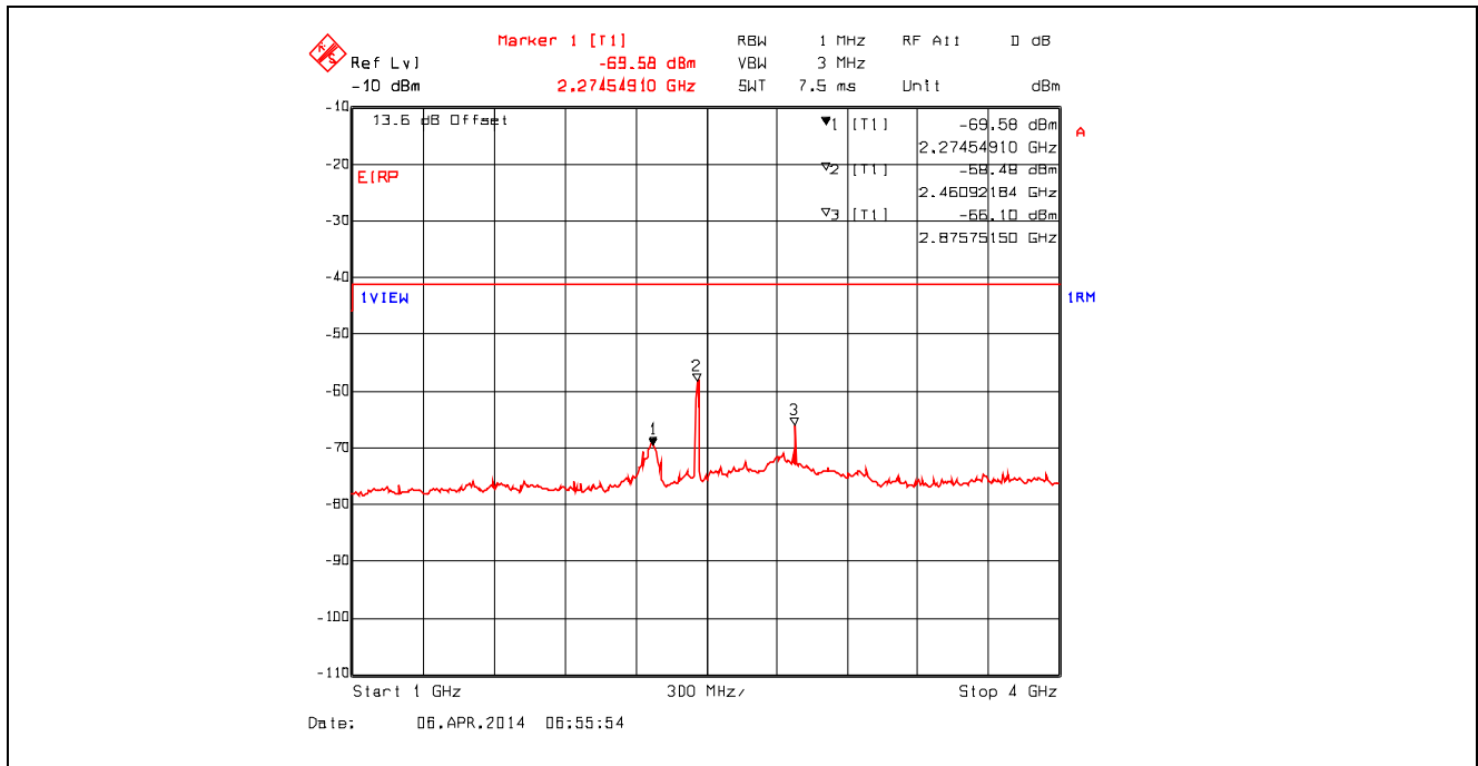
Plot 5.4.4.3.4. Conducted Spurious Emissions – Restricted Bands 802.11n, 6.5 Mbps, 2462 MHz, 1 GHz - 4 GHz, RMS Detector with Band (Notch) Reject Filter
