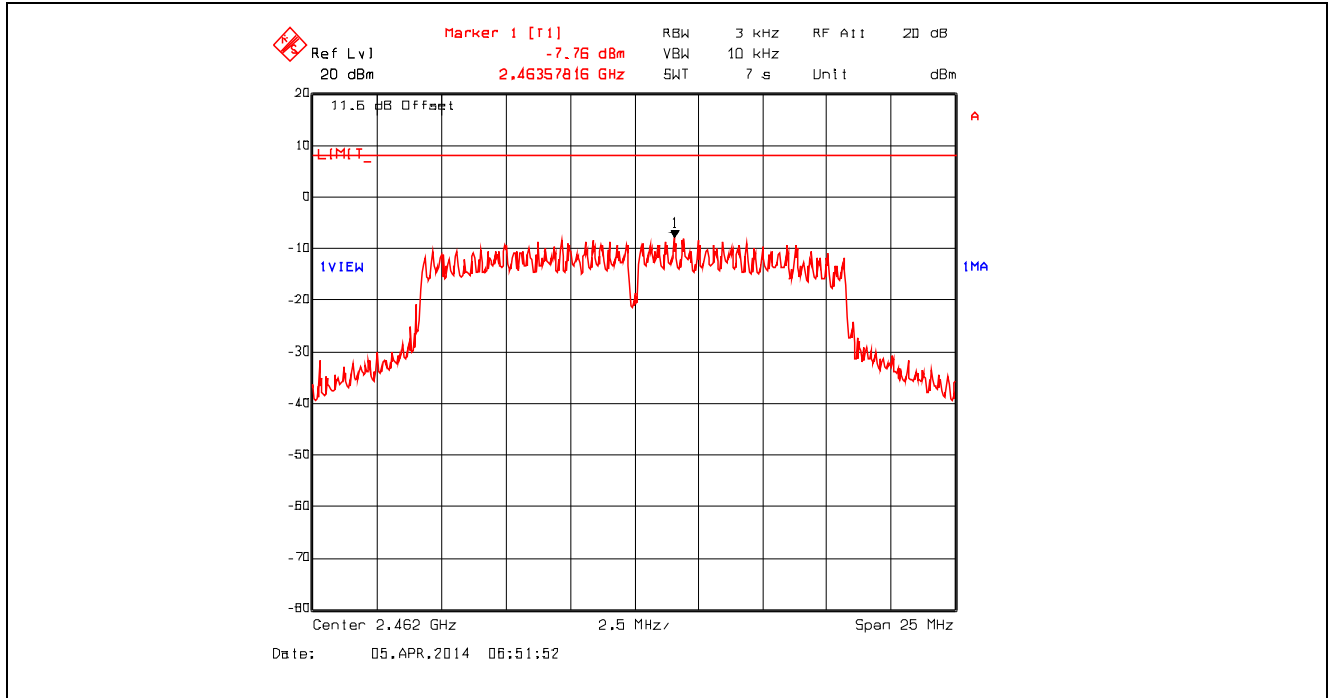
Plot 5.6.4.15. Power Spectral Density, 802.11g, 18 Mbps QPSK, 2462 MHz
