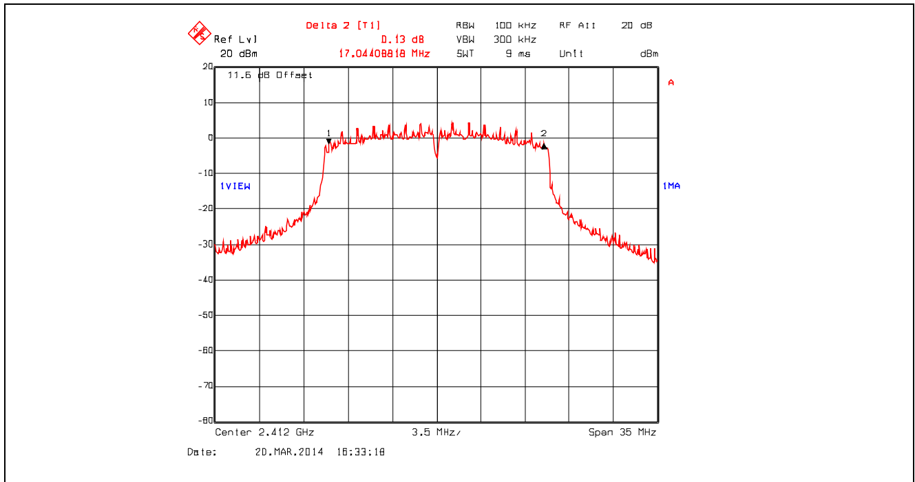
Plot 5.2.4.28. 6 dB Bandwidth, 802.11n 800ns, 39 Mbps 16-QAM 3/4, 2412 MHz
