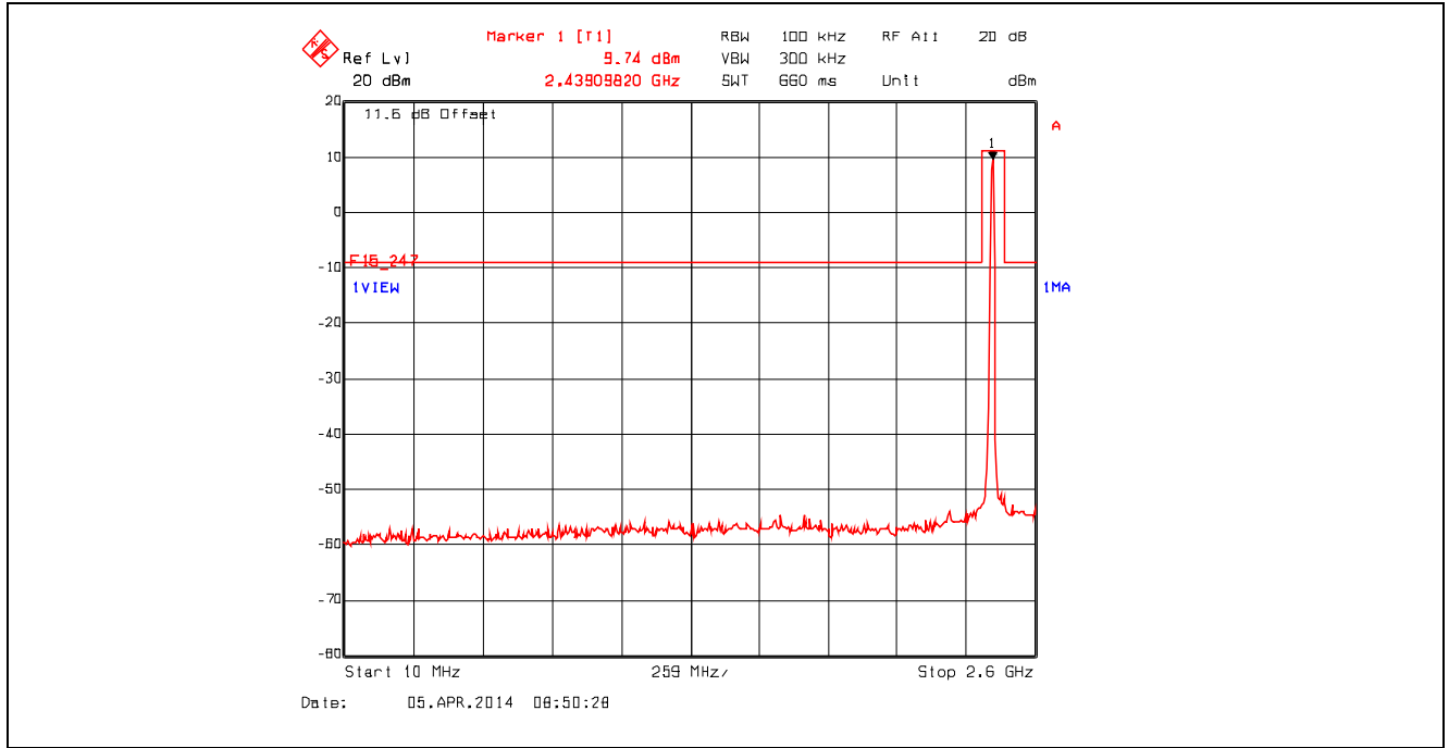
Plot 5.4.4.2.3. Conducted Spurious Emissions - Non Restricted Frequency Bands 802.11b, 2437 MHz, 1 Mbps, 10 MHz - 2.6 GHz
