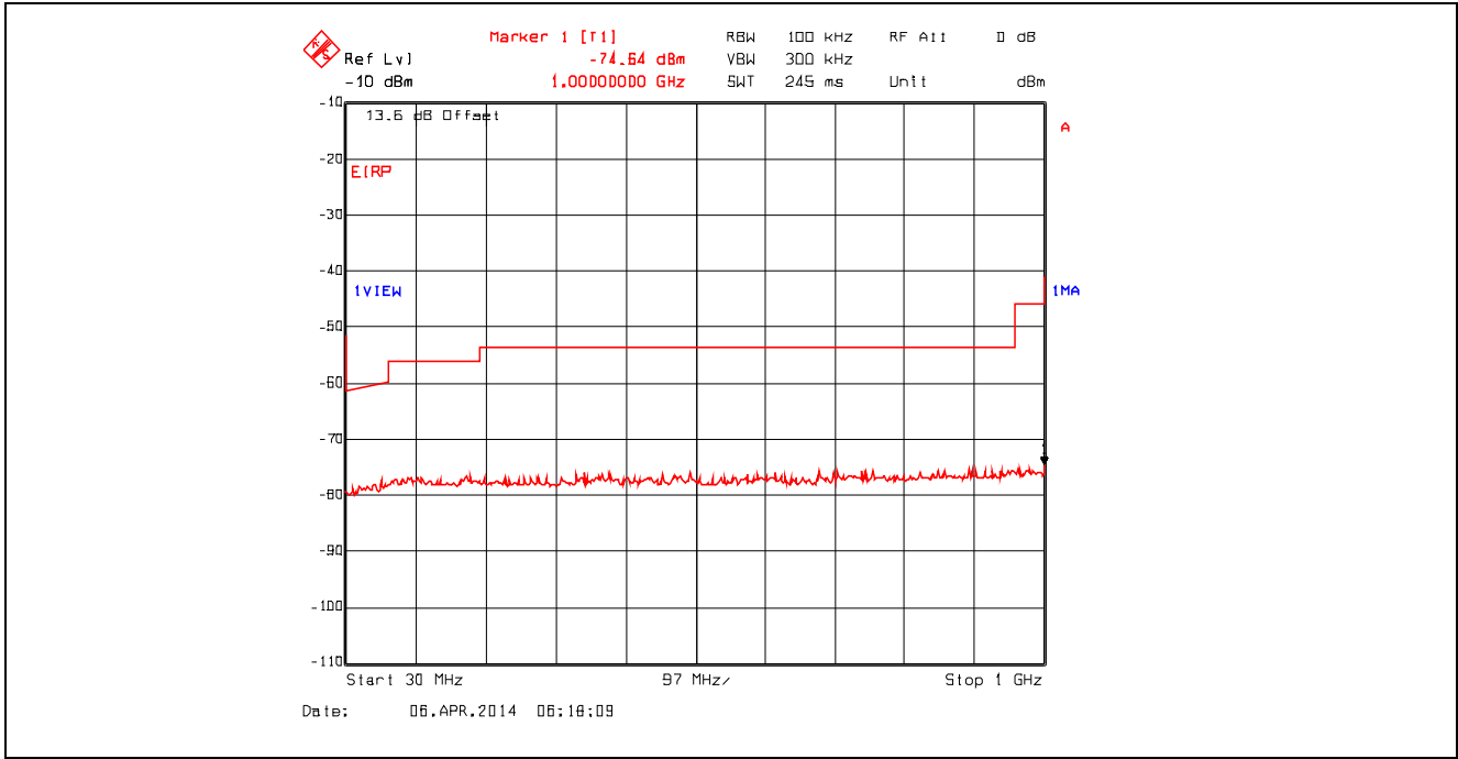
Plot 5.4.4.3.13. Conducted Spurious Emissions – Restricted Bands 802.11b, 1 Mbps, 2462 MHz, 30 MHz - 1 GHz, Peak Detector with Band (Notch) Reject Filter
