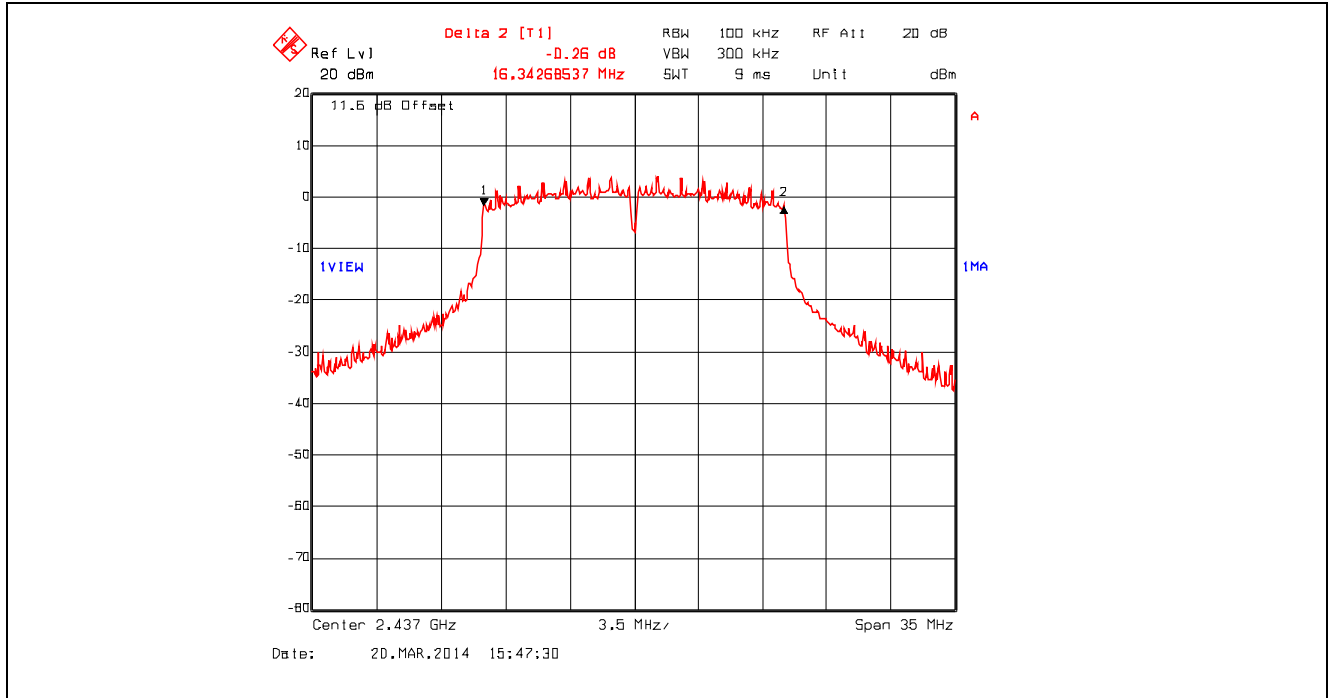
Plot 5.2.4.17. 6 dB Bandwidth, 802.11g, 36 Mbps 16-QAM, 2437 MHz
