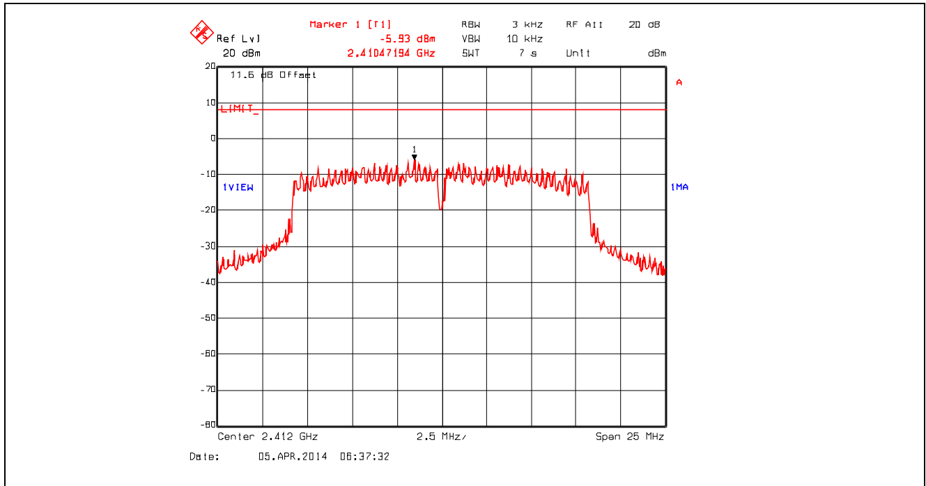
Plot 5.6.4.10. Power Spectral Density, 802.11g, 9 Mbps BPSK, 2412 MHz
