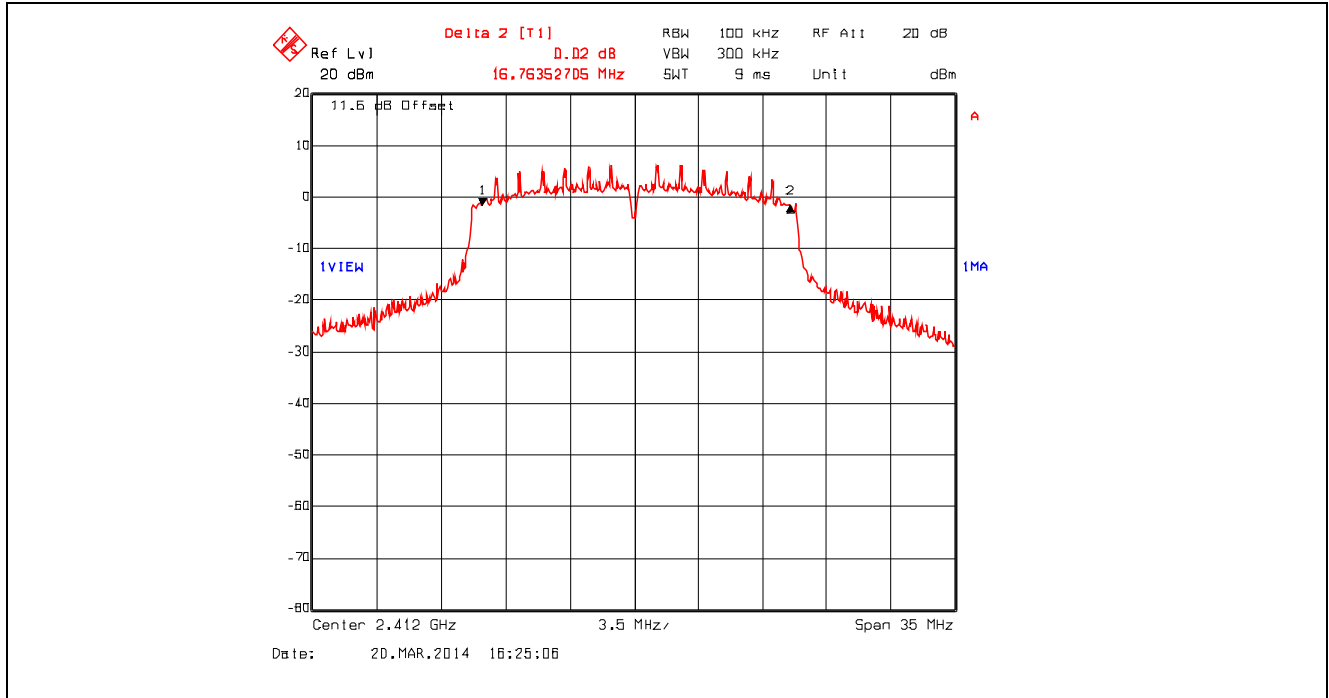
Plot 5.2.4.25. 6 dB Bandwidth, 802.11n 800ns, 19.5 Mbps QPSK 3/4, 2412 MHz
