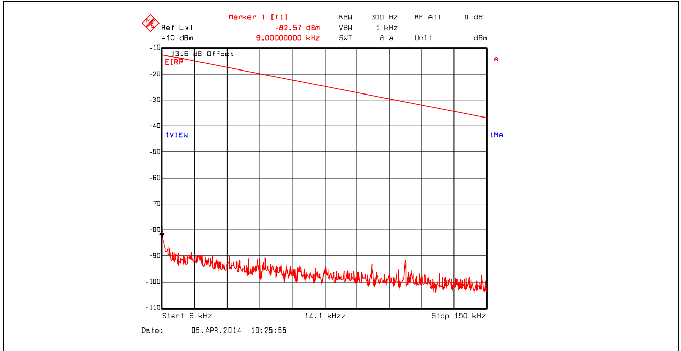
Plot 5.4.4.3.6. Conducted Spurious Emissions – Restricted Bands 802.11b, 1 Mbps, 2437 MHz, 9 kHz - 150 kHz, Peak Detector with Band (Notch) Reject Filter
