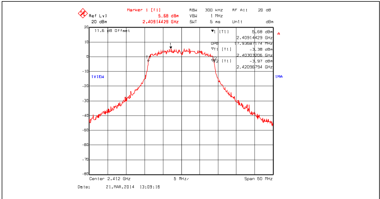
Plot 5.2.4.64. 99% Occupied Bandwidth, 802.11n 800ns, 65 Mbps 64-QAM 5/6, 2412 MHz
