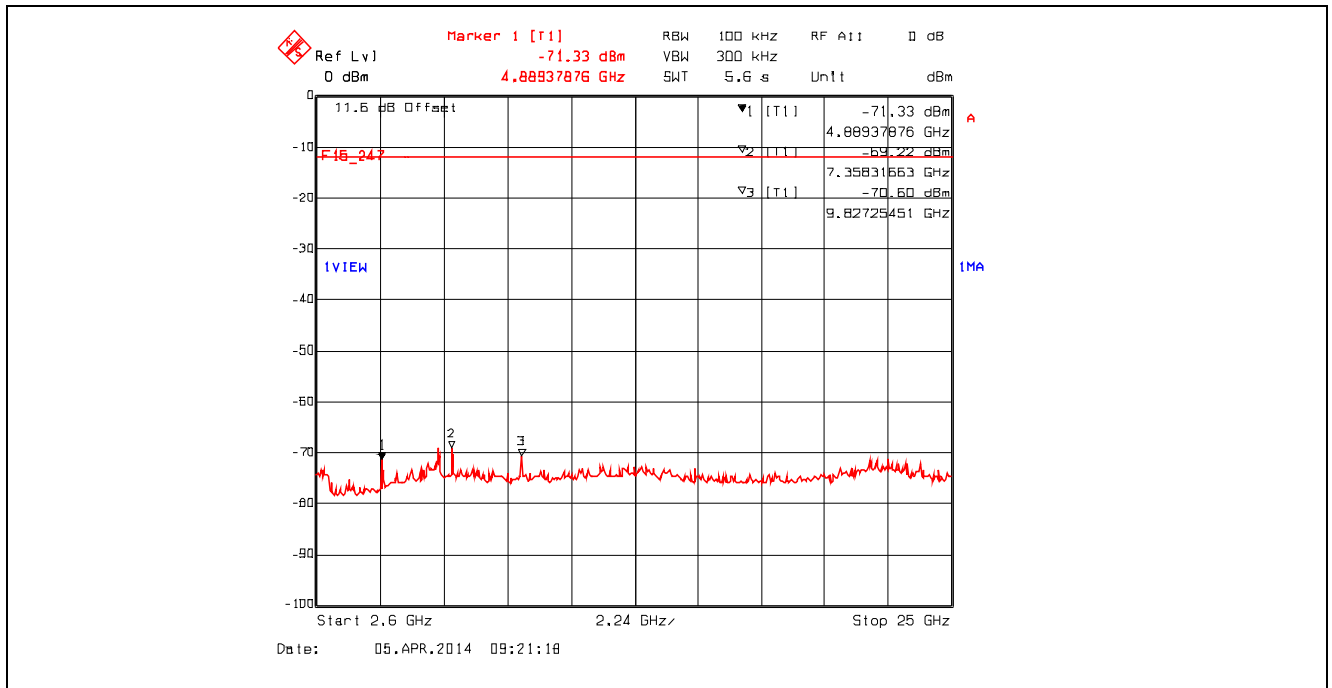
Plot 5.4.4.2.18. Conducted Spurious Emissions - Non Restricted Frequency Bands 802.11n, 2462 MHz, 6.5 Mbps, 2.6 GHz - 25 GHz
