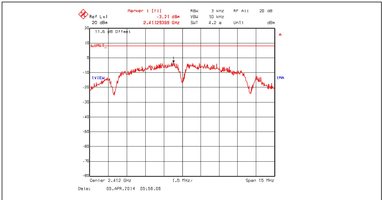
Plot 5.6.4.4. Power Spectral Density, 802.11b, 2 Mbps DQPSK, 2412 MHz
