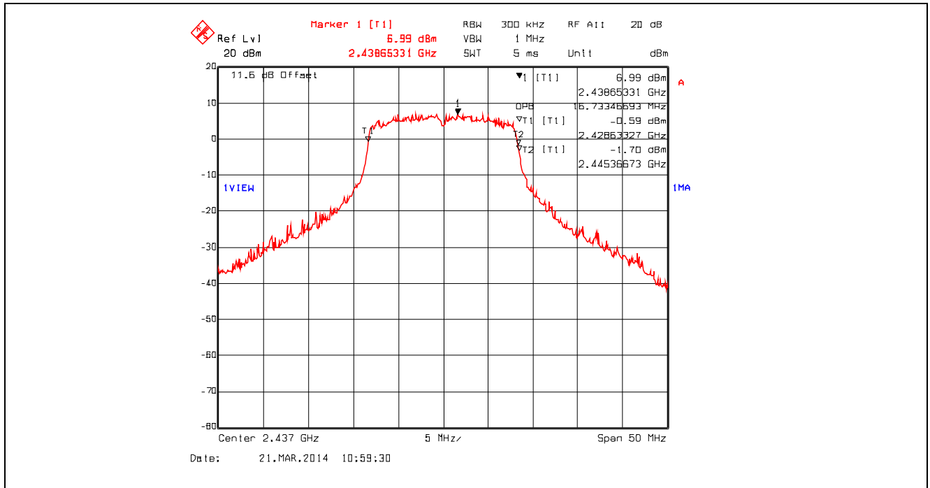
Plot 5.2.4.50. 99% Occupied Bandwidth, 802.11g, 36 Mbps 16-QAM, 2437 MHz
