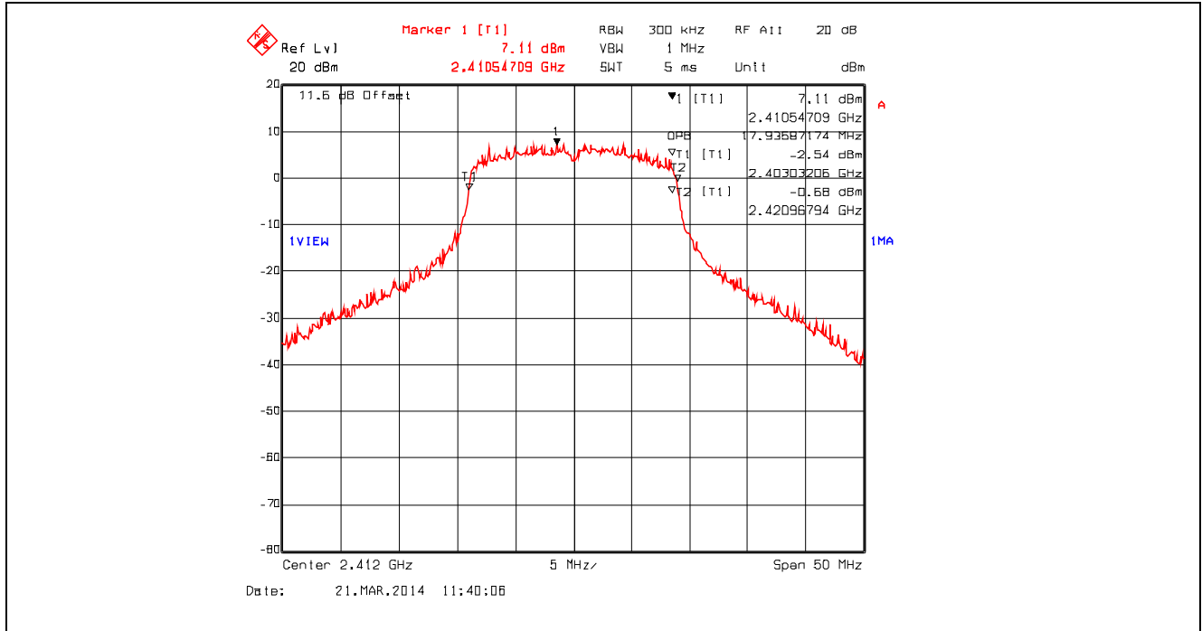
Plot 5.2.4.61. 99% Occupied Bandwidth, 802.11n 800ns, 39 Mbps 16-QAM 3/4, 2412 MHz
