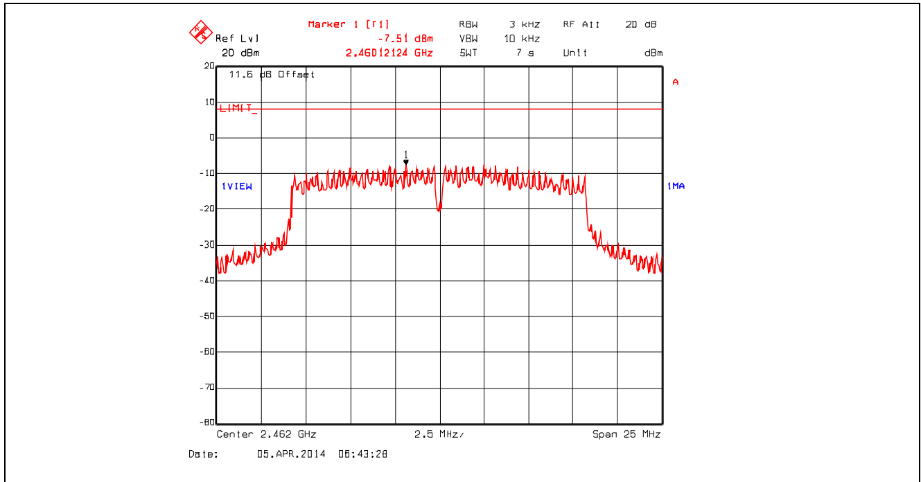
Plot 5.6.4.12. Power Spectral Density, 802.11g, 9 Mbps BPSK, 2462 MHz
