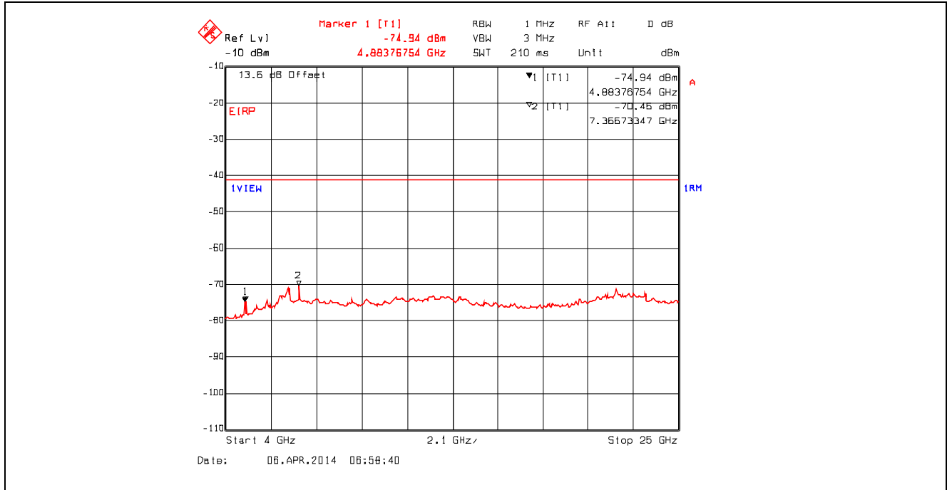
Plot 5.4.4.3.45. Conducted Spurious Emissions – Restricted Bands 802.11n, 6.5 Mbps, 2462 MHz, 4 GHz - 25 GHz, RMS Detector with High Pass Filter
