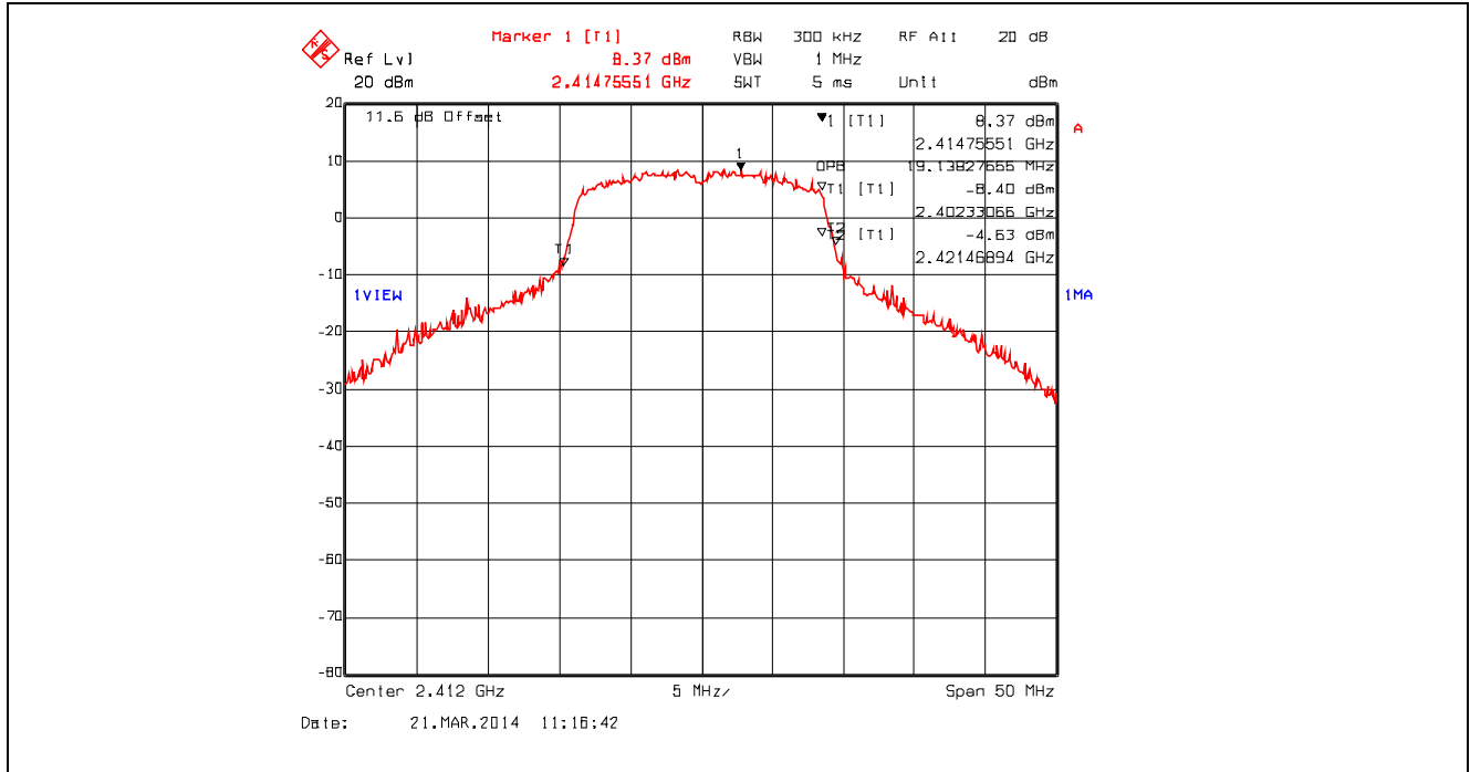
Plot 5.2.4.55. 99% Occupied Bandwidth, 802.11n 800ns, 6.5 Mbps BPSK1/2, 2412 MHz
