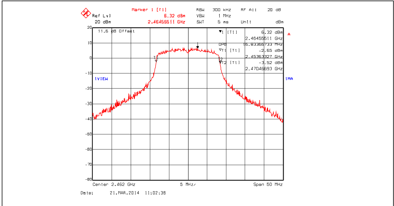
Plot 5.2.4.51. 99% Occupied Bandwidth, 802.11g, 36 Mbps 16-QAM, 2462 MHz
