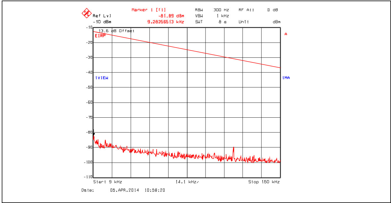
Plot 5.4.4.3.41. Conducted Spurious Emissions – Restricted Bands 802.11n, 6.5 Mbps, 2462 MHz, 9 kHz - 150 kHz, Peak Detector with Band (Notch) Reject Filter
