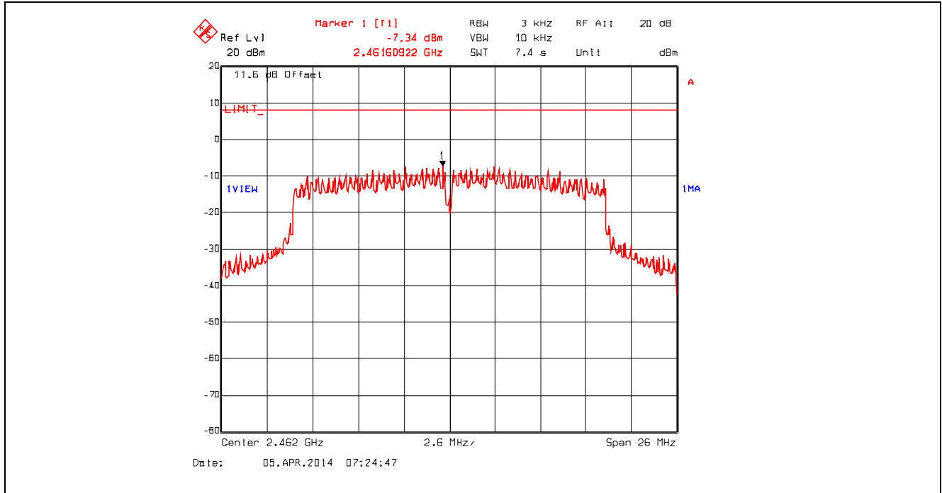
Plot 5.6.4.24. Power Spectral Density, 802.11n 800ns, 6.5 Mbps BPSK1/2, 2462 MHz
