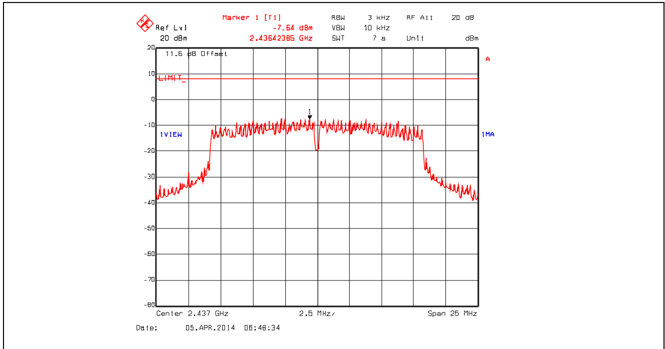
Plot 5.6.4.14. Power Spectral Density, 802.11g, 18 Mbps QPSK, 2437 MHz
