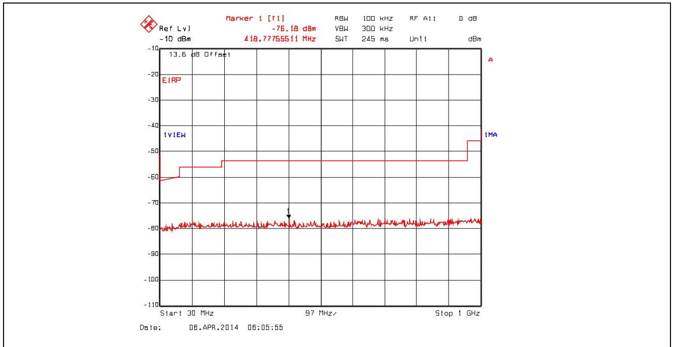
Plot 5.4.4.3.18. Conducted Spurious Emissions – Restricted Bands 802.11g, 9 Mbps, 2412 MHz, 30 MHz - 1 GHz, Peak Detector with Band (Notch) Reject Filter
