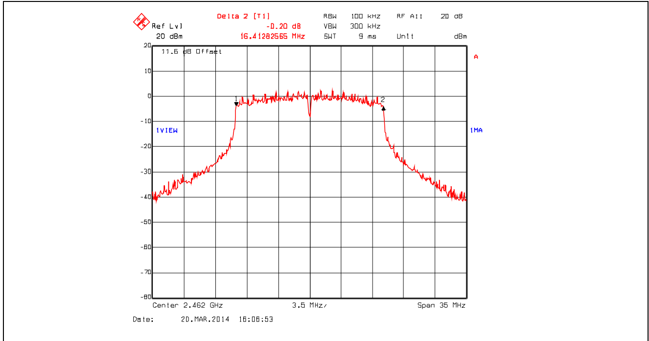
Plot 5.2.4.21. 6 dB Bandwidth, 802.11g, 54 Mbps 64-QAM, 2462 MHz
