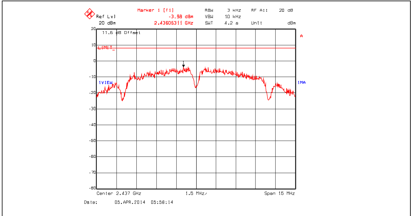
Plot 5.6.4.5. Power Spectral Density, 802.11b, 2 Mbps DQPSK, 2437 MHz
