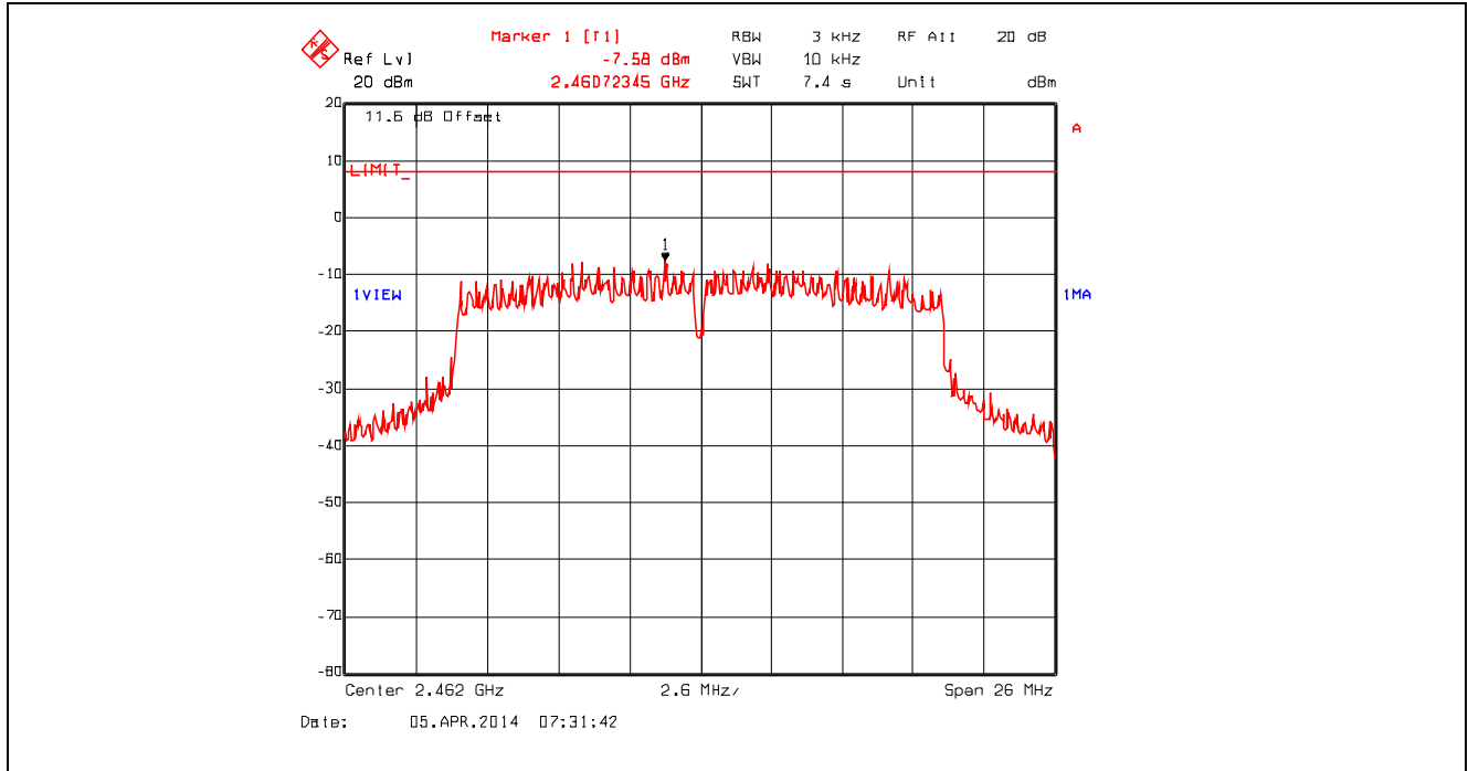
Plot 5.6.4.27. Power Spectral Density, 802.11n 800ns, 19.5 Mbps QPSK 3/4, 2462 MHz
