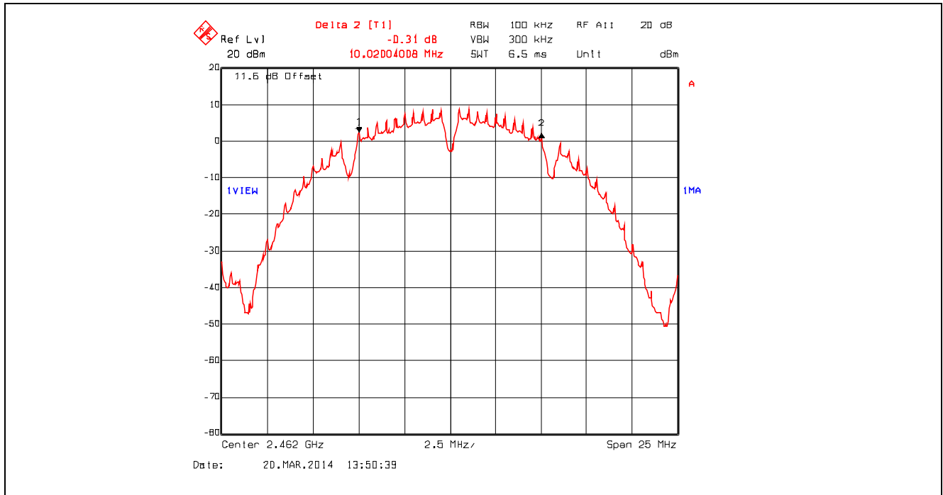
Plot 5.2.4.3. 6 dB Bandwidth, 802.11b, 1 Mbps DBPSK, 2462 MHz
