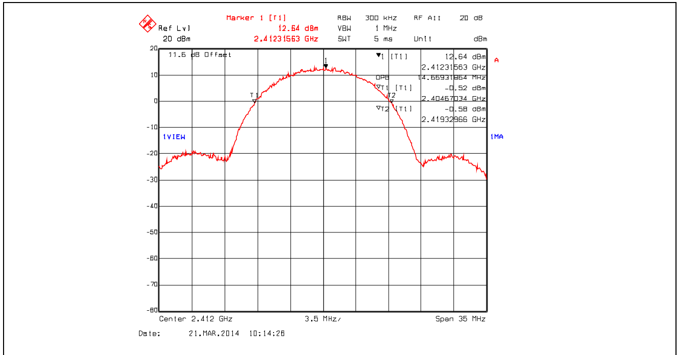
Plot 5.2.4.40. 99% Occupied Bandwidth, 802.11b, 11 Mbps CCK, 2412 MHz
