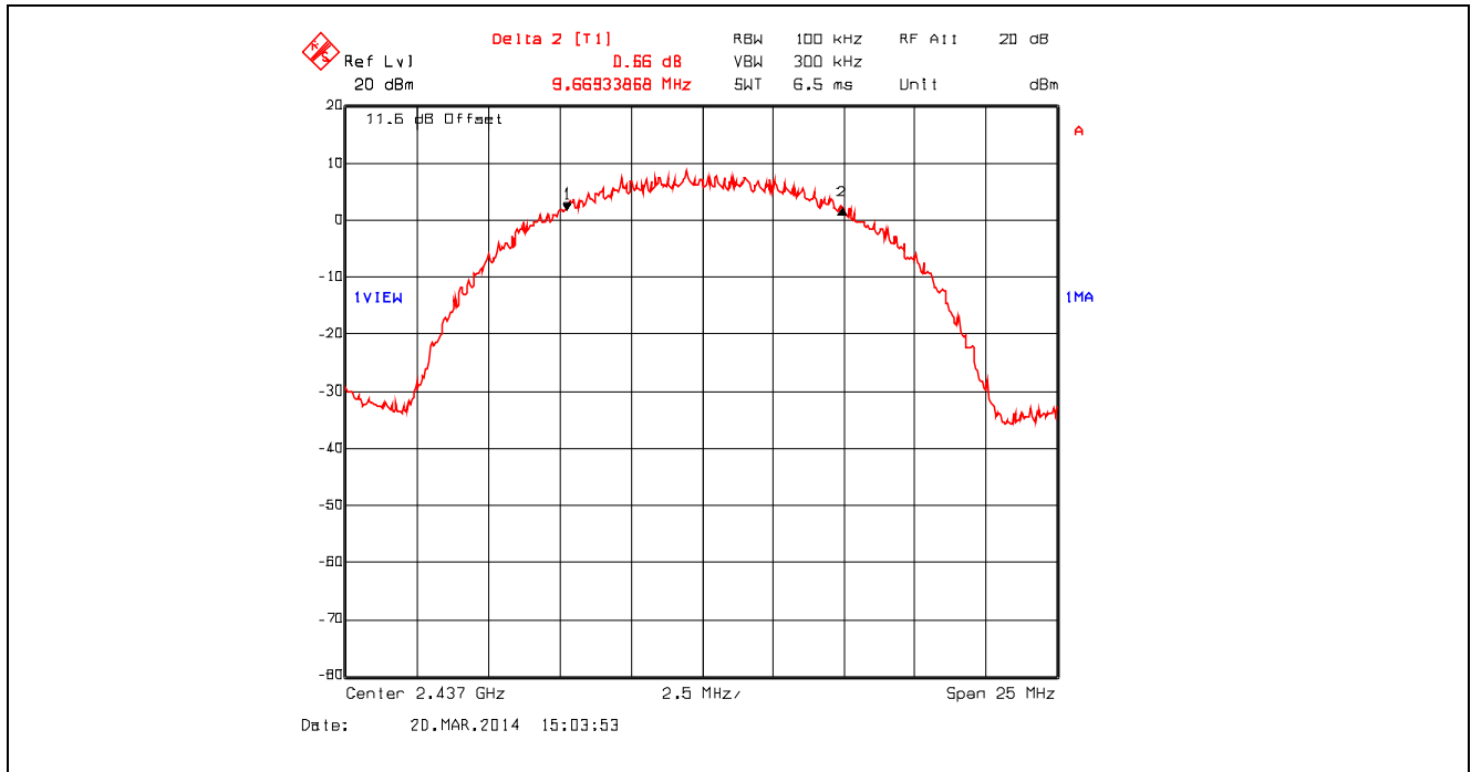
Plot 5.2.4.8. 6 dB Bandwidth, 802.11b, 11 Mbps CCK, 2437 MHz
