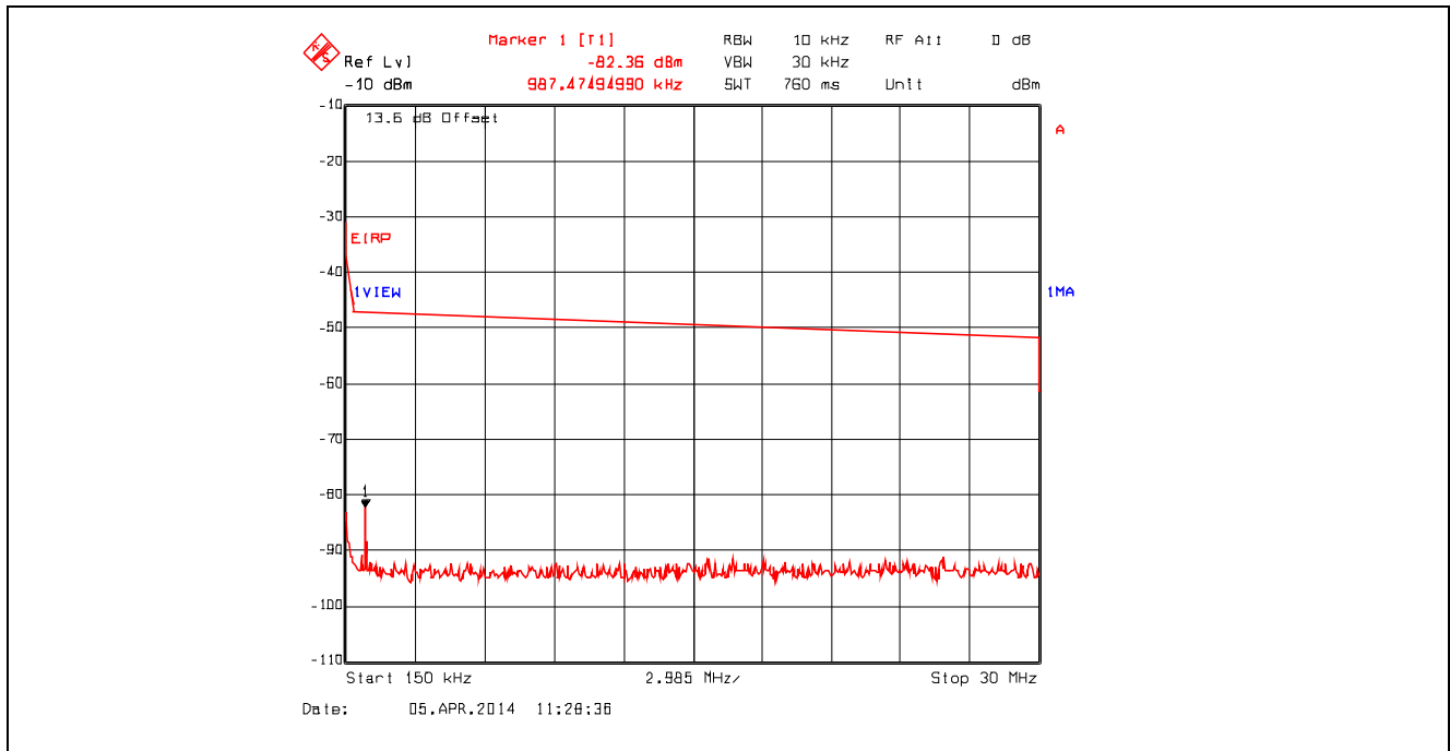
Plot 5.4.4.3.22. Conducted Spurious Emissions – Restricted Bands 802.11g, 9 Mbps, 2437 MHz, 150 kHz - 30 MHz, Peak Detector with Band (Notch) Reject Filter
