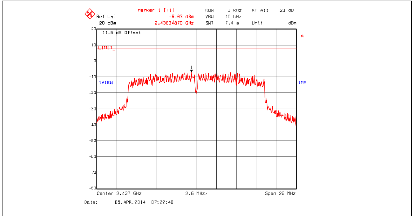
Plot 5.6.4.23. Power Spectral Density, 802.11n 800ns, 6.5 Mbps BPSK1/2, 2437 MHz
