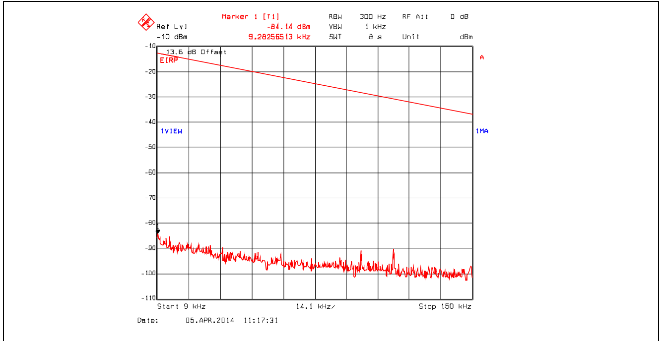
Plot 5.4.4.3.31. Conducted Spurious Emissions – Restricted Bands 802.11n, 6.5 Mbps, 2412 MHz, 9 kHz - 150 kHz, Peak Detector with Band (Notch) Reject Filter
