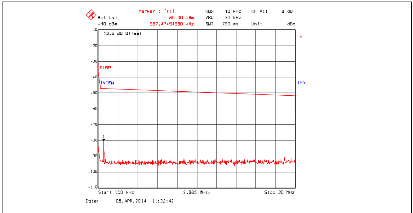
Plot 5.4.4.3.32. Conducted Spurious Emissions – Restricted Bands 802.11n, 6.5 Mbps, 2412 MHz, 150 kHz - 30 MHz, Peak Detector with Band (Notch) Reject Filter
