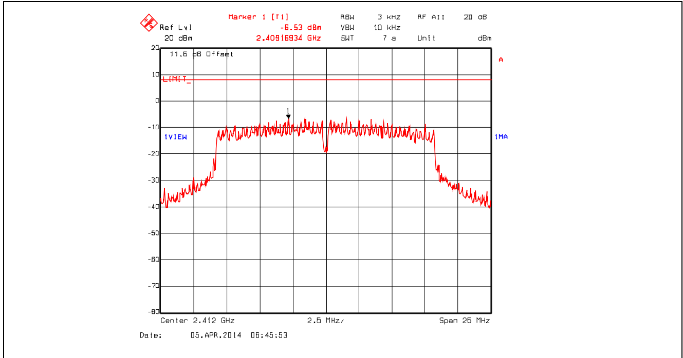
Plot 5.6.4.13. Power Spectral Density, 802.11g, 18 Mbps QPSK, 2412 MHz
