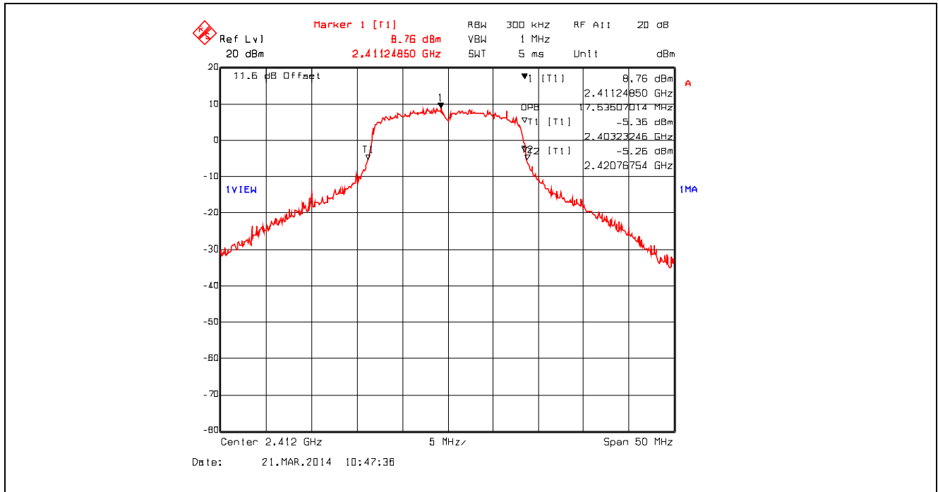
Plot 5.2.4.46. 99% Occupied Bandwidth, 802.11g, 18 Mbps QPSK, 2412 MHz
