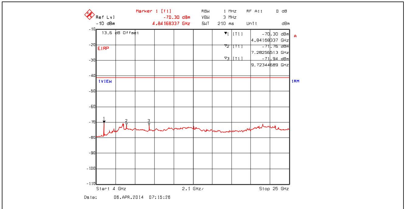
Plot 5.4.4.3.10. Conducted Spurious Emissions – Restricted Bands 802.11b, 1 Mbps, 2437 MHz, 4 GHz - 25 GHz, RMS Detector with High Pass Filter
