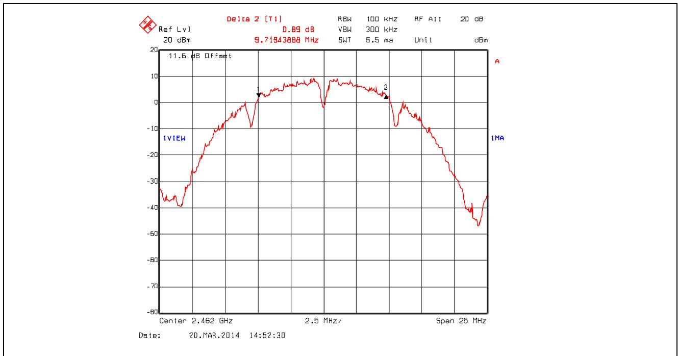
Plot 5.2.4.6. 6 dB Bandwidth, 802.11b, 2 Mbps DQPSK, 2462 MHz
