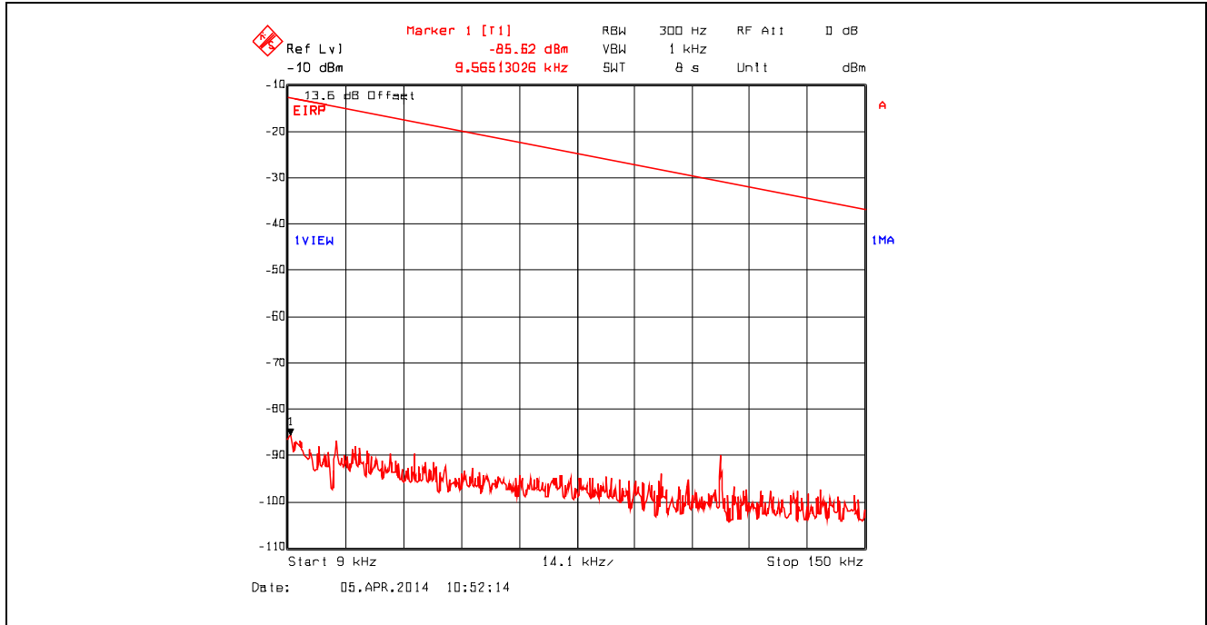
Plot 5.4.4.3.21. Conducted Spurious Emissions – Restricted Bands 802.11g, 9 Mbps, 2437 MHz, 9 kHz - 150 kHz, Peak Detector with Band (Notch) Reject Filter
