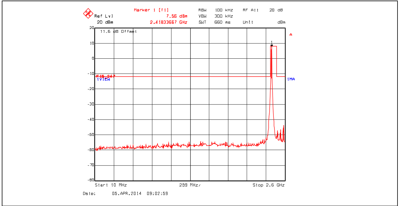
Plot 5.4.4.2.7. Conducted Spurious Emissions - Non Restricted Frequency Bands 802.11g, 2412 MHz, 9 Mbps, 10 MHz - 2.6 GHz
