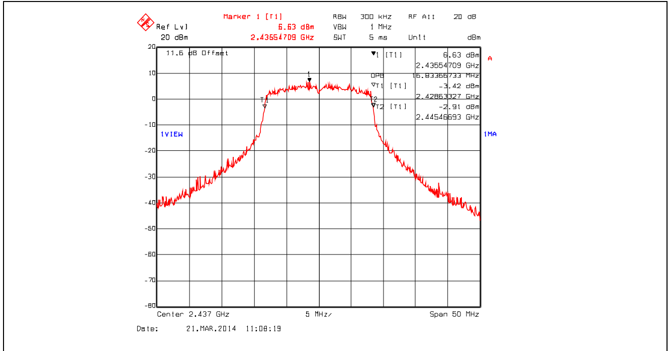
Plot 5.2.4.53. 99% Occupied Bandwidth, 802.11g, 54 Mbps 64-QAM, 2437 MHz
