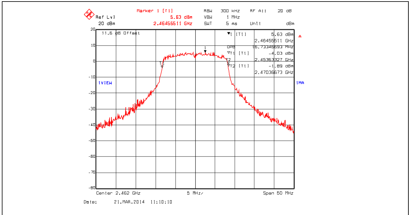
Plot 5.2.4.54. 99% Occupied Bandwidth, 802.11g, 54 Mbps 64-QAM, 2462 MHz
