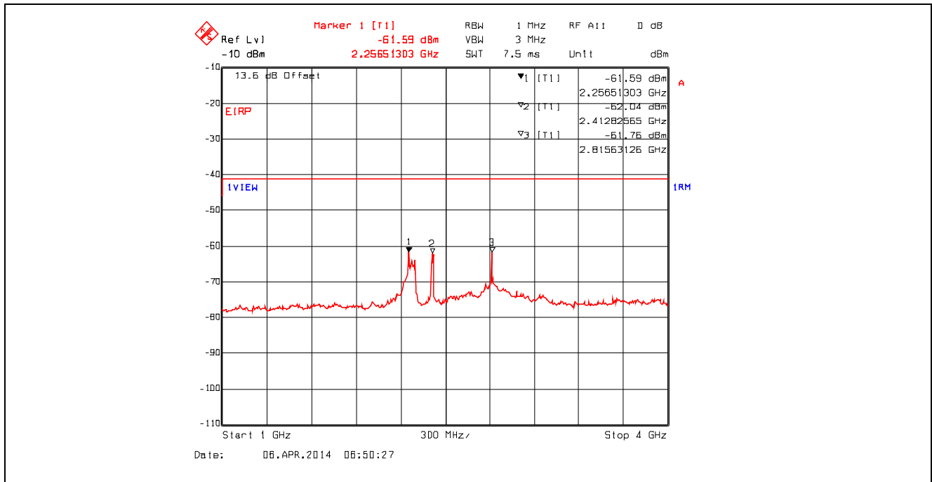
Plot 5.4.4.34. Conducted Spurious Emissions – Restricted Bands 802.11n, 6.5 Mbps, 2412 MHz, 1 GHz - 4 GHz, RMS Detector with Band (Notch) Reject Filter
