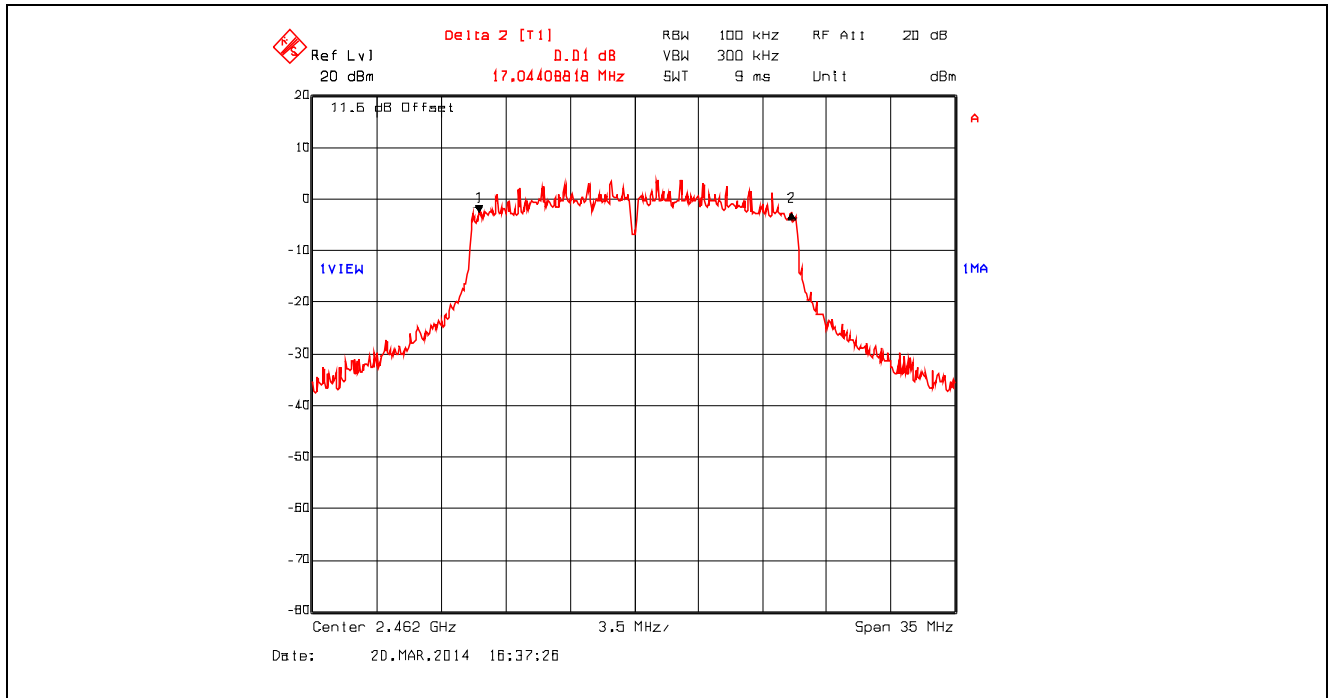
Plot 5.2.4.30. 6 dB Bandwidth, 802.11n 800ns, 39 Mbps 16-QAM 3/4, 2462 MHz
