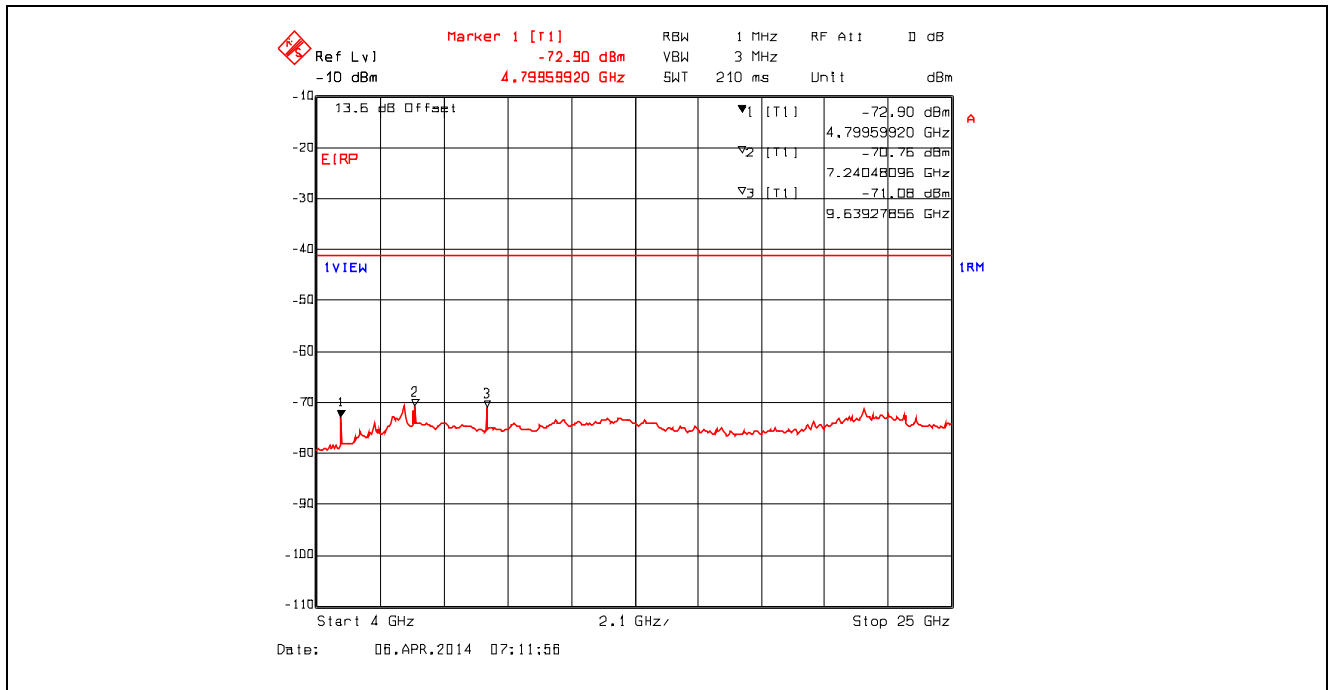
Plot 5.4.4.3.20. Conducted Spurious Emissions – Restricted Bands 802.11g, 9 Mbps, 2412 MHz, 4 GHz - 25 GHz, RMS Detector with High Pass Filter
