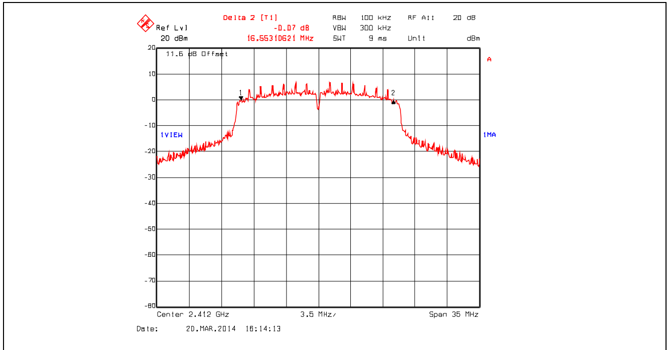
Plot 5.2.4.22. 6 dB Bandwidth, 802.11n 800ns, 6.5 Mbps BPSK1/2, 2412 MHz
