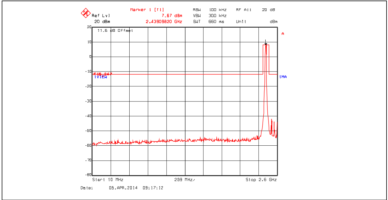
Plot 5.4.4.2.15. Conducted Spurious Emissions - Non Restricted Frequency Bands 802.11n, 2437 MHz, 6.5 Mbps, 10 MHz - 2.6 GHz
