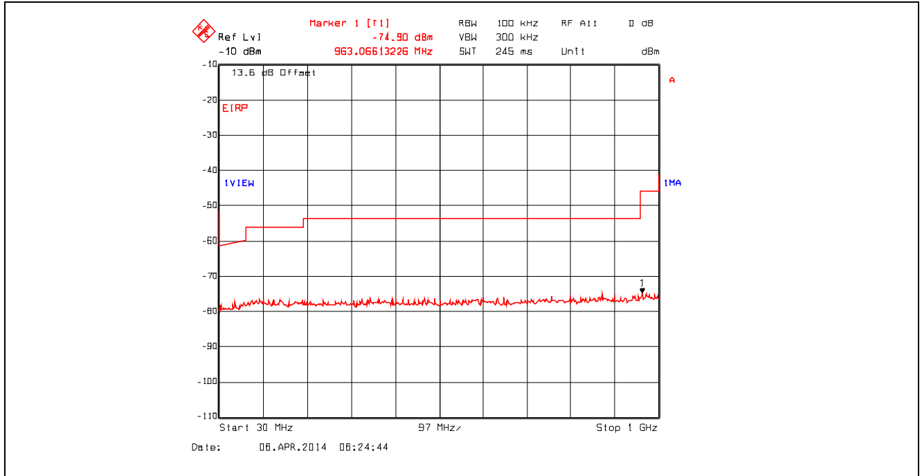
Plot 5.4.4.3.3. Conducted Spurious Emissions – Restricted Bands 802.11b, 1 Mbps, 2412 MHz, 30 MHz - 1 GHz, Peak Detector with Band (Notch) Reject Filter
