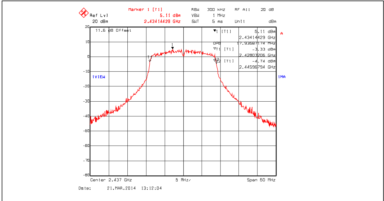
Plot 5.2.4.65. 99% Occupied Bandwidth, 802.11n 800ns, 65 Mbps 64-QAM 5/6, 2437 MHz
