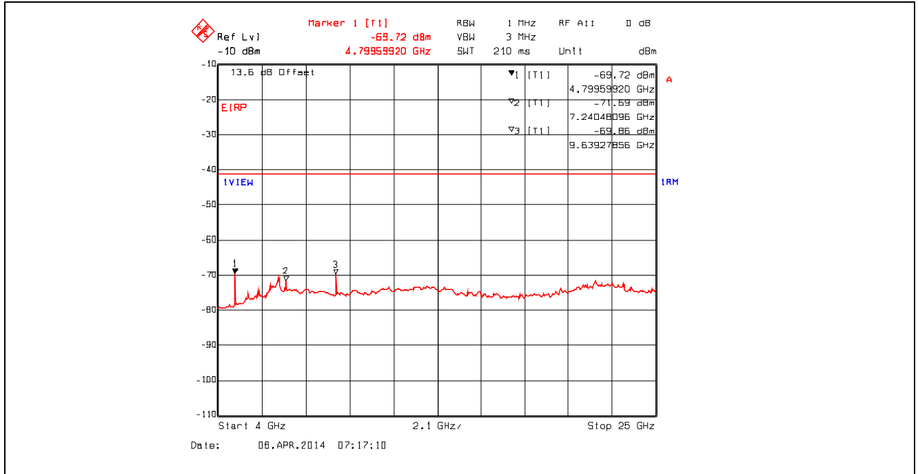
Plot 5.4.4.3.5. Conducted Spurious Emissions – Restricted Bands 802.11b, 1 Mbps, 2412 MHz, 4 GHz - 25 GHz, RMS Detector with High Pass Filter
