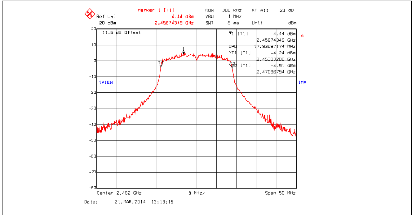
Plot 5.2.4.66. 99% Occupied Bandwidth, 802.11n 800ns, 65 Mbps 64-QAM 5/6, 2462 MHz
