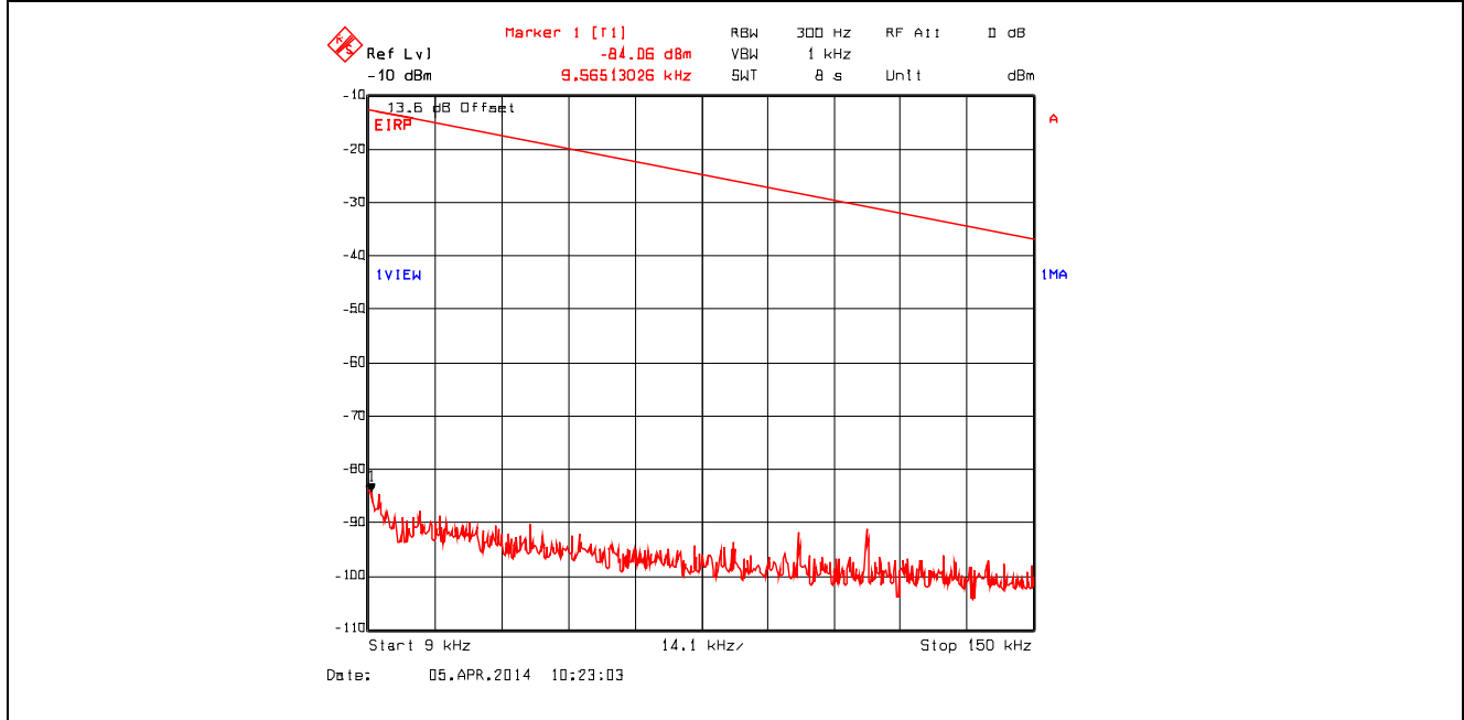
Plot 5.4.4.3.1. Conducted Spurious Emissions – Restricted Bands 802.11b, 1 Mbps, 2412 MHz, 9 kHz - 150 kHz, Peak Detector with Band (Notch) Reject Filter
