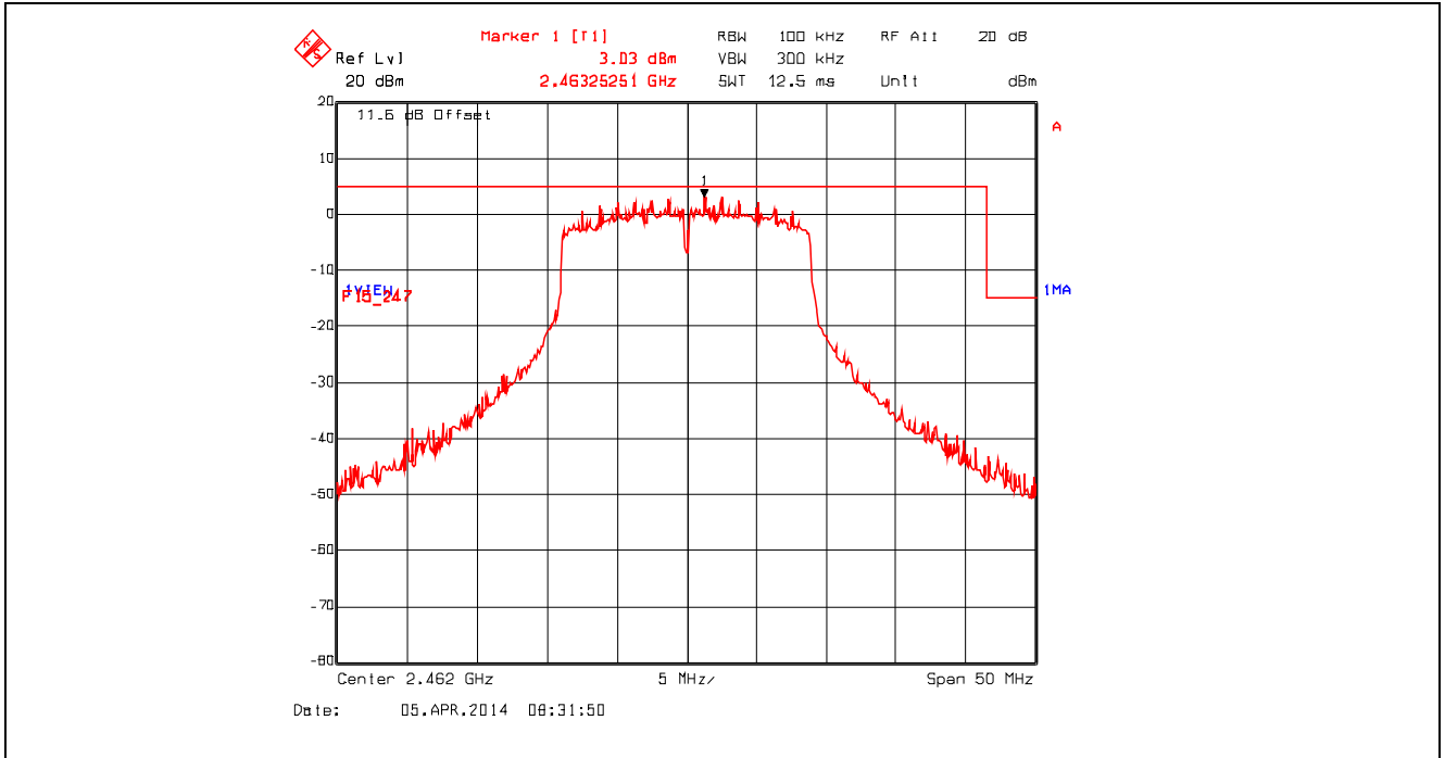
Plot 5.4.4.1.6. Band-Edge RF Conducted Emissions, Upper Band-edge, 2462 MHz, 802.11n 800ns, 65 Mbps
