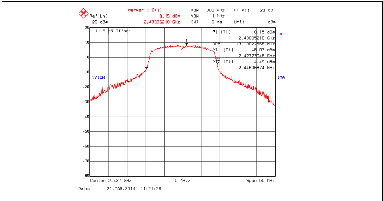
Plot 5.2.4.56. 99% Occupied Bandwidth, 802.11n 800ns, 6.5 Mbps BPSK1/2, 2437 MHz
