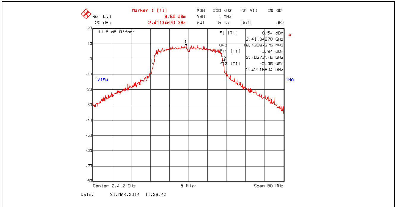
Plot 5.2.4.58. 99% Occupied Bandwidth, 802.11n 800ns, 19.5 Mbps QPSK 3/4, 2412 MHz
