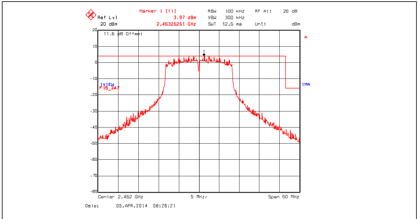
Plot 5.4.4.1.4. Band-Edge RF Conducted Emissions, Upper Band-edge, 2462 MHz, 802.11g, 54 Mbps
