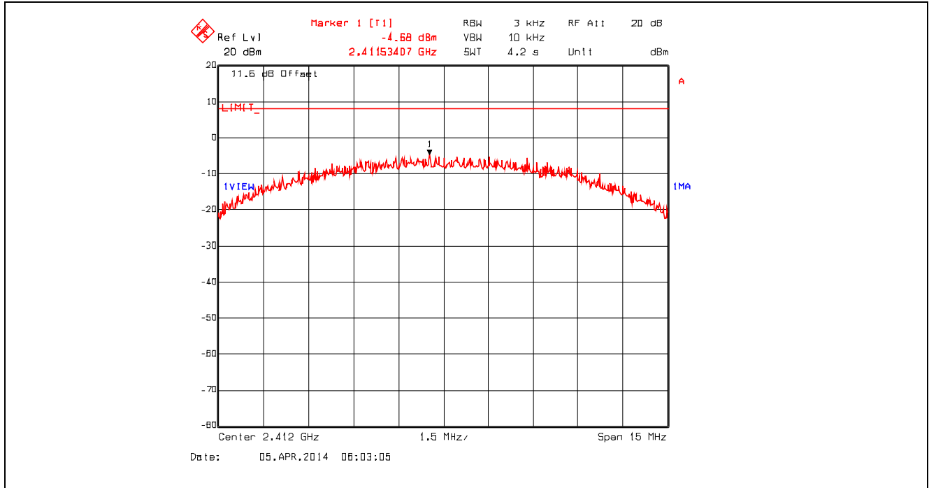
Plot 5.6.4.7. Power Spectral Density, 802.11b, 11 Mbps CCK, 2412 MHz
