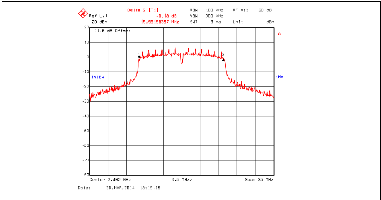
Plot 5.2.4.12. 6 dB Bandwidth, 802.11g, 9 Mbps BPSK, 2462 MHz
