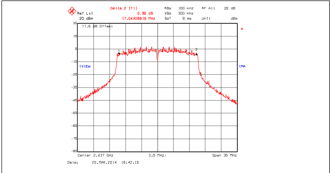
Plot 5.2.4.32. 6 dB Bandwidth, 802.11n 800ns, 65 Mbps 64-QAM 5/6, 2437 MHz
