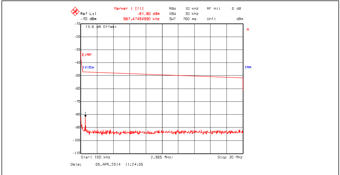
Plot 5.4.4.3.7. Conducted Spurious Emissions – Restricted Bands 802.11b, 1 Mbps, 2437 MHz, 150 kHz - 30 MHz, Peak Detector with Band (Notch) Reject Filter
