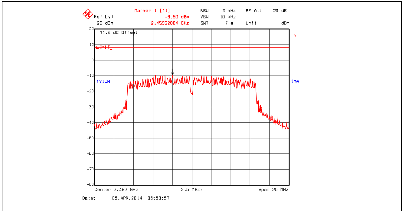
Plot 5.6.4.18. Power Spectral Density, 802.11g, 36 Mbps 16-QAM, 2462 MHz
