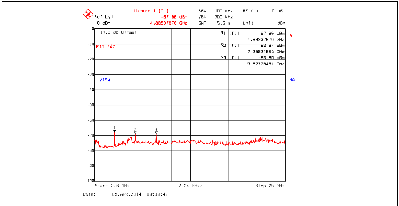
Plot 5.4.4.2.12. Conducted Spurious Emissions - Non Restricted Frequency Bands 802.11g, 2462 MHz, 9 Mbps, 2.6 GHz - 25 GHz
