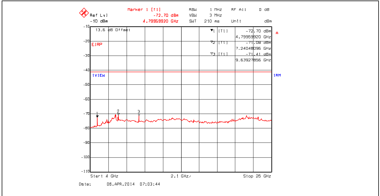
Plot 5.4.4.3.35. Conducted Spurious Emissions – Restricted Bands 802.11n, 6.5 Mbps, 2412 MHz, 4 GHz - 25 GHz, RMS Detector with High Pass Filter
