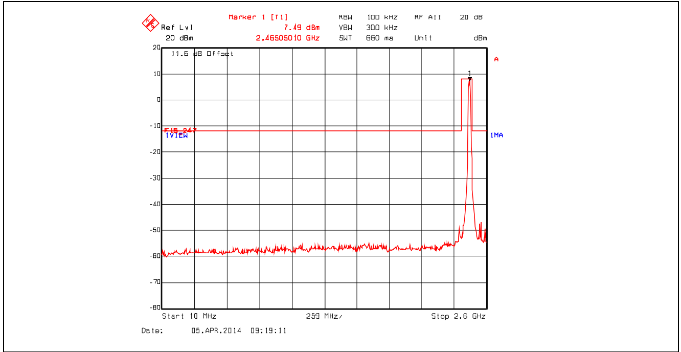
Plot 5.4.4.2.17. Conducted Spurious Emissions - Non Restricted Frequency Bands 802.11n, 2462 MHz, 6.5 Mbps, 10 MHz - 2.6 GHz
