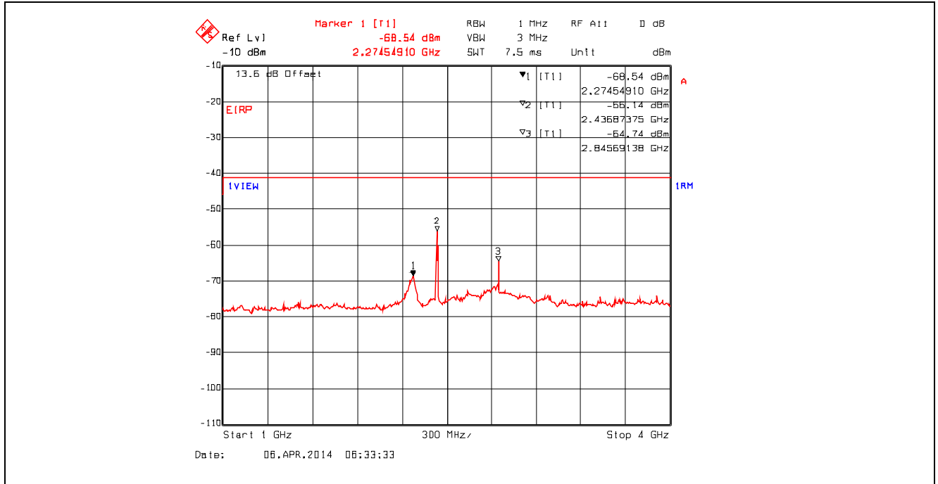
Plot 5.4.4.3.9. Conducted Spurious Emissions – Restricted Bands 802.11b, 1 Mbps, 2437 MHz, 1 GHz - 4 GHz, RMS Detector with Band (Notch) Reject Filter
