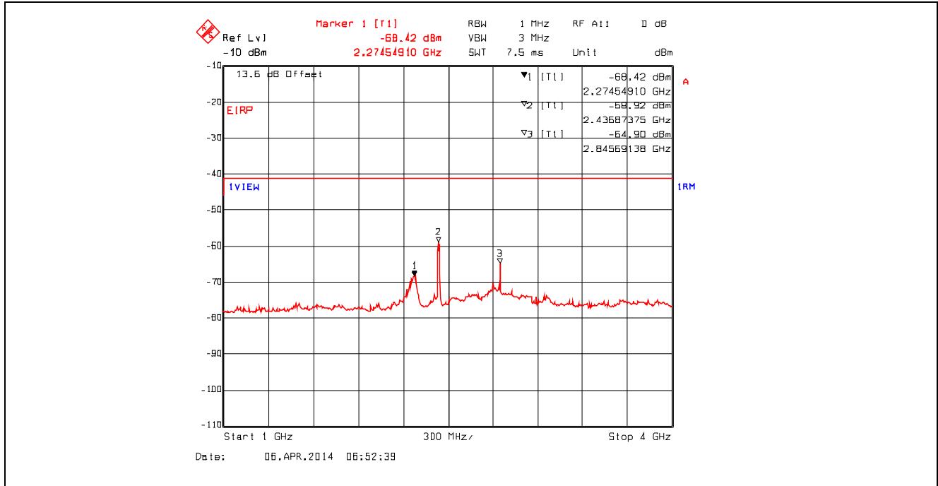
Plot 5.4.4.3.39. Conducted Spurious Emissions – Restricted Bands 802.11n, 6.5 Mbps, 2437 MHz, 1 GHz - 4 GHz, RMS Detector with Band (Notch) Reject Filter
