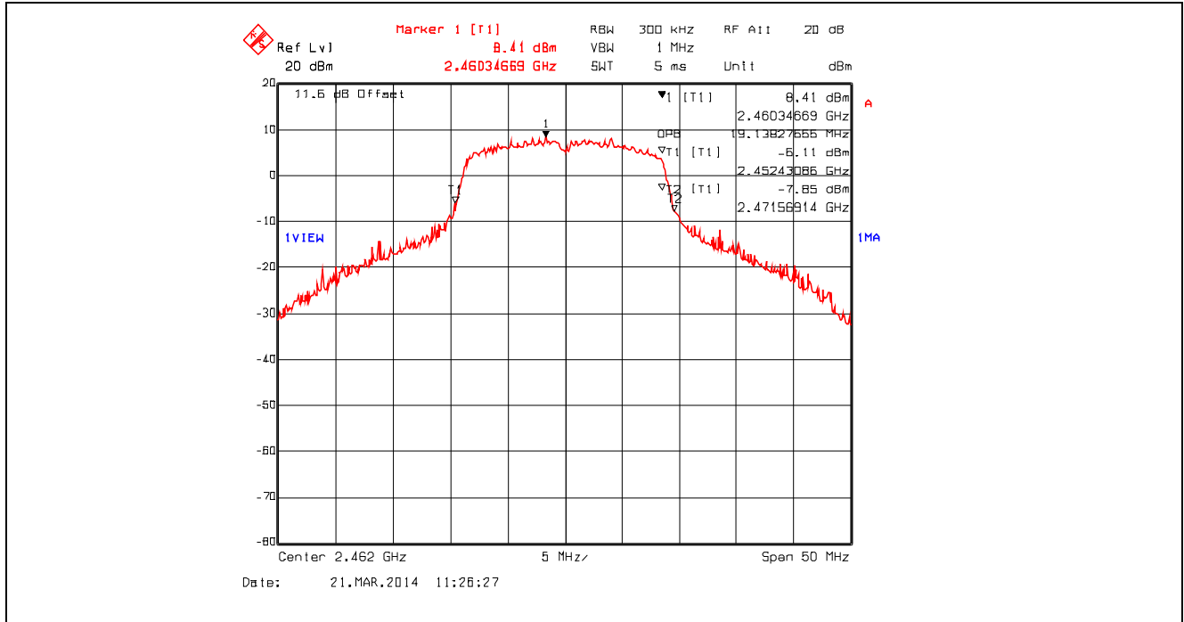
Plot 5.2.4.57. 99% Occupied Bandwidth, 802.11n 800ns, 6.5 Mbps BPSK1/2, 2462 MHz
