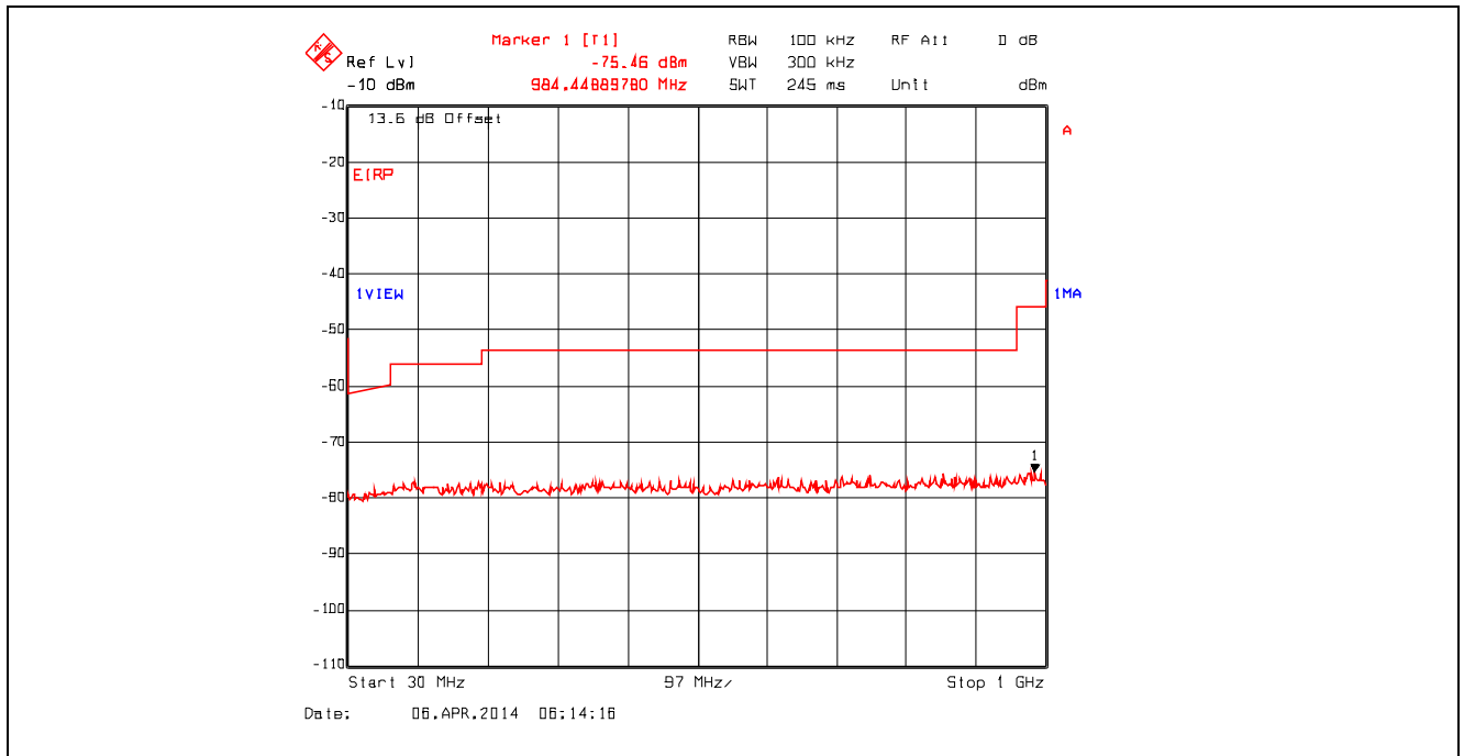
Plot 5.4.4.3.28. Conducted Spurious Emissions – Restricted Bands 802.11g, 9 Mbps, 2462 MHz, 30 MHz - 1 GHz, Peak Detector with Band (Notch) Reject Filter
