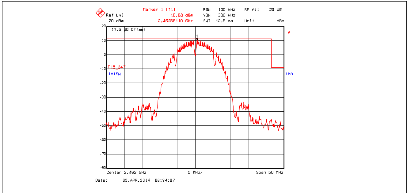
Plot 5.4.4.1.2. Band-Edge RF Conducted Emissions, Upper Band-edge, 2462 MHz, 802.11b, 1 Mbps
