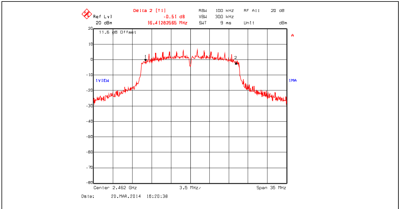
Plot 5.2.4.24. 6 dB Bandwidth, 802.11n 800ns, 6.5 Mbps BPSK1/2, 2462 MHz
