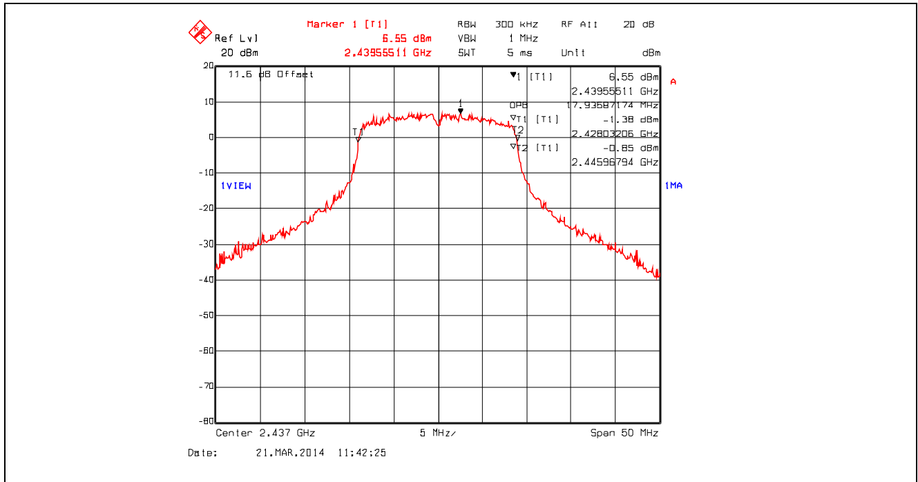
Plot 5.2.4.62. 99% Occupied Bandwidth, 802.11n 800ns, 39 Mbps 16-QAM 3/4, 2437 MHz
