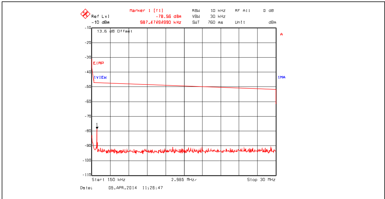
Plot 5.4.4.3.12. Conducted Spurious Emissions – Restricted Bands 802.11b, 1 Mbps, 2462 MHz, 150 kHz - 30 MHz, Peak Detector with Band (Notch) Reject Filter
