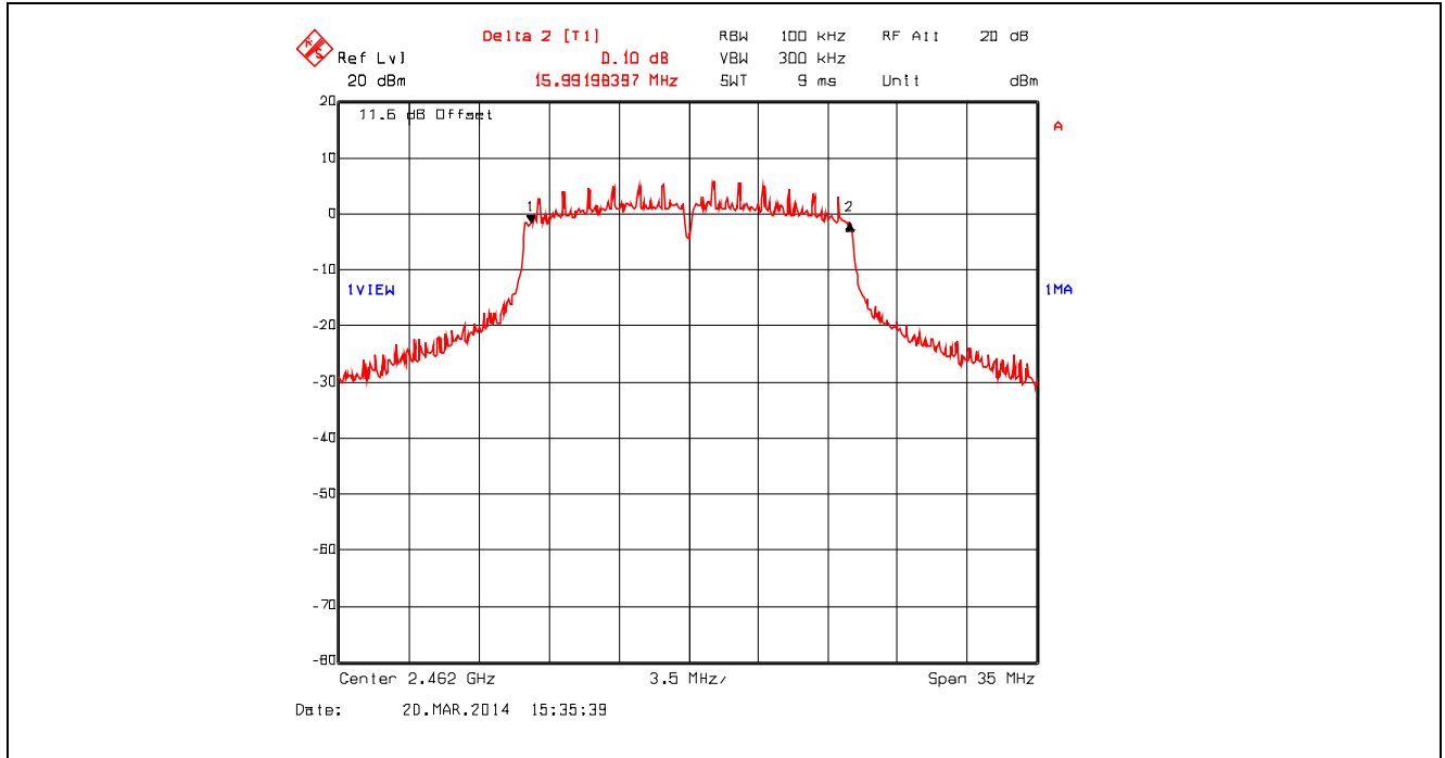
Plot 5.2.4.15. 6 dB Bandwidth, 802.11g, 18 Mbps QPSK, 2462 MHz
