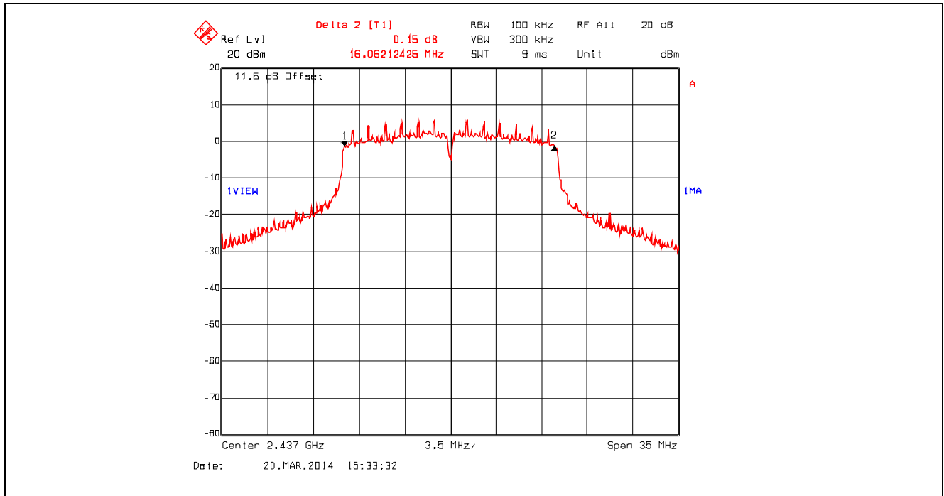
Plot 5.2.4.14. 6 dB Bandwidth, 802.11g, 18 Mbps QPSK, 2437 MHz
