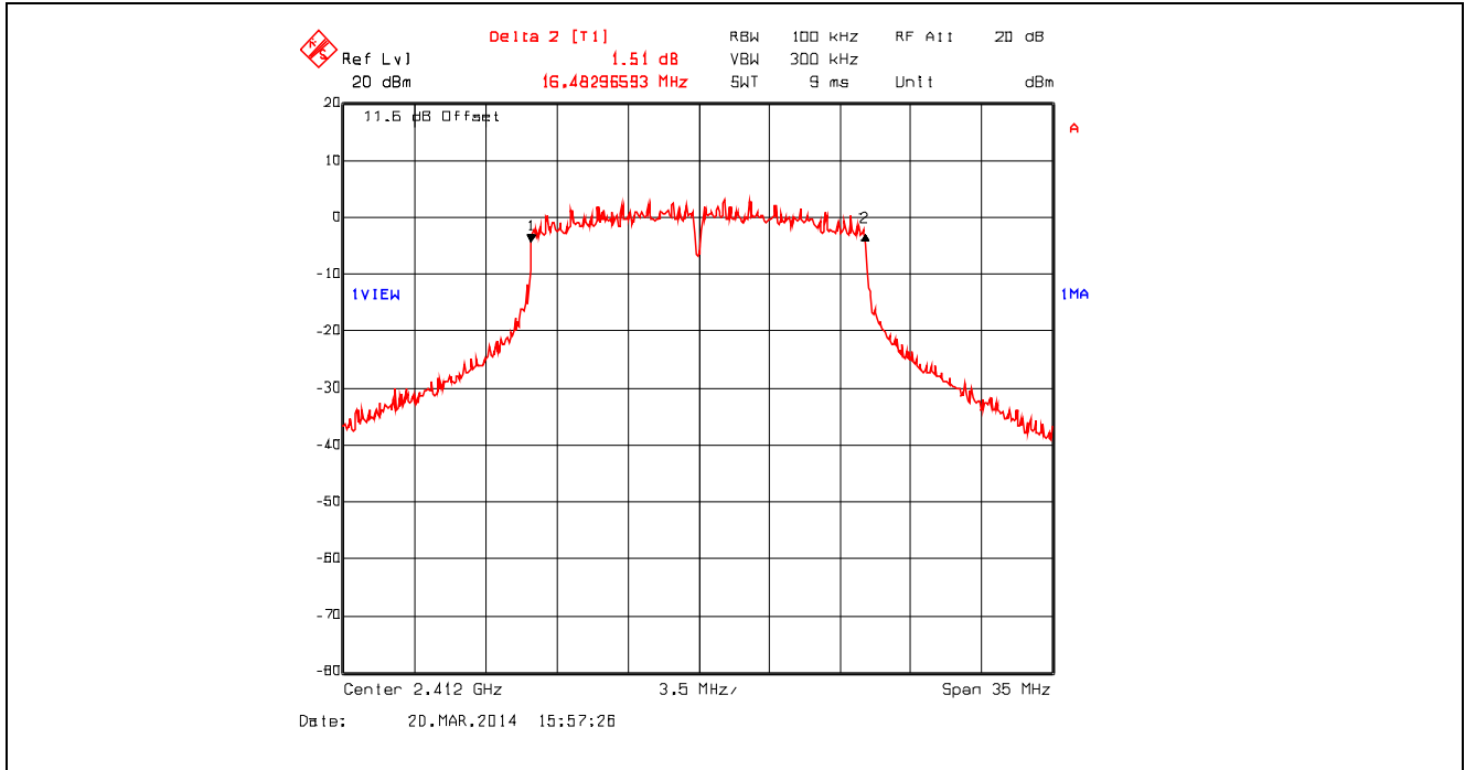
Plot 5.2.4.19. 6 dB Bandwidth, 802.11g, 54 Mbps 64-QAM, 2412 MHz
