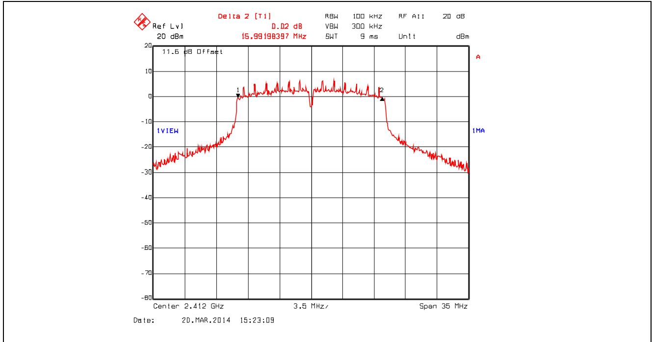
Plot 5.2.4.13. 6 dB Bandwidth, 802.11g, 18 Mbps QPSK, 2412 MHz
