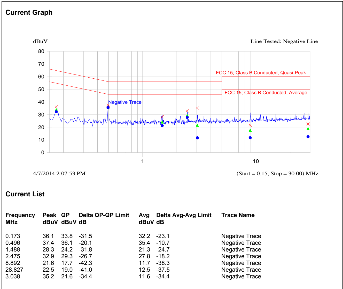
Plot 5.1.4.2. Power Line Conducted Emissions; Line Voltage: 12 V DC; Line Tested: Negative, Tx Mode
