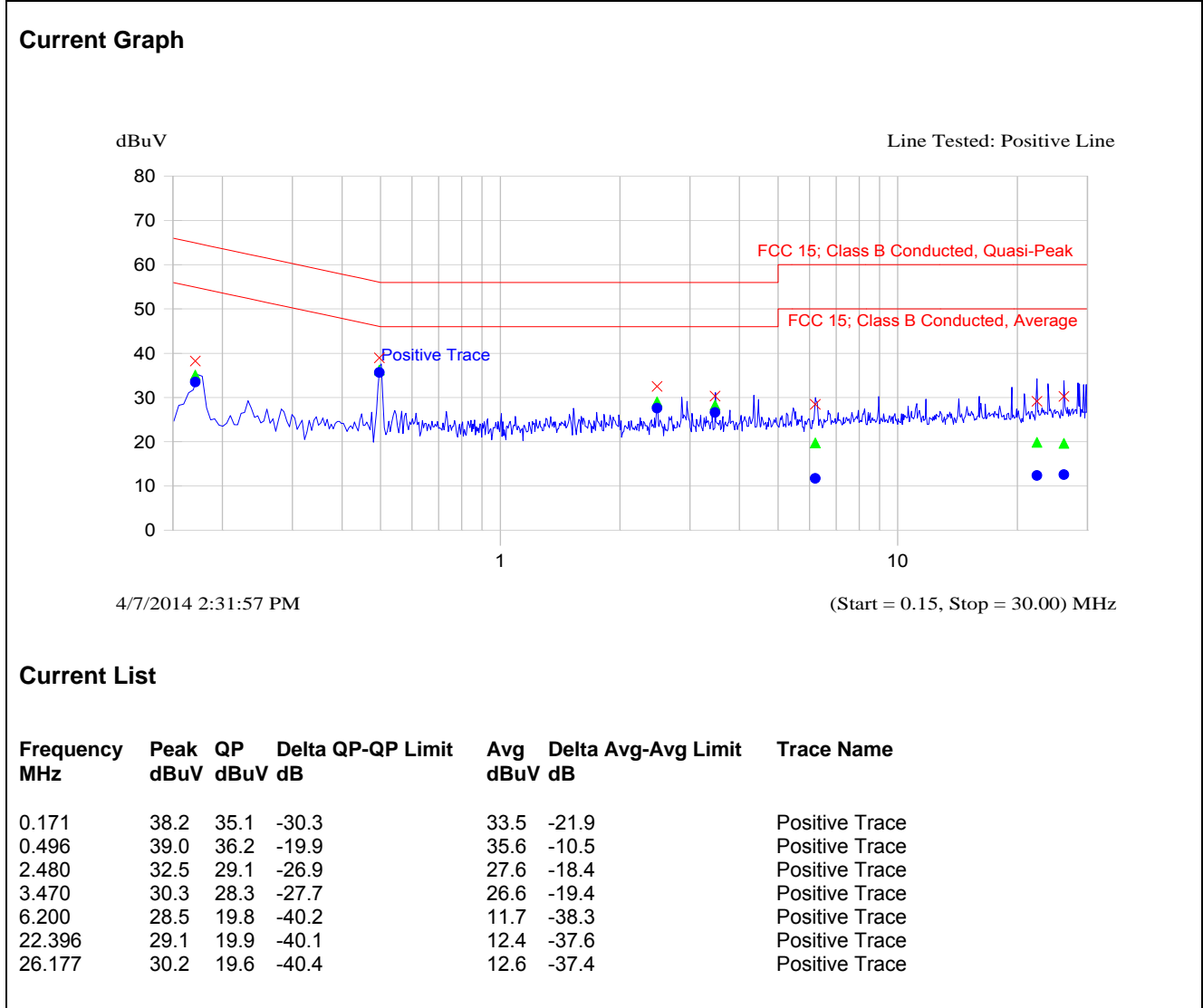
Plot 5.1.4.5. Power Line Conducted Emissions; Line Voltage: 12 V DC; Line Tested: Positive, Rx Mode
