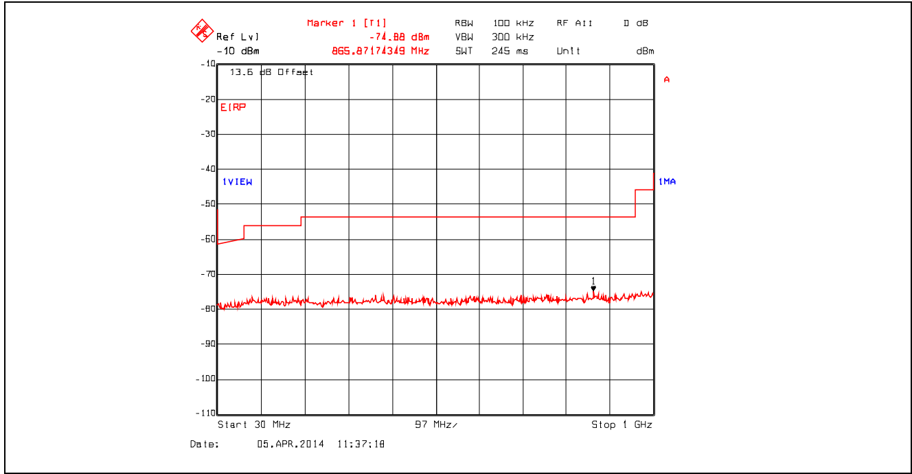
Plot 5.4.4.33. Conducted Spurious Emissions – Restricted Bands 802.11n, 6.5 Mbps, 2412 MHz, 30 MHz - 1 GHz, Peak Detector with Band (Notch) Reject Filter
