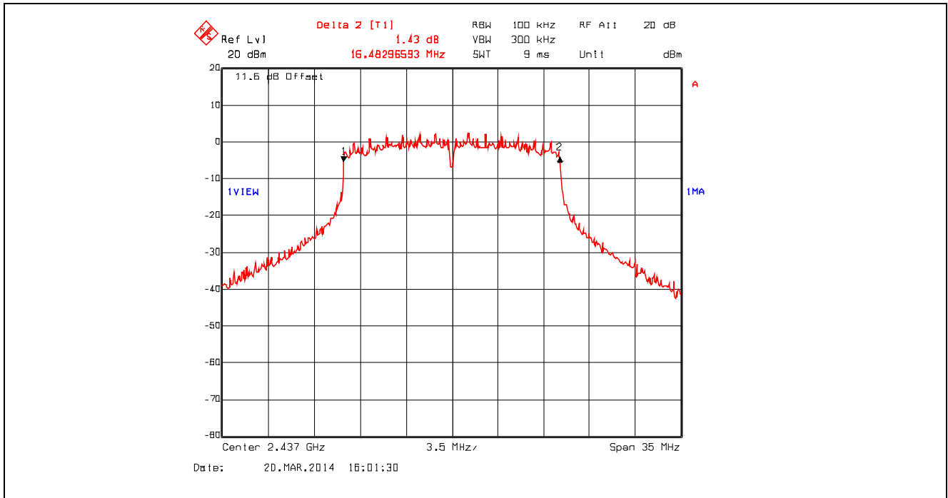
Plot 5.2.4.20. 6 dB Bandwidth, 802.11g, 54 Mbps 64-QAM, 2437 MHz
