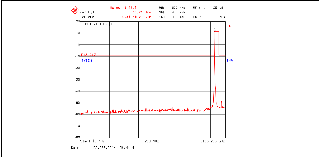
Plot 5.4.4.2.1. Conducted Spurious Emissions - Non Restricted Frequency Bands 802.11b, 2412 MHz, 1 Mbps, 10 MHz - 2.6 GHz
