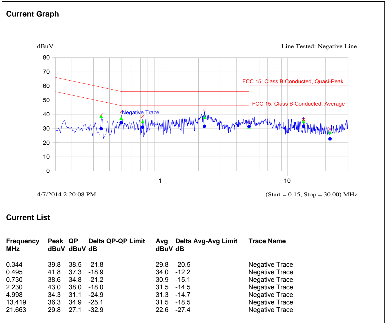
Plot 5.1.4.6. Power Line Conducted Emissions; Line Voltage: 12 V DC; Line Tested: Negative, Rx Mode
