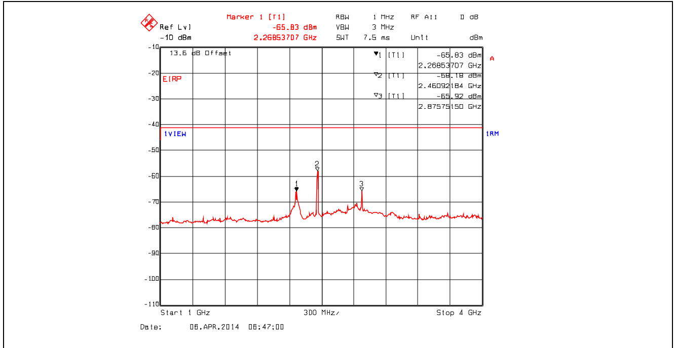
Plot 5.4.4.3.29. Conducted Spurious Emissions – Restricted Bands 802.11g, 9 Mbps, 2462 MHz, 1 GHz - 4 GHz, RMS Detector with Band (Notch) Reject Filter
