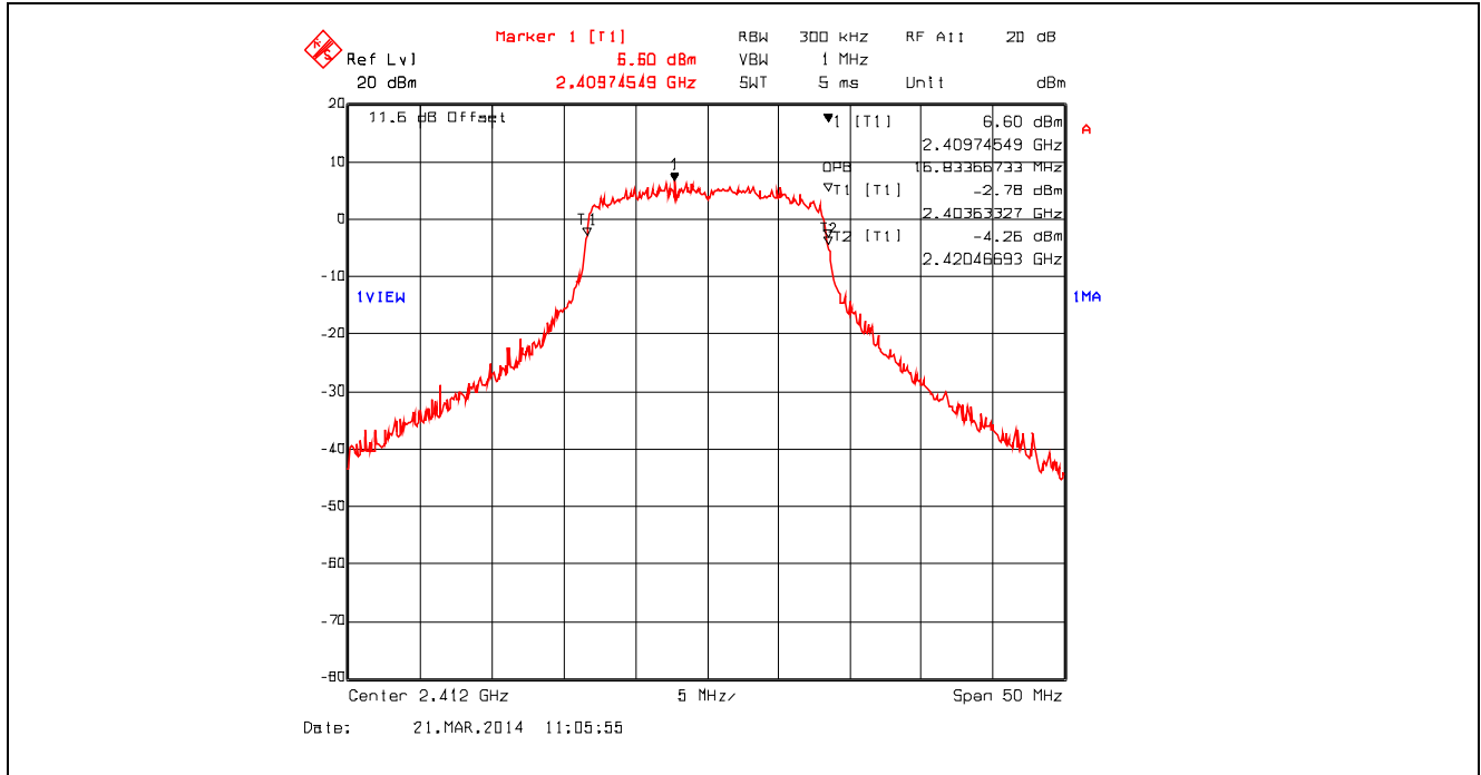
Plot 5.2.4.52. 99% Occupied Bandwidth, 802.11g, 54 Mbps 64-QAM, 2412 MHz
