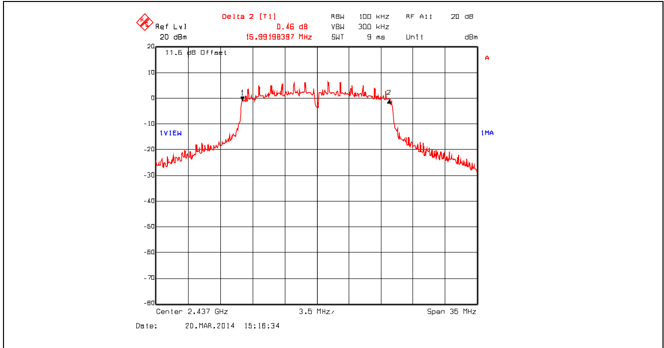
Plot 5.2.4.11. 6 dB Bandwidth, 802.11g, 9 Mbps BPSK, 2437 MHz
