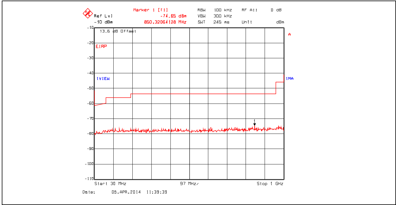
Plot 5.4.4.3.3. Conducted Spurious Emissions – Restricted Bands 802.11n, 6.5 Mbps, 2462 MHz, 30 MHz - 1 GHz, Peak Detector with Band (Notch) Reject Filter
