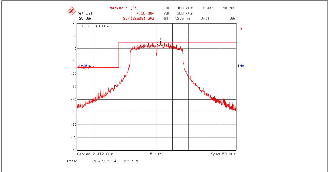
Plot 5.4.4.1.3. Band-Edge RF Conducted Emissions, Lower Band-edge, 2412 MHz, 802.11g, 54 Mbps
