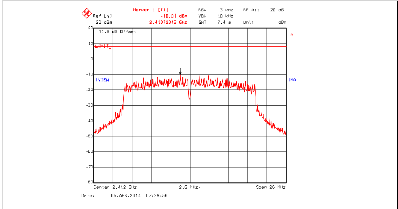
Plot 5.6.4.31. Power Spectral Density, 802.11n 800ns, 65 Mbps 64-QAM 5/6, 2412 MHz
