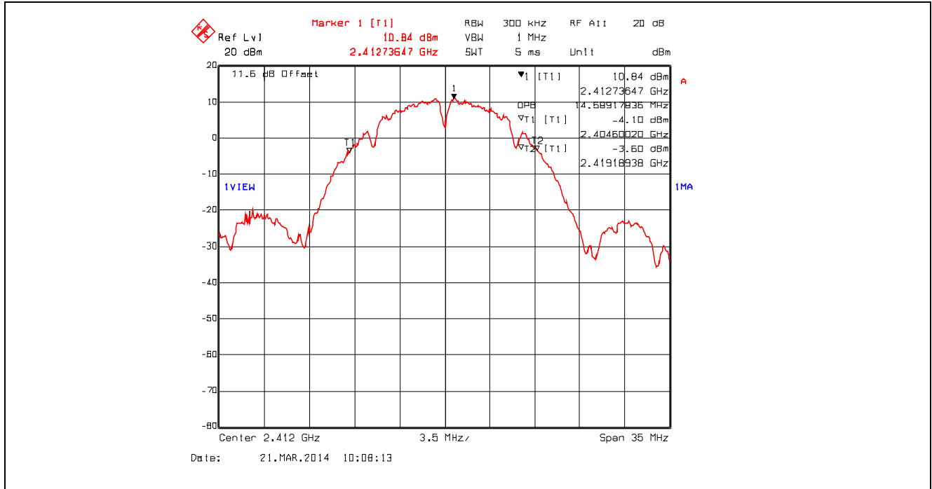
Plot 5.2.4.37. 99% Occupied Bandwidth, 802.11b, 2 Mbps DQPSK, 2412 MHz
