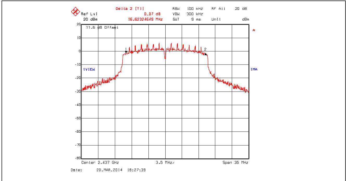
Plot 5.2.4.26. 6 dB Bandwidth, 802.11n 800ns, 19.5 Mbps QPSK 3/4, 2437 MHz
