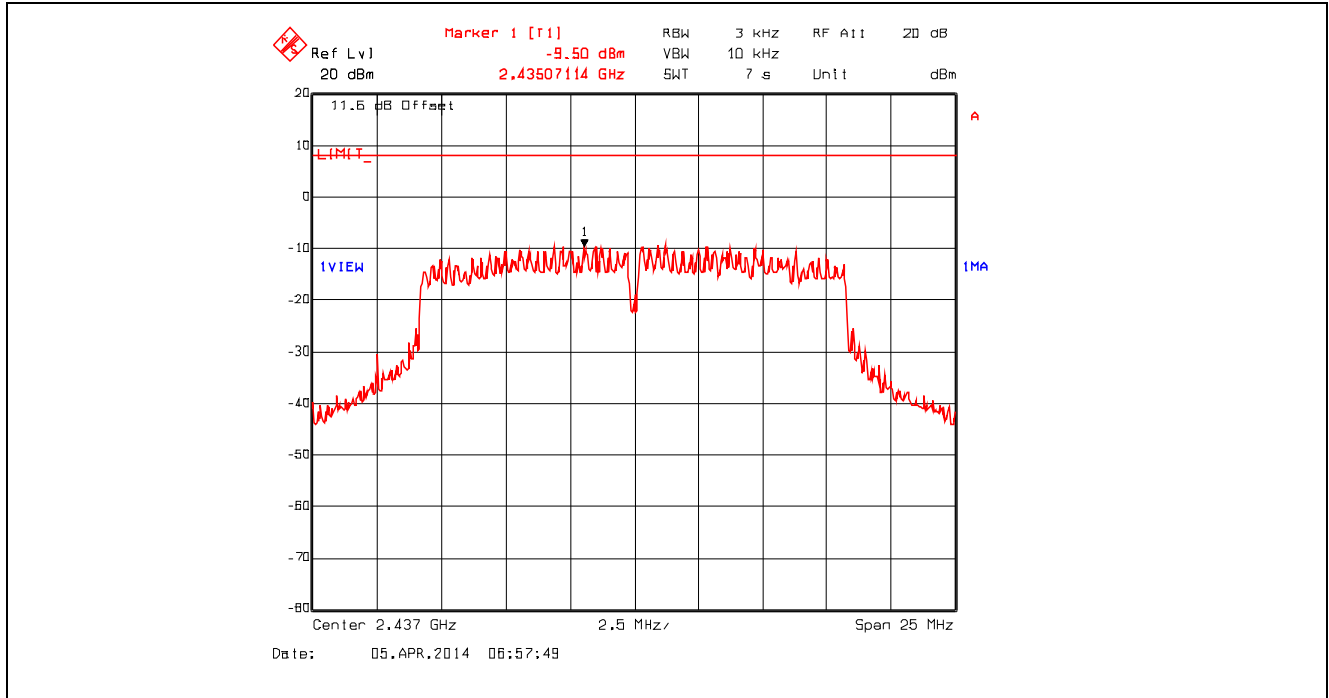
Plot 5.6.4.17. Power Spectral Density, 802.11g, 36 Mbps 16-QAM, 2437 MHz
