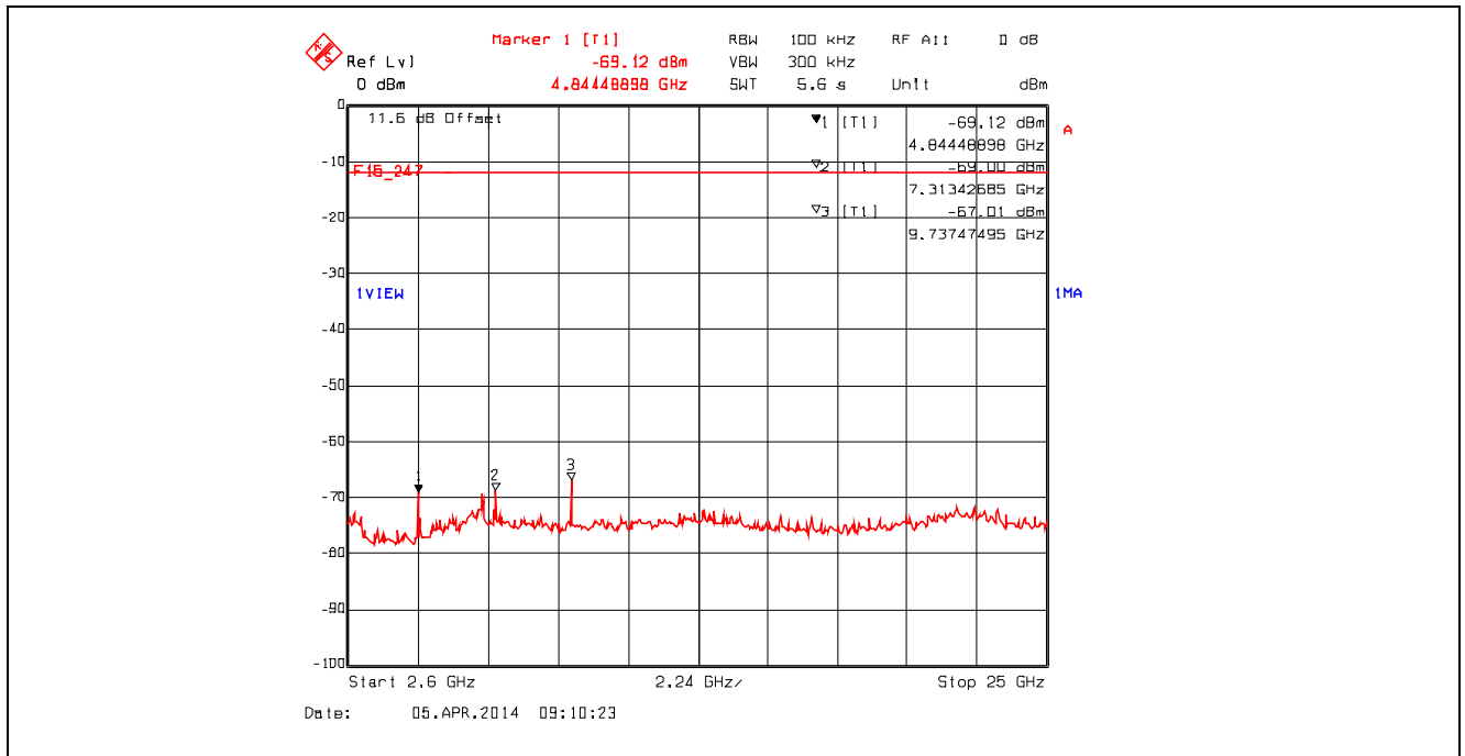
Plot 5.4.4.2.10. Conducted Spurious Emissions - Non Restricted Frequency Bands 802.11g, 2437 MHz, 9 Mbps, 2.6 GHz - 25 GHz
