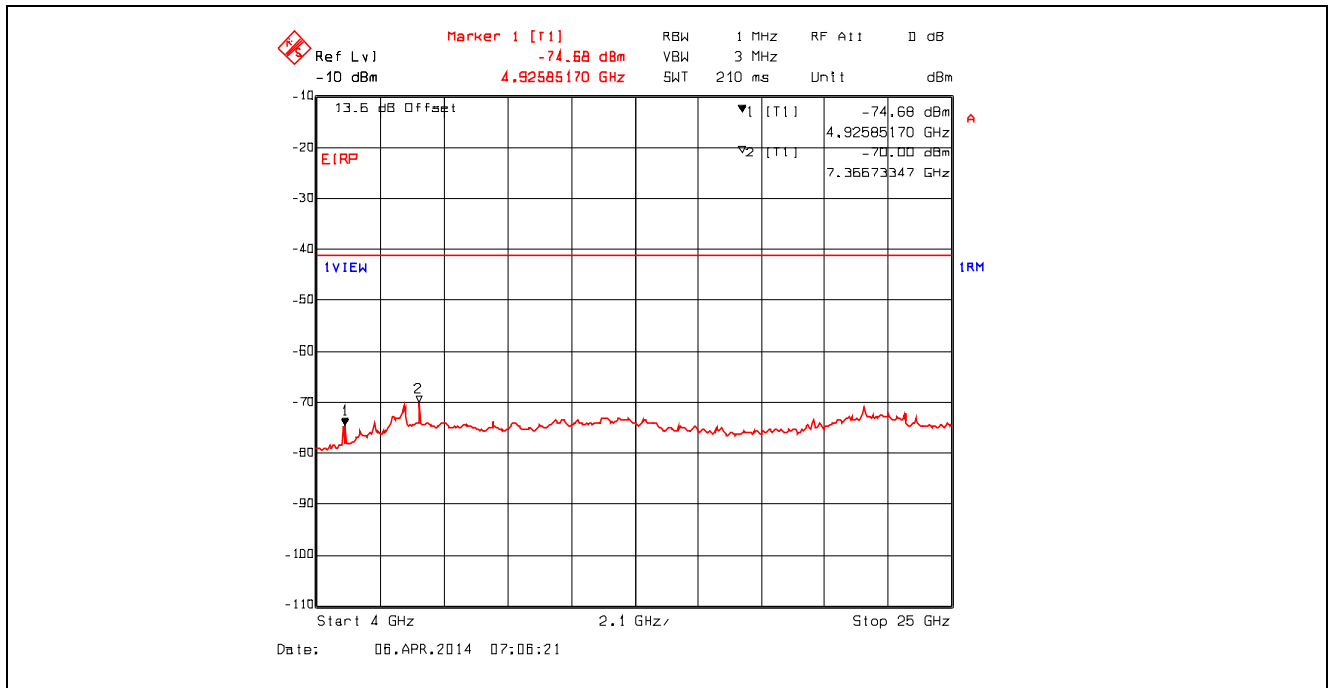
Plot 5.4.4.3.30. Conducted Spurious Emissions – Restricted Bands 802.11g, 9 Mbps, 2462 MHz, 4 GHz - 25 GHz, RMS Detector with High Pass Filter
