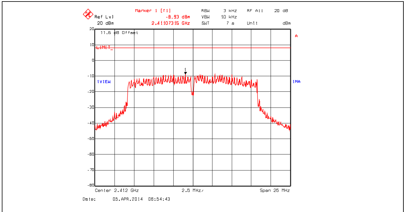
Plot 5.6.4.16. Power Spectral Density, 802.11g, 36 Mbps 16-QAM, 2412 MHz
