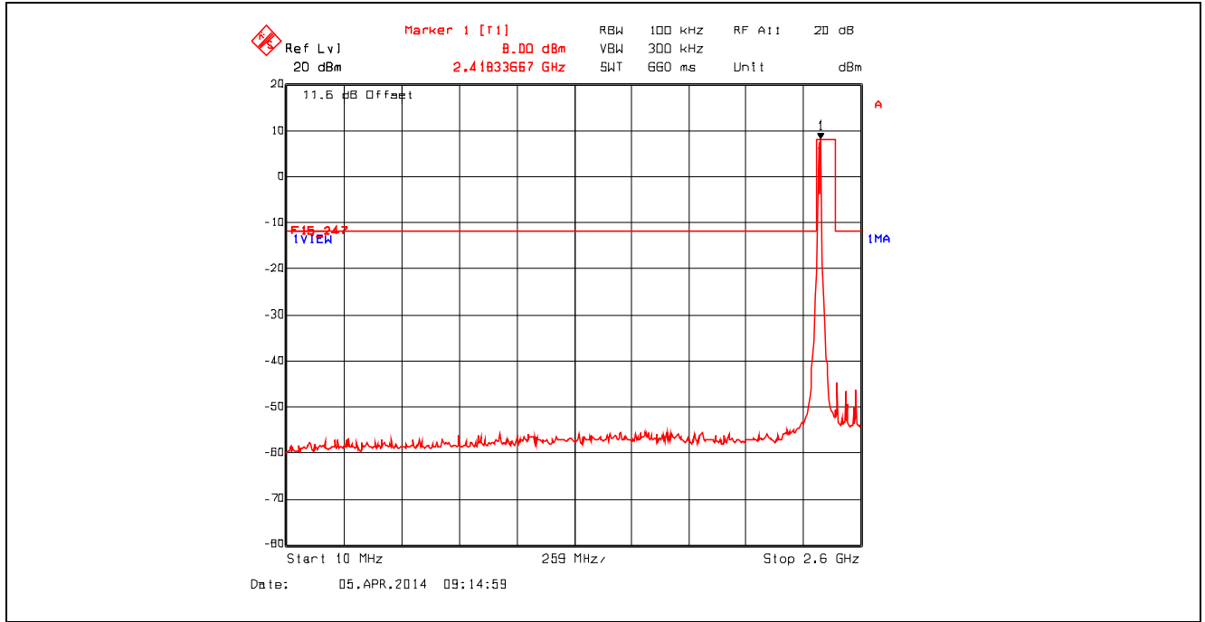
Plot 5.4.4.2.13. Conducted Spurious Emissions - Non Restricted Frequency Bands 802.11n, 2412 MHz, 6.5 Mbps, 10 MHz - 2.6 GHz
