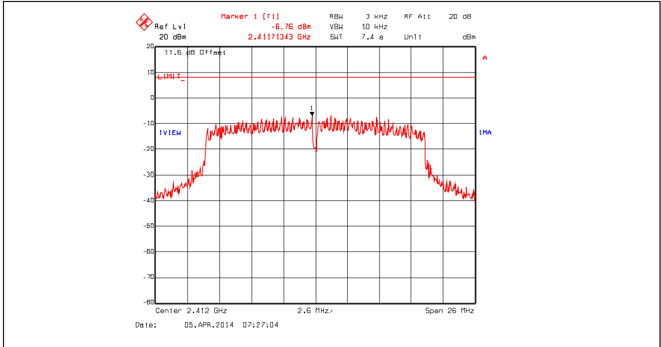
Plot 5.6.4.25. Power Spectral Density, 802.11n 800ns, 19.5 Mbps QPSK 3/4, 2412 MHz
