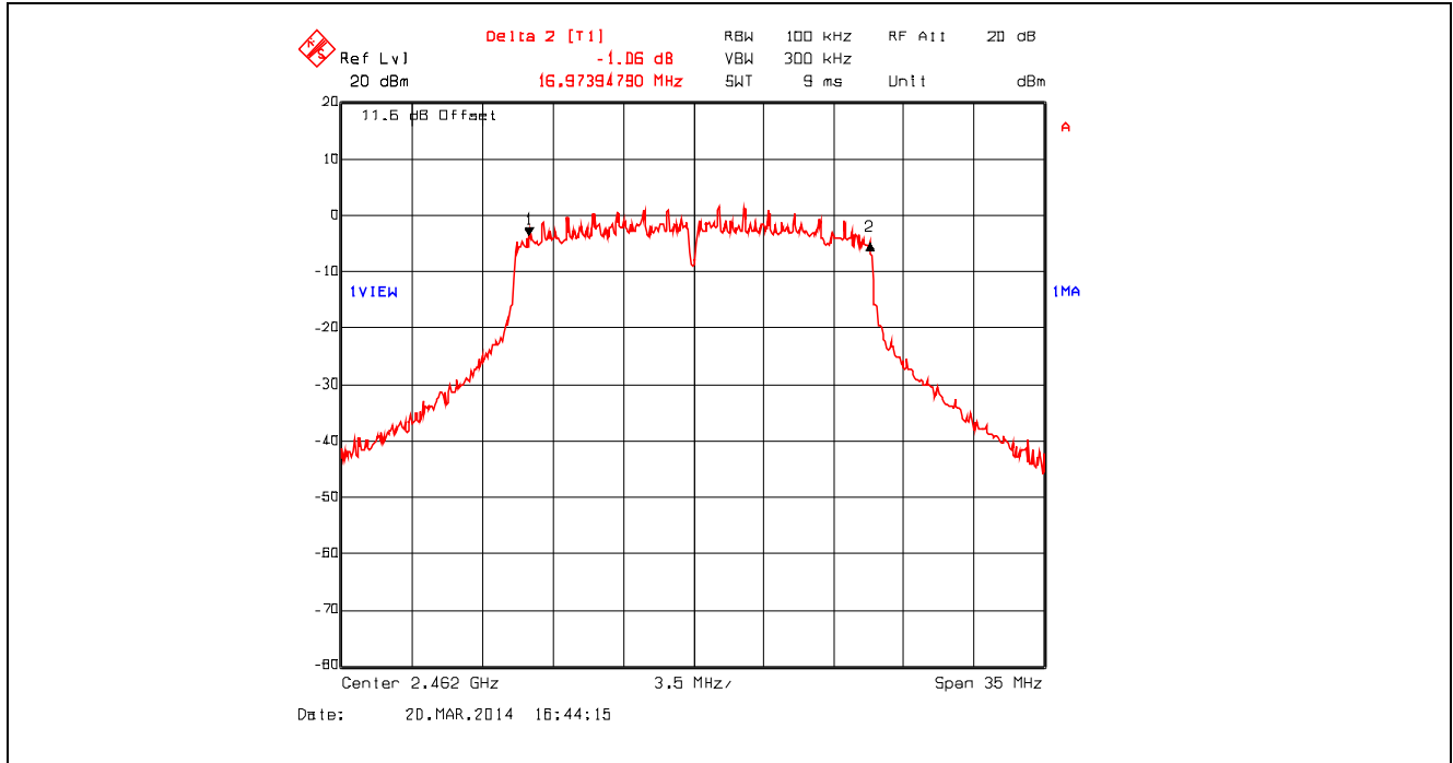
Plot 5.2.4.33. 6 dB Bandwidth, 802.11n 800ns, 65 Mbps 64-QAM 5/6, 2462 MHz
