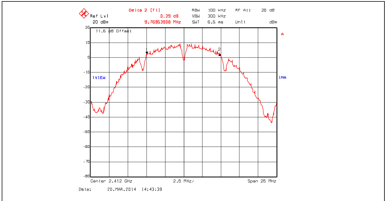
Plot 5.2.4.4. 6 dB Bandwidth, 802.11b, 2 Mbps DQPSK, 2412 MHz
