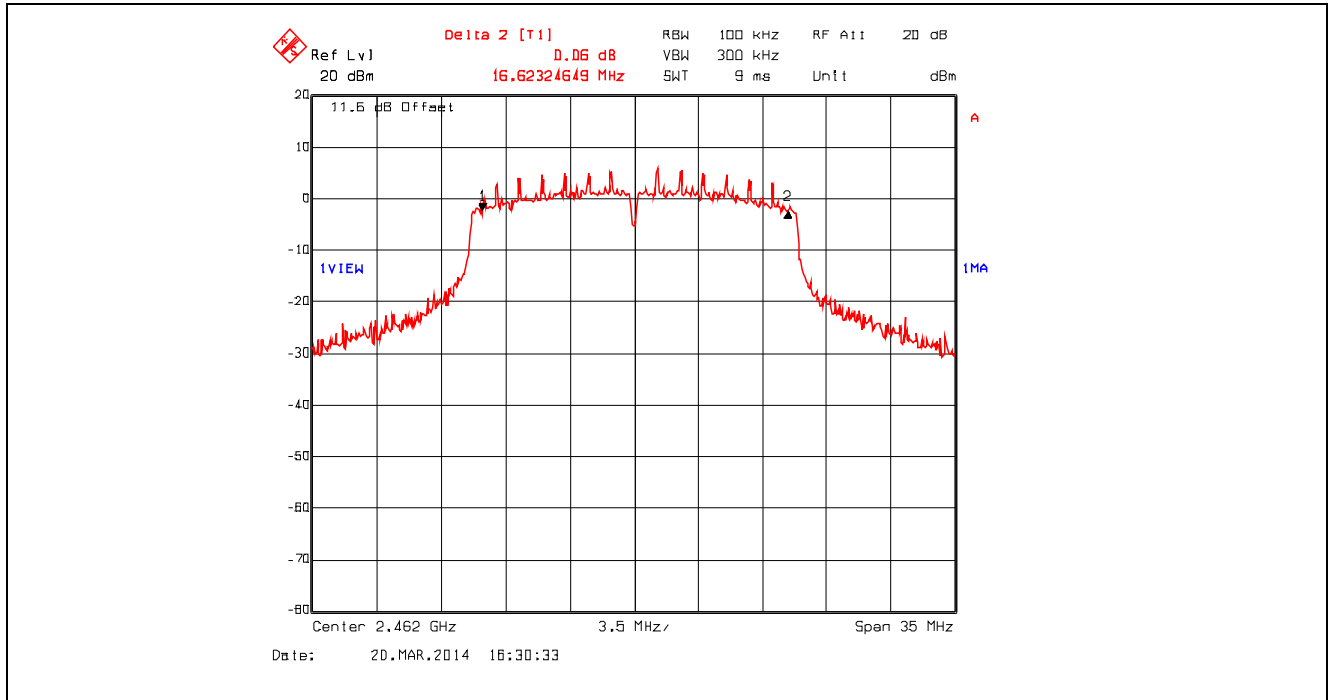
Plot 5.2.4.27. 6 dB Bandwidth, 802.11n 800ns, 19.5 Mbps QPSK 3/4, 2462 MHz
