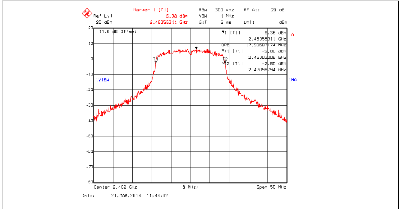
Plot 5.2.4.63. 99% Occupied Bandwidth, 802.11n 800ns, 39 Mbps 16-QAM 3/4, 2462 MHz
