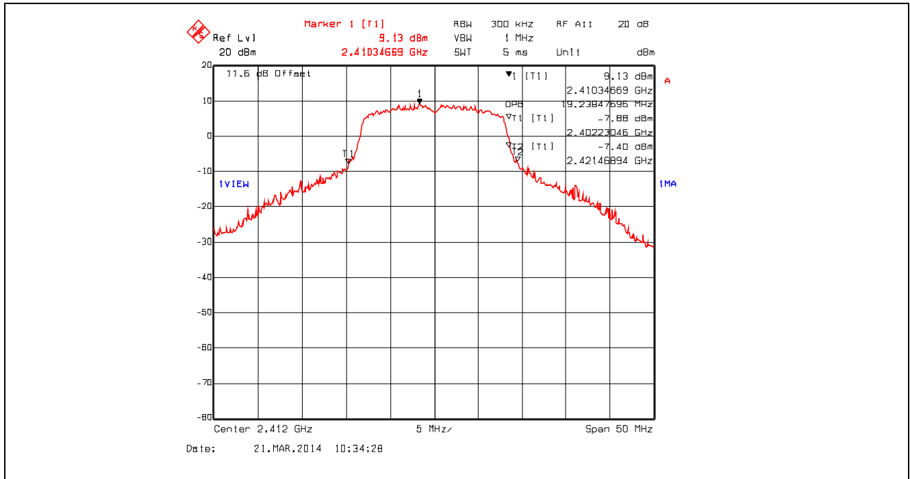
Plot 5.2.4.43. 99% Occupied Bandwidth, 802.11g, 9 Mbps BPSK, 2412 MHz
