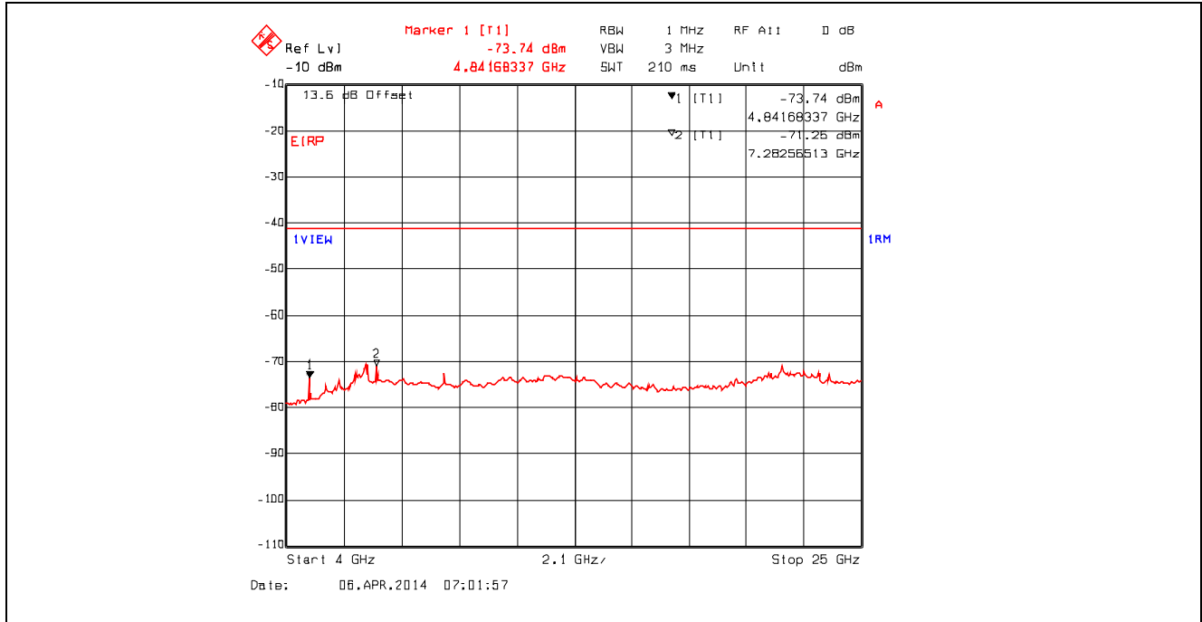
Plot 5.4.4.3.40. Conducted Spurious Emissions – Restricted Bands 802.11n, 6.5 Mbps, 2437 MHz, 4 GHz - 25 GHz, RMS Detector with High Pass Filter
