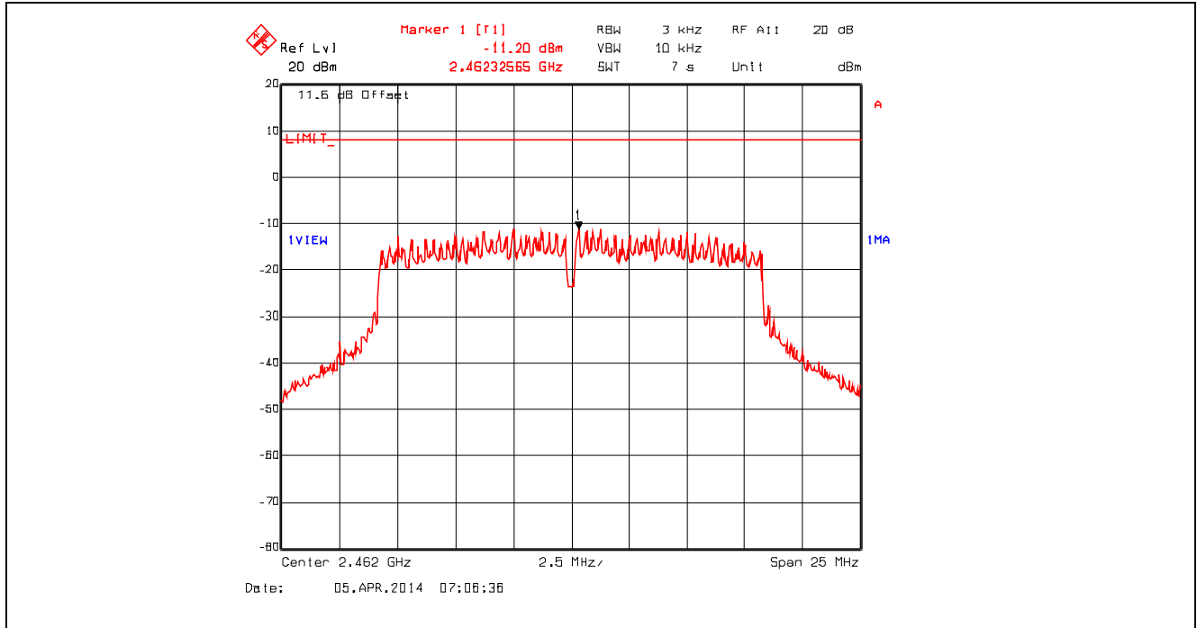
Plot 5.6.4.21. Power Spectral Density, 802.11g, 54 Mbps 64-QAM, 2462 MHz
