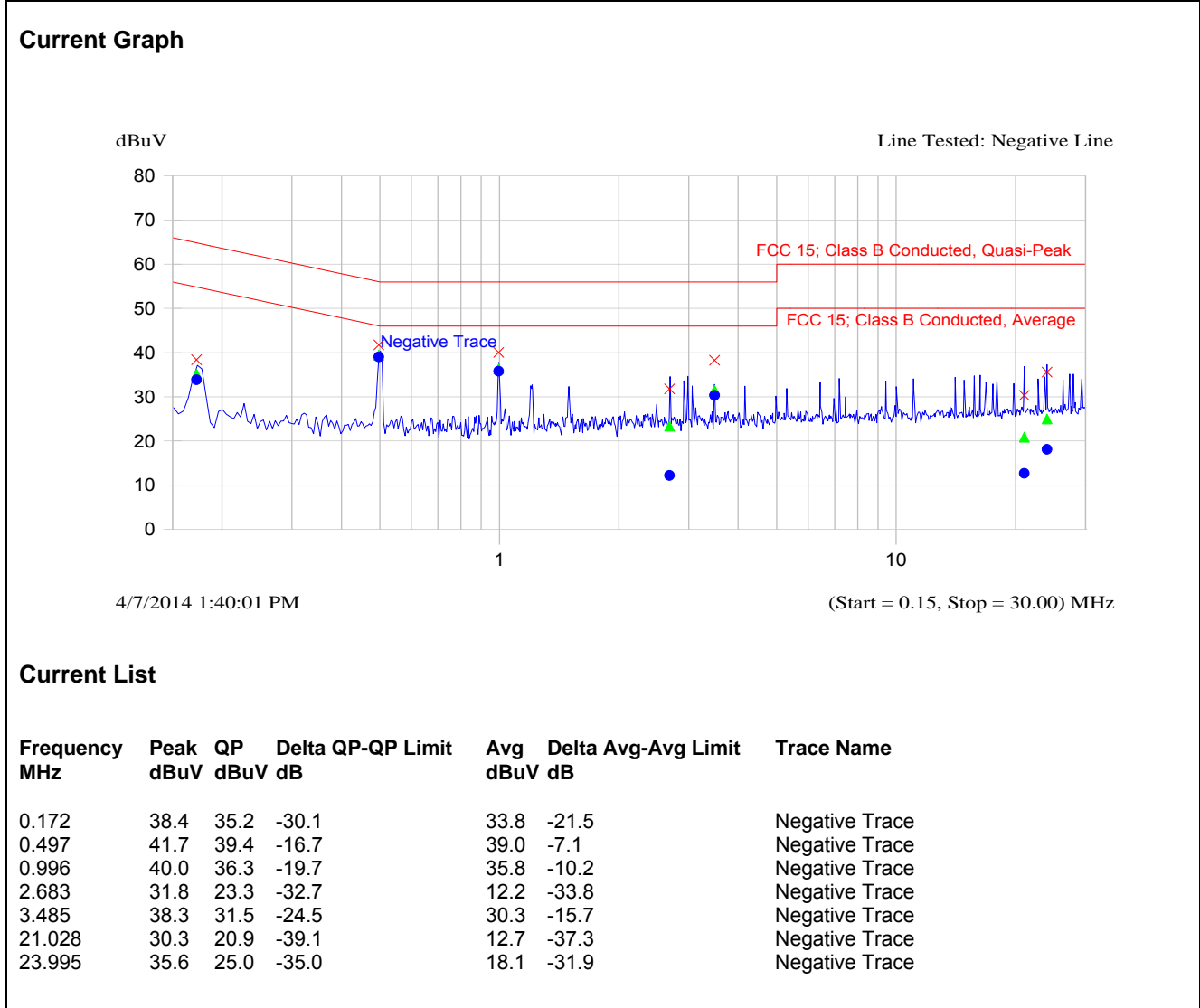
Plot 5.1.4.4. Power Line Conducted Emissions; Line Voltage: 24 V DC; Line Tested: Negative, Tx Mode
