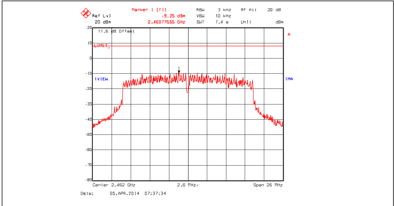
Plot 5.6.4.30. Power Spectral Density, 802.11n 800ns, 39 Mbps 16-QAM 3/4, 2462 MHz
