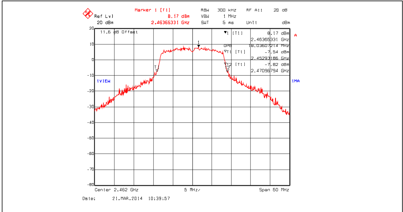
Plot 5.2.4.45. 99% Occupied Bandwidth, 802.11g, 9 Mbps BPSK, 2462 MHz
