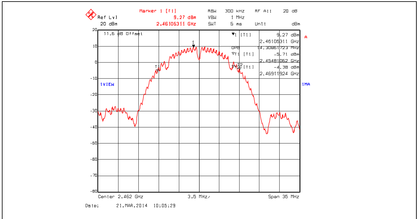
Plot 5.2.4.36. 99% Occupied Bandwidth, 802.11b, 1 Mbps DBPSK, 2462 MHz
