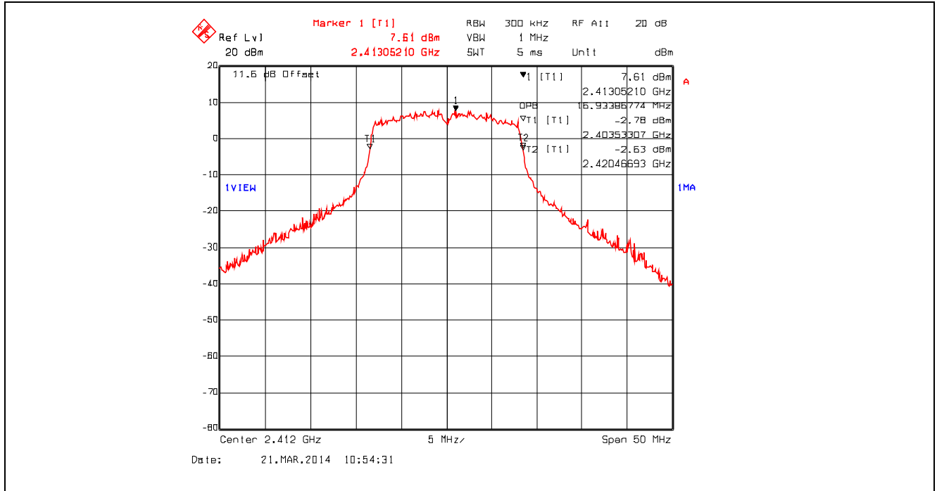
Plot 5.2.4.49. 99% Occupied Bandwidth, 802.11g, 36 Mbps 16-QAM, 2412 MHz
