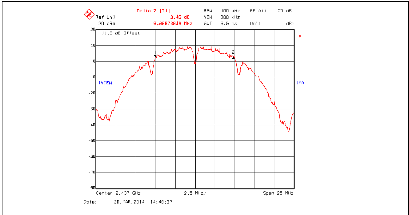
Plot 5.2.4.5. 6 dB Bandwidth, 802.11b, 2 Mbps DQPSK, 2437 MHz
