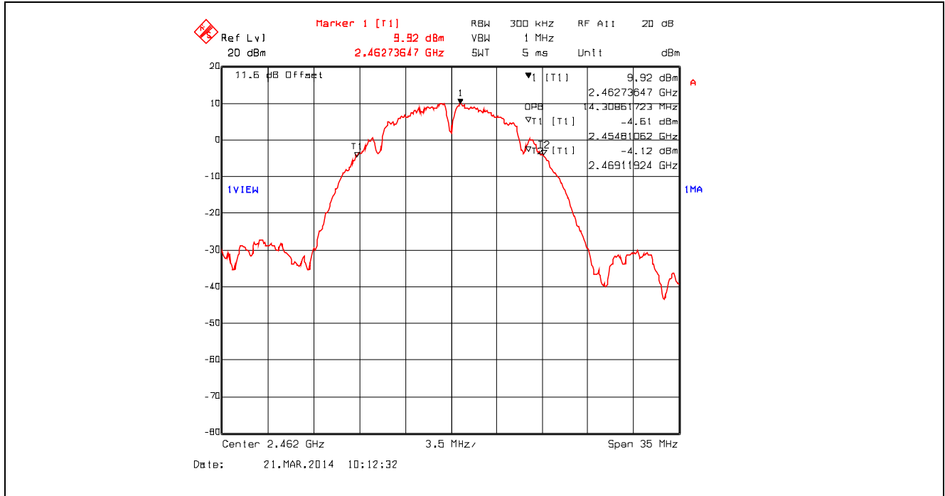
Plot 5.2.4.39. 99% Occupied Bandwidth, 802.11b, 2 Mbps DQPSK, 2462 MHz
