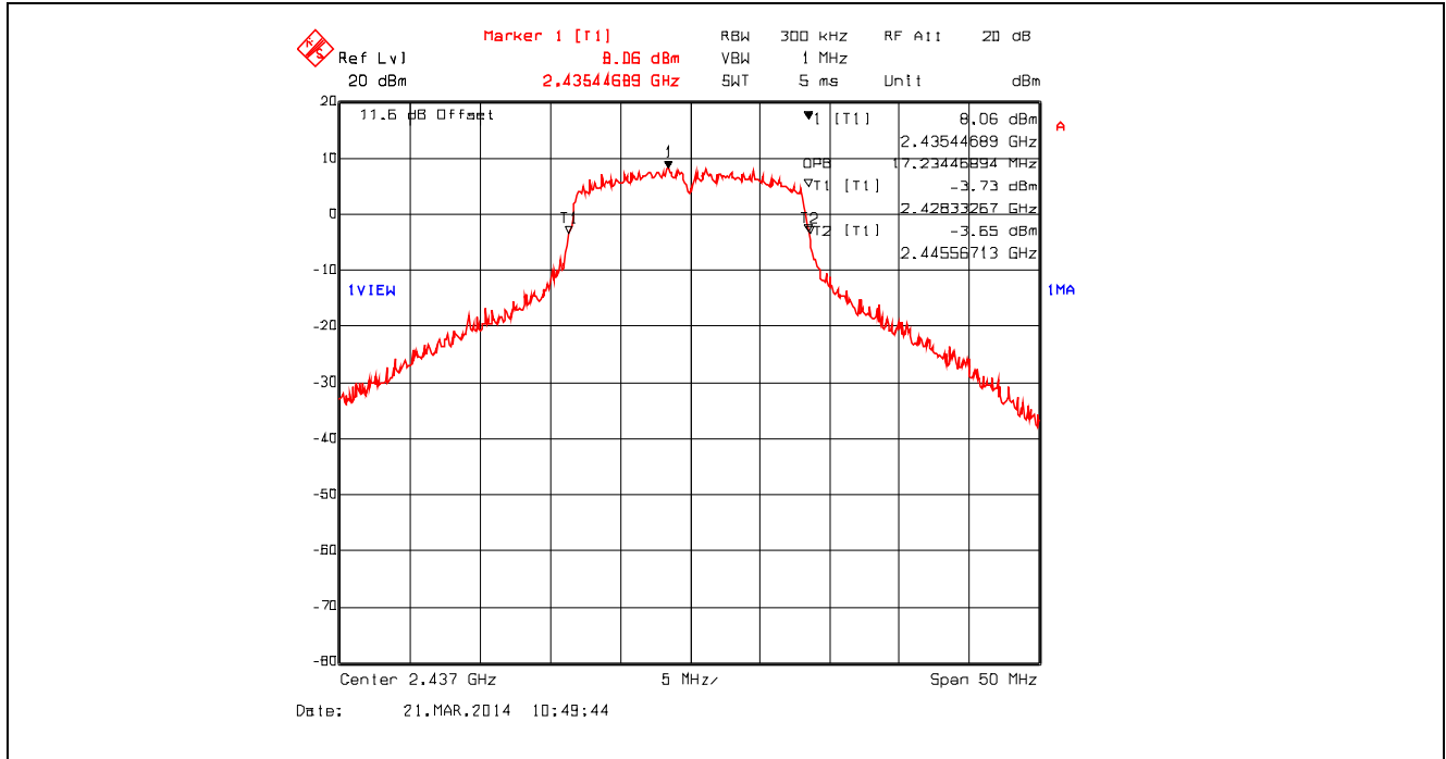
Plot 5.2.4.47. 99% Occupied Bandwidth, 802.11g, 18 Mbps QPSK, 2437 MHz
