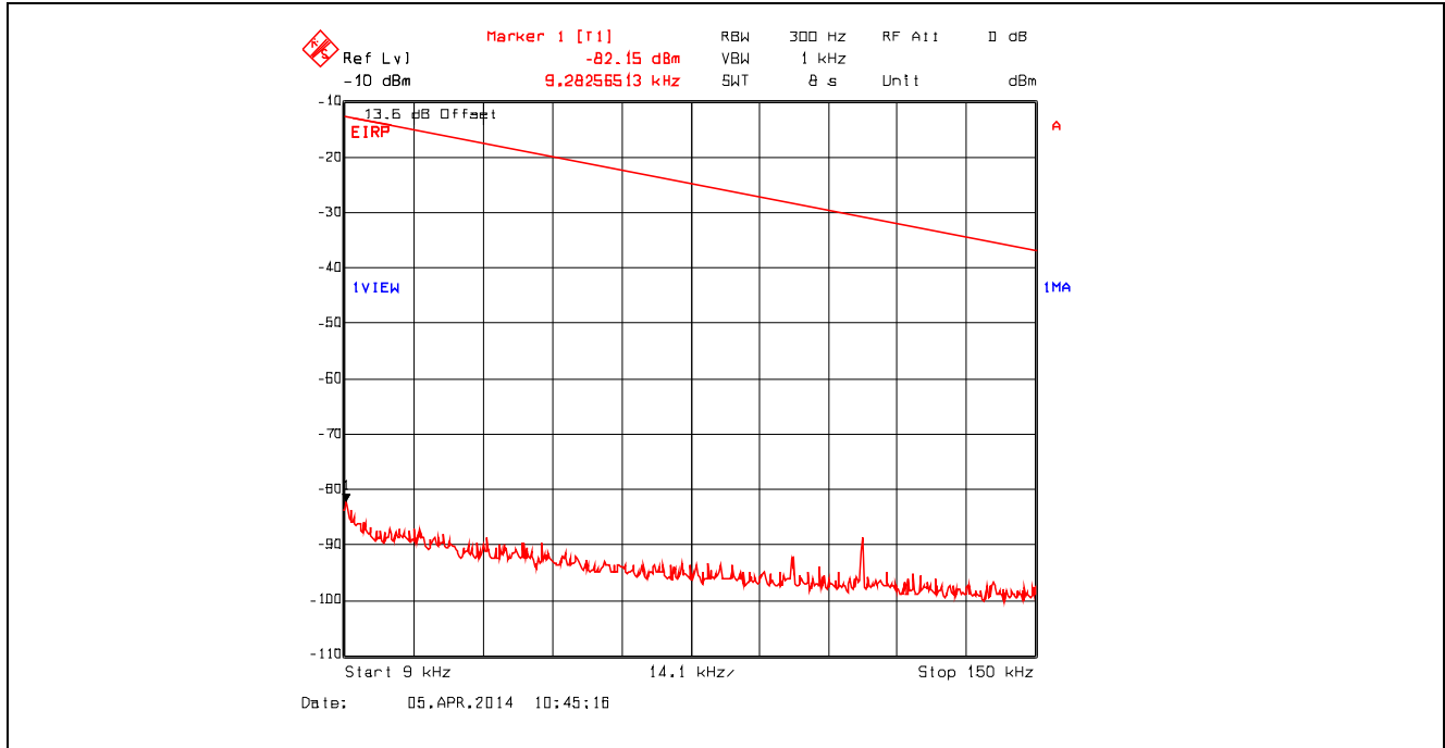
Plot 5.4.4.3.11. Conducted Spurious Emissions – Restricted Bands 802.11b, 1 Mbps, 2462 MHz, 9 kHz - 150 kHz, Peak Detector with Band (Notch) Reject Filter
