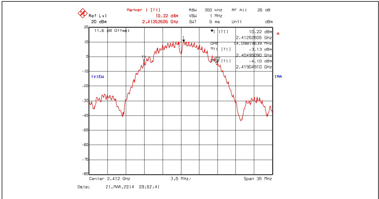
Plot 5.2.4.34. 99% Occupied Bandwidth, 802.11b, 1 Mbps DBPSK, 2412 MHz
