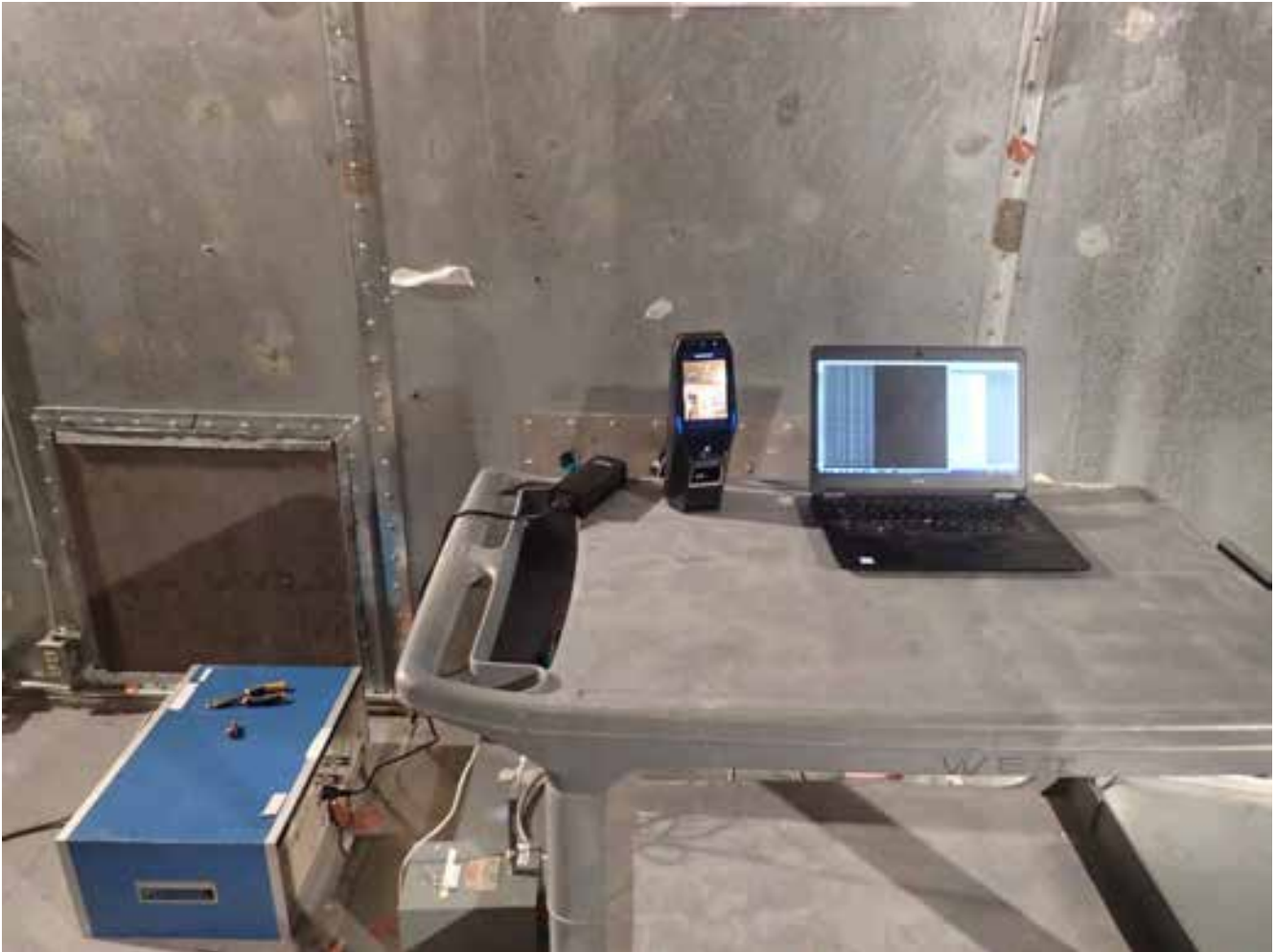
Power Line Conducted Emissions (EUT Powered by PoE Injector Power over Ethernet)
