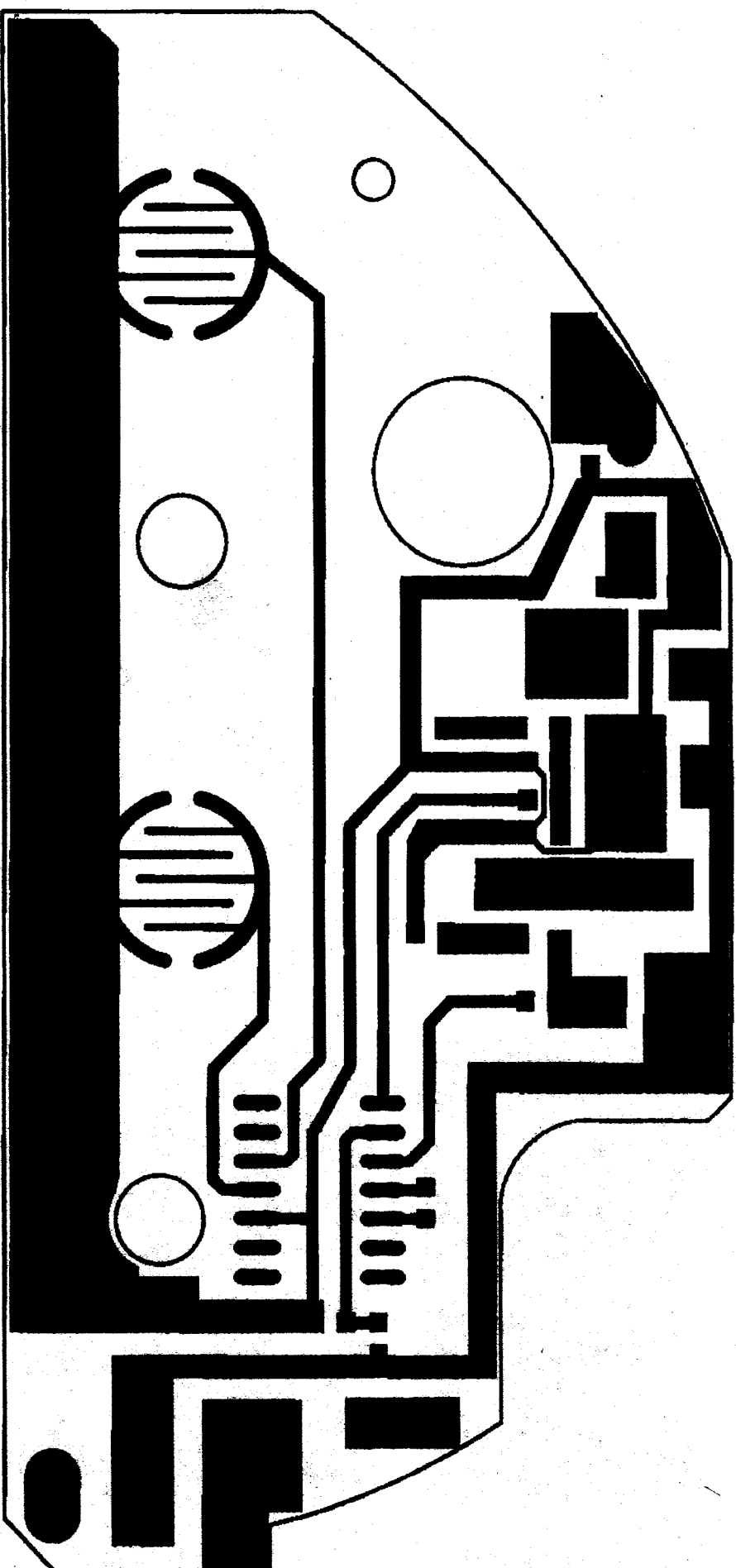
Transmitter PCB Bottom Layer Layout
