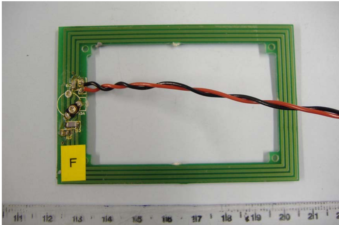
LARGER REMOTE ANTENNA (81mm x 54mm)
