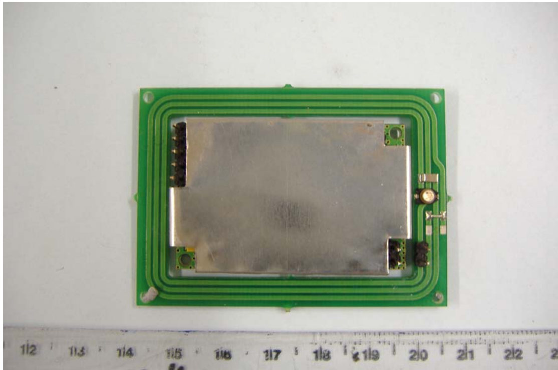
EUT TOP OVERVIEW ATTACHED ANTENNA (61mm x 45mm)
