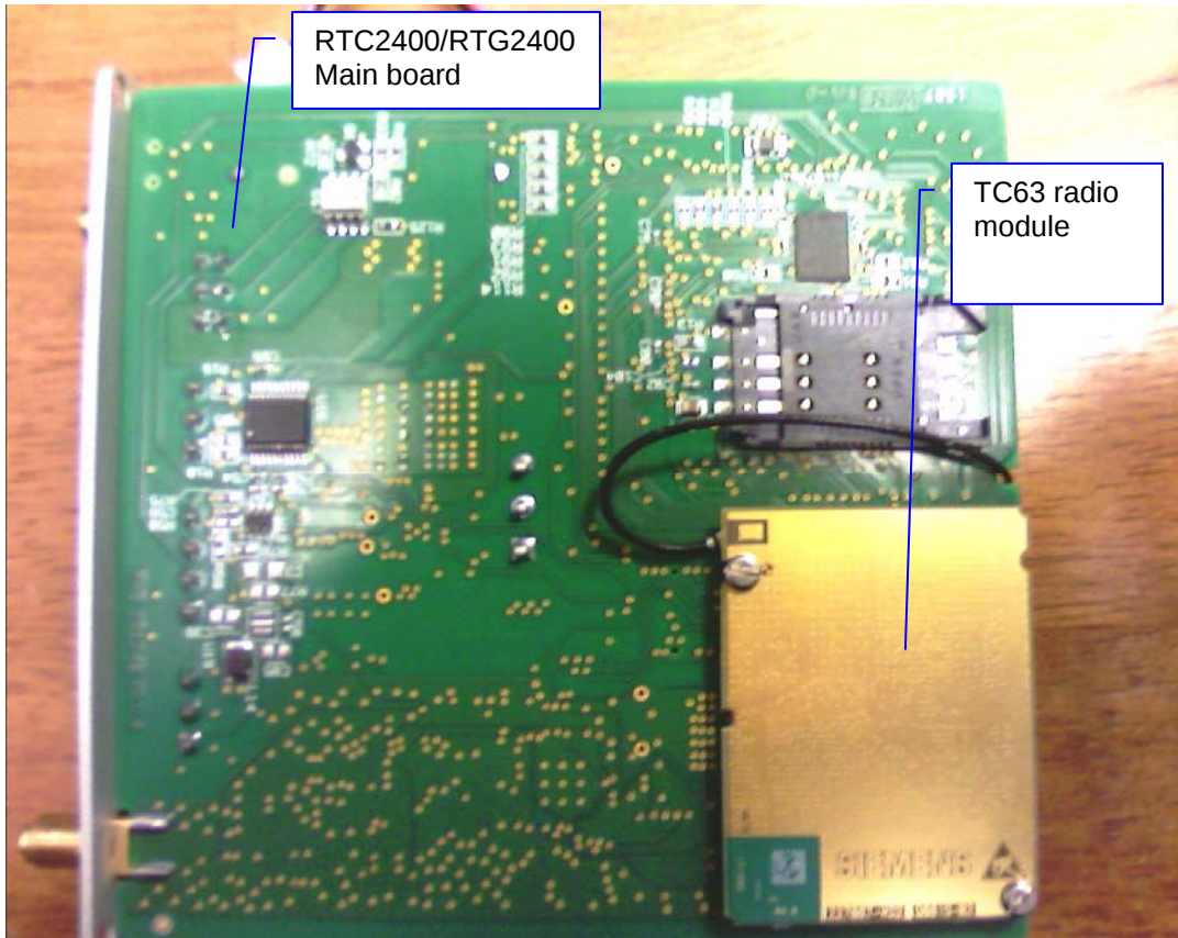
RTG2400 main board with TC63 radio module
