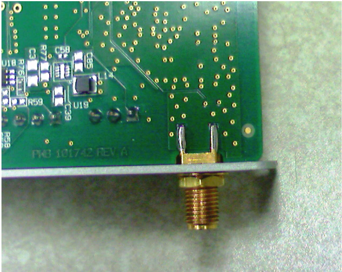
Photo 4 - Motherboard (back of Zigbee radio circuit)
