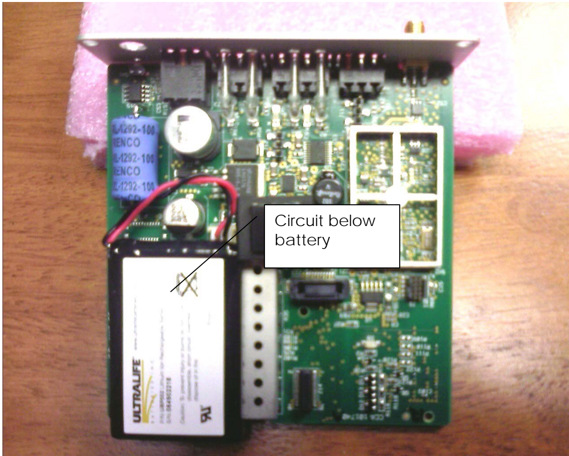
Photo 6 - Motherboard - Top without shields
