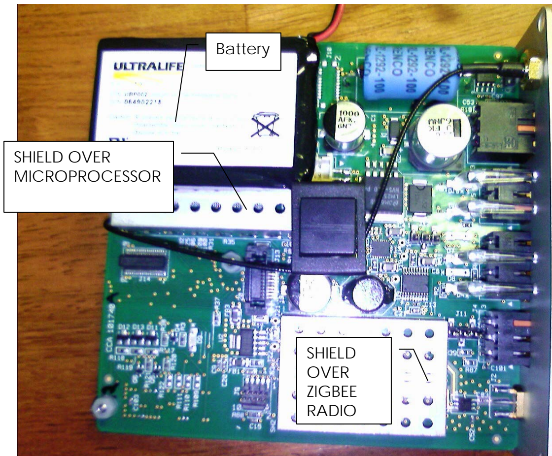
Photo 1 – Mother Board - Top
