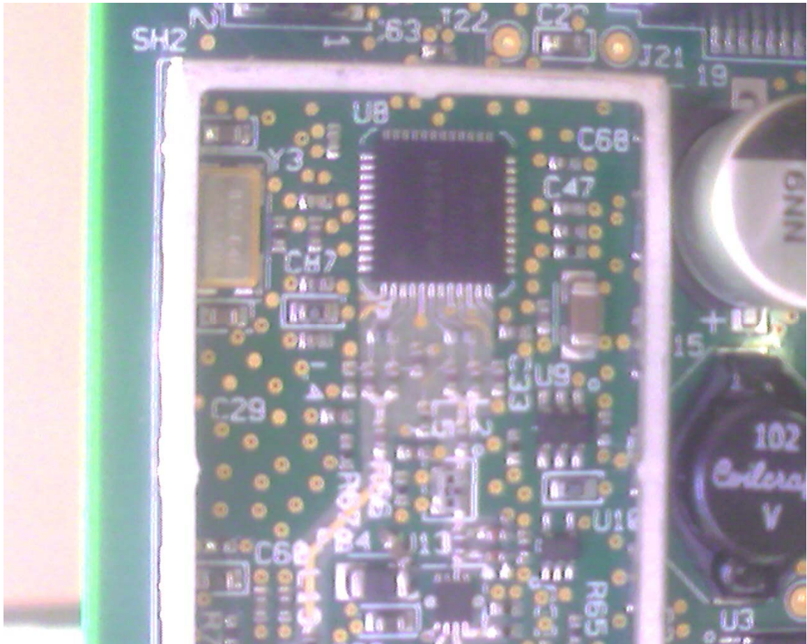
Photo 7 – ZigBee radio circuit (top) without shield closeup
