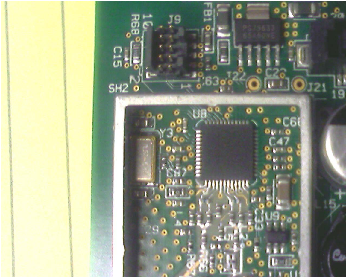
Photo 9 - ZigBee radio circuit (top) closeup
