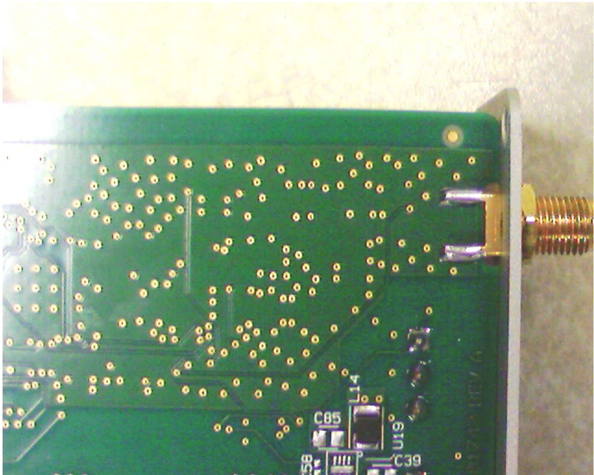
Photo 5 - Motherbaord bottom - Back of ZigBee radio circuit
