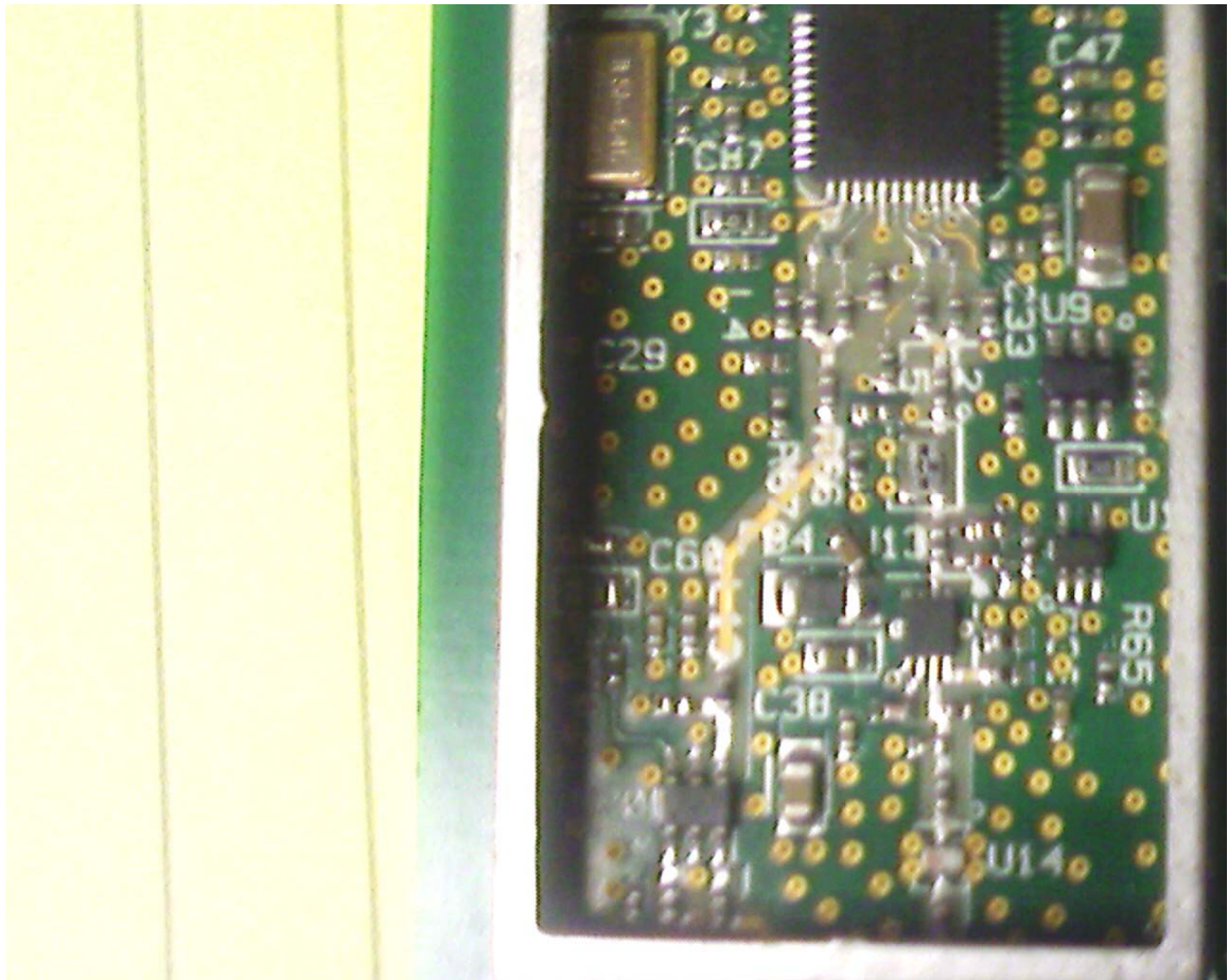
Photo 10 - ZigBee radio circuit (top) closeup
