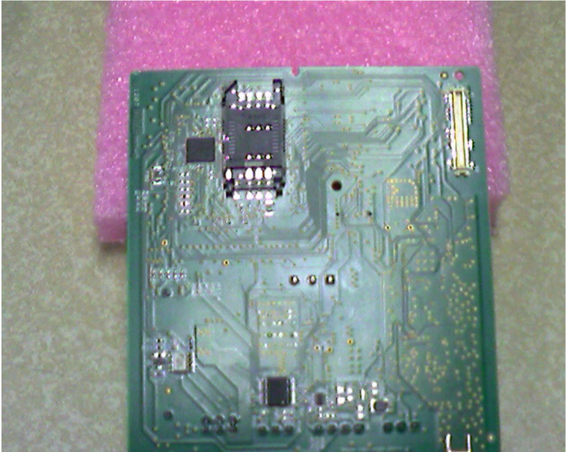
Photo 3 - Motherboard Bottom
