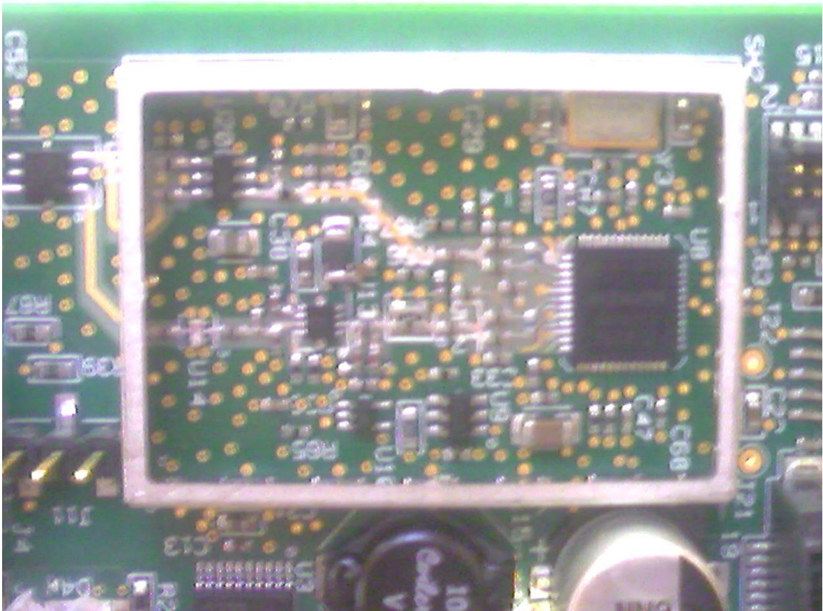
Photo 8 - ZigBee radio circuit (top) without shield
