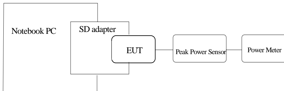
Figure 3: Output power measurement configuration.
