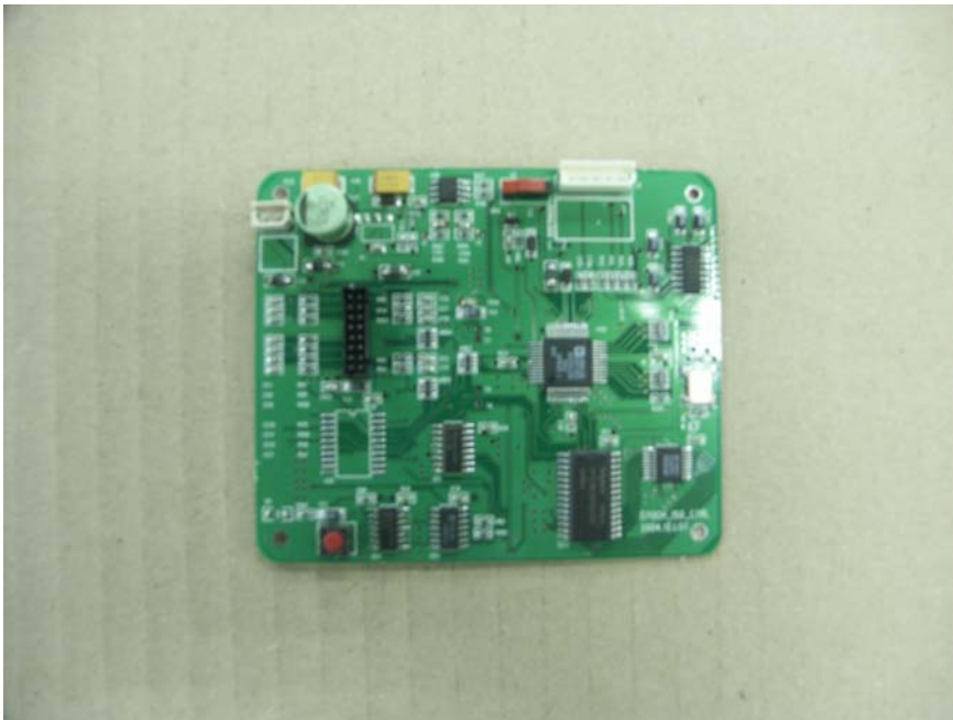
Isolation Module (EMM-04-040) – Board2 Bottom View
