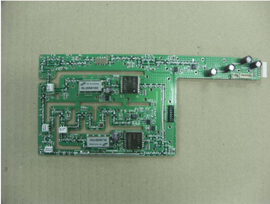
Isolation Module (EMM-04-040) – Board1 Bottom View
