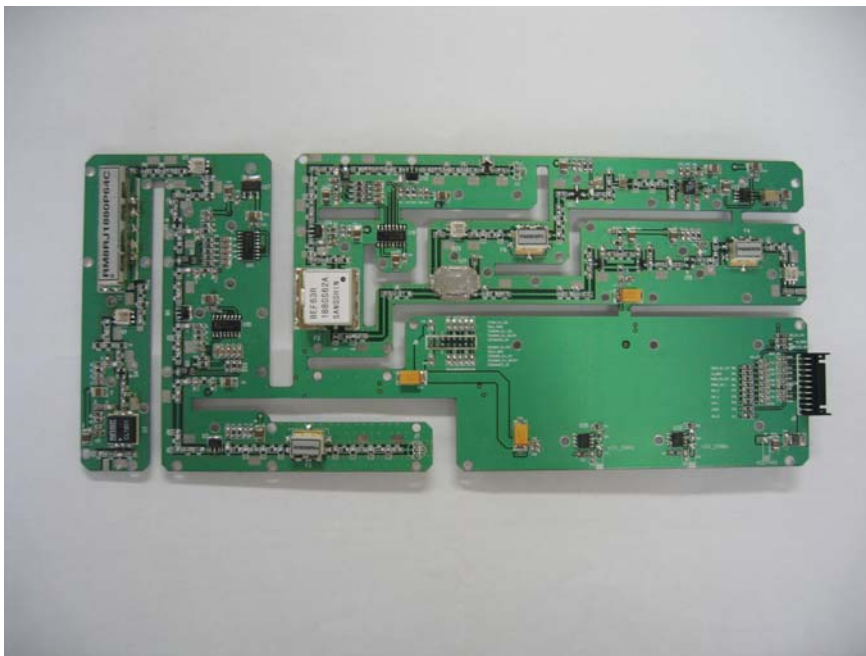
UDC Module (EMM-04-039) - Circuit board Rear Top
