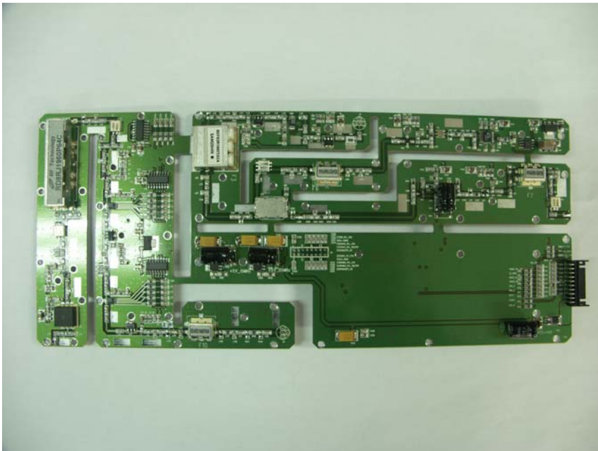
UDC Module (EMM-04-038) - Circuit Board Front Top
