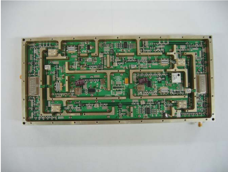
UDC Module (EMM-04-038) - Unit Internal Rear
