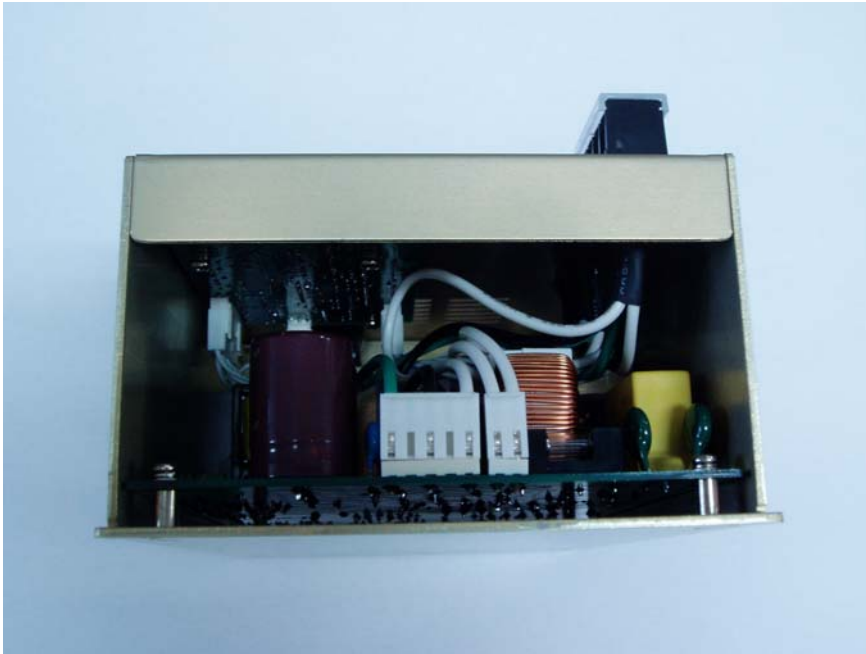
Power Supply (MPSA300-270605-F) View 3
