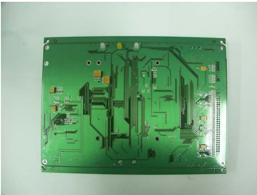
Isolation Module (EMM-04-040) – Board1 Top View
