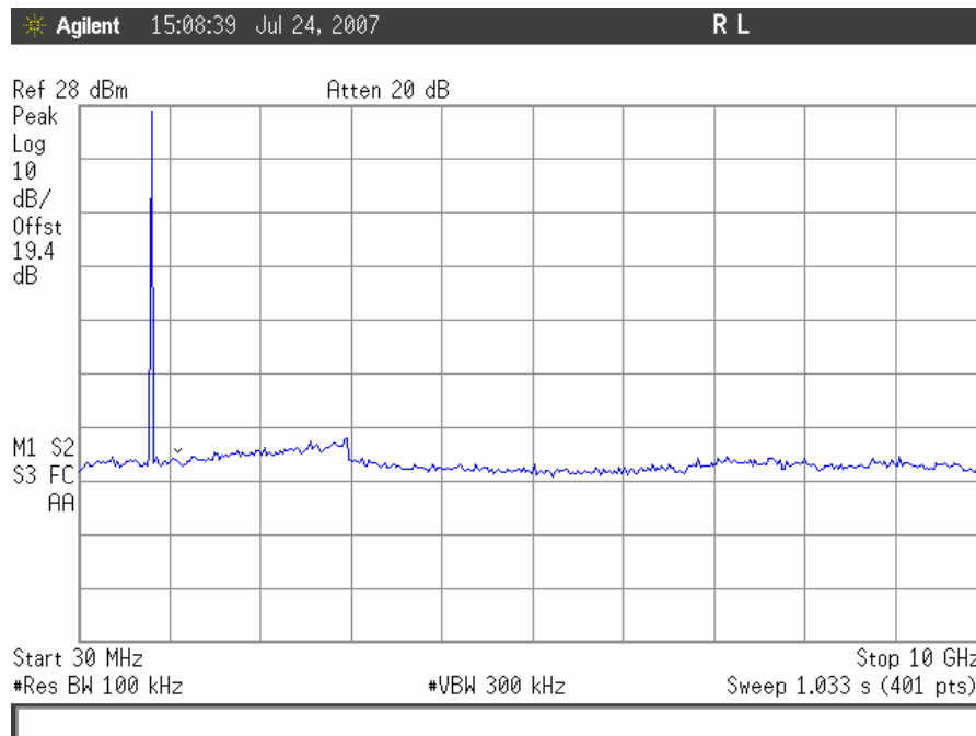
Conducted Spurious Emissions, TDMA High Channel Uplink
