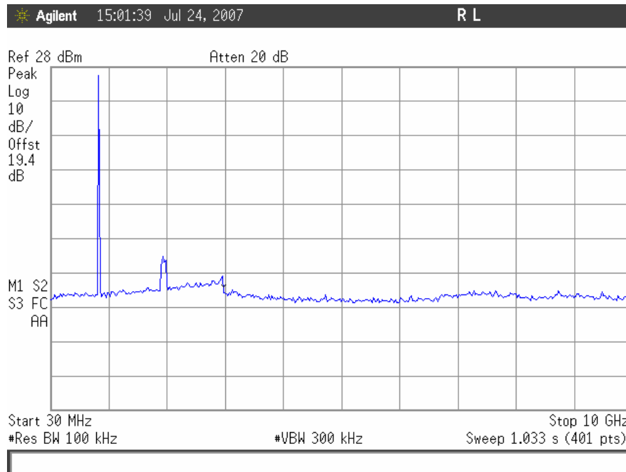
Conducted Spurious Emissions, GSM Mid Channel Downlink, 30MHz – 10GHz
