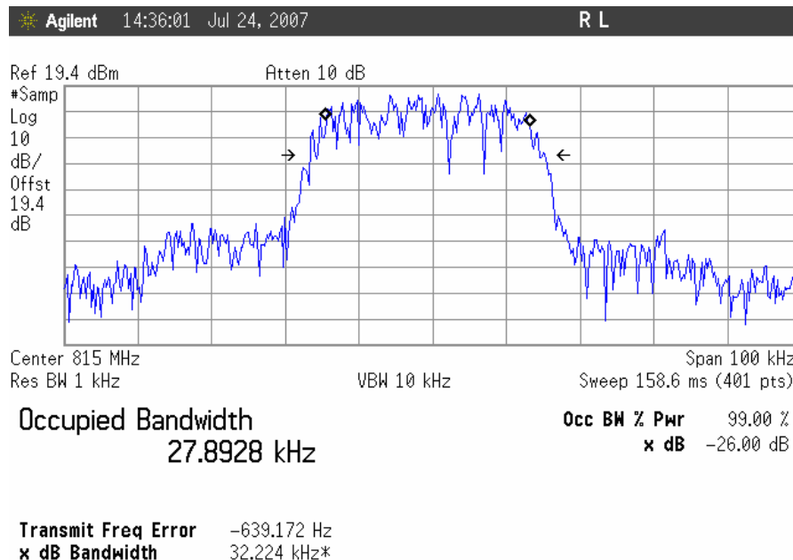
Occupied Bandwidth, TDMA Uplink, Mid Channel Output
