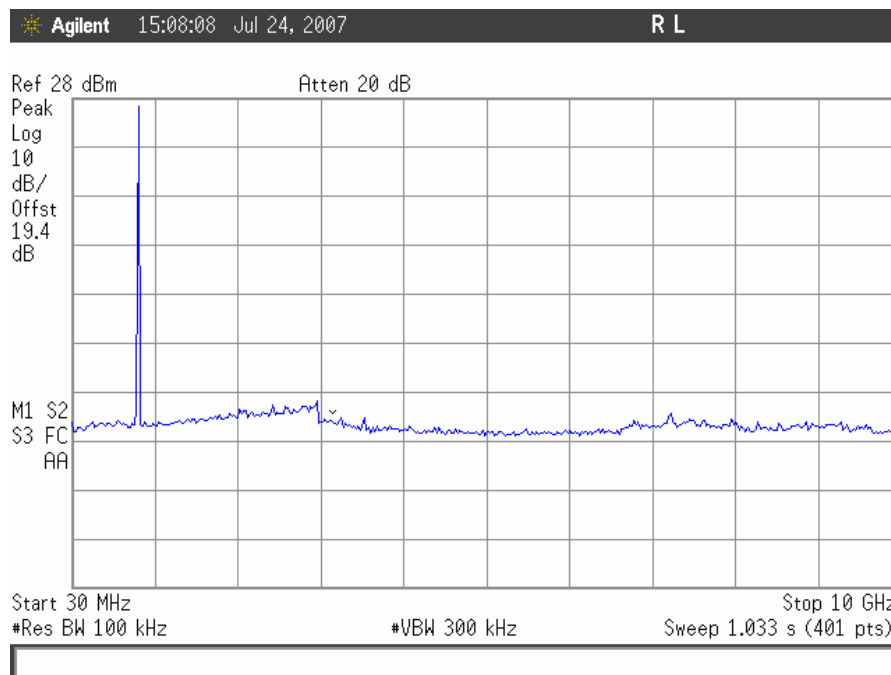
Conducted Spurious Emissions, TDMA Mid Channel Uplink
