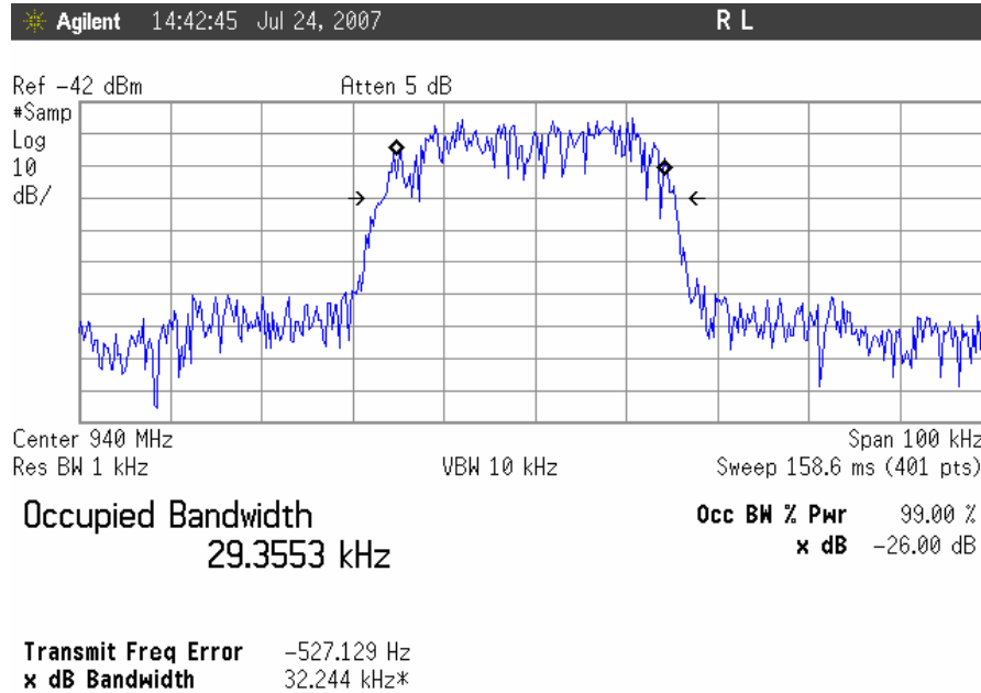
Occupied Bandwidth, TDMA Downlink, High Channel Input
