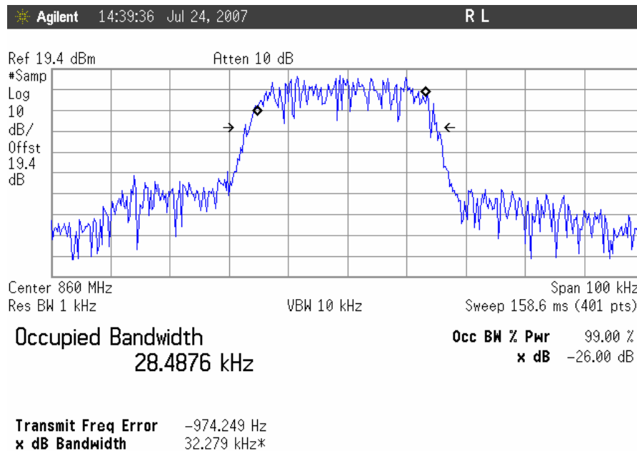
Occupied Bandwidth, TDMA Downlink, Mid Channel Output
