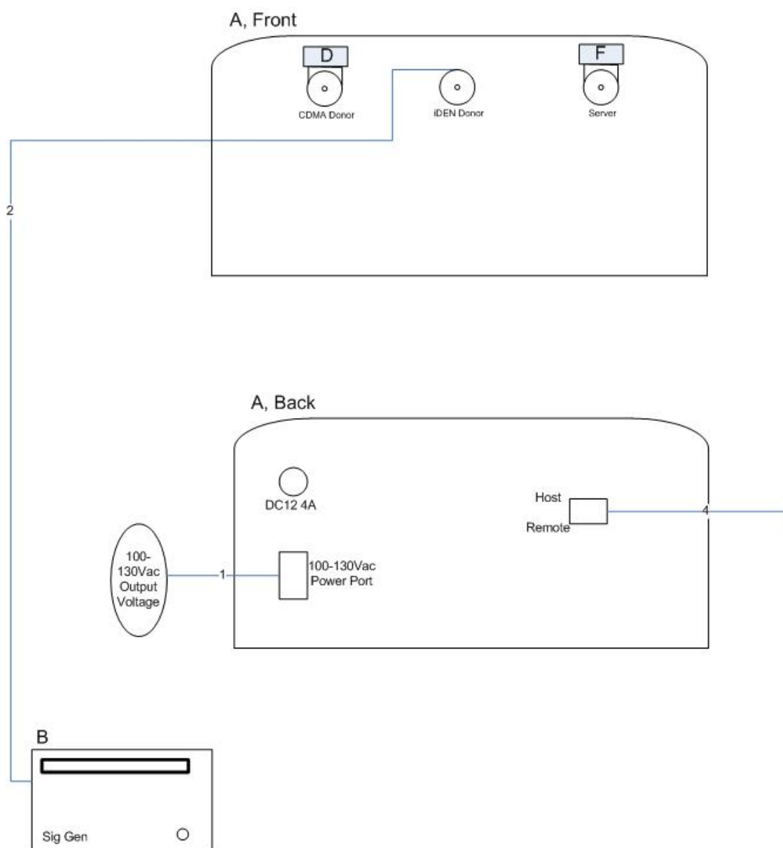
Figure 4. Block Diagram of Test Configuration (Spurious Emissions – Downlink)
