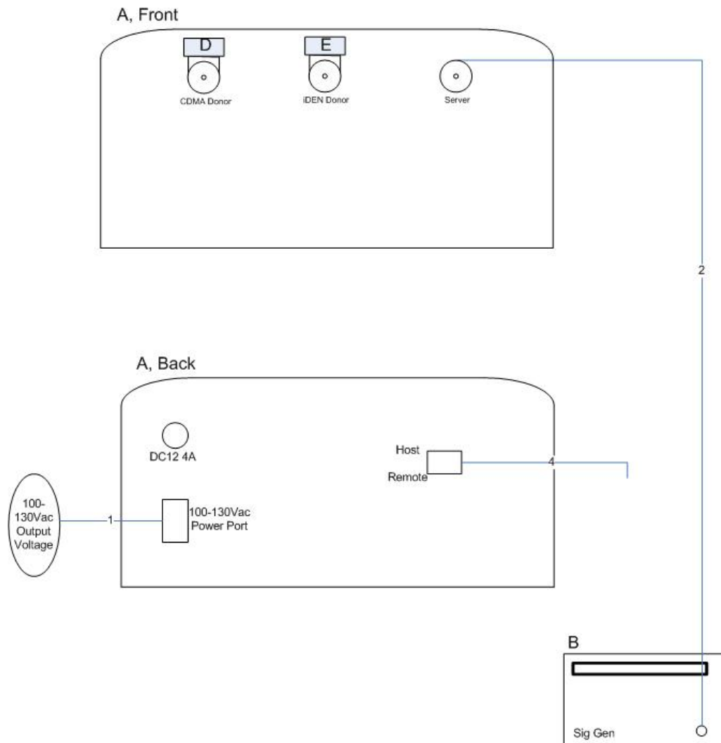
Figure 5. Block Diagram of Test Configuration (Spurious Emissions – Uplink)
