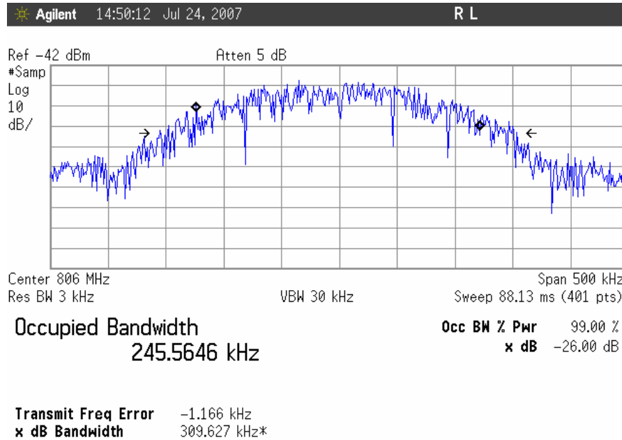
Occupied Bandwidth, GSM Uplink, Low Channel Input
