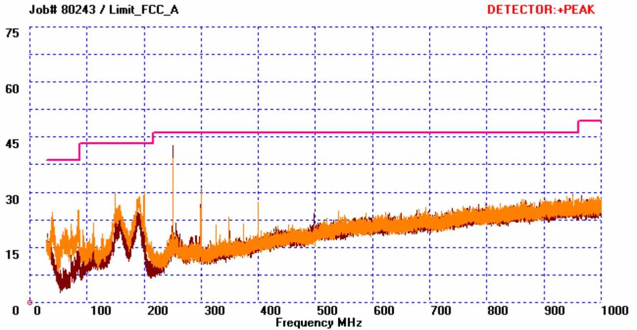
Radiated Emissions 30MHz – 1GHz Plot
