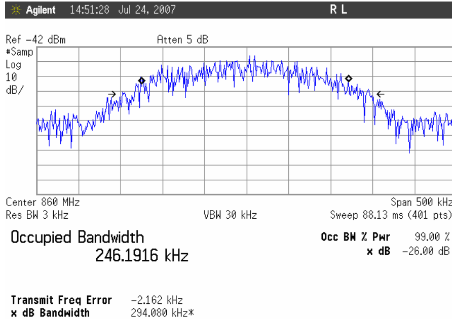
Occupied Bandwidth, GSM Downlink, Mid Channel Input
