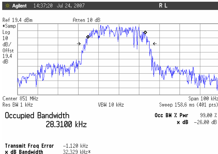
Occupied Bandwidth, TDMA Downlink, Low Channel Output
