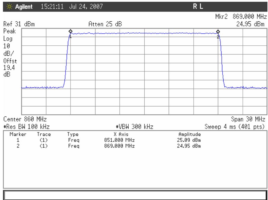
Out of Band Rejection, Downlink 15MHz
