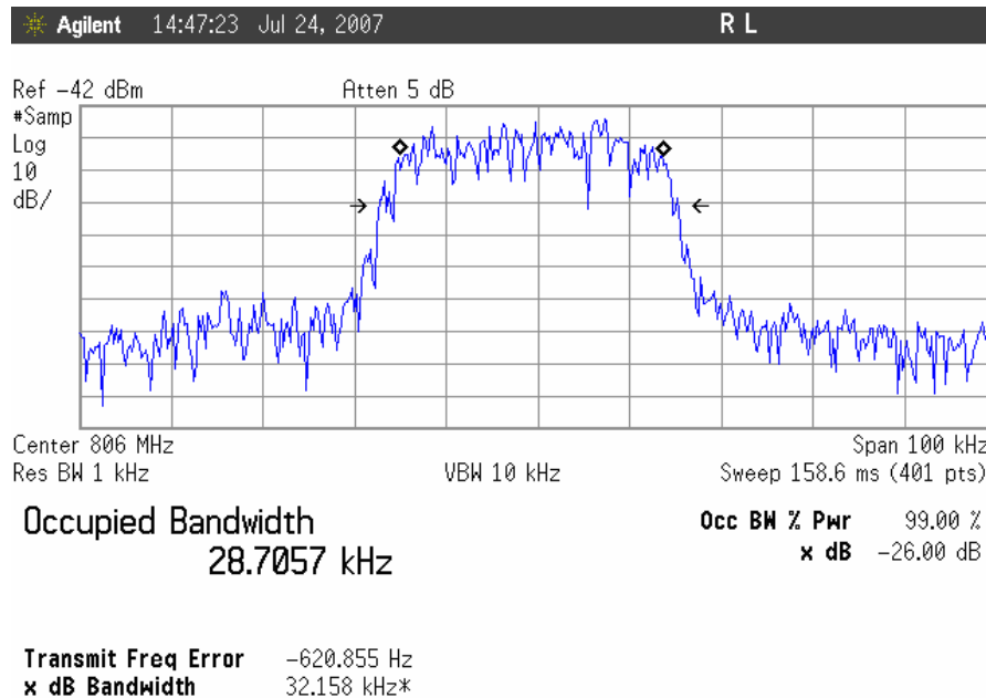
Occupied Bandwidth, TDMA Uplink, Low Channel Input
