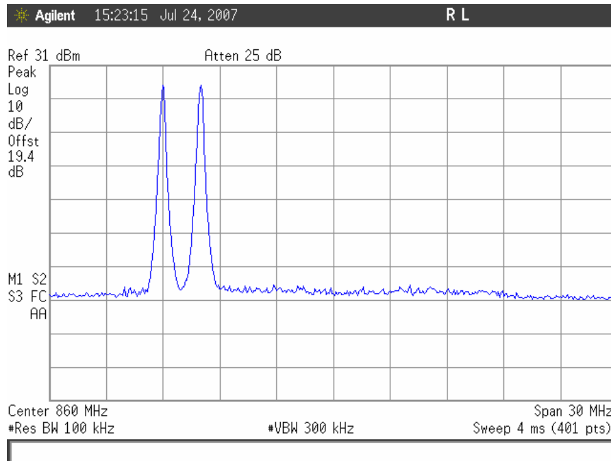
Plot 1. TDMA Intermodulation, Downlink Low End
