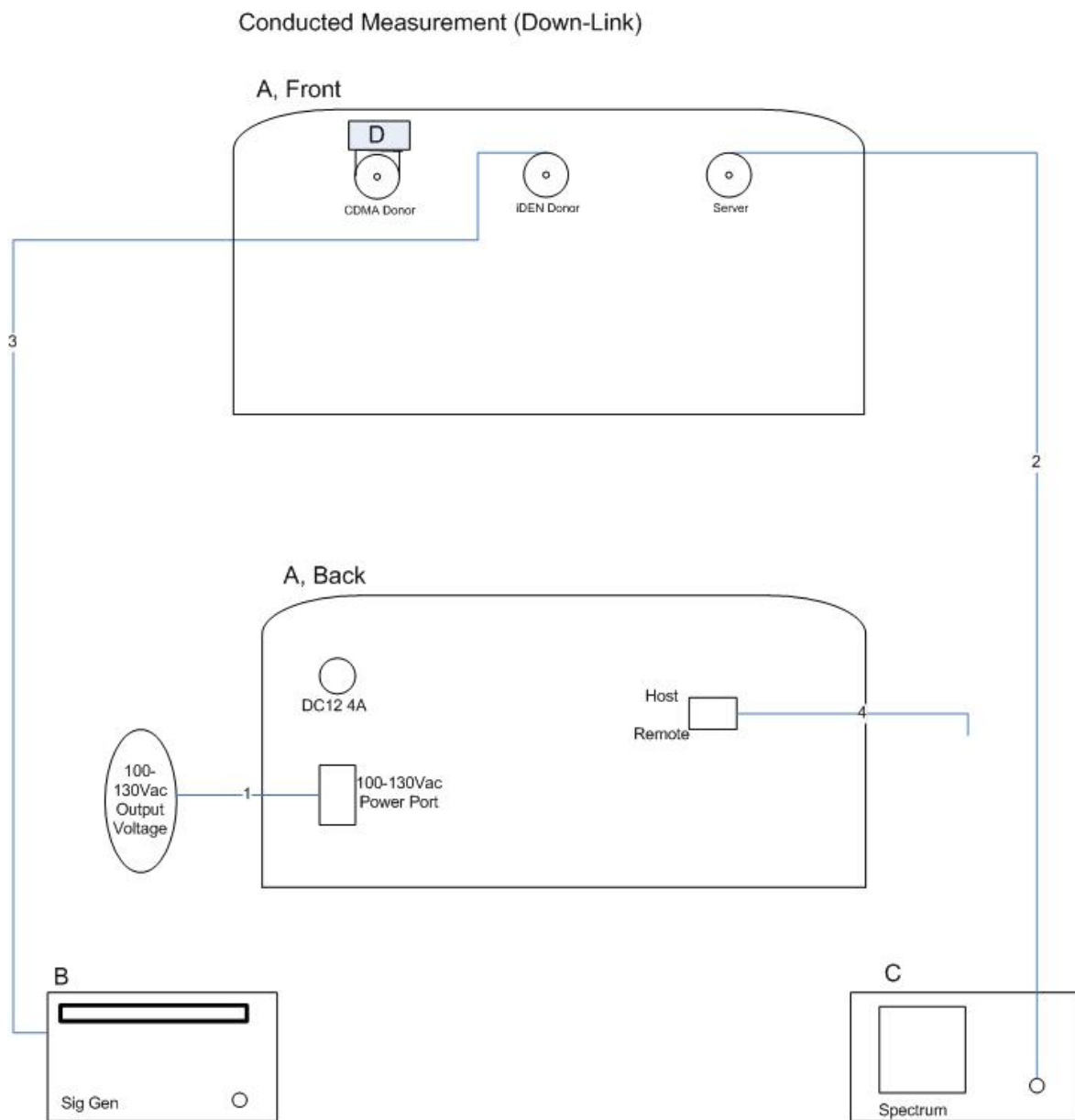
Figure 2. Block Diagram of Test Configuration (Conducted Measurement – Downlink)
