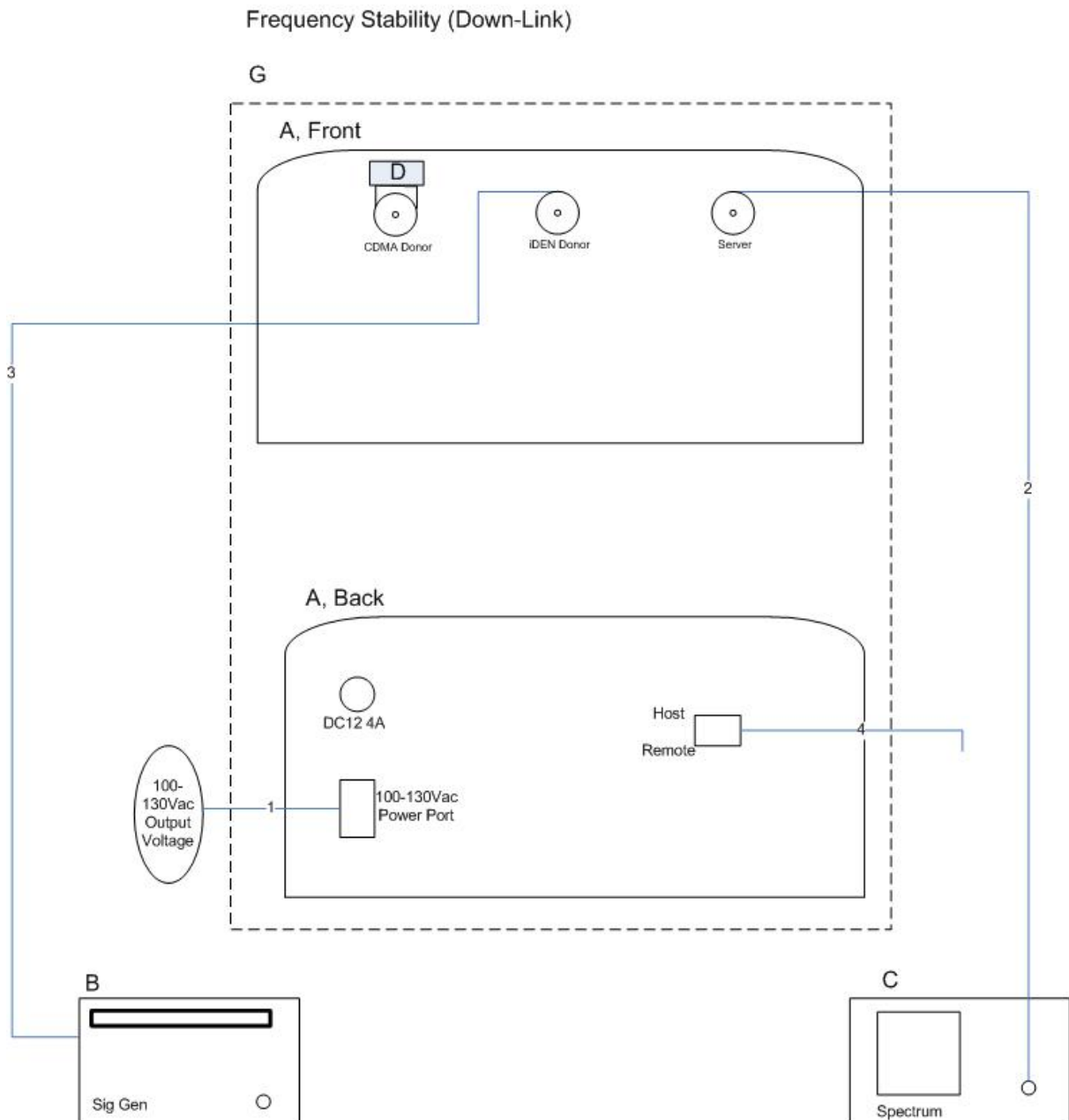
Figure 6. Block Diagram of Test Configuration (Frequency Stability)
