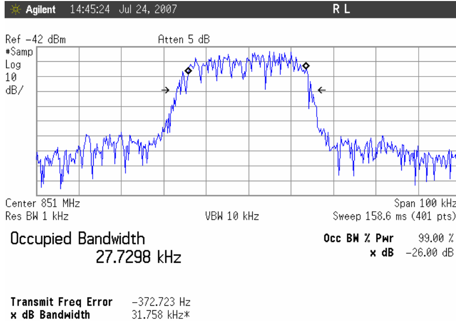
Occupied Bandwidth, TDMA Downlink, Low Channel Input
