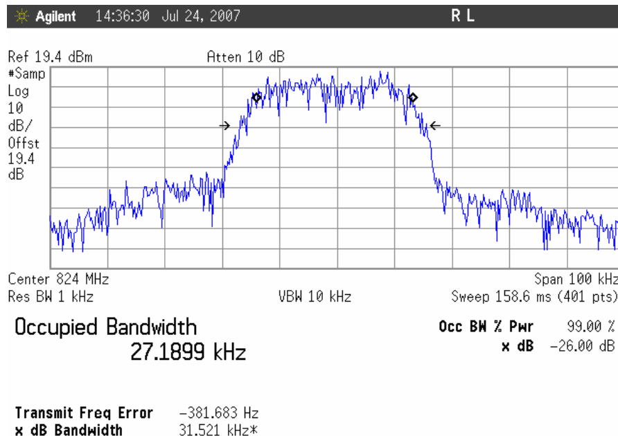
Occupied Bandwidth, TDMA Uplink, High Channel Output
