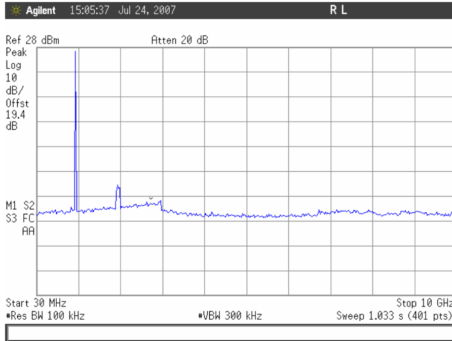
Conducted Spurious Emissions, TDMA High Channel Downlink
