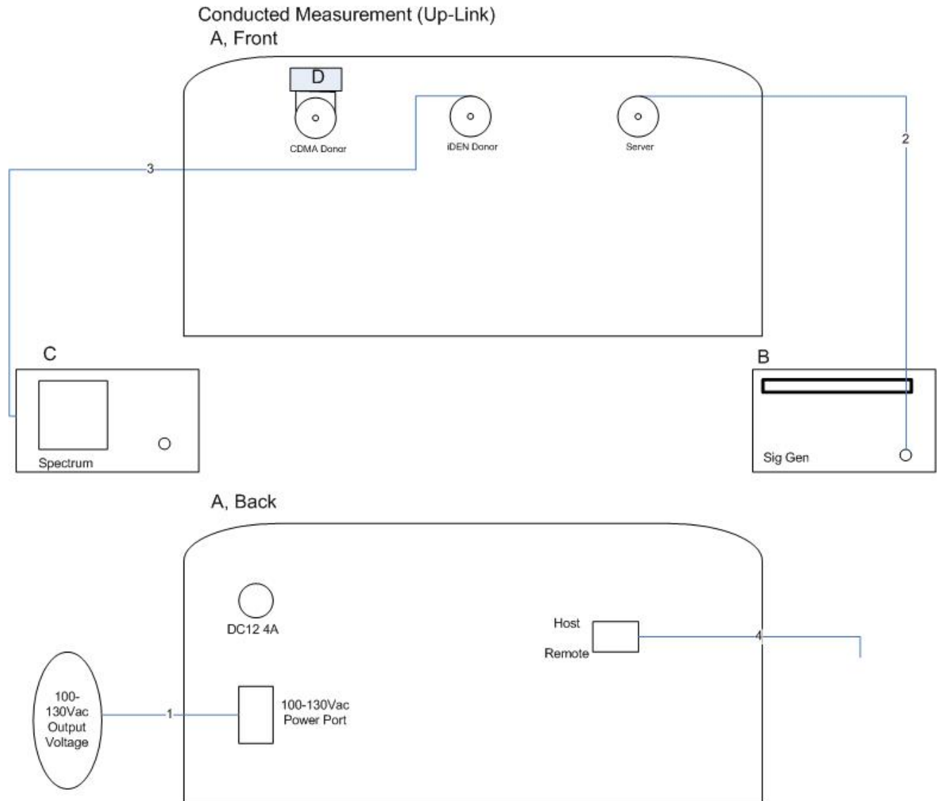
Figure 3. Block Diagram of Test Configuration (Conducted Measurement – Uplink)
