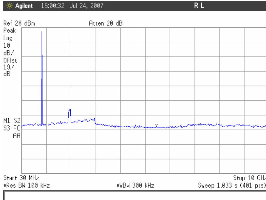
Conducted Spurious Emissions, GSM Low Channel Downlink, 30MHz – 10GHz
