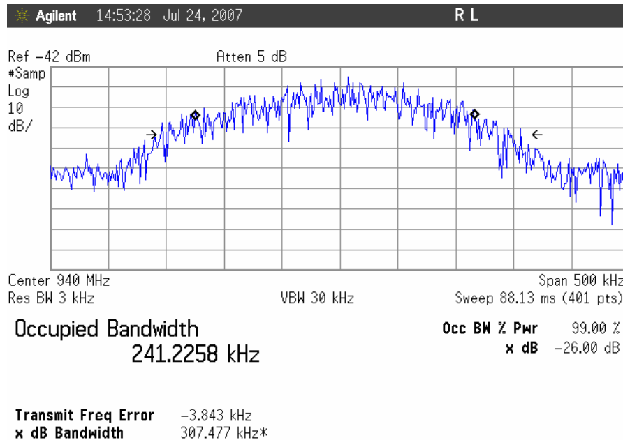
Occupied Bandwidth, GSM Downlink, High Channel Input
