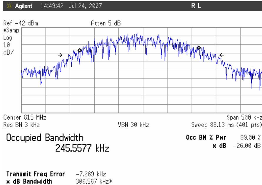
Occupied Bandwidth, GSM Uplink, Mid Channel Input
