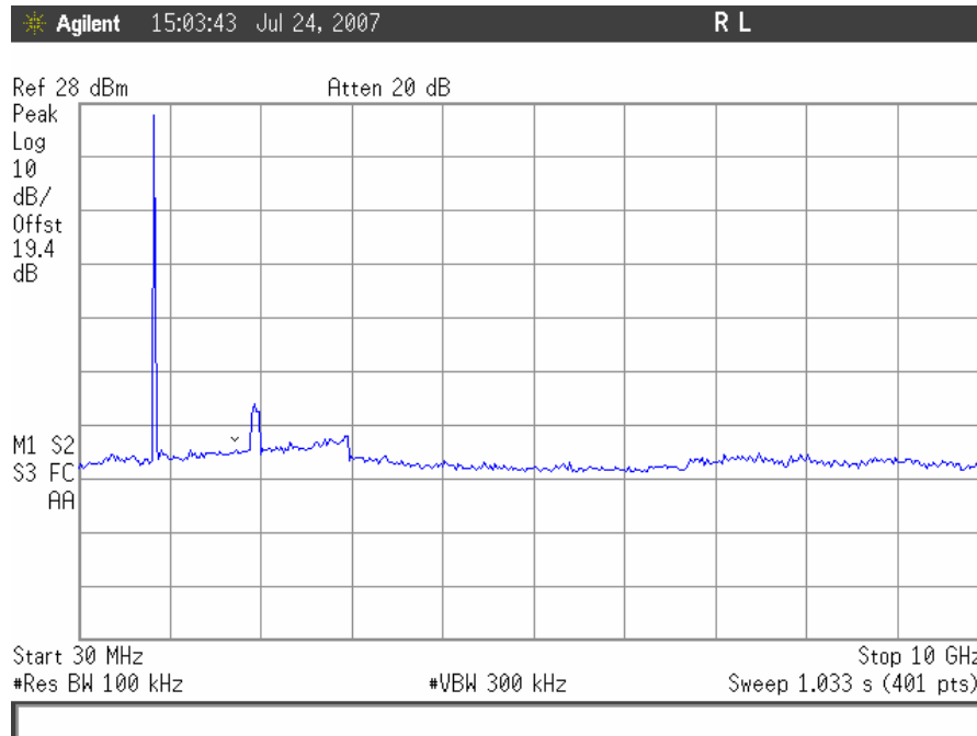
Conducted Spurious Emissions, TDMA Mid Channel Downlink
