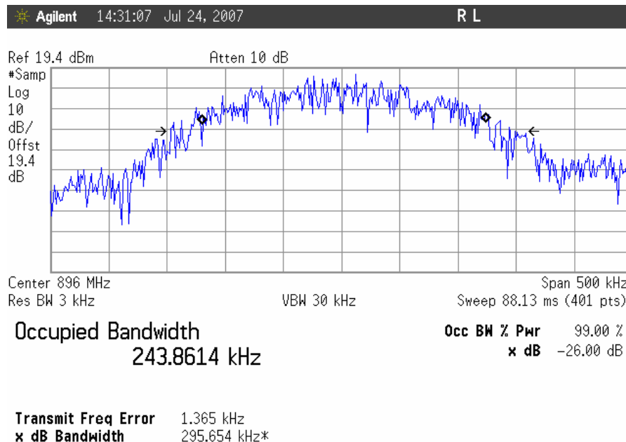
Occupied Bandwidth, GSM Uplink, Low Channel Output
