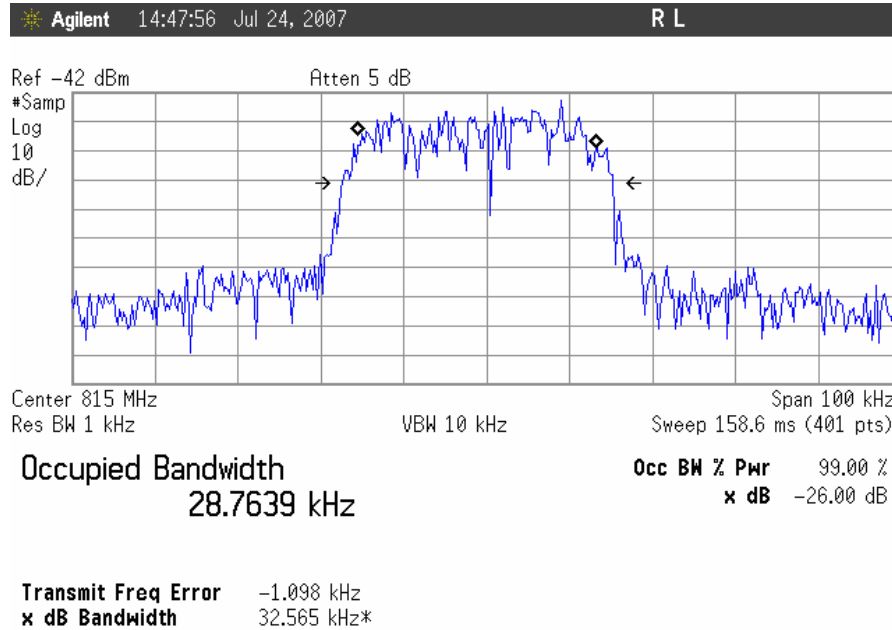
Occupied Bandwidth, TDMA Uplink, Mid Channel Input
