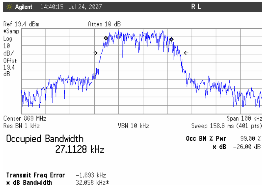
Occupied Bandwidth, TDMA Downlink, High Channel Output
