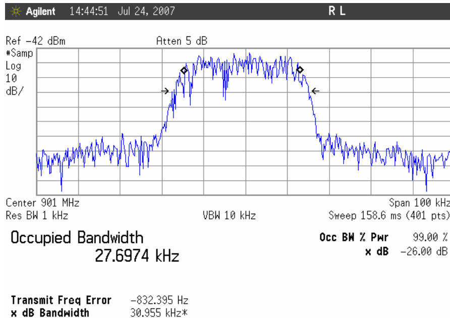
Occupied Bandwidth, TDMA Uplink, High Channel Input
