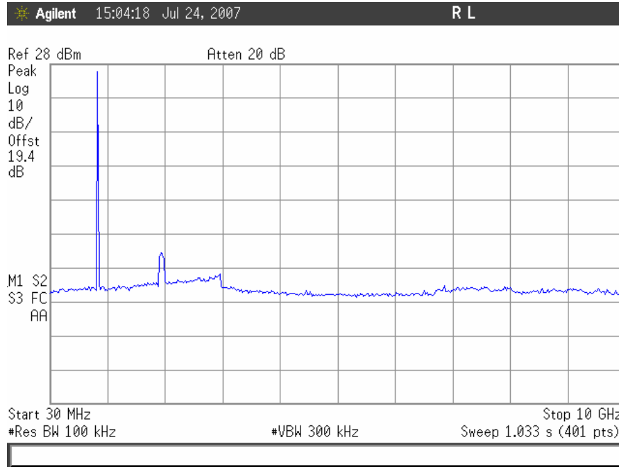
Conducted Spurious Emissions, TDMA Low Channel Downlink
