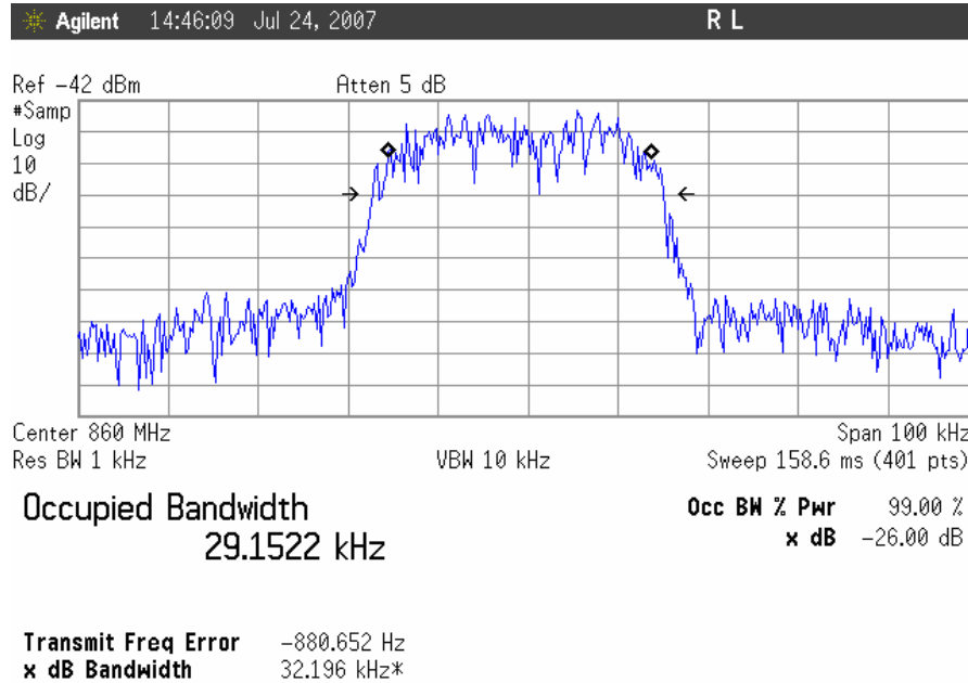
Occupied Bandwidth, TDMA Downlink, Mid Channel Input
