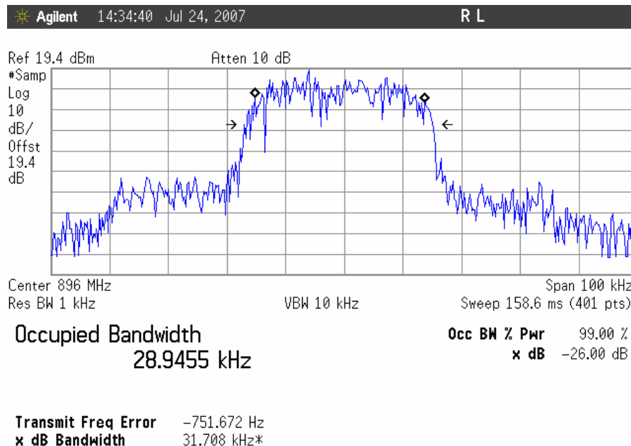
Occupied Bandwidth, TDMA Uplink, Low Channel Output
