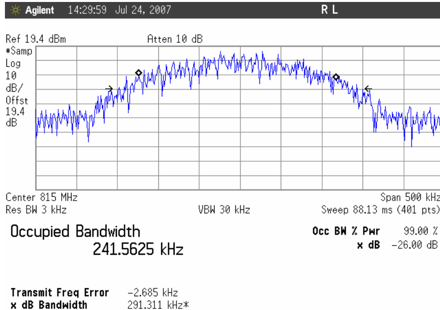
Occupied Bandwidth, GSM Uplink, Mid Channel Output
