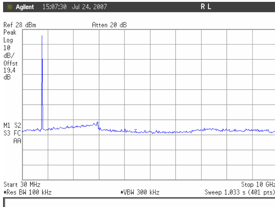
Conducted Spurious Emissions, TDMA Low Channel Uplink
