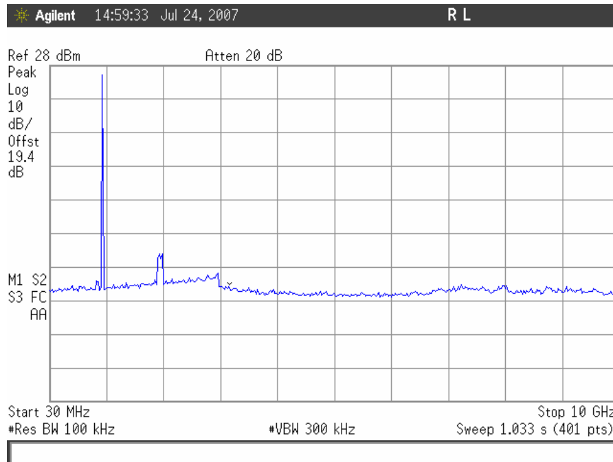
Conducted Spurious Emissions, GSM High Channel Downlink, 30MHz – 10GHz
