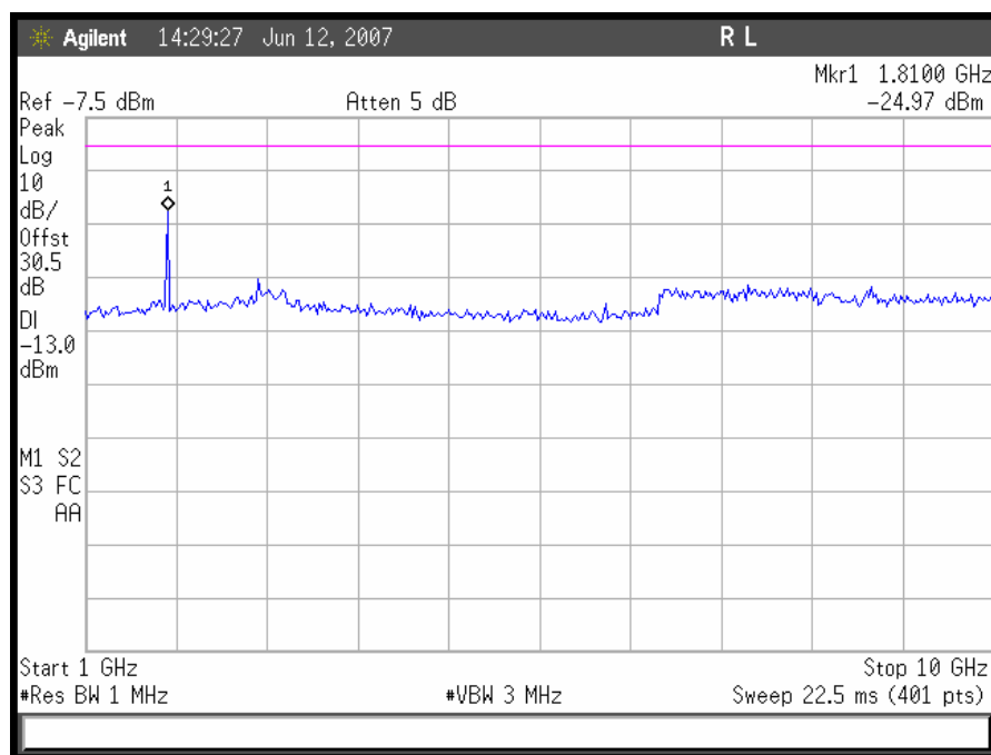
Conducted Spurious Emissions, GSM High Channel Uplink, 1GHz – 10GHz
