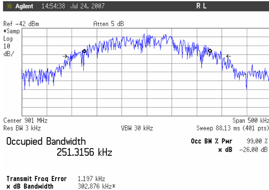
Occupied Bandwidth, GSM Uplink, High Channel Input
