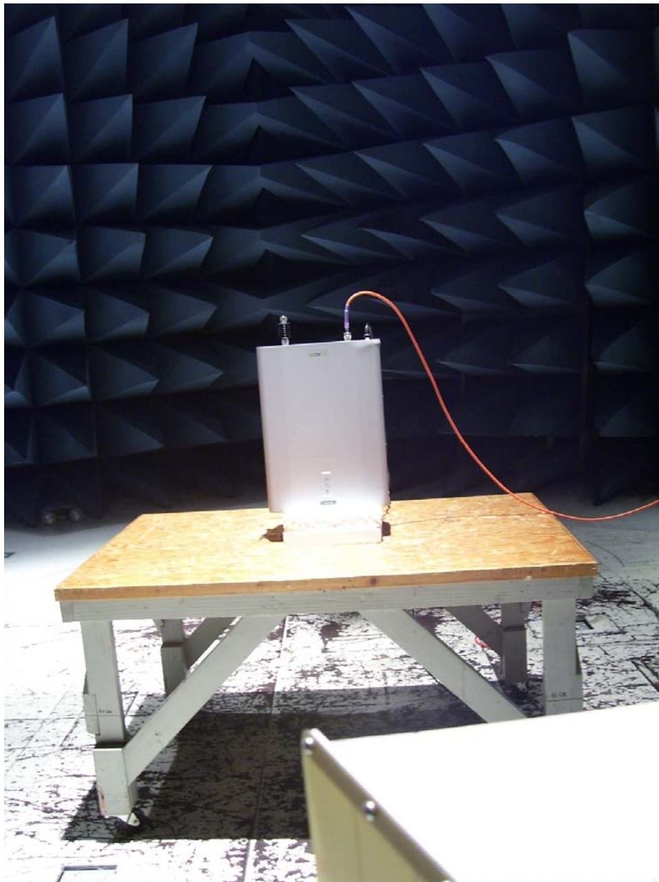
Photograph Test Equipment and setup for various Radiated Measurements
