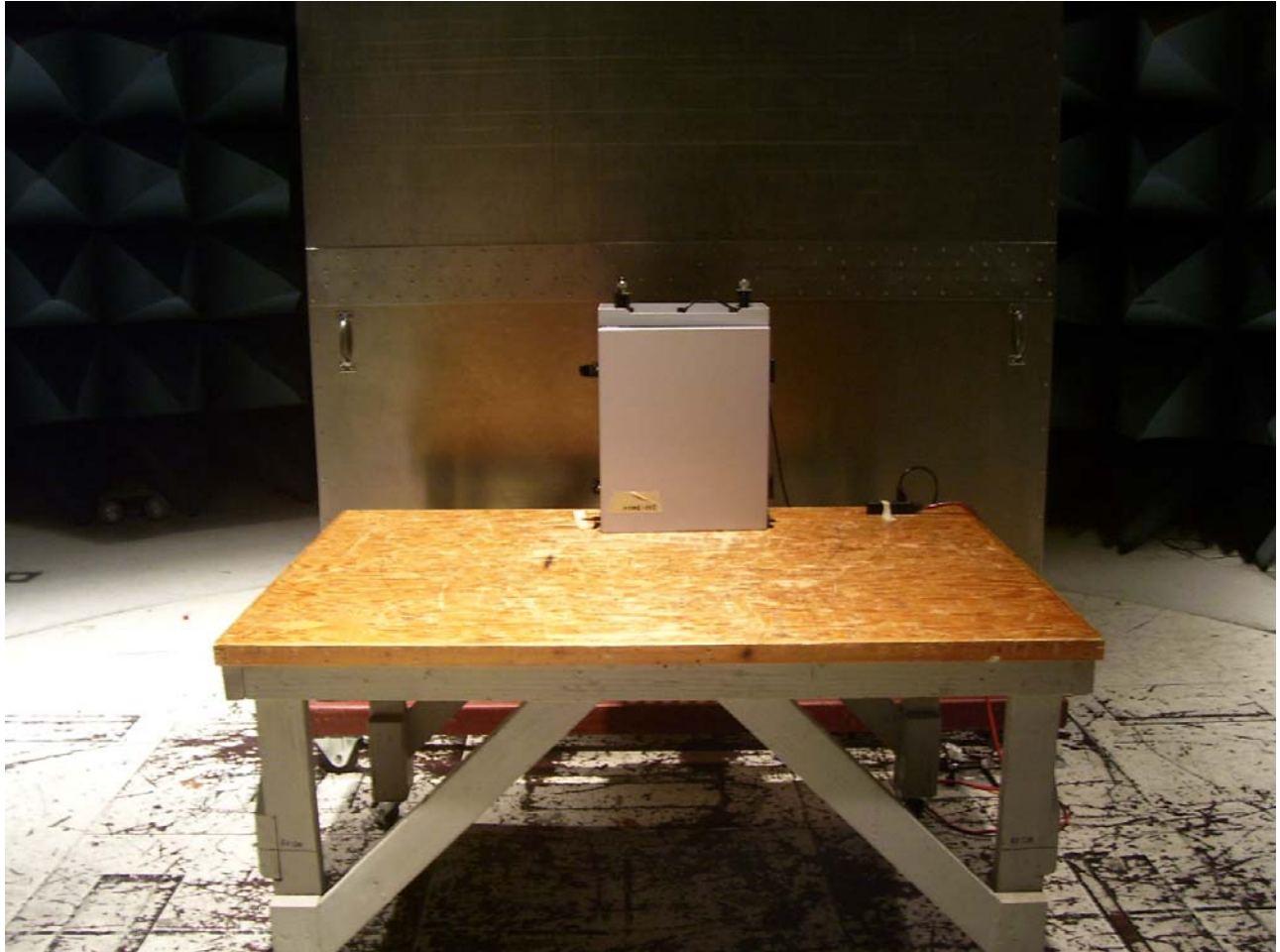
Photograph Conducted Emissions Test Setup
