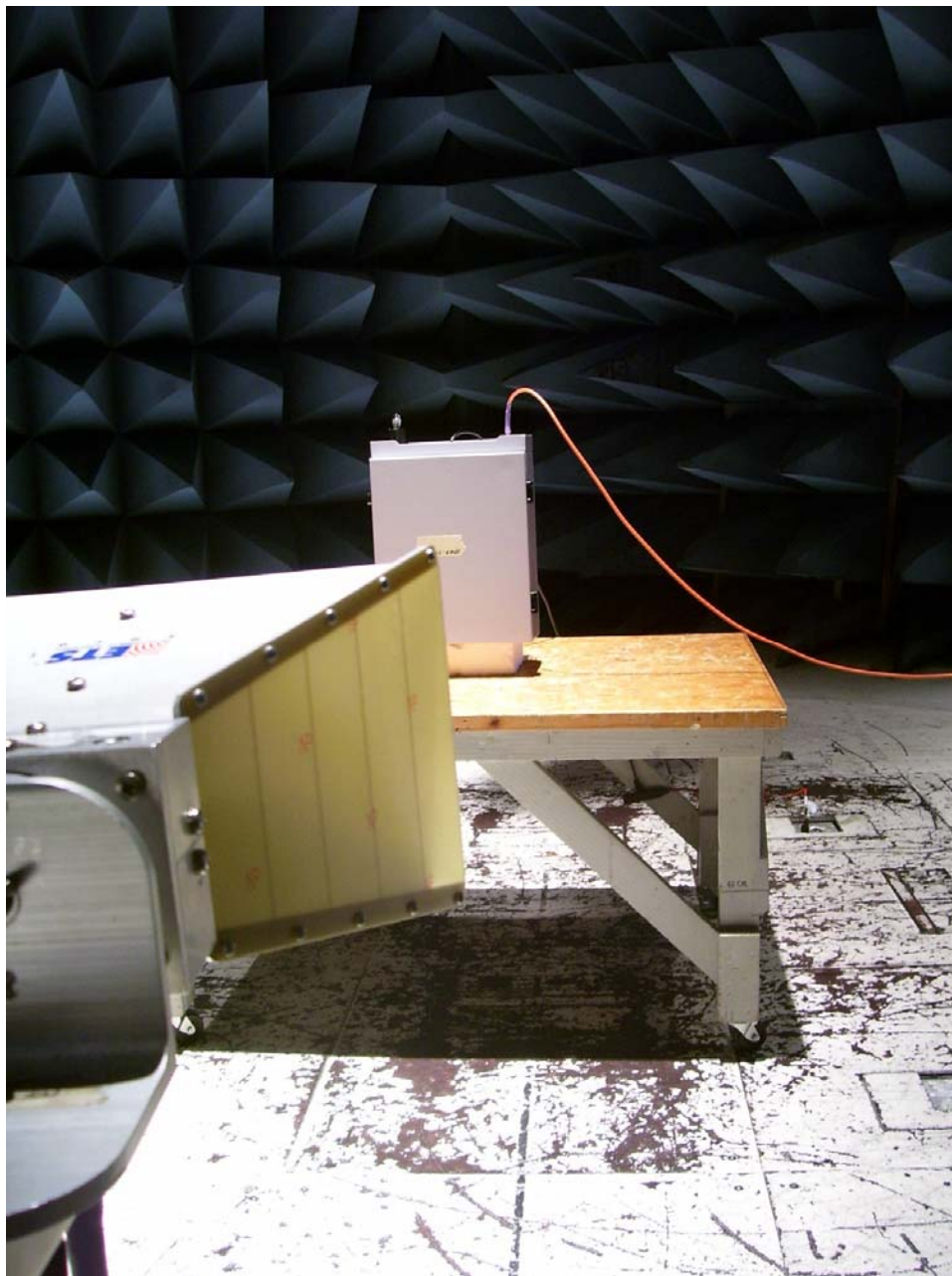
Radiated Spurious Emissions, Test Setup (Uplink)
