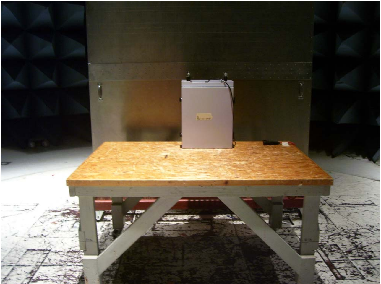
Conducted Emissions Test Setup Photograph
