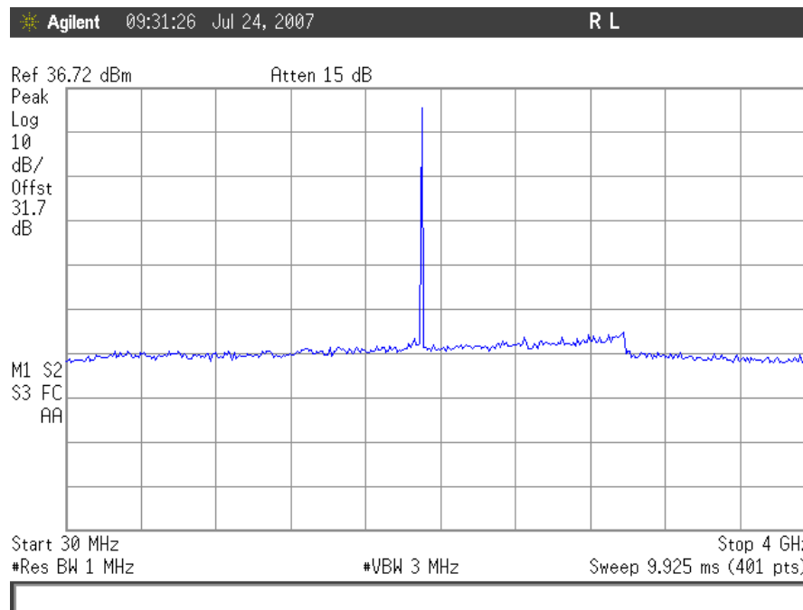
Plot 66. Conducted Spurious Emissions, GSM High Channel 30MHz – 4GHz, Uplink
