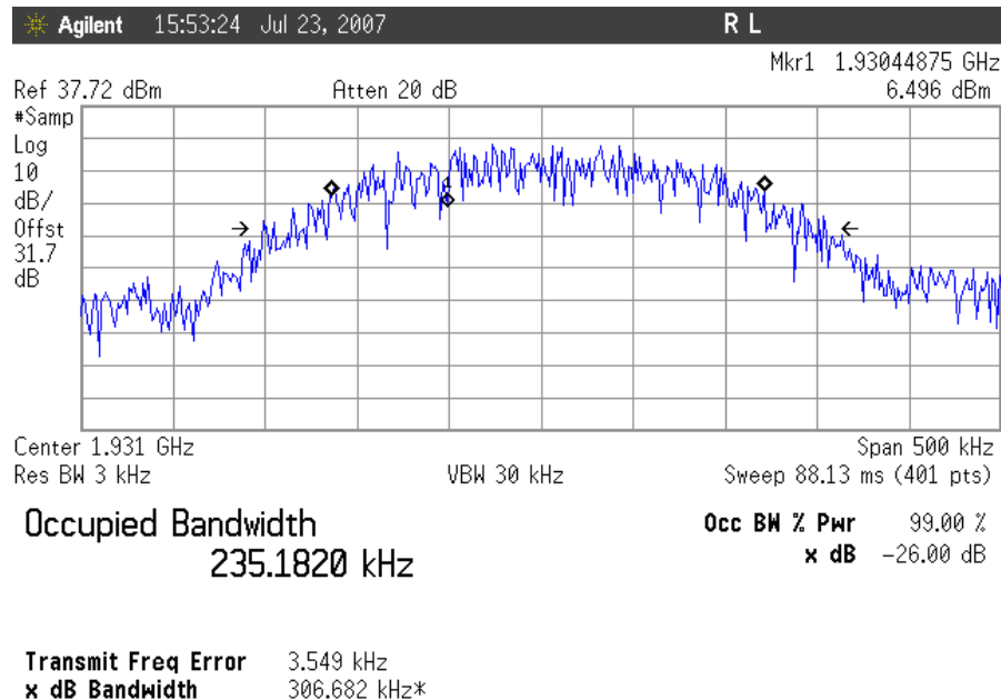
Plot 17. Occupied Bandwidth, GSM Downlink, Low Channel Output
