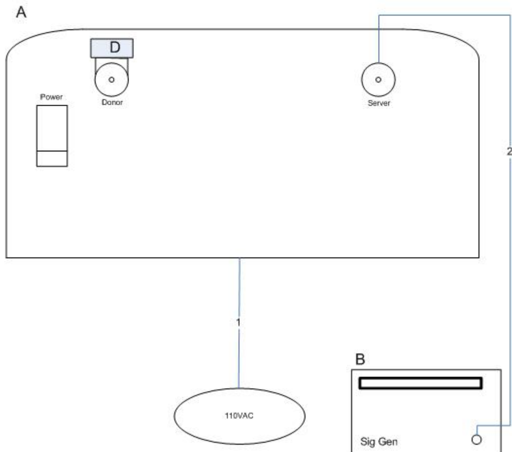
Figure 2. Block Diagram of Test Configuration (Spurious Emissions – Uplink)
