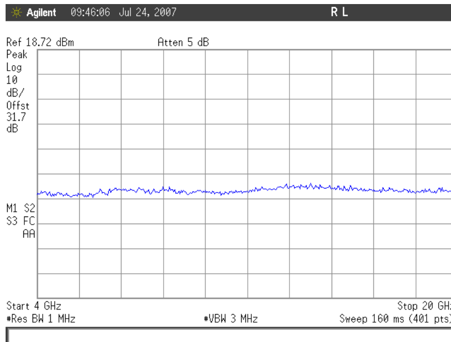
Plot 75. Conducted Spurious Emissions, TDMA Mid Channel 4GHz – 20GHz, Downlink
