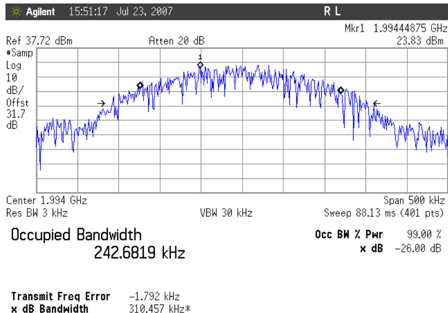
Plot 21. Occupied Bandwidth, GSM Downlink, High Channel Output
