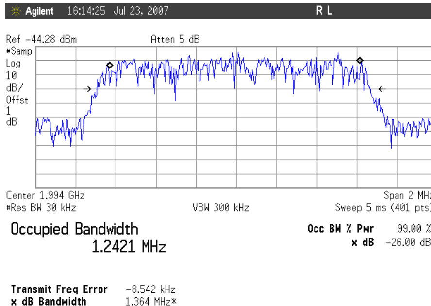
Plot 8. Occupied Bandwidth, CDMA Downlink, High Channel Input
