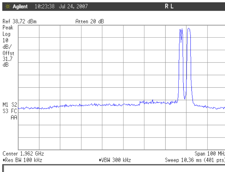
Plot 53. CDMA Intermodulation, Downlink High End
