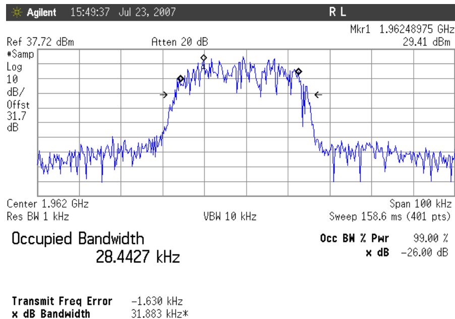
Plot 31. Occupied Bandwidth, TDMA Downlink, Mid Channel Output
