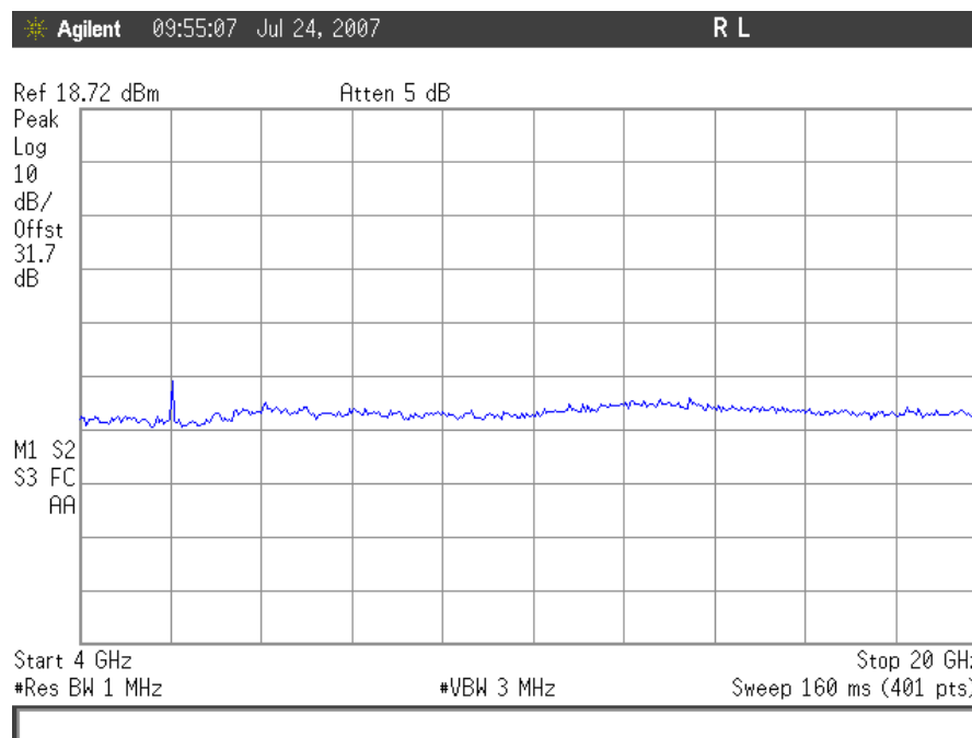
Plot 49. Conducted Spurious Emissions, CDMA Mid Channel 4GHz – 20GHz, Uplink
