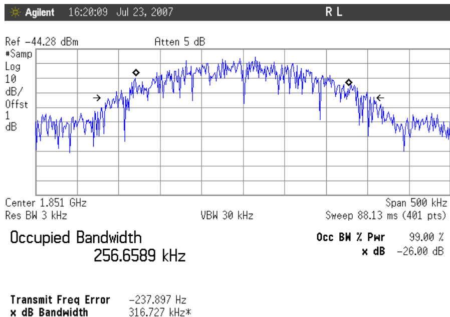
Plot 22. Occupied Bandwidth, GSM Uplink, Low Channel Input
