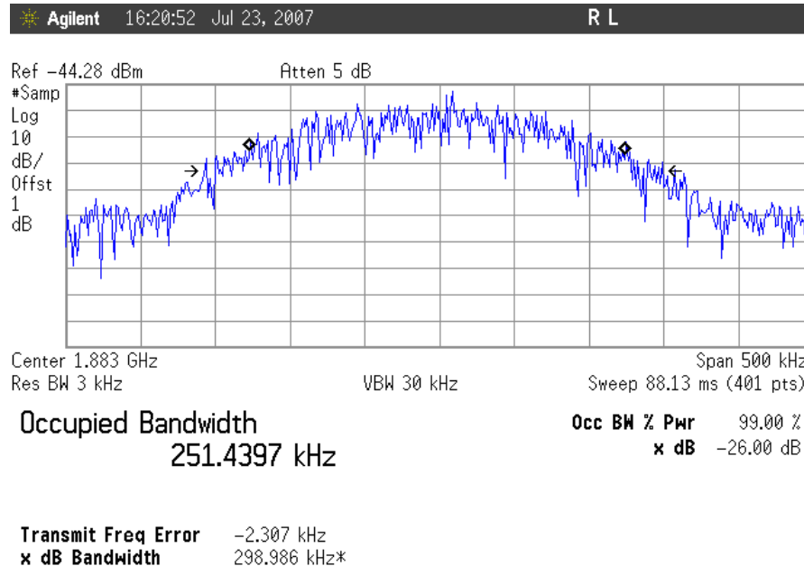
Plot 24. Occupied Bandwidth, GSM Uplink, Mid Channel Input
