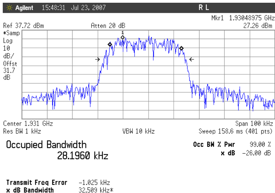
Plot 29. Occupied Bandwidth, TDMA Downlink, Low Channel Output
