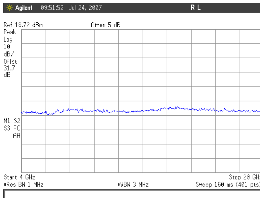
Plot 43. Conducted Spurious Emissions, CDMA Mid Channel 4GHz – 20GHz, Downlink
