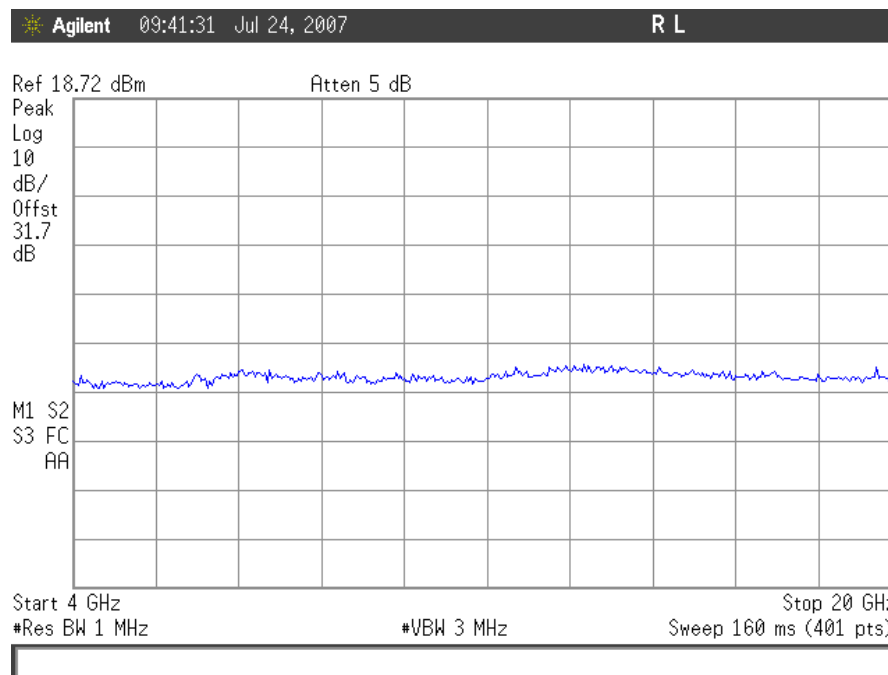
Plot 65. Conducted Spurious Emissions, GSM Mid Channel 4GHz – 20GHz, Uplink
