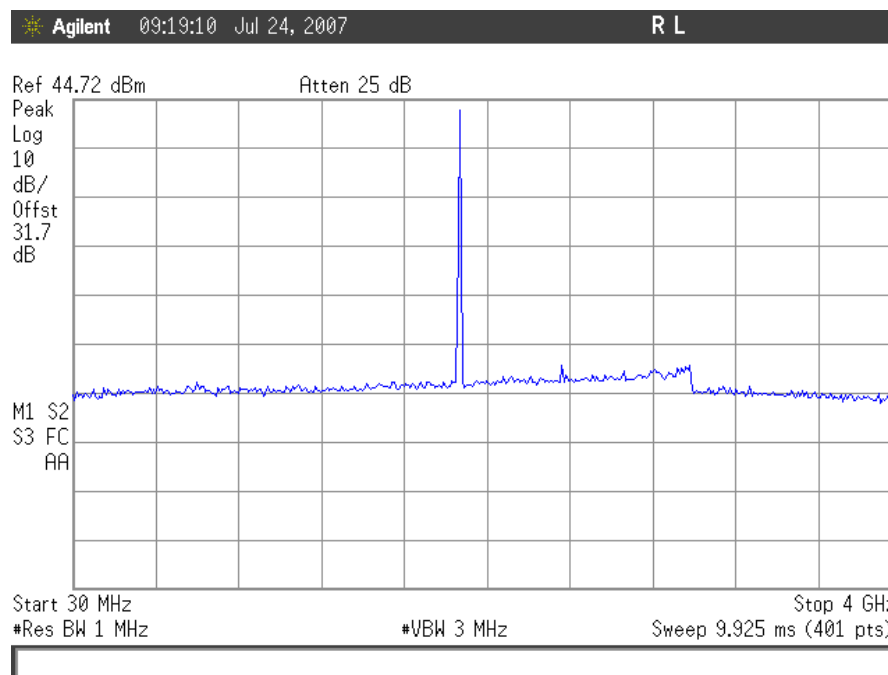
Plot 48. Conducted Spurious Emissions, CDMA Mid Channel 30MHz – 4GHz, Uplink
