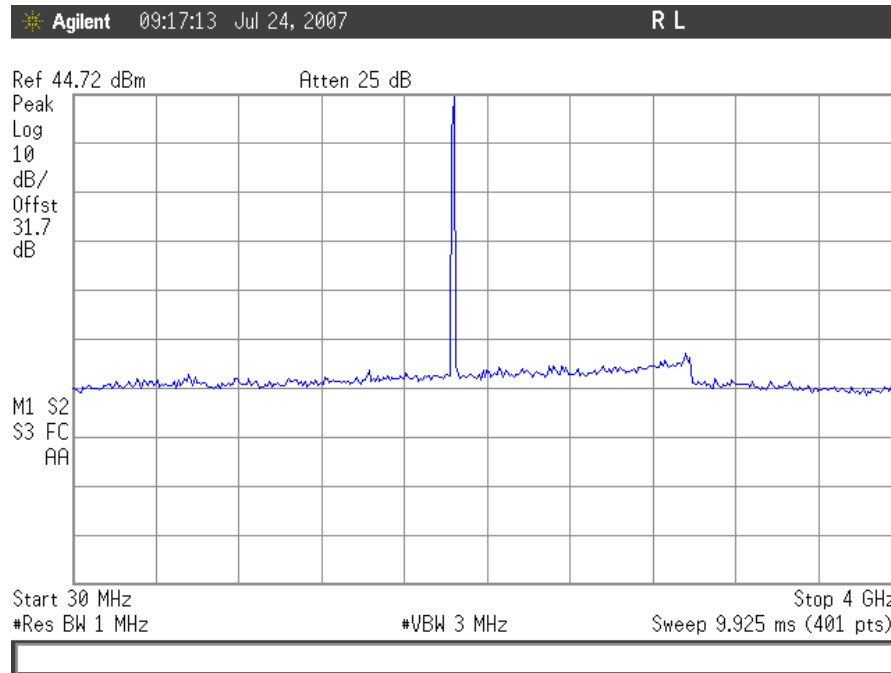
Plot 46. Conducted Spurious Emissions, CDMA Low Channel 30MHz – 4GHz, Uplink
