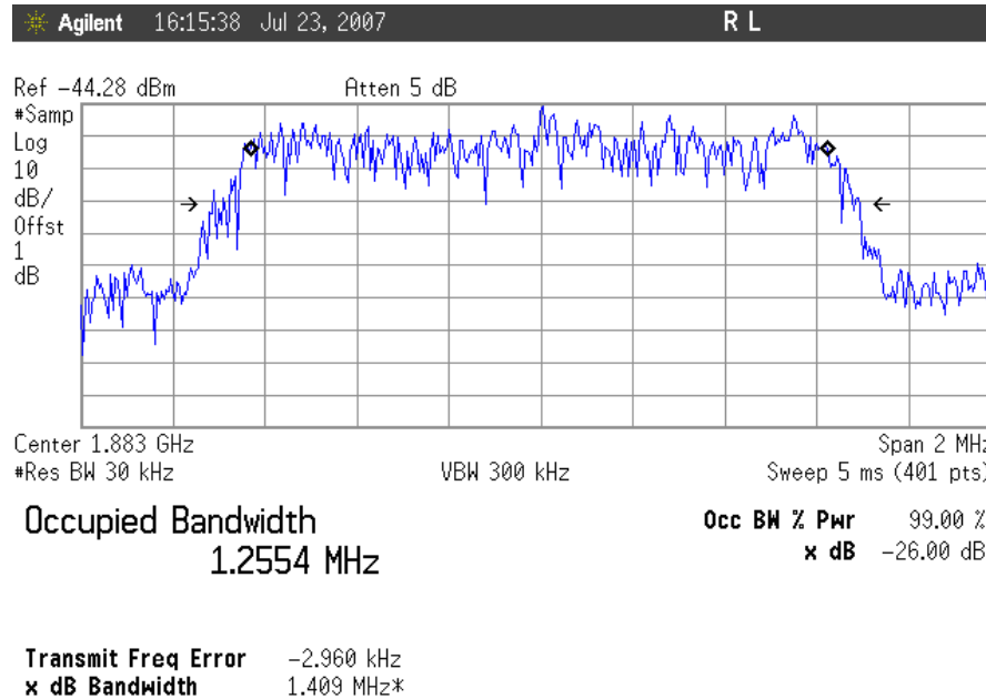
Plot 12. Occupied Bandwidth, CDMA Uplink, Mid Channel Input
