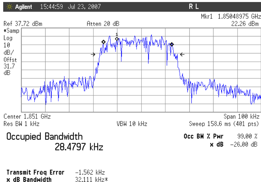
Plot 35. Occupied Bandwidth, TDMA Uplink, Low Channel Output
