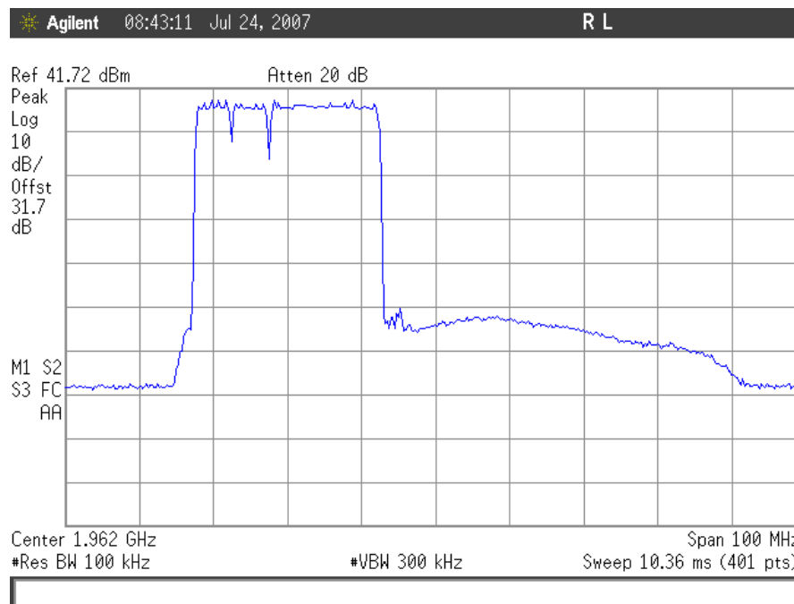
Plot 88. Out of Band Rejection, Downlink Low End
