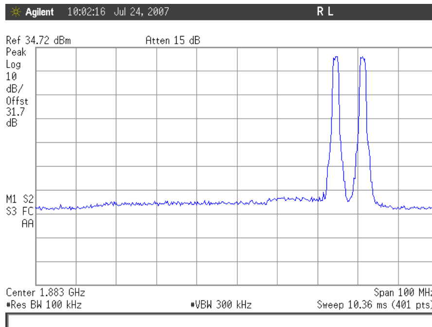
Plot 55. CDMA Intermodulation, Uplink High End
