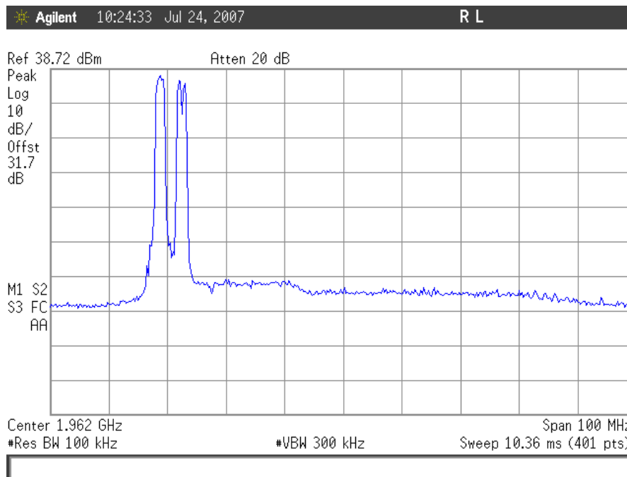
Plot 52. CDMA Intermodulation, Downlink Low End
