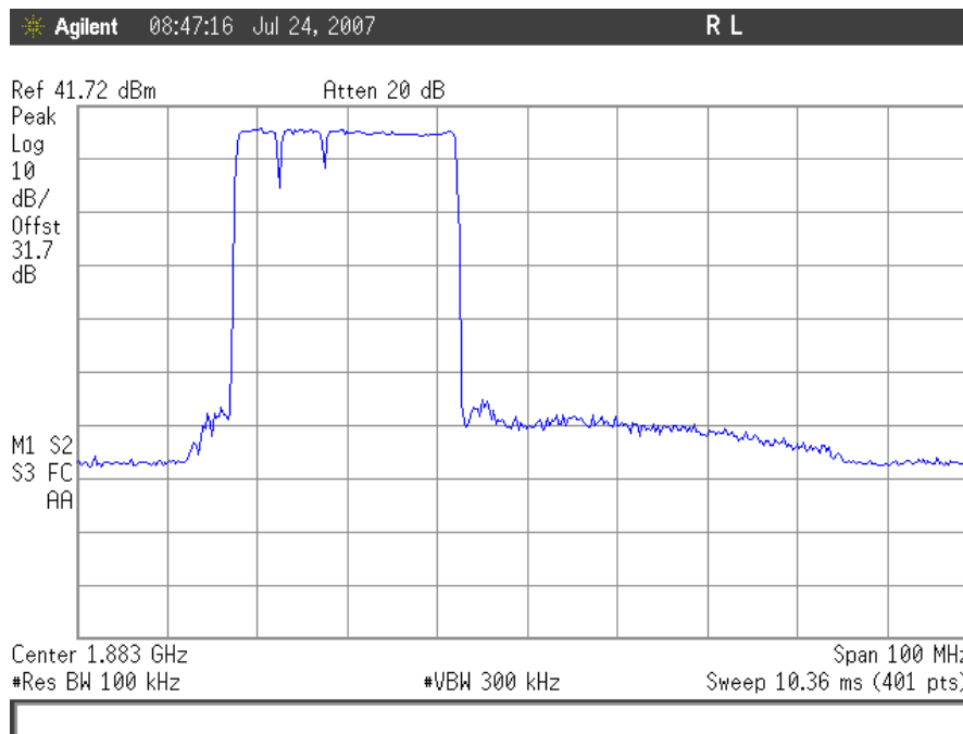
Plot 90. Out of Band Rejection, Uplink Low End, 15MHz
