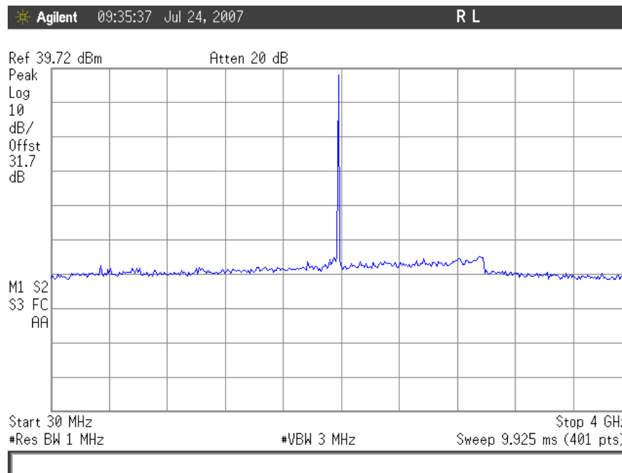
Plot 60. Conducted Spurious Emissions, GSM High Channel 30MHz – 4GHz, Downlink
