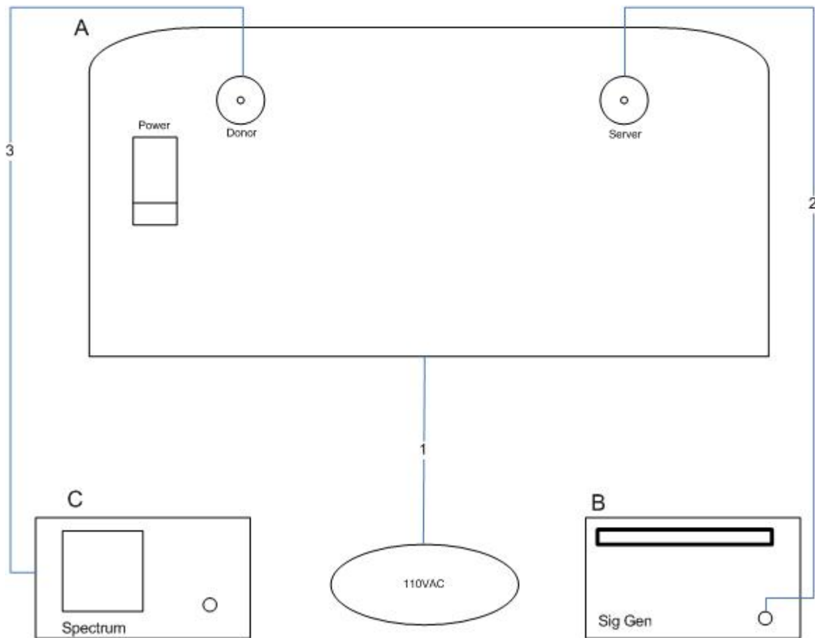
Figure 4. Block Diagram of Test Configuration (Conducted Measurement – Uplink)
