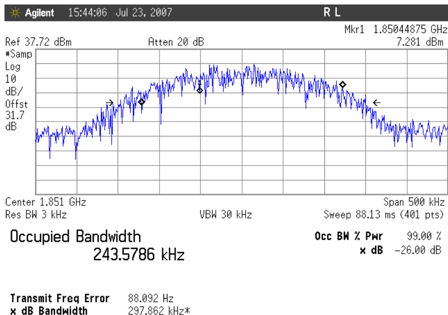
Plot 23. Occupied Bandwidth, GSM Uplink, Low Channel Output
