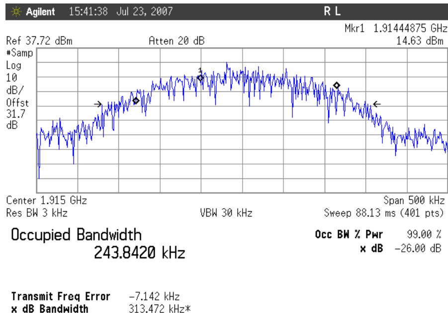
Plot 27. Occupied Bandwidth, GSM Uplink, High Channel Output
