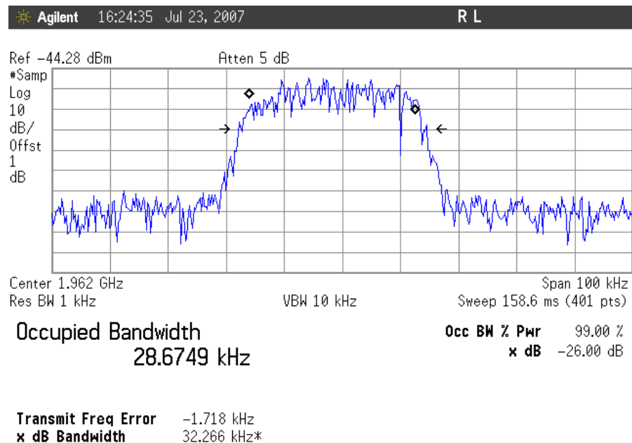
Plot 30. Occupied Bandwidth, TDMA Downlink, Mid Channel Input
