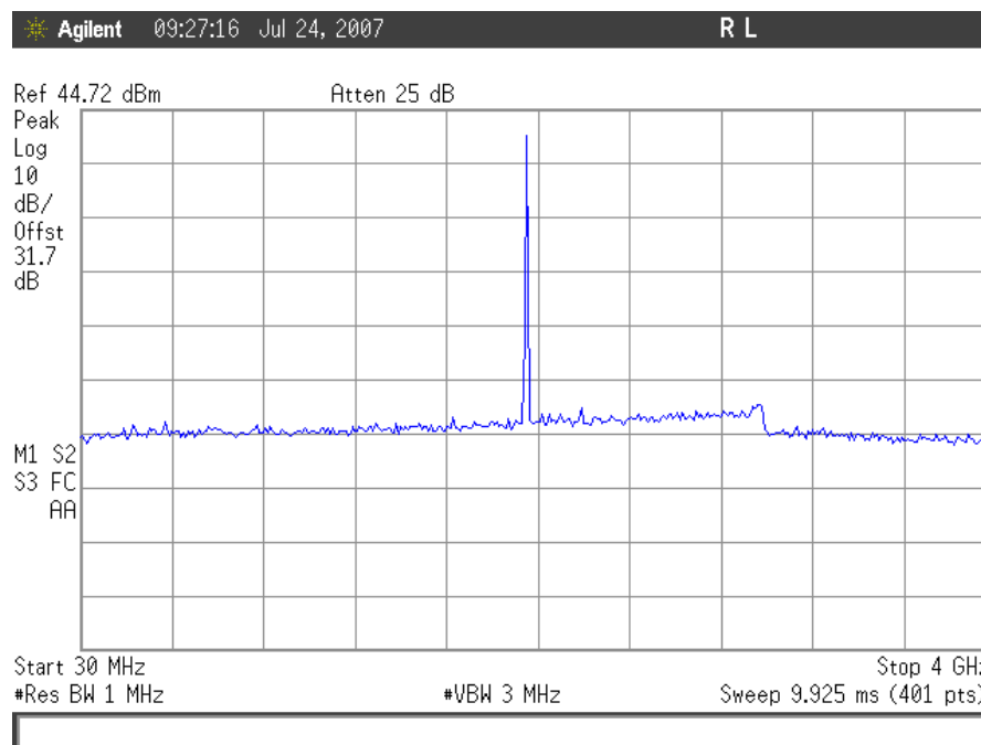
Plot 74. Conducted Spurious Emissions, TDMA Mid Channel 30MHz – 4GHz, Downlink
