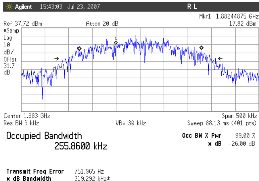
Plot 25. Occupied Bandwidth, GSM Uplink, Mid Channel Output
