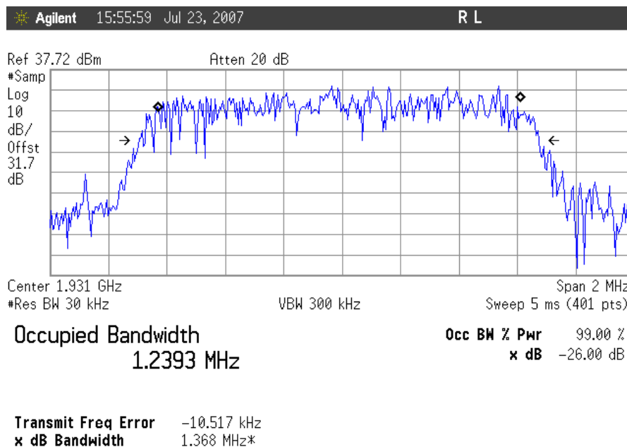
Plot 5. Occupied Bandwidth, CDMA Downlink, Low Channel Output
