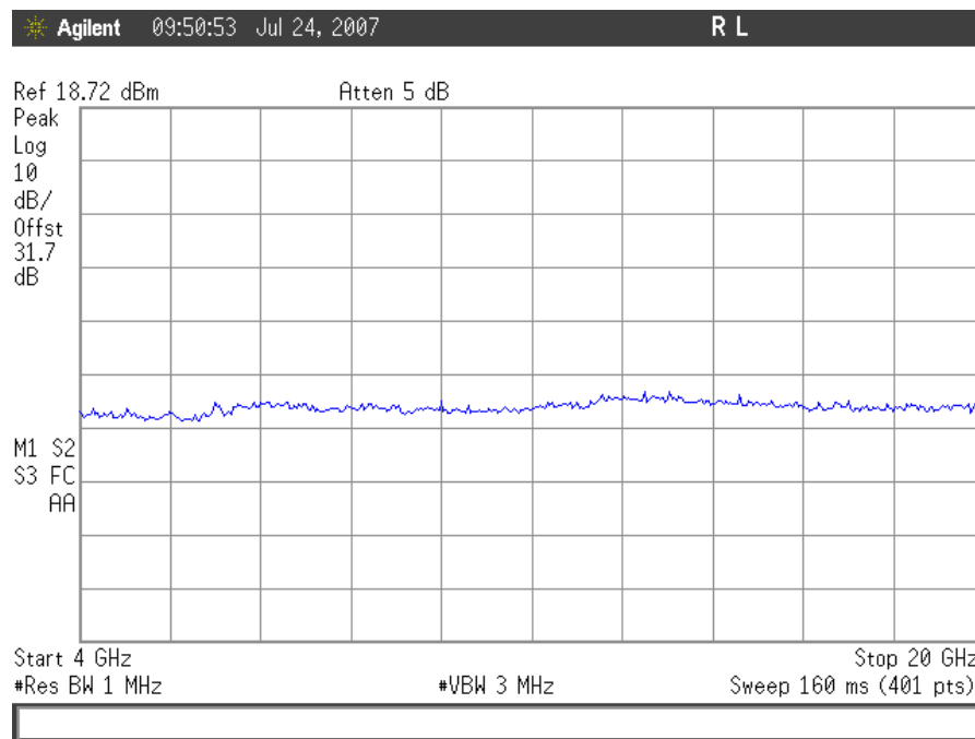
Plot 45. Conducted Spurious Emissions, CDMA High Channel 4GHz – 20GHz, Downlink
