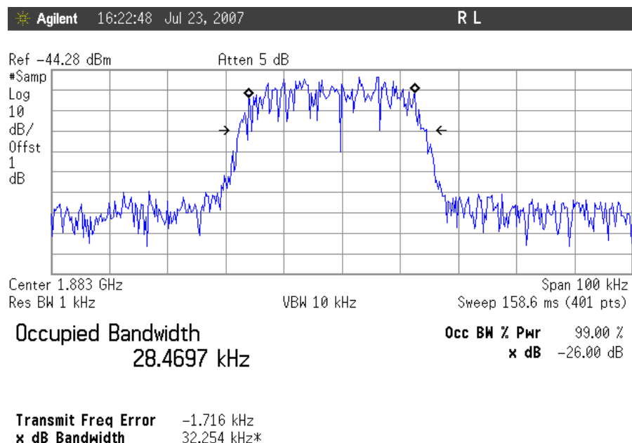
Plot 36. Occupied Bandwidth, TDMA Uplink, Mid Channel Input
