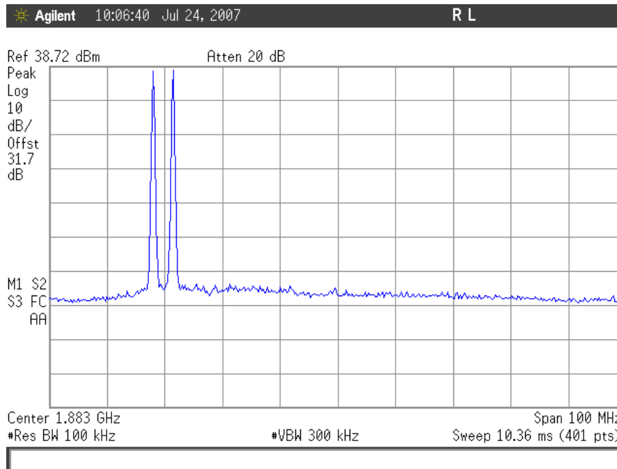
Plot 86. TDMA Intermodulation, Uplink Low End
