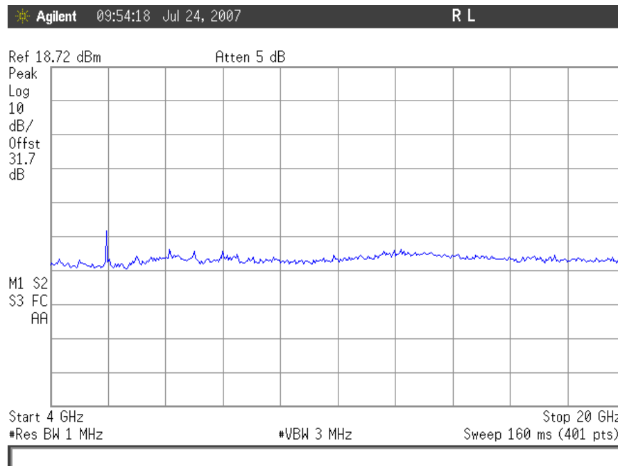
Plot 47. Conducted Spurious Emissions, CDMA Low Channel 4GHz – 20GHz, Uplink
