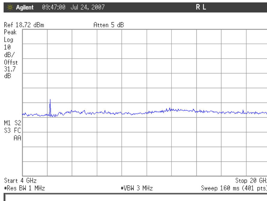
Plot 73. Conducted Spurious Emissions, TDMA Low Channel 4GHz – 20GHz, Downlink
