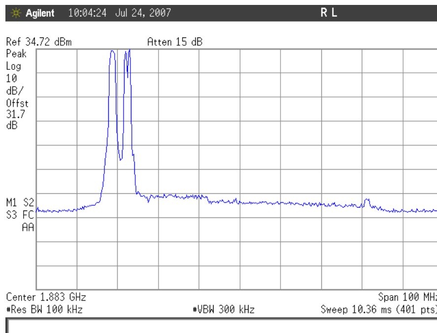
Plot 54. CDMA Intermodulation, Uplink Low End
