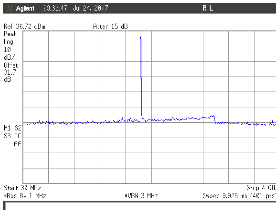
Plot 62. Conducted Spurious Emissions, GSM Low Channel 30MHz – 4GHz, Uplink
