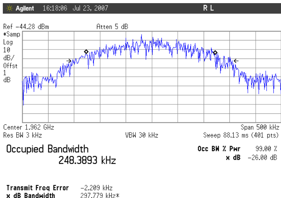
Plot 18. Occupied Bandwidth, GSM Downlink, Mid Channel Input
