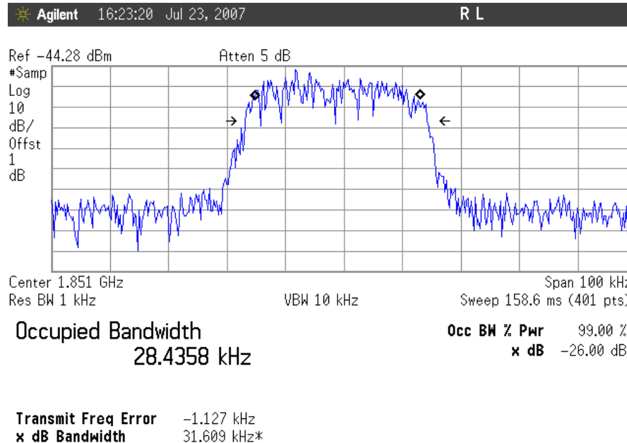
Plot 34. Occupied Bandwidth, TDMA Uplink, Low Channel Input
