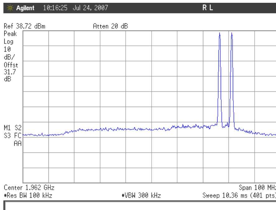
Plot 69. GSM Intermodulation, Downlink High End
