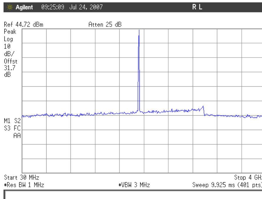
Plot 40. Conducted Spurious Emissions, CDMA Low Channel 30MHz – 4GHz, Downlink
