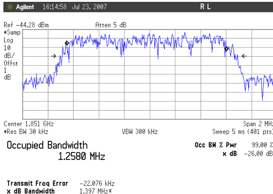
Plot 10. Occupied Bandwidth, CDMA Uplink, Low Channel Input
