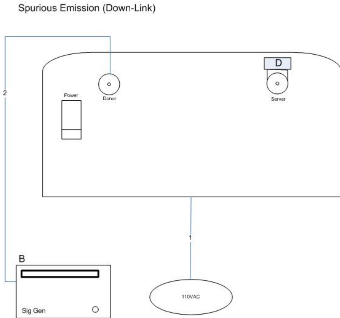
Figure 1. Block Diagram of Test Configuration (Spurious Emissions - Downlink)
