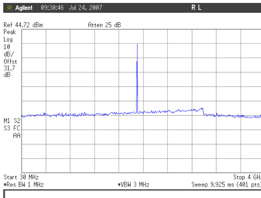
Plot 82. Conducted Spurious Emissions, TDMA High Channel 30MHz – 4GHz, Uplink
