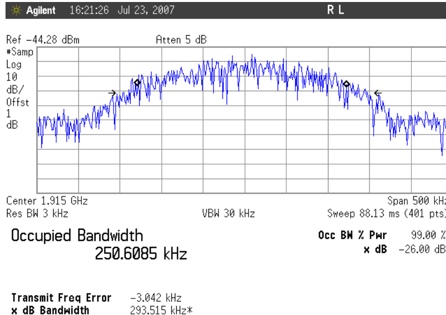
Plot 26. Occupied Bandwidth, GSM Uplink, High Channel Input
