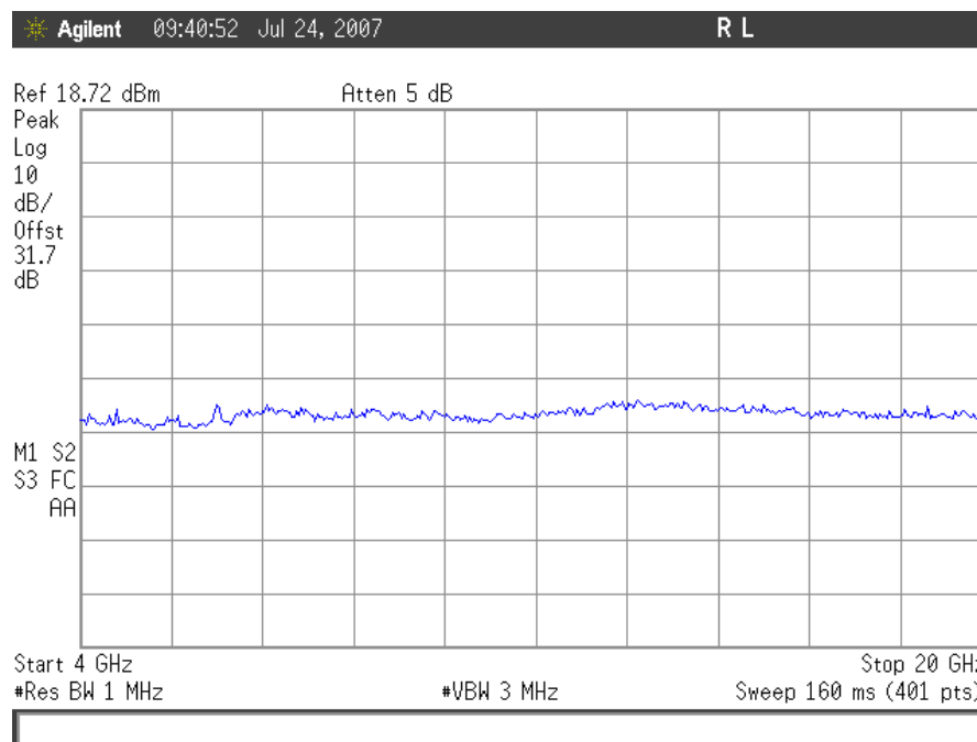
Plot 63. Conducted Spurious Emissions, GSM Low Channel 4GHz – 20GHz, Uplink
