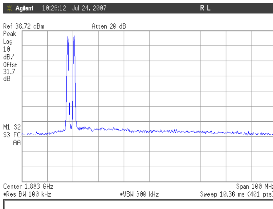
Plot 70. GSM Intermodulation, Uplink Low End
