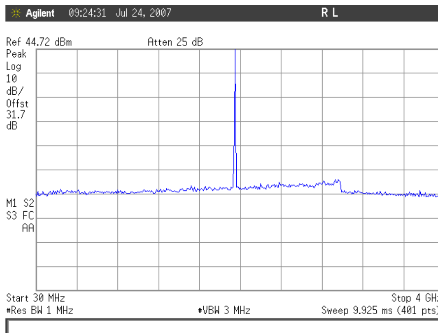
Plot 42. Conducted Spurious Emissions, CDMA Mid Channel 30MHz – 4GHz, Downlink
