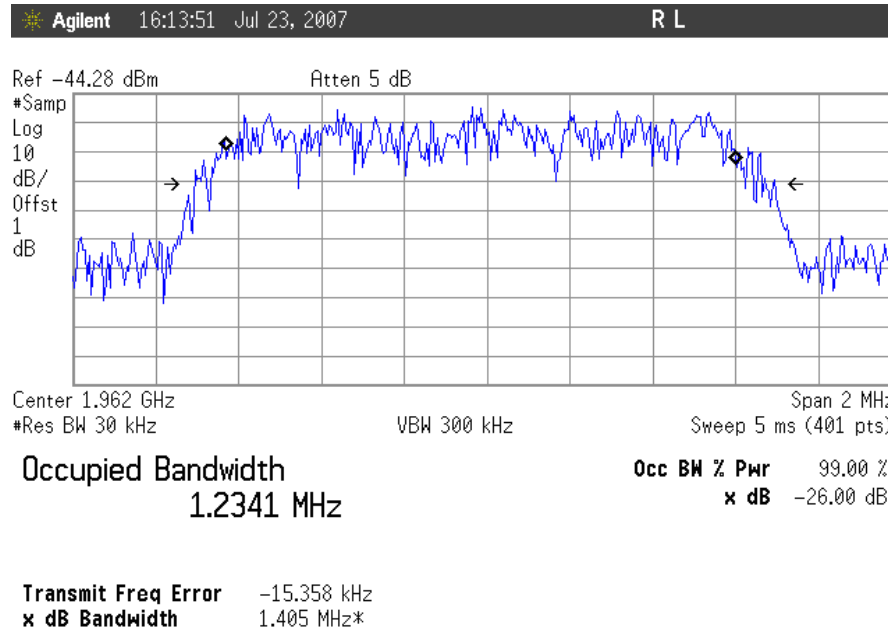
Plot 6. Occupied Bandwidth, CDMA Downlink, Mid Channel Input
