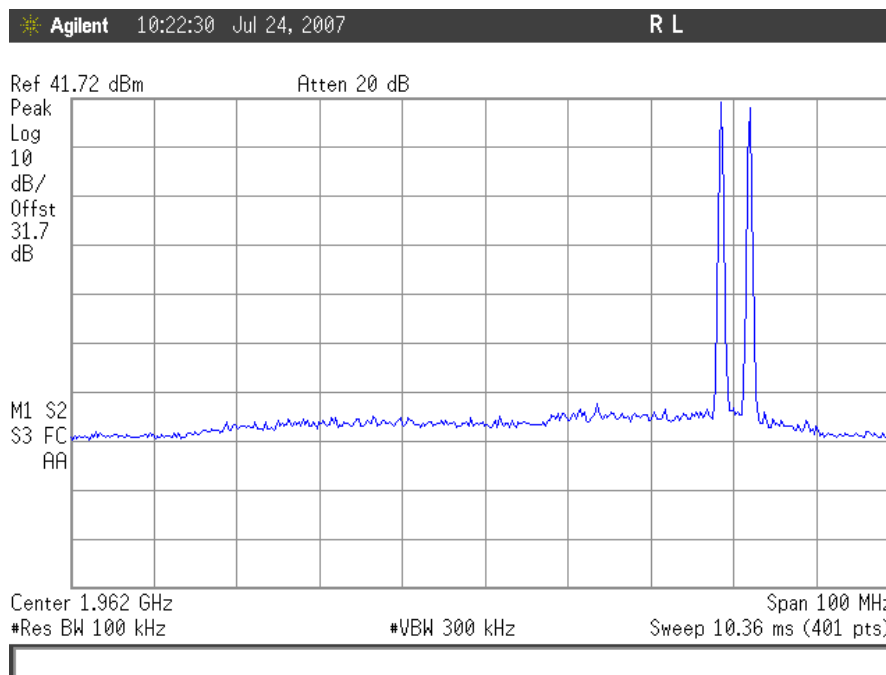
Plot 85. TDMA Intermodulation, Downlink High End
