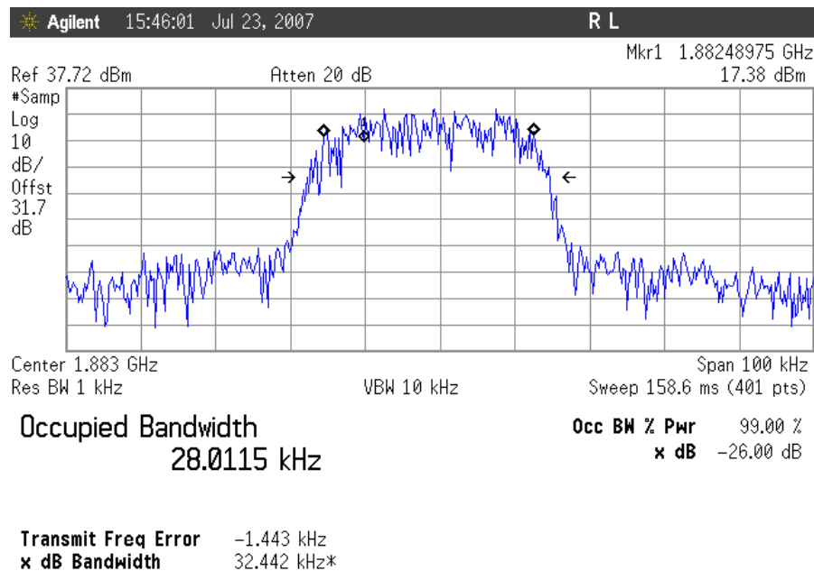
Plot 37. Occupied Bandwidth, TDMA Uplink, Mid Channel Output
