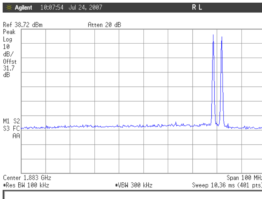
Plot 87. TDMA Intermodulation, Uplink High End
