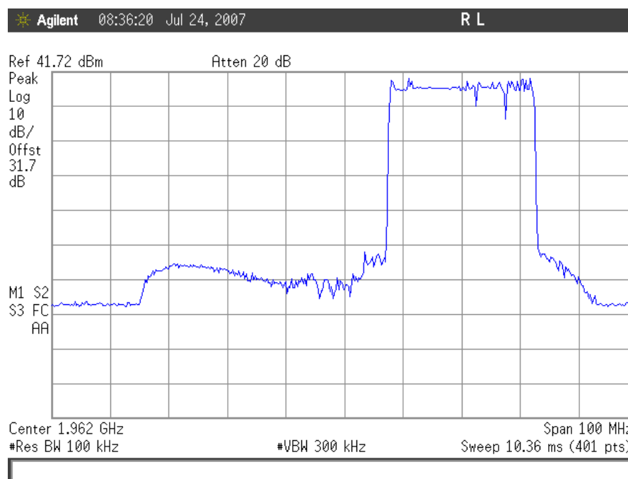
Plot 89. Out of Band Rejection, Downlink High End
