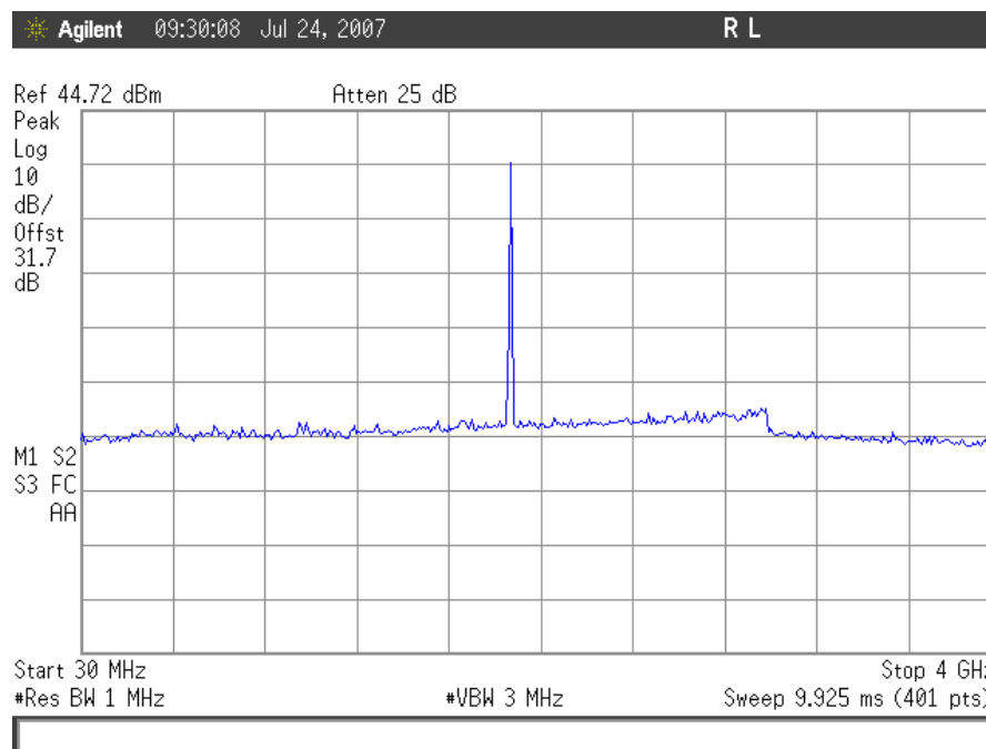
Plot 80. Conducted Spurious Emissions, TDMA Mid Channel 30MHz – 4GHz, Uplink
