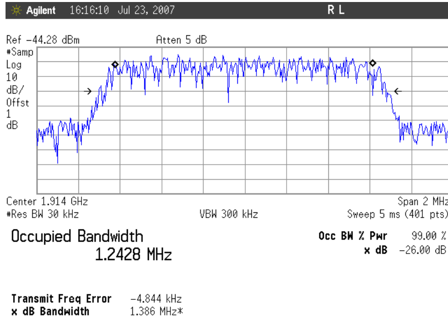
Plot 14. Occupied Bandwidth, CDMA Uplink, High Channel Input
