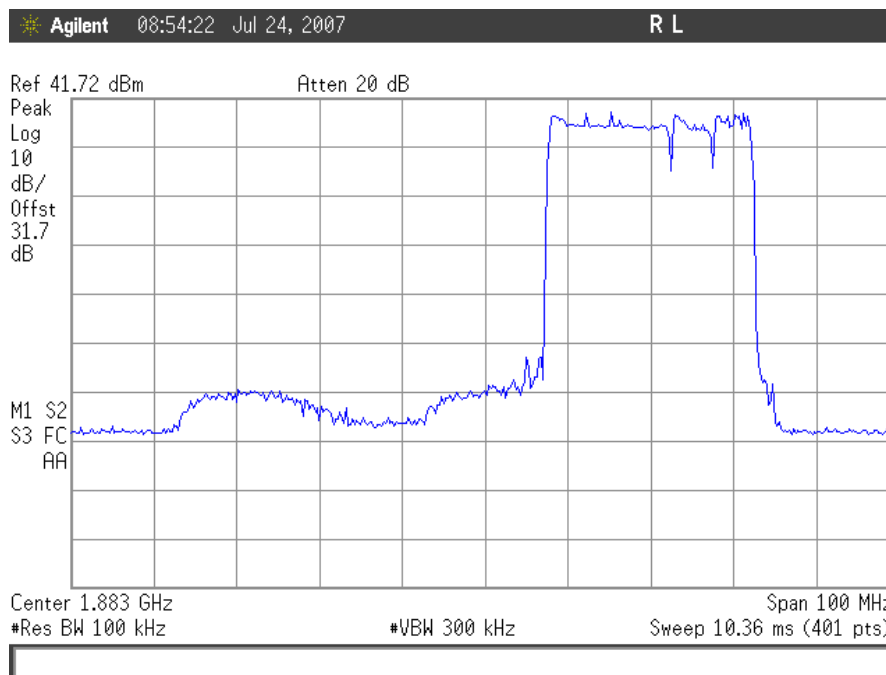
Plot 91. Out of Band Rejection, Uplink High End, 15MHz
