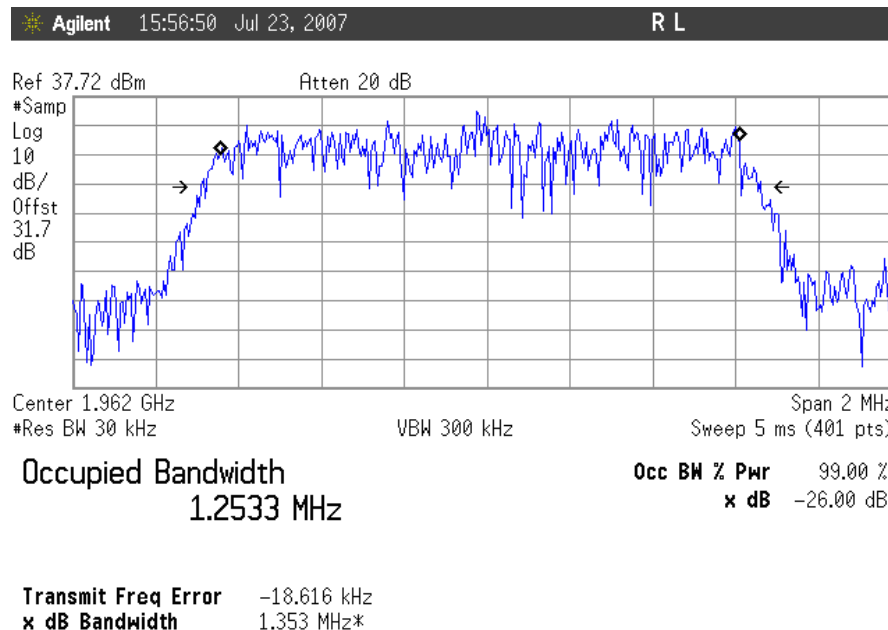
Plot 7. Occupied Bandwidth, CDMA Downlink, Mid Channel Output
