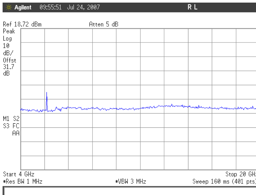
Plot 51. Conducted Spurious Emissions, CDMA High Channel 4GHz – 20GHz, Uplink
