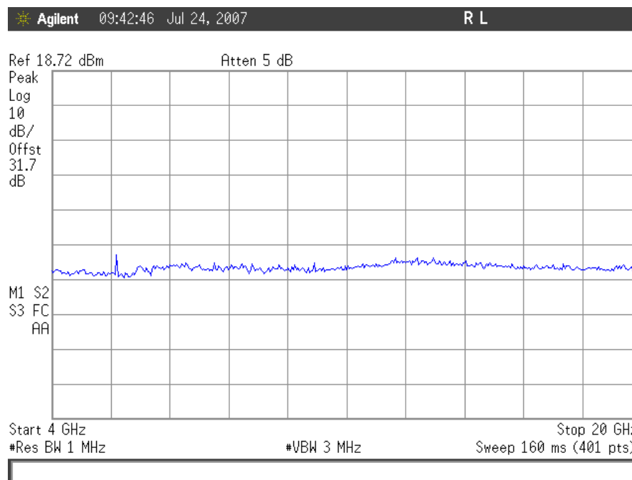
Plot 83. Conducted Spurious Emissions, TDMA High Channel 4GHz – 20GHz, Uplink
