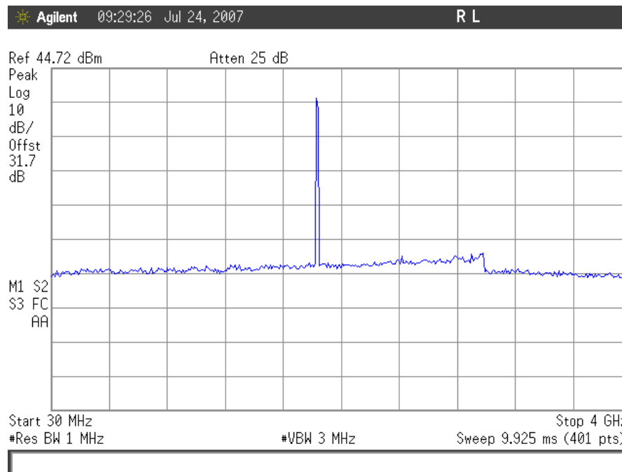
Plot 78. Conducted Spurious Emissions, TDMA Low Channel 30MHz – 4GHz, Uplink
