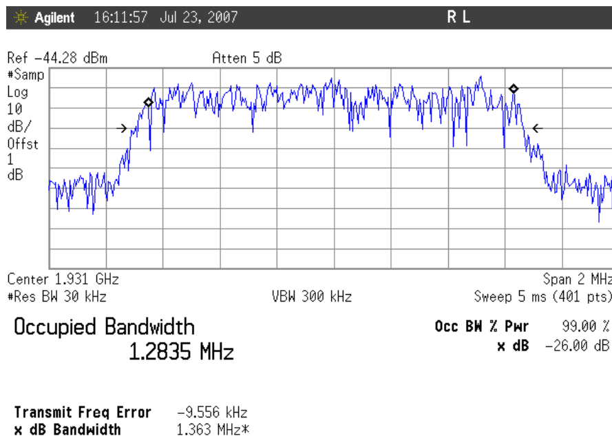
Plot 4. Occupied Bandwidth, CDMA Downlink, Low Channel Input
