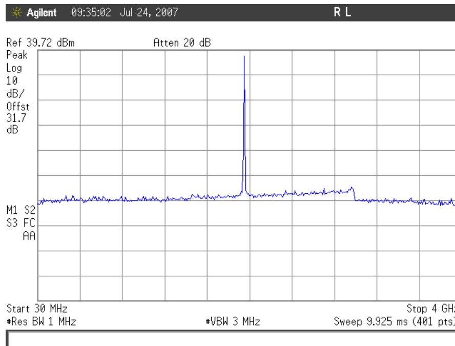
Plot 58. Conducted Spurious Emissions, GSM Mid Channel 30MHz – 4GHz, Downlink
