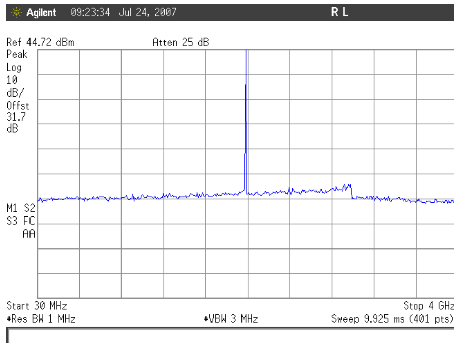
Plot 44. Conducted Spurious Emissions, CDMA High Channel 30MHz – 4GHz, Downlink
