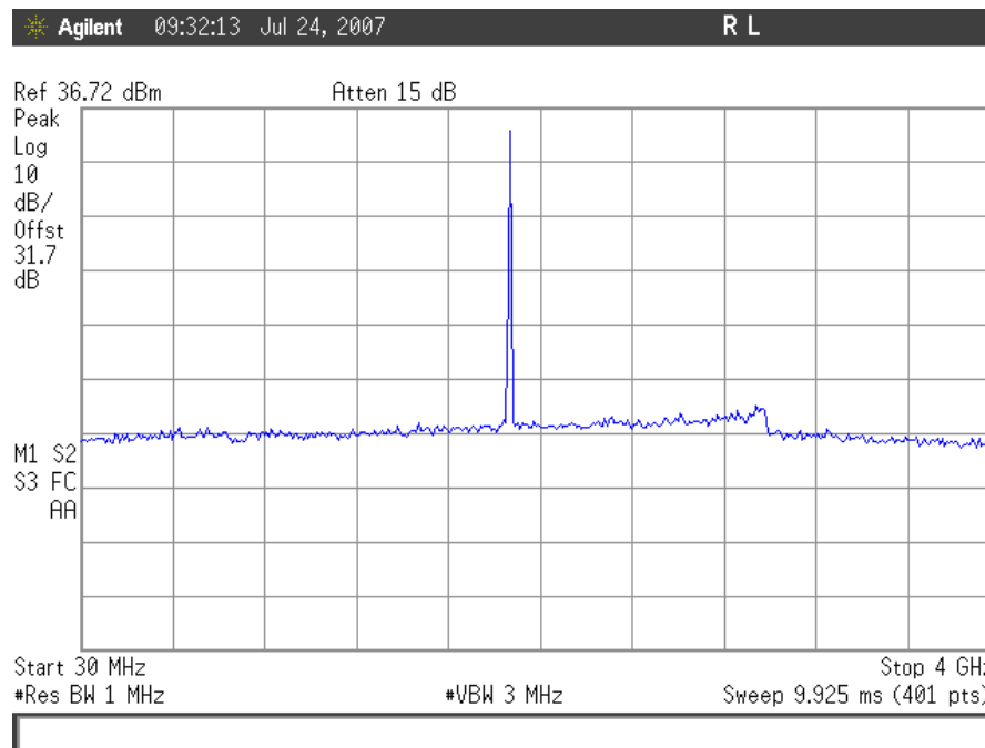
Plot 64. Conducted Spurious Emissions, GSM Mid Channel 30MHz – 4GHz, Uplink
