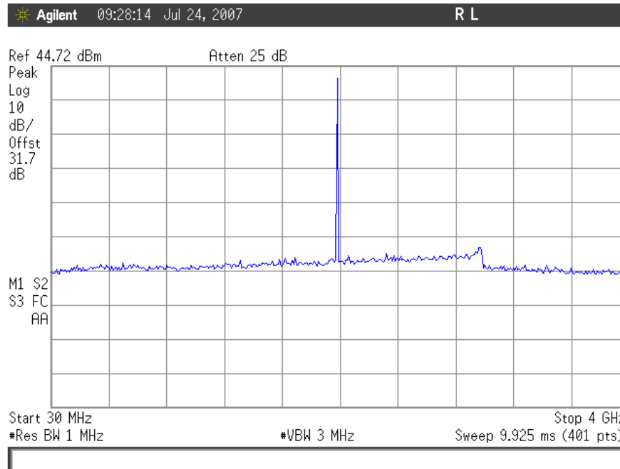
Plot 76. Conducted Spurious Emissions, TDMA High Channel 30MHz – 4GHz, Downlink
