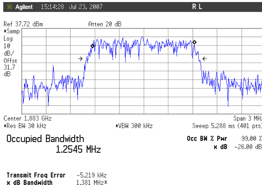
Plot 13. Occupied Bandwidth, CDMA Uplink, Mid Channel Output
