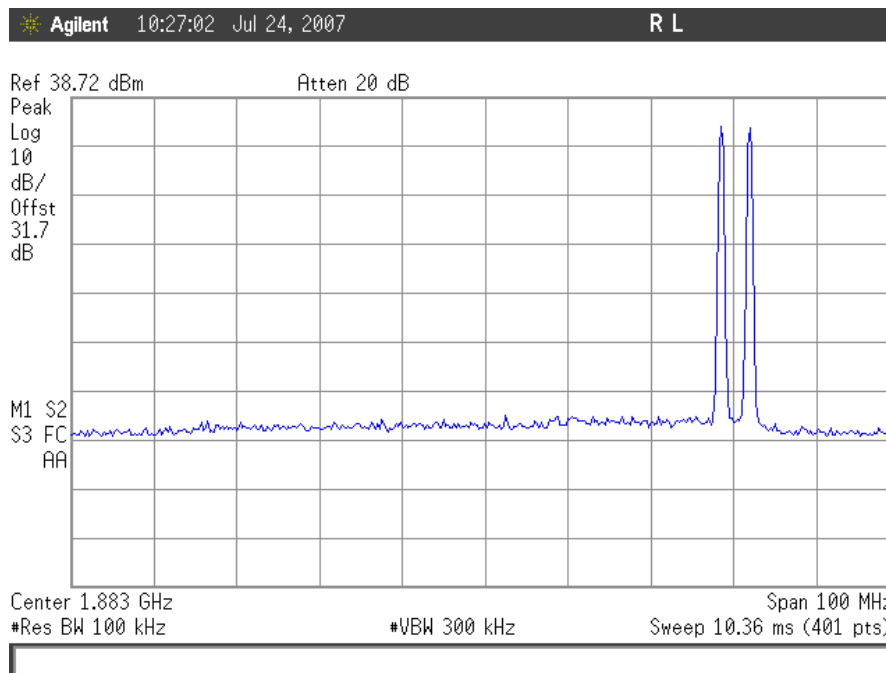
Plot 71. GSM Intermodulation, Uplink High End
