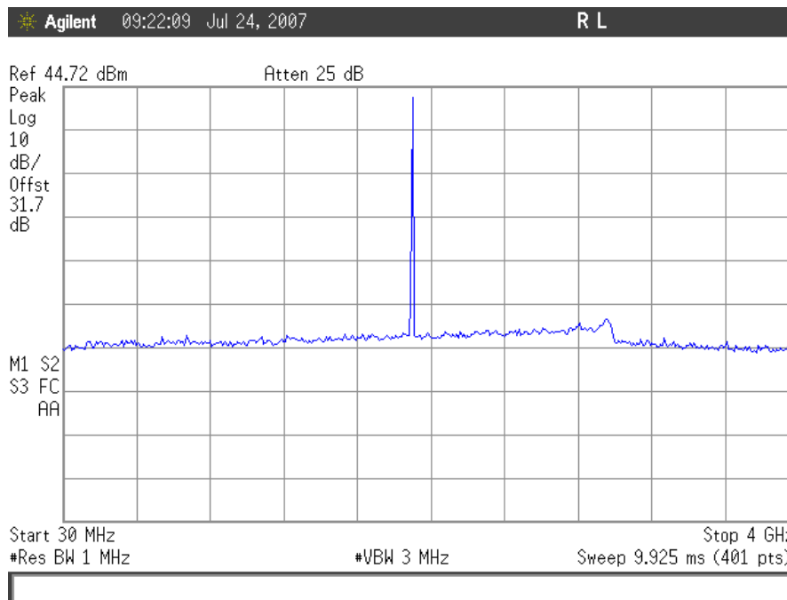
Plot 50. Conducted Spurious Emissions, CDMA High Channel 30MHz – 4GHz, Uplink
