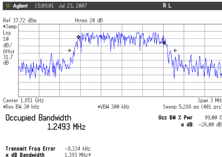
Plot 11. Occupied Bandwidth, CDMA Uplink, Low Channel Output
