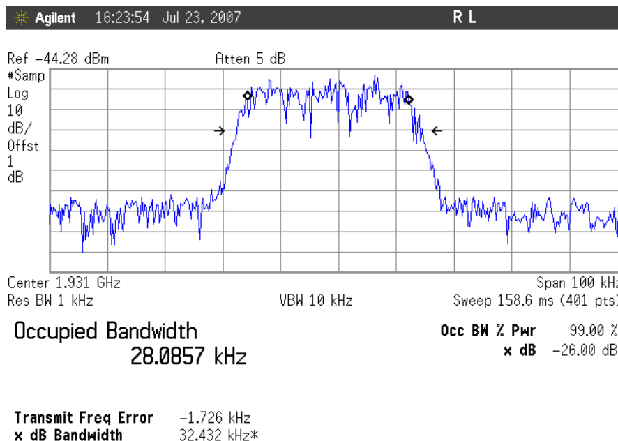
Plot 28. Occupied Bandwidth, TDMA Downlink, Low Channel Input
