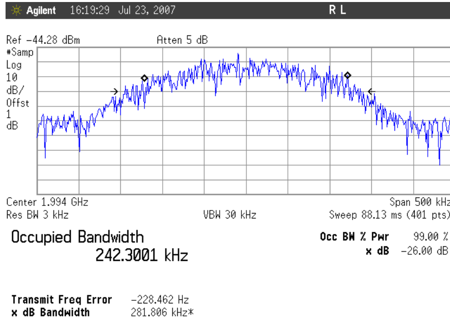
Plot 20. Occupied Bandwidth, GSM Downlink, High Channel Input
