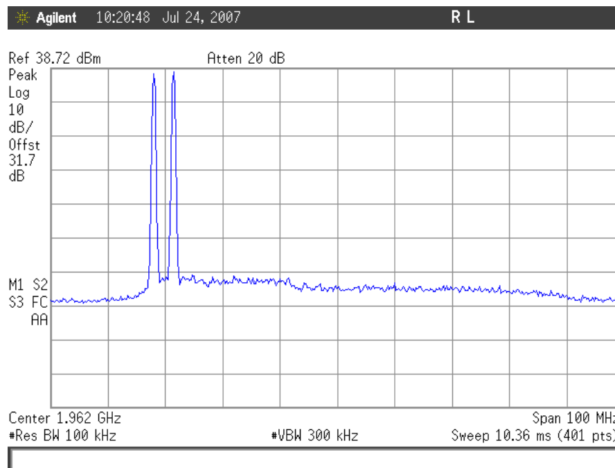
Plot 68. GSM Intermodulation, Downlink Low End
