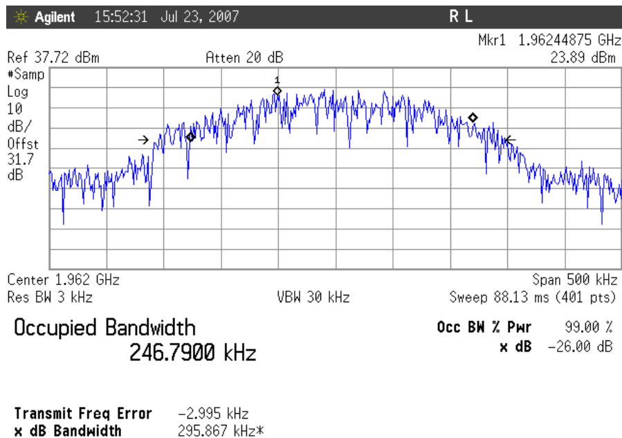
Plot 19. Occupied Bandwidth, GSM Downlink, Mid Channel Output
