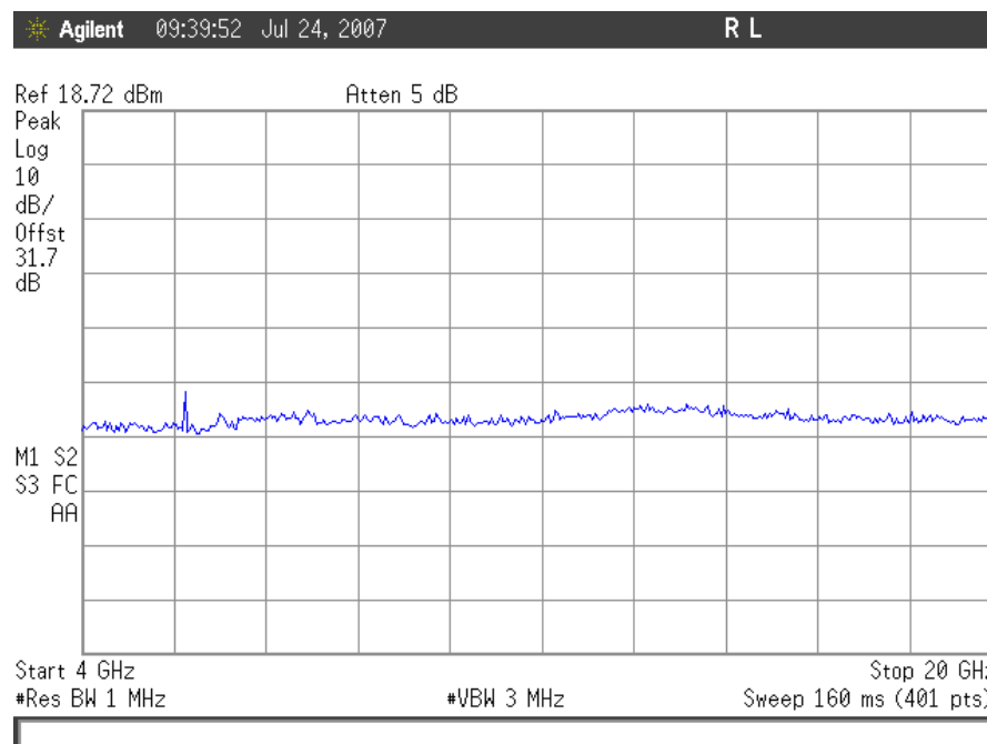
Plot 57. Conducted Spurious Emissions, GSM Low Channel 4GHz – 20GHz, Downlink
