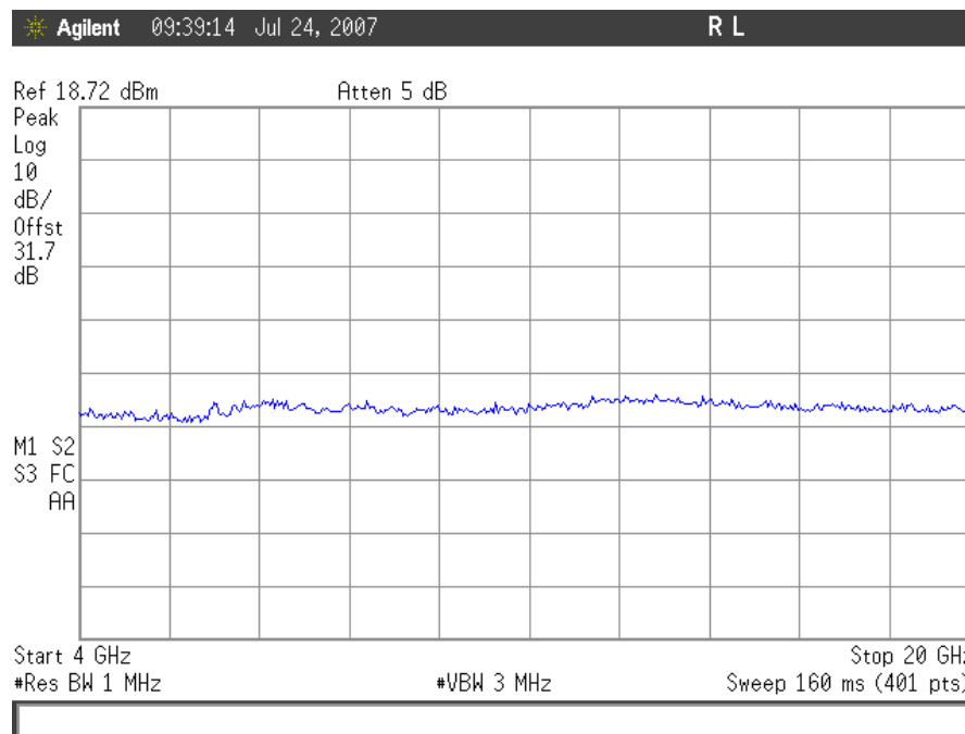
Plot 59. Conducted Spurious Emissions, GSM Mid Channel 4GHz – 20GHz, Downlink
