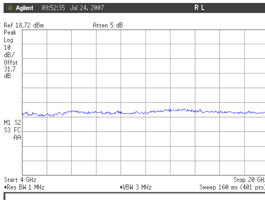
Plot 41. Conducted Spurious Emissions, CDMA Low Channel 4GHz – 20GHz, Downlink
