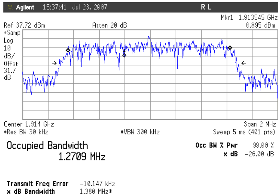
Plot 15. Occupied Bandwidth, CDMA Uplink, High Channel Output
