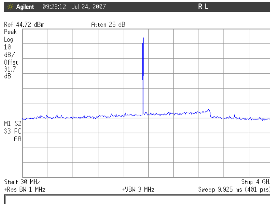
Plot 72. Conducted Spurious Emissions, TDMA Low Channel 30MHz – 4GHz, Downlink
