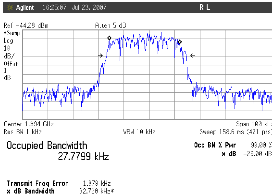
Plot 32. Occupied Bandwidth, TDMA Downlink, High Channel Input
