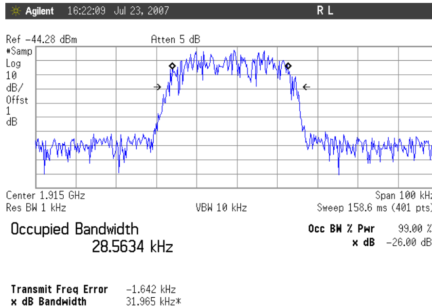
Plot 38. Occupied Bandwidth, TDMA Uplink, High Channel Input
