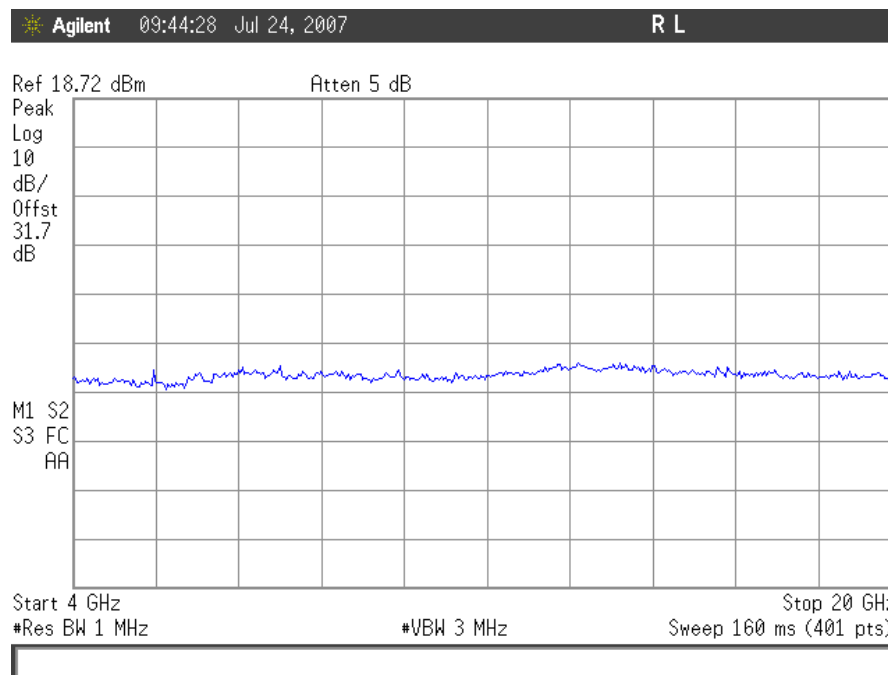
Plot 79. Conducted Spurious Emissions, TDMA Low Channel 4GHz – 20GHz, Uplink
