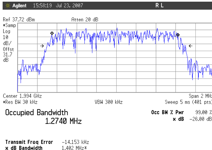
Plot 9. Occupied Bandwidth, CDMA Downlink, High Channel Output
