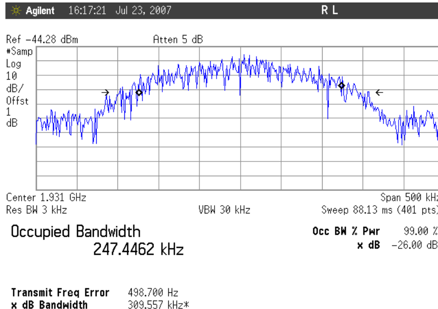
Plot 16. Occupied Bandwidth, GSM Downlink, Low Channel Input
