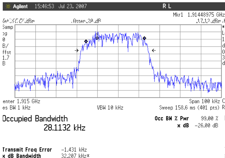
Plot 39. Occupied Bandwidth, TDMA Uplink, High Channel Output
