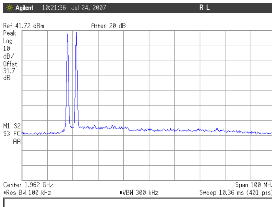
Plot 84. TDMA Intermodulation, Downlink Low End
