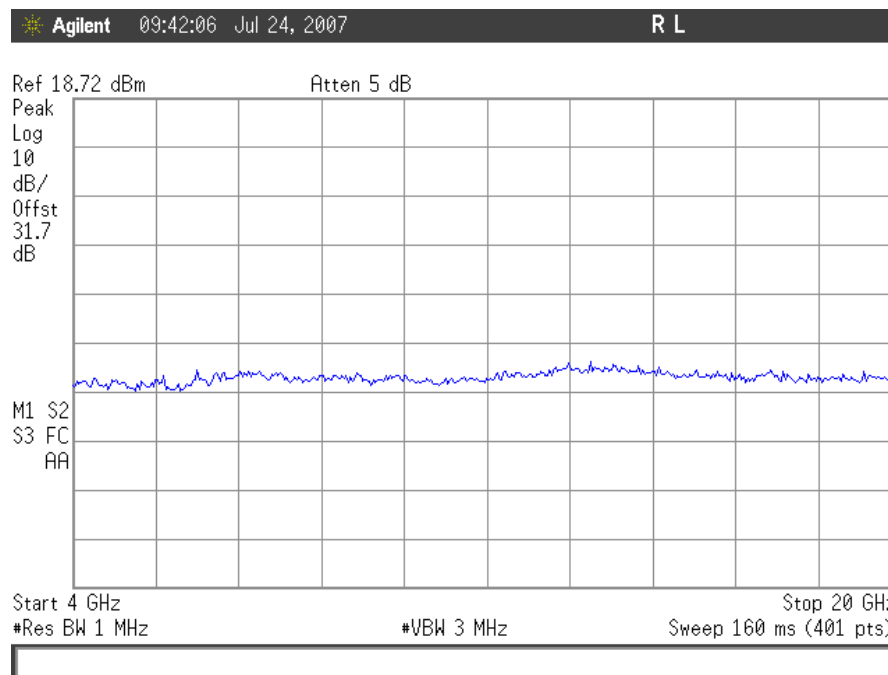
Plot 67. Conducted Spurious Emissions, GSM High Channel 4GHz – 20GHz, Uplink
