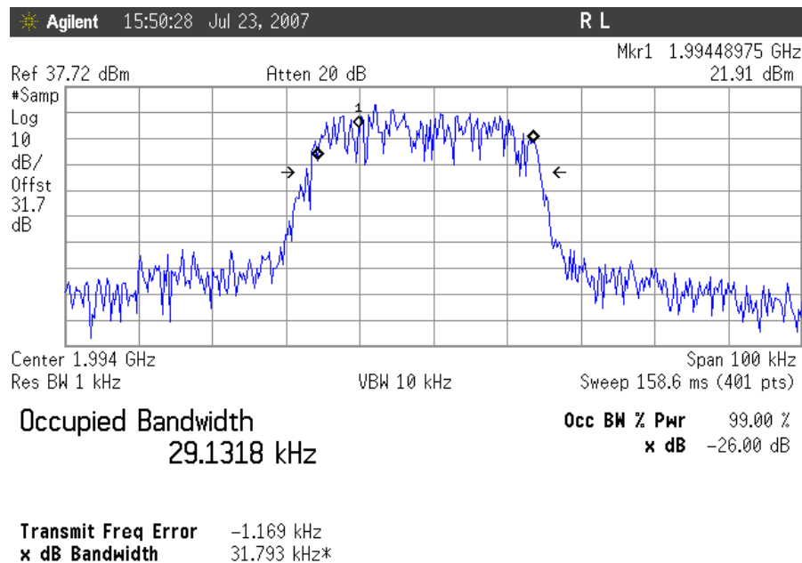
Plot 33. Occupied Bandwidth, TDMA Downlink, High Channel Output
