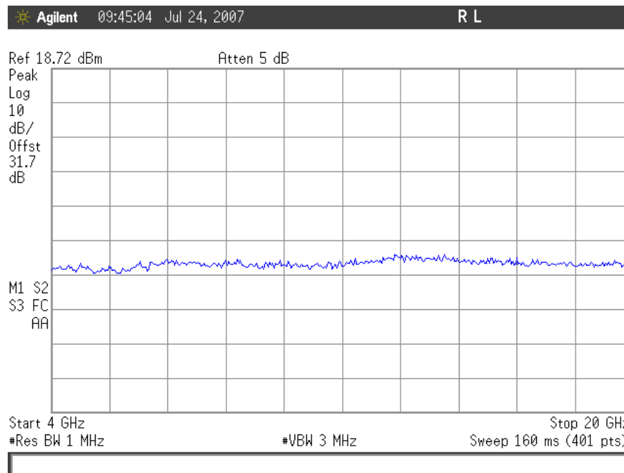
Plot 81. Conducted Spurious Emissions, TDMA Mid Channel 4GHz – 20GHz, Uplink
