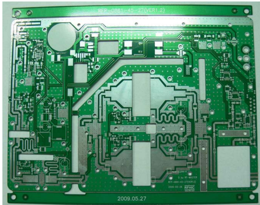
< Bare PCB Front >
