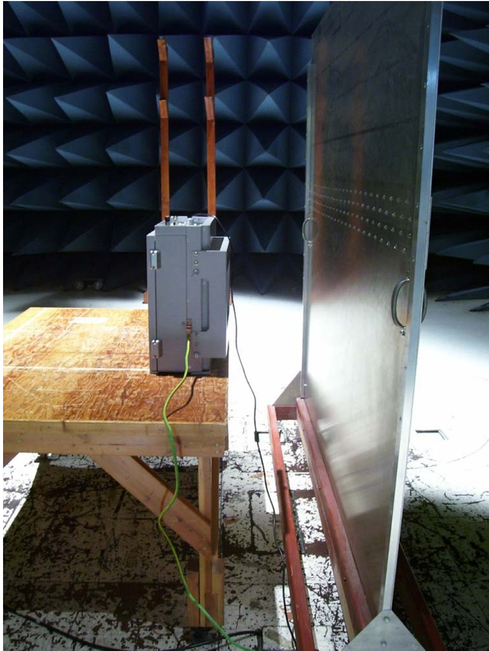
Photograph 3. Conducted Emissions Test Setup Photograph
