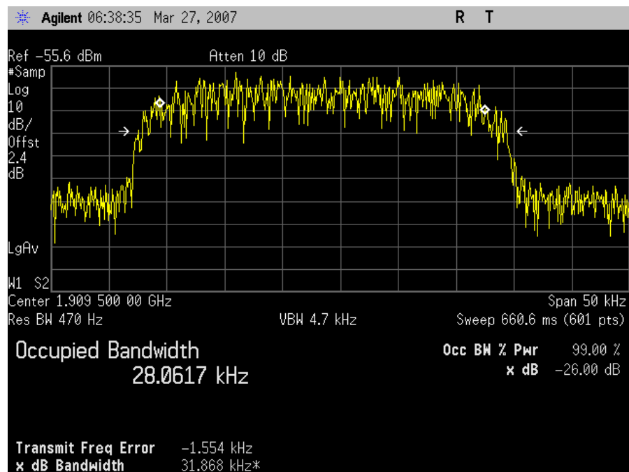
High Channel Input – UpLink
