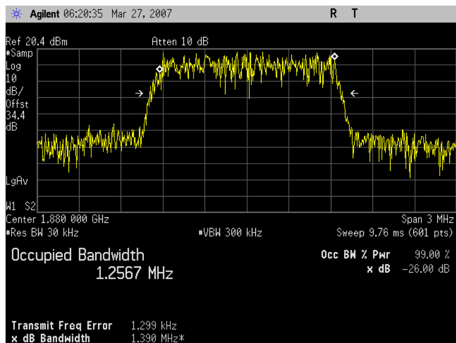
Mid Channel Output – UpLink
