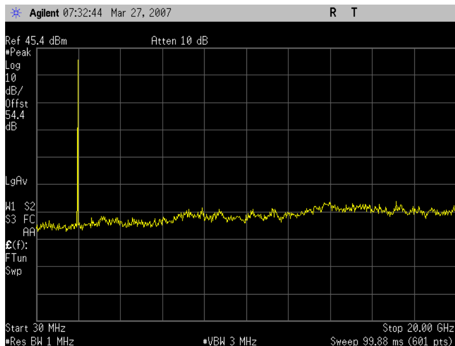
Conducted Spurious Emissions High Channel DownLink
