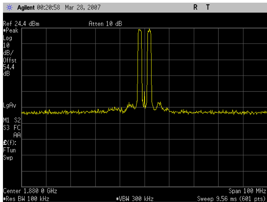
CDMA Uplink Intermodulation Mid Channel
