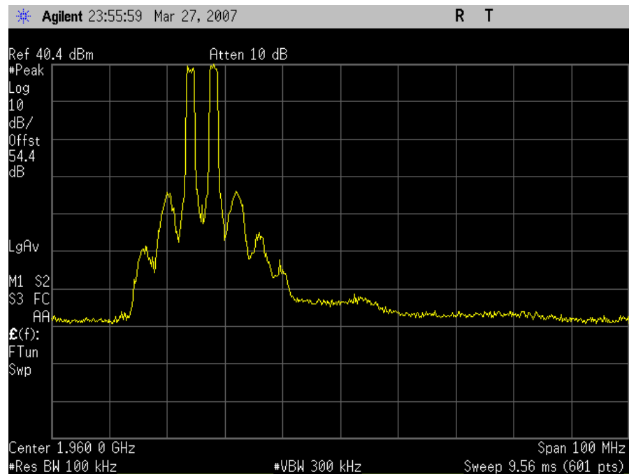
CDMA Downlink Intermodulation Low Channel
