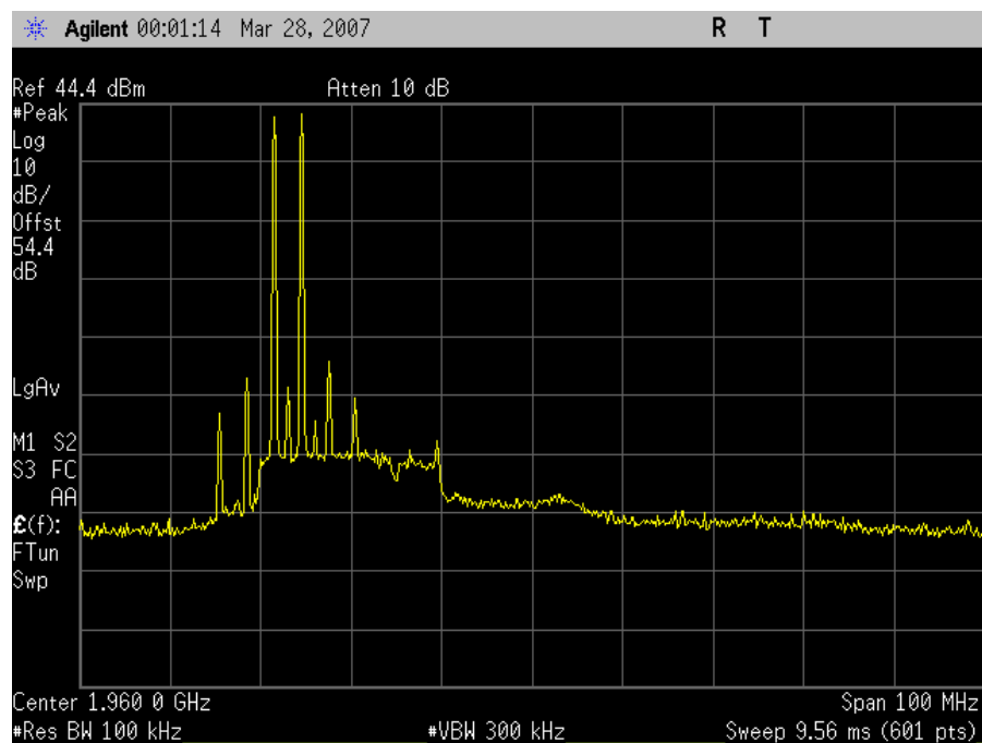
TDMA Downlink Intermodulation Low Channel
