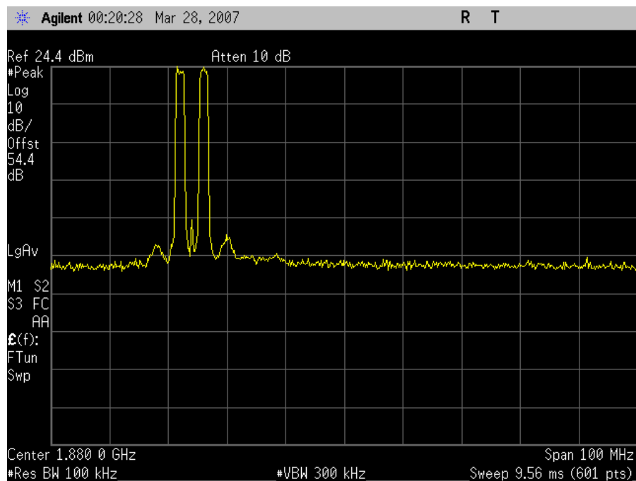
CDMA Uplink Intermodulation Low Channel
