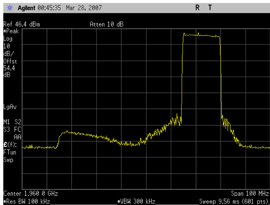
Out of Band Rejection Downlink – 15MHz High End
