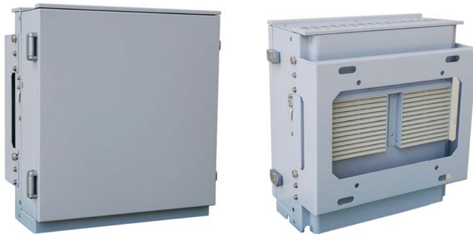
Photograph 1. Advanced RF Technologies Epoch-HP-20, Epoch-HP-10, Epoch-HP-05 and Epoch-HP-XX with 5MHz and 15MHz filters (1900MHz band)
