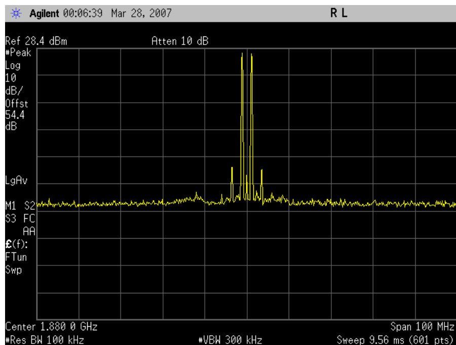
GSM Uplink Intermodulation Mid Channel
