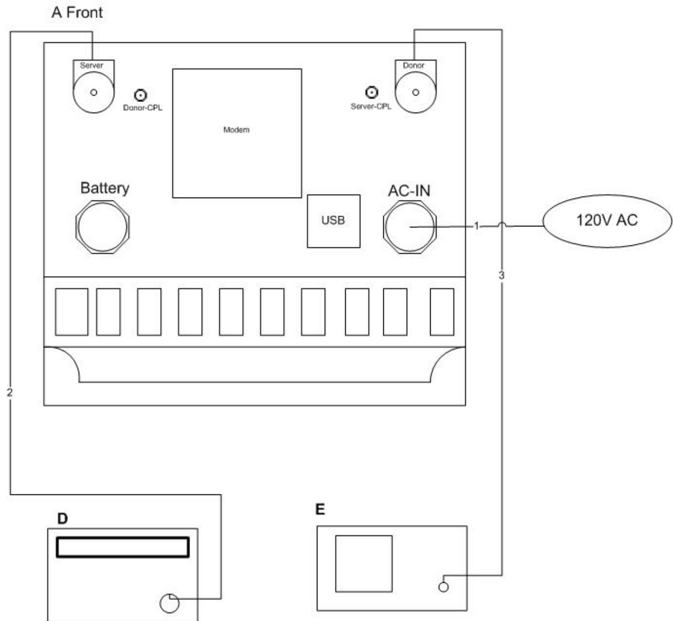
Figure 4. Block Diagram of Test Configuration (Conducted Measurement – Uplink)
