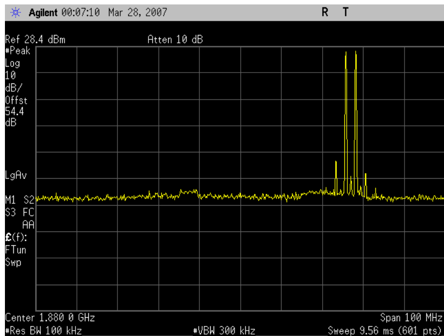
GSM Uplink Intermodulation High Channel
