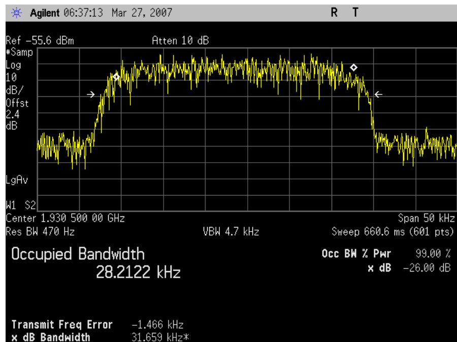
Low Channel Input - DownLink
