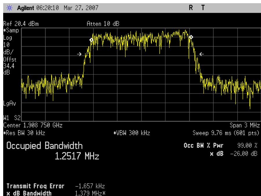
High Channel Output – UpLink
