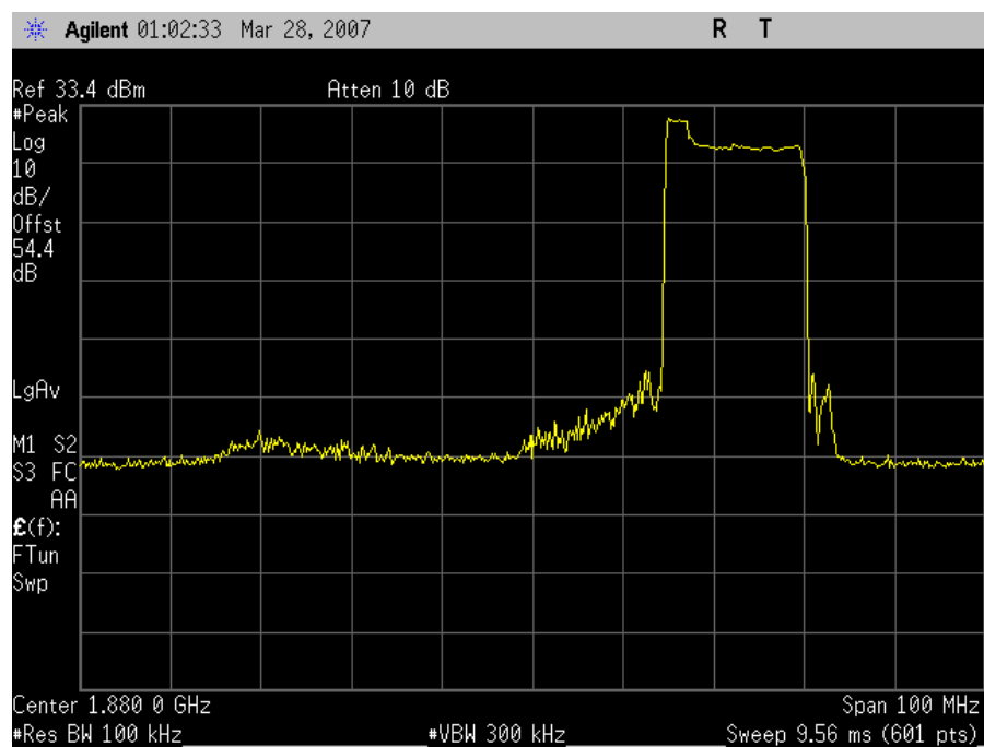
Out of Band Rejection Uplink – 15MHz High End
