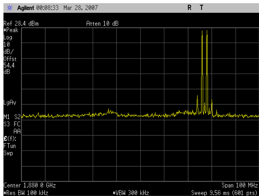
TDMA Uplink Intermodulation High Channel
