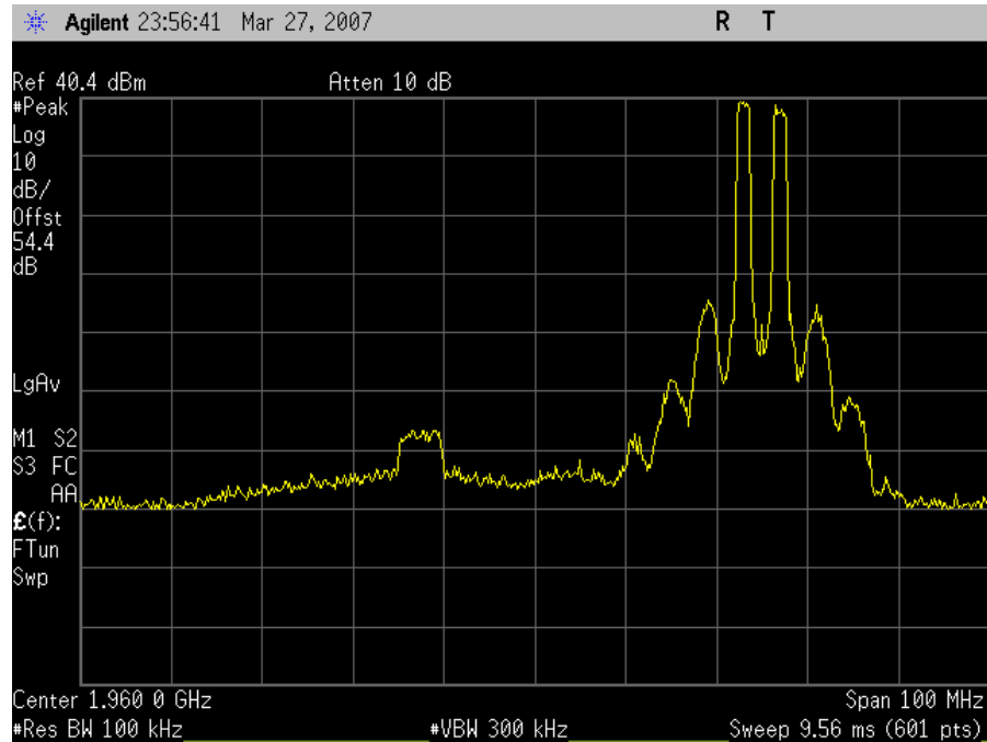
CDMA Downlink Intermodulation High Channel
