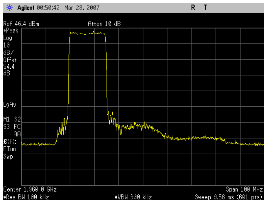
Out of Band Rejection Downlink – 15MHz Low End
