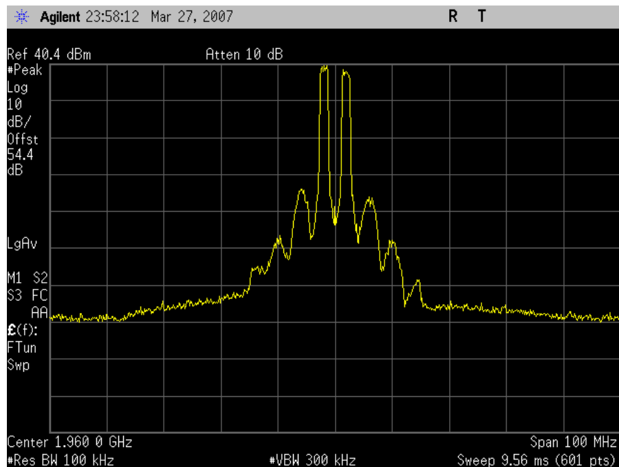
CDMA Downlink Intermodulation Mid Channel
