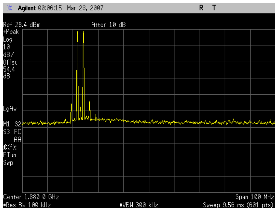
GSM Uplink Intermodulation Low Channel
