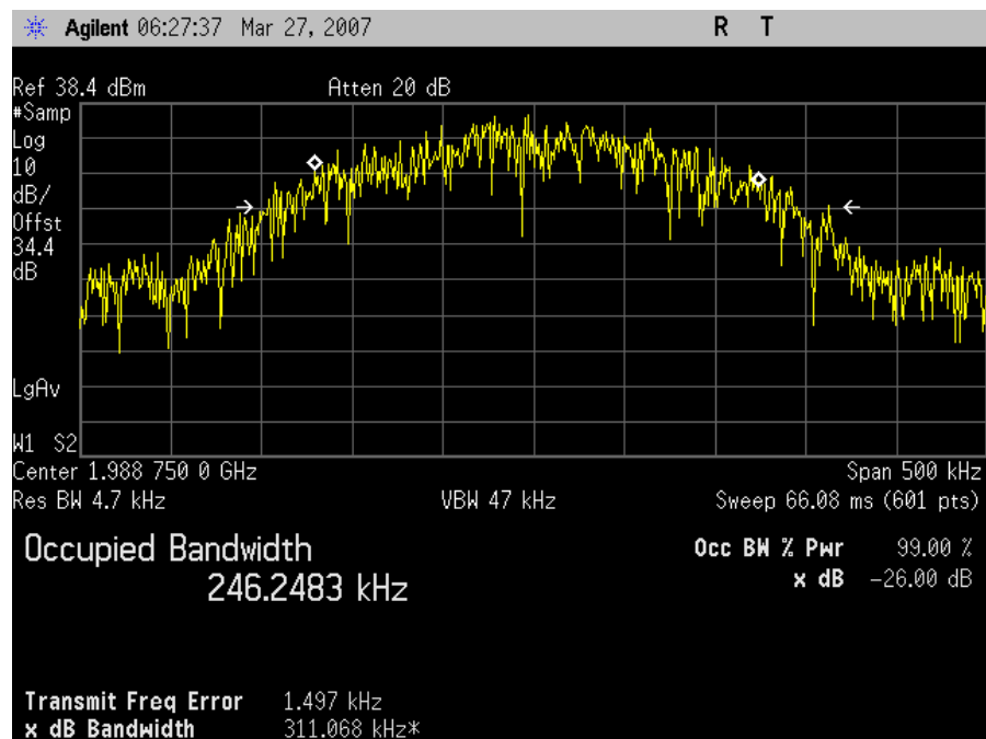
High Channel Output – DownLink
