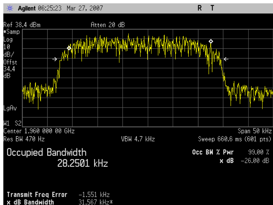
Mid Channel Output – DownLink
