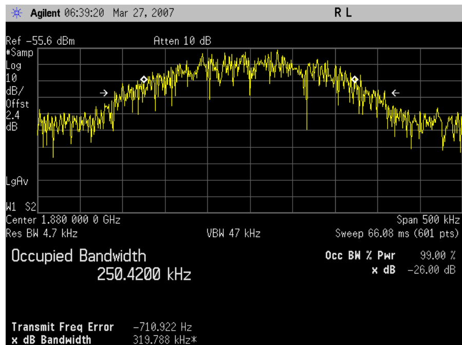
Mid Channel Input – UpLink
