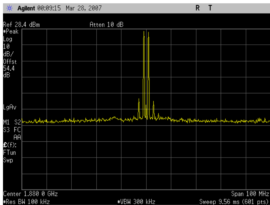
TDMA Uplink Intermodulation Mid Channel
