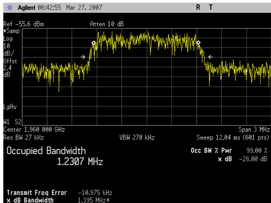
Mid Channel Input – DownLink
