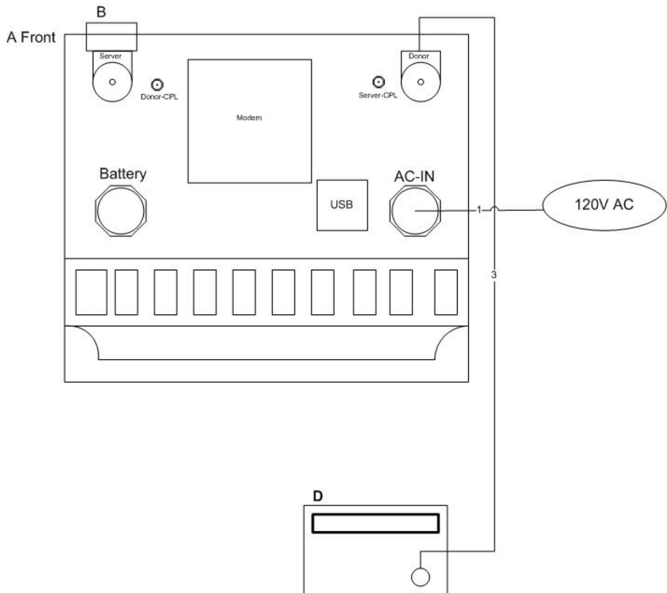
Figure 1. Block Diagram of Test Configuration (Spurious Emissions - Downlink)
