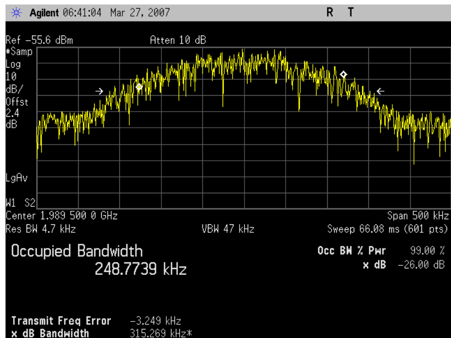
High Channel Input – DownLink
