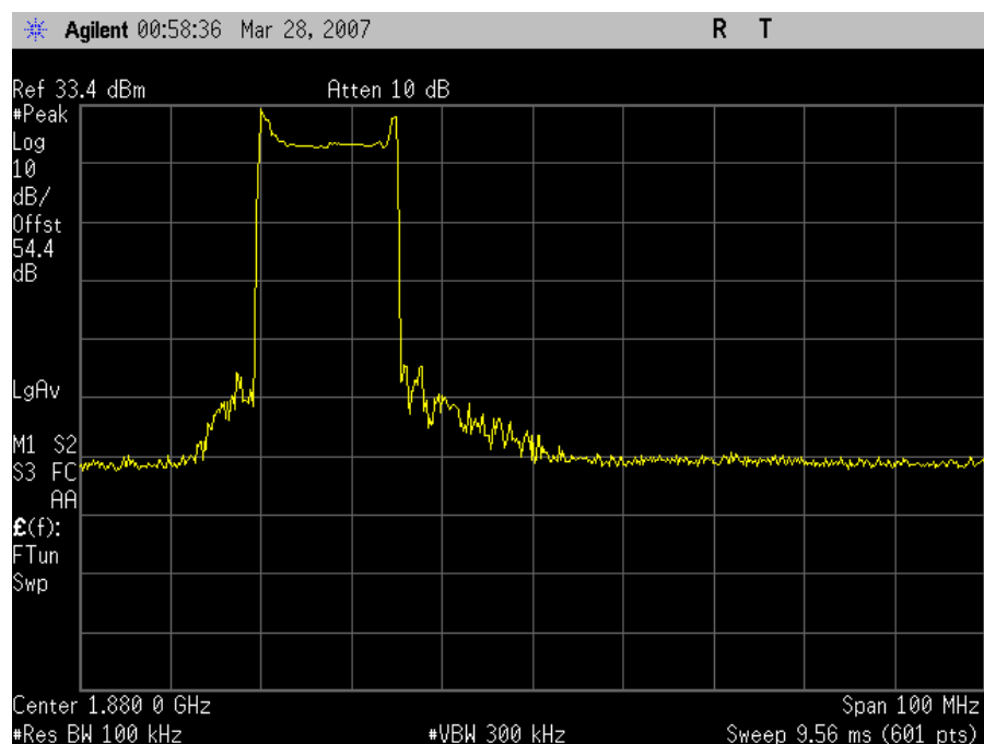
Out of Band Rejection Uplink – 15MHz Low End
