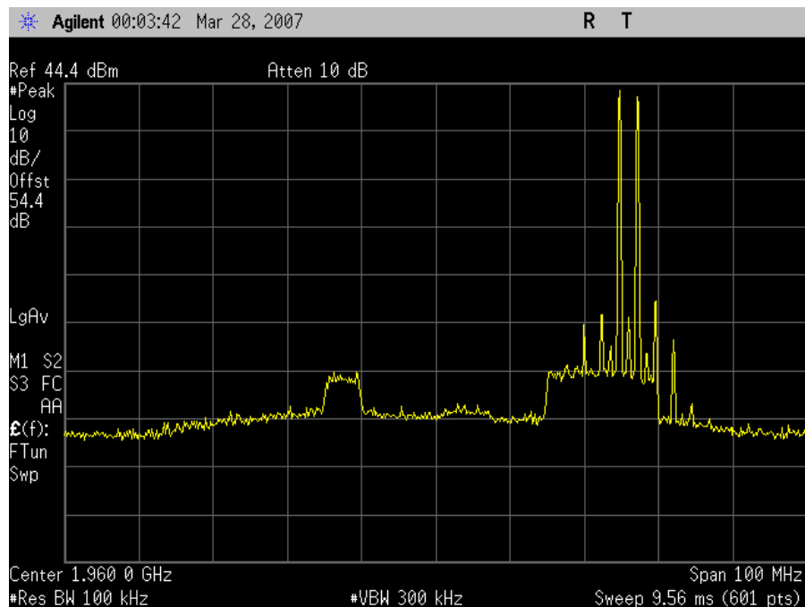
GSM Downlink Intermodulation High Channel
