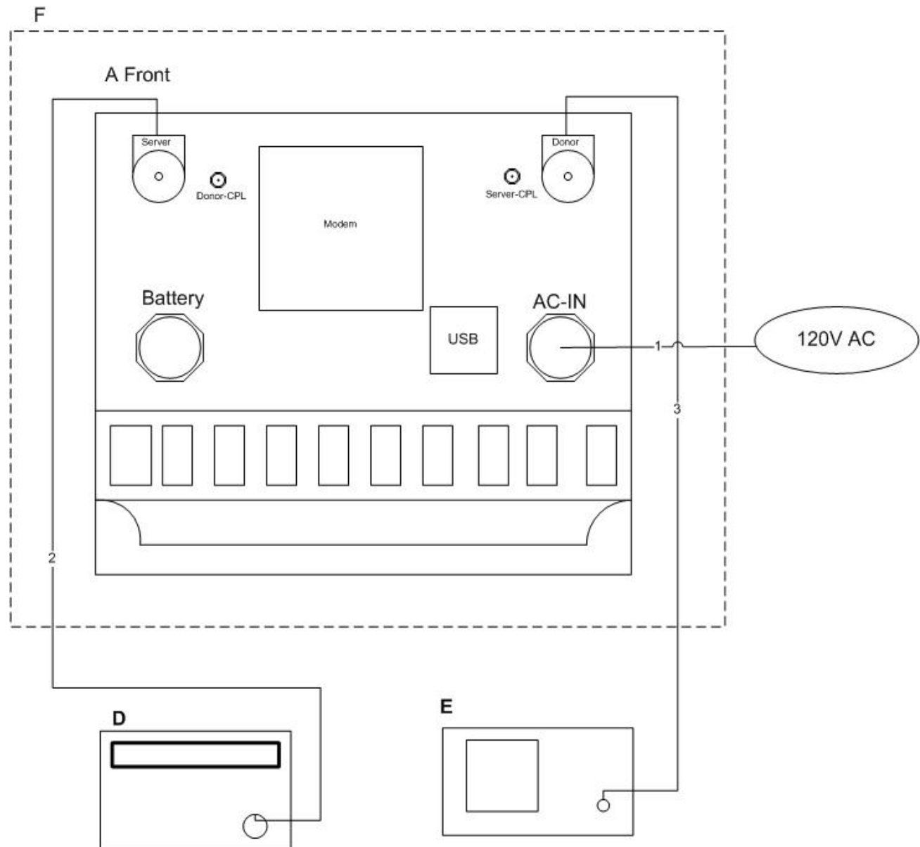
Figure 6. Block Diagram of Test Configuration (Frequency Stability)
