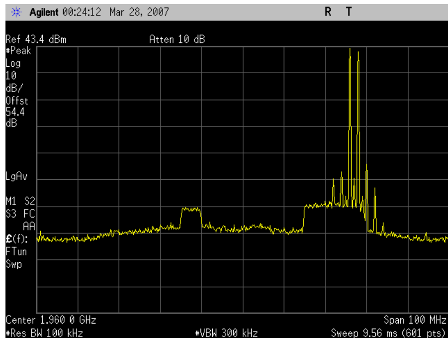
TDMA Downlink Intermodulation High Channel
