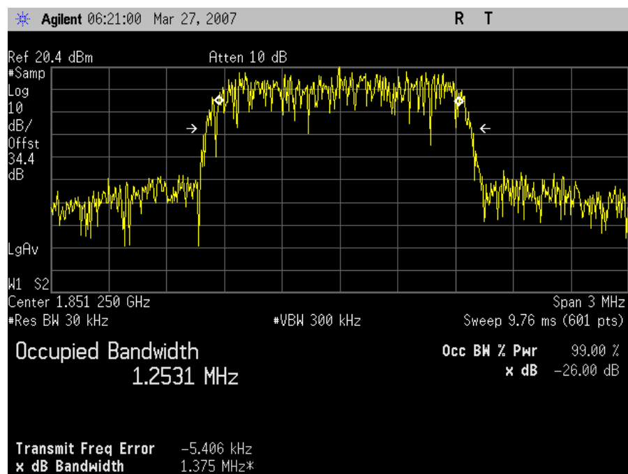
Low Channel Output - UpLink
