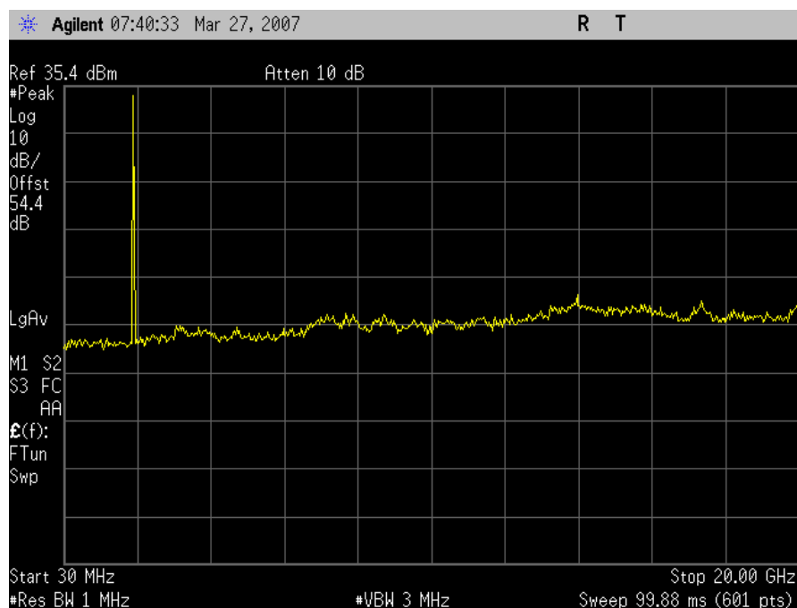
Conducted Spurious Emissions High Channel UpLink
