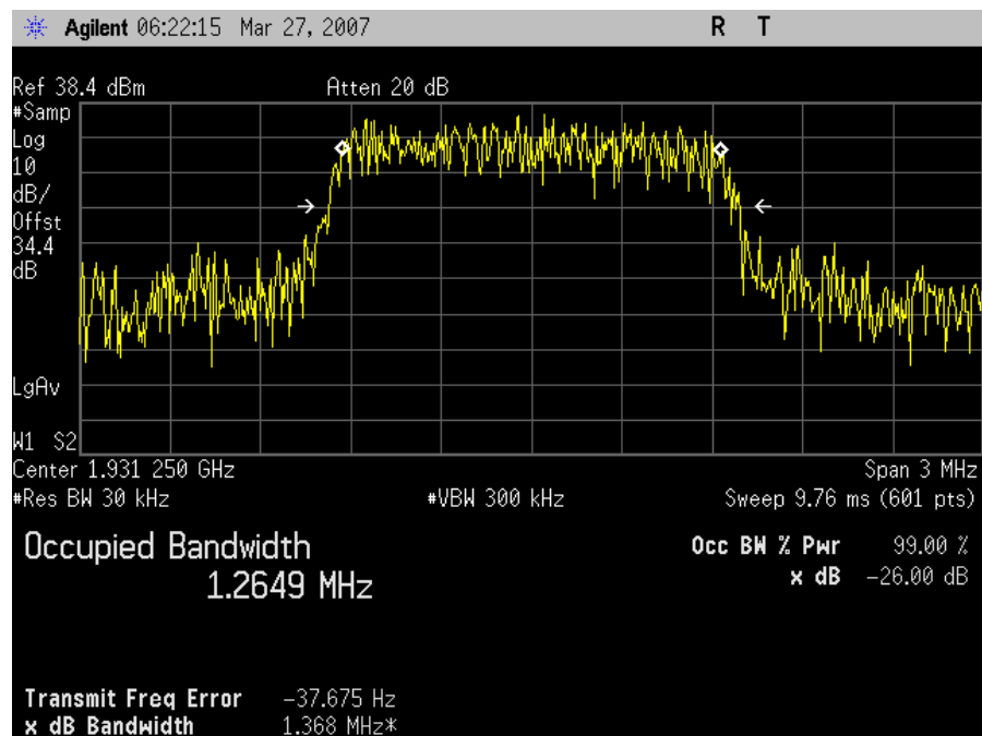
Low Channel Output - DownLink
