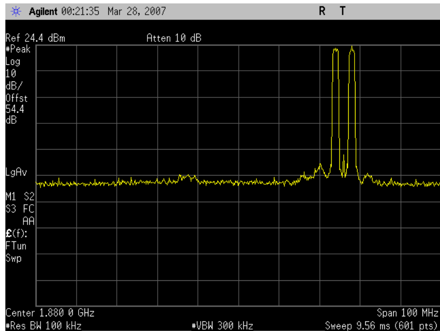
CDMA Uplink Intermodulation High Channel
