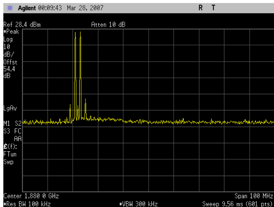
TDMA Uplink Intermodulation Low Channel
