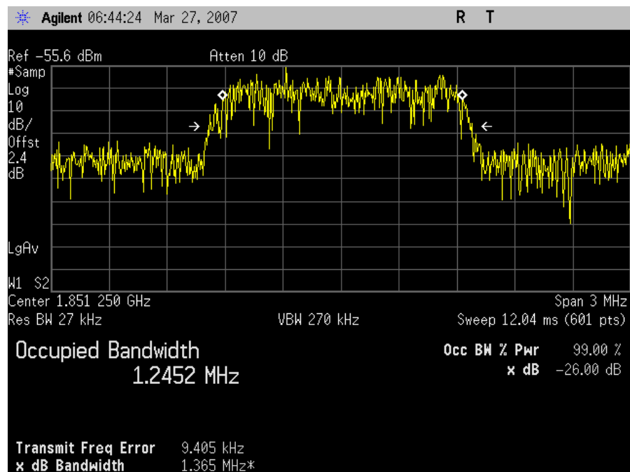
Low Channel Input - UpLink
