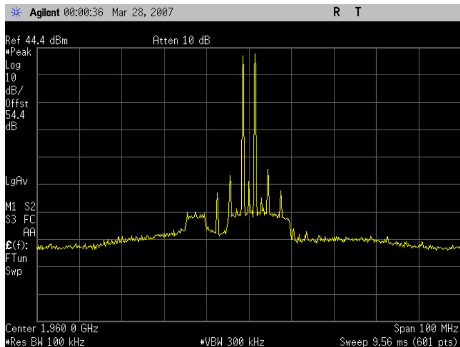
TDMA Downlink Intermodulation Mid Channel
