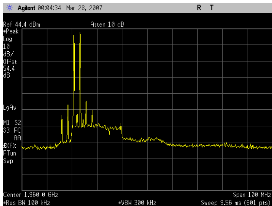
GSM Downlink Intermodulation Low Channel
