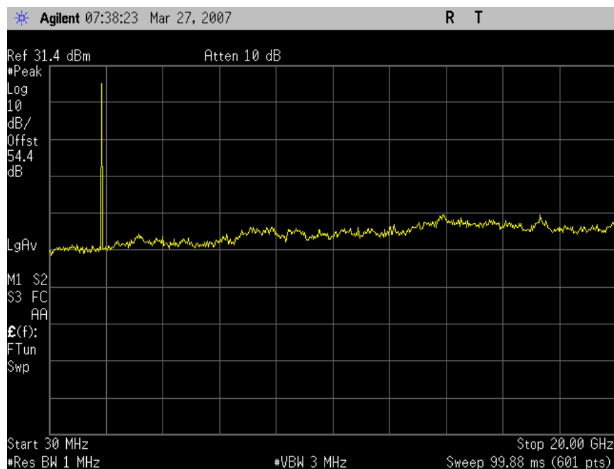
Conducted Spurious Emissions Low Channel UpLink
