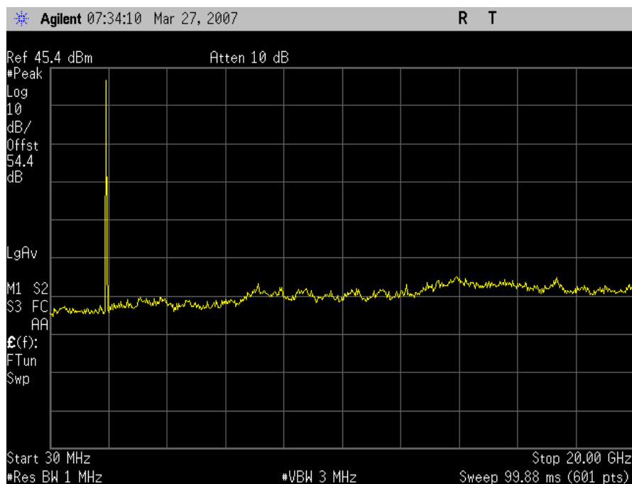
Conducted Spurious Emissions Low Channel DownLink
