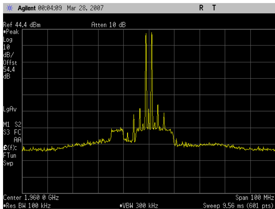
GSM Downlink Intermodulation Mid Channel
