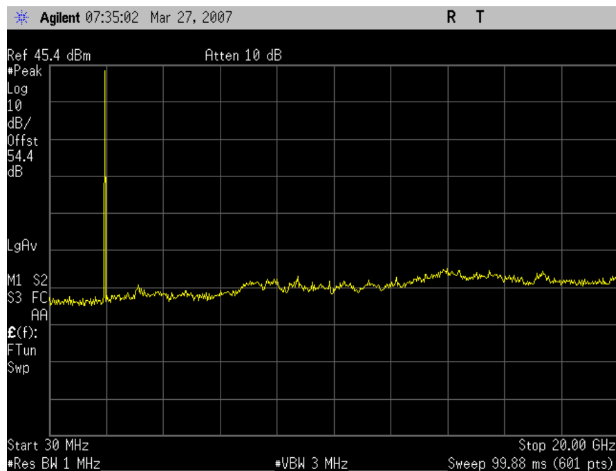
Conducted Spurious Emissions Mid Channel DownLink
