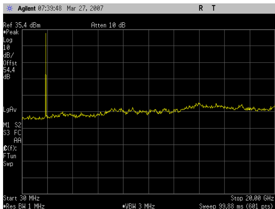
Conducted Spurious Emissions Mid Channel UpLink
