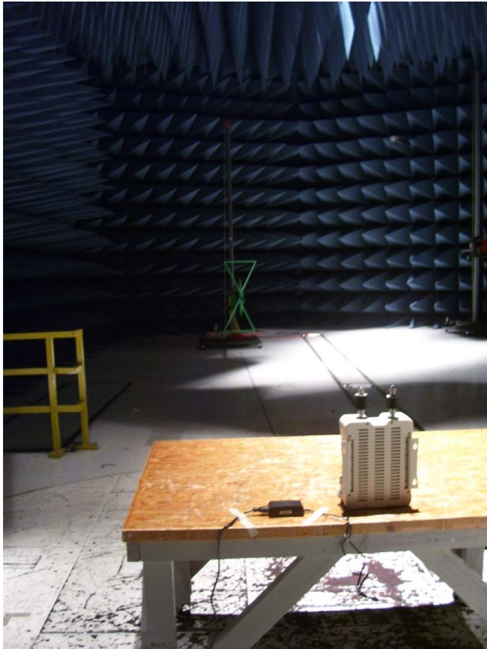
Radiated Emission Limits, Test Setup
