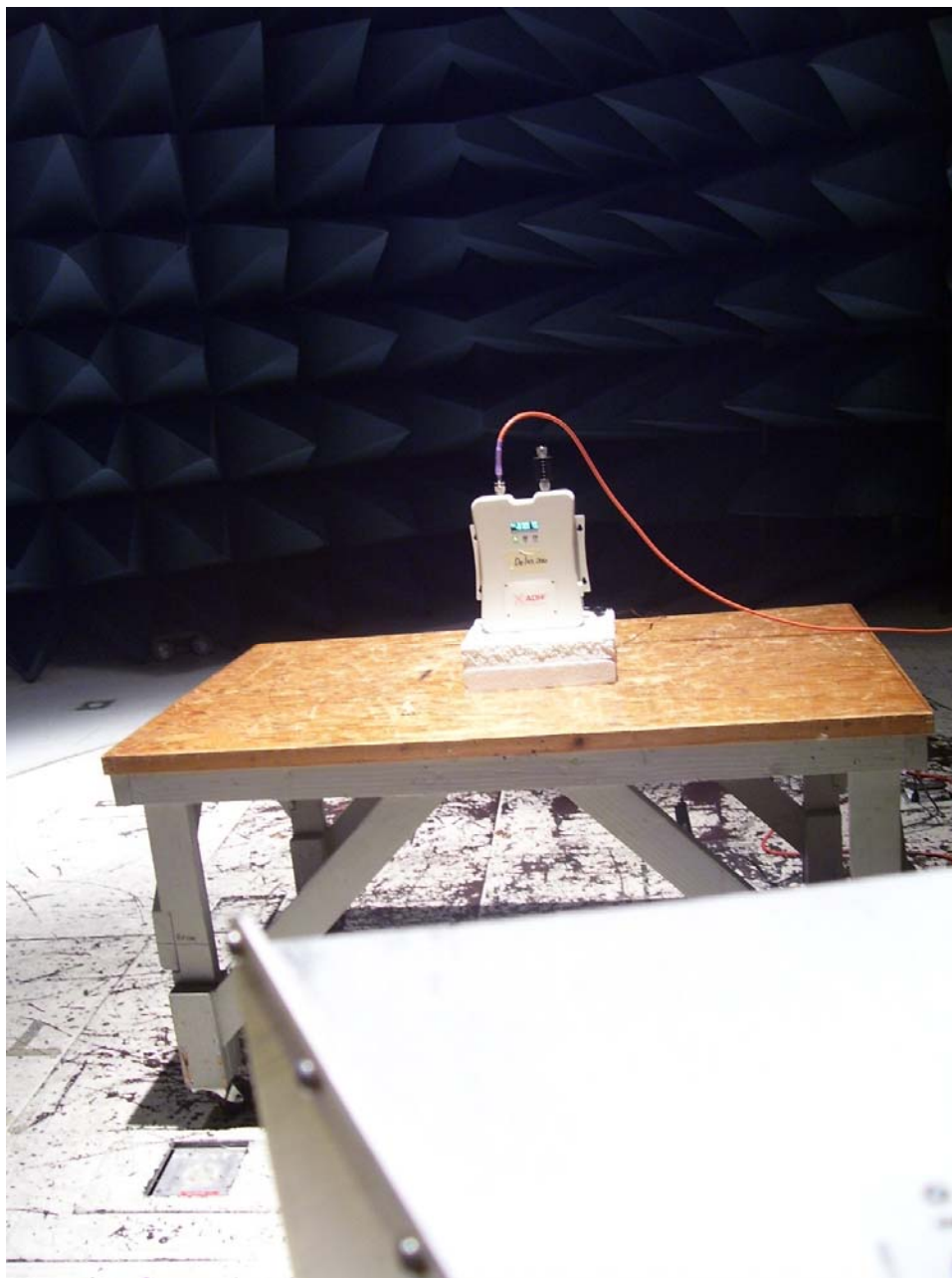
Radiated Spurious Emissions, Test Setup, Downlink
