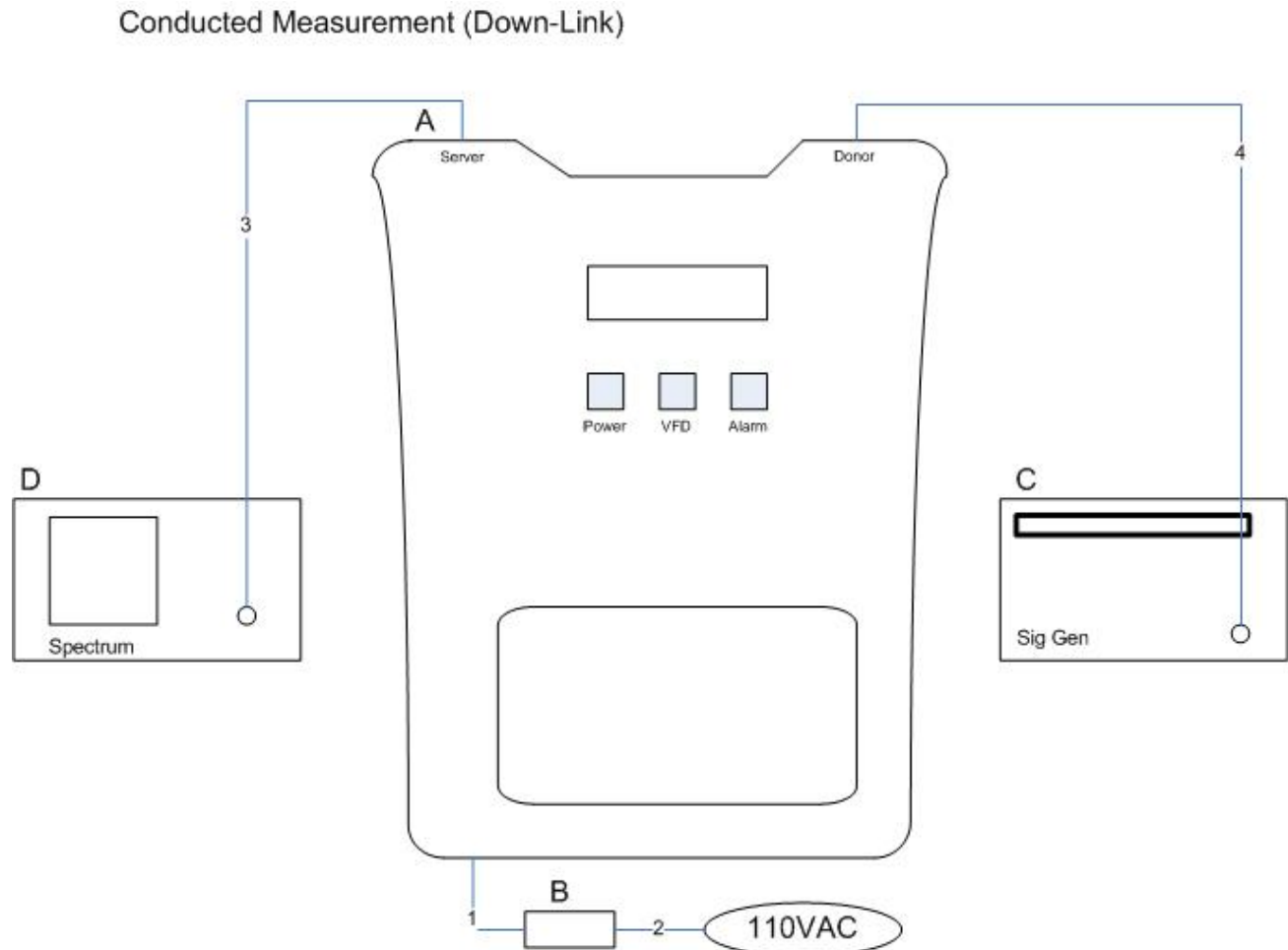
Figure 2. Block Diagram of Test Configuration (Conducted Measurement-Downlink)
