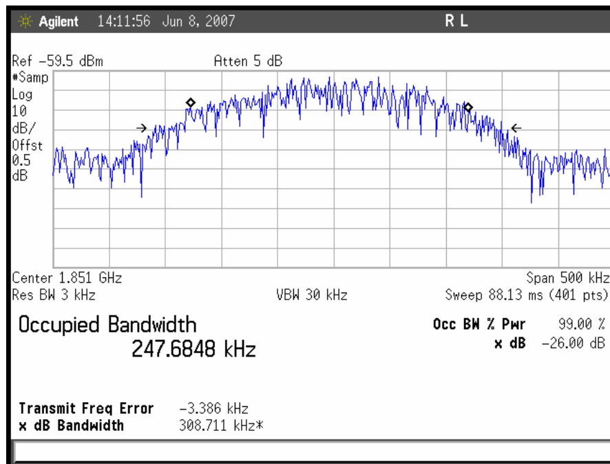
Plot 20. Occupied Bandwidth, GSM Uplink, Low Channel Input
