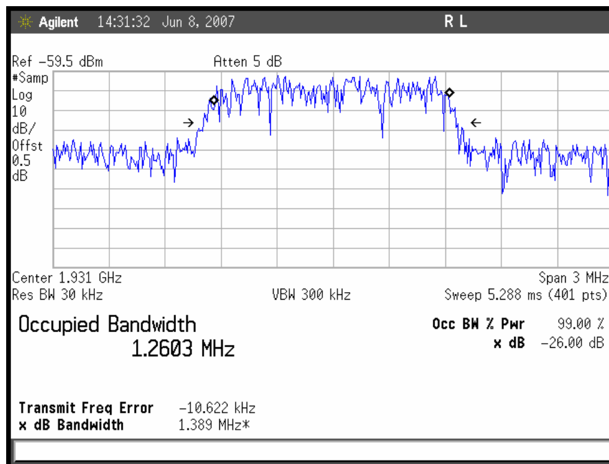
Plot 2. Occupied Bandwidth, CDMA Downlink, Low Channel Input
