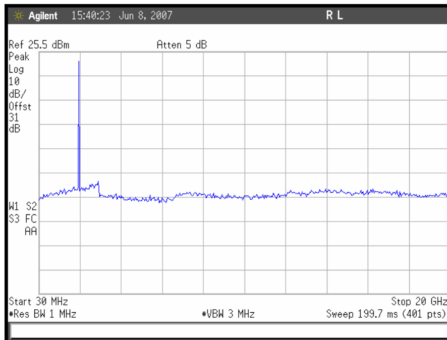
Plot 52. Conducted Spurious Emissions, GSM High Channel Downlink
