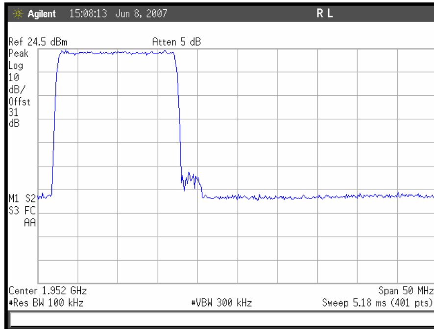
Plot 68. Out of Band Rejection, Downlink Low End filter
