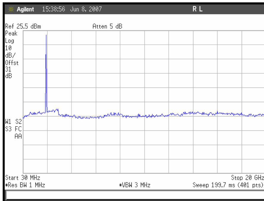
Plot 58. Conducted Spurious Emissions, TDMA Low Channel Downlink
