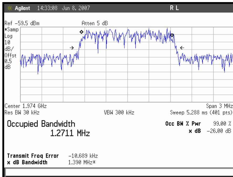
Plot 6. Occupied Bandwidth, CDMA Downlink, High Channel Input
