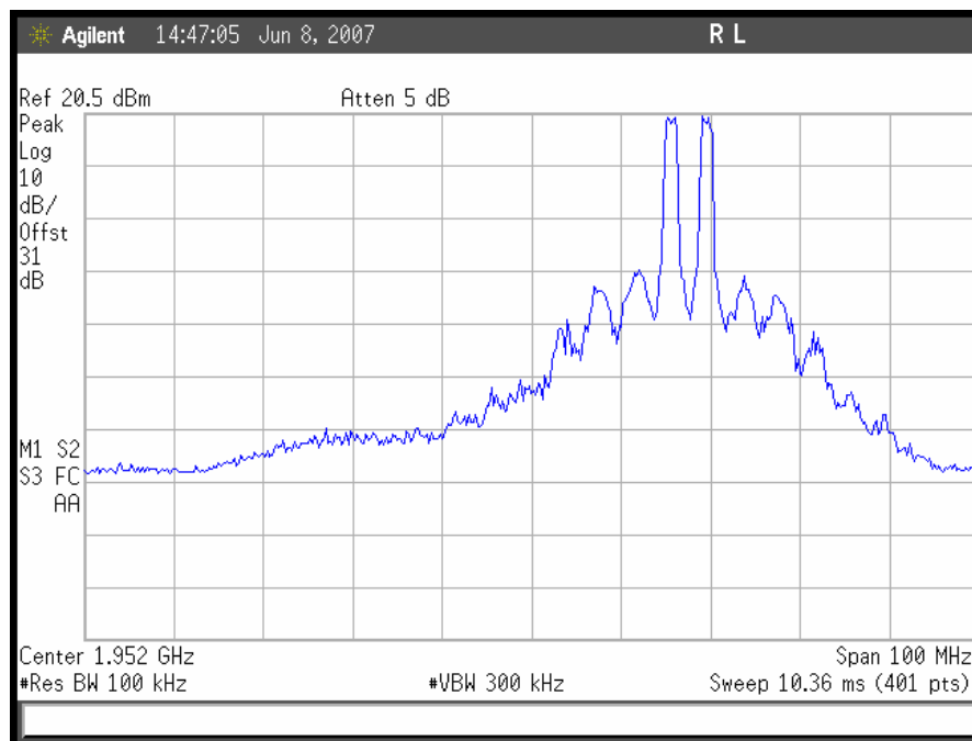
Plot 45. CDMA Intermodulation, Downlink High End
