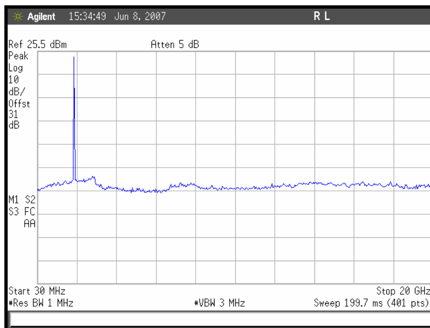
Plot 59. Conducted Spurious Emissions, TDMA Low Channel Uplink
