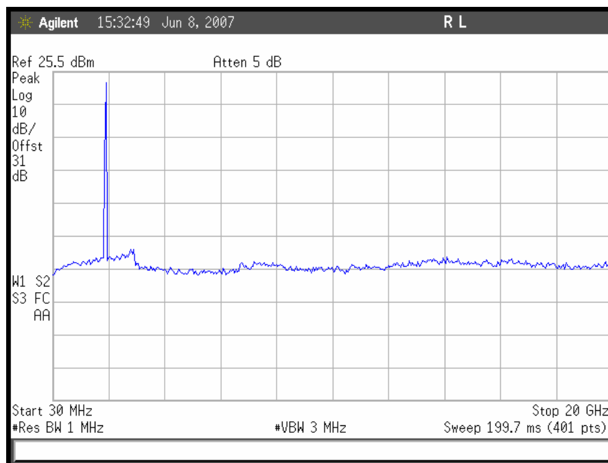
Plot 53. Conducted Spurious Emissions, GSM High Channel Uplink
