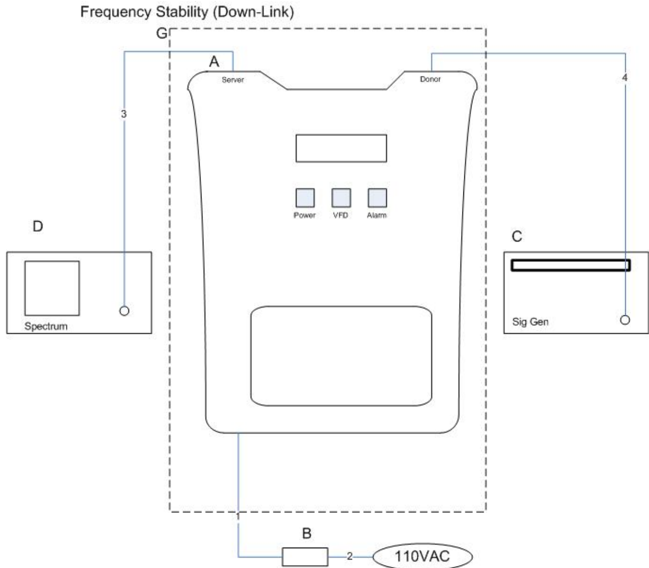
Figure 6. Block Diagram of Test Configuration (Frequency Stability)
