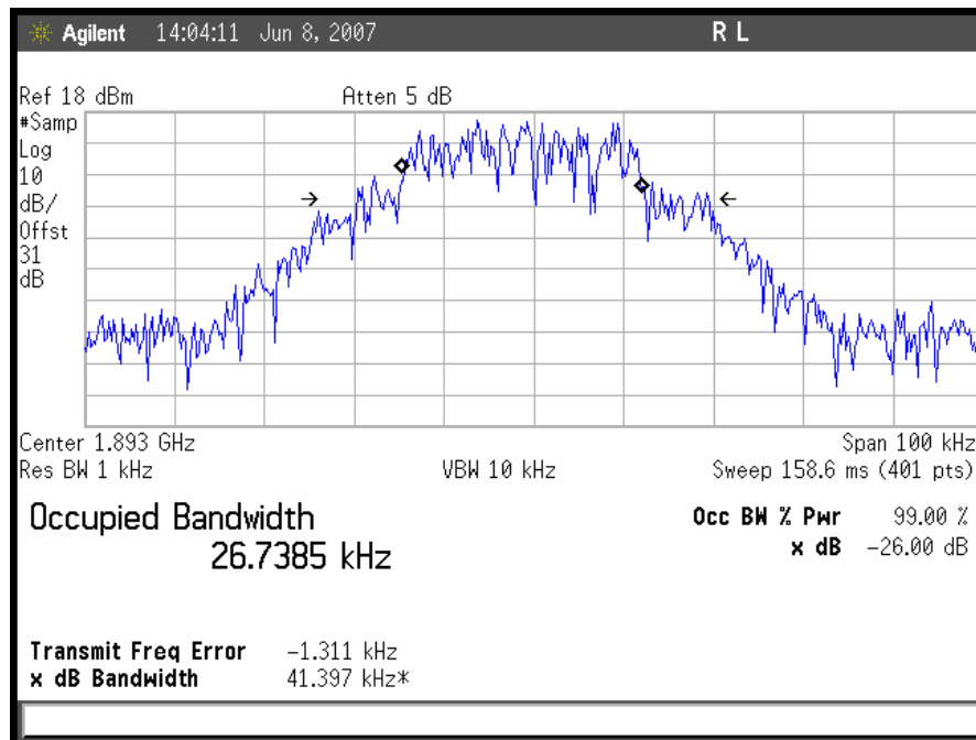
Plot 37. Occupied Bandwidth, TDMA Uplink, High Channel Output
