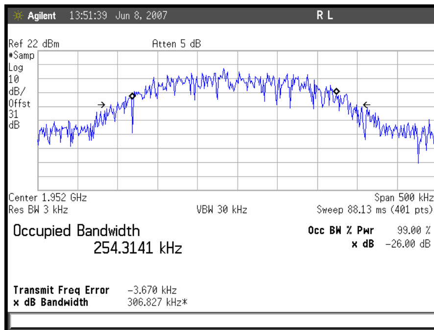
Plot 17. Occupied Bandwidth, GSM Downlink, Mid Channel Output
