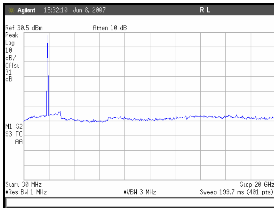
Plot 43. Conducted Spurious Emissions, CDMA High Channel Uplink
