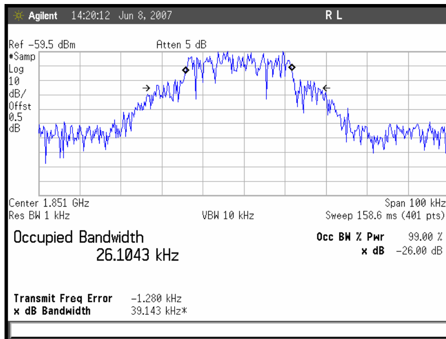
Plot 32. Occupied Bandwidth, TDMA Uplink, Low Channel Input
