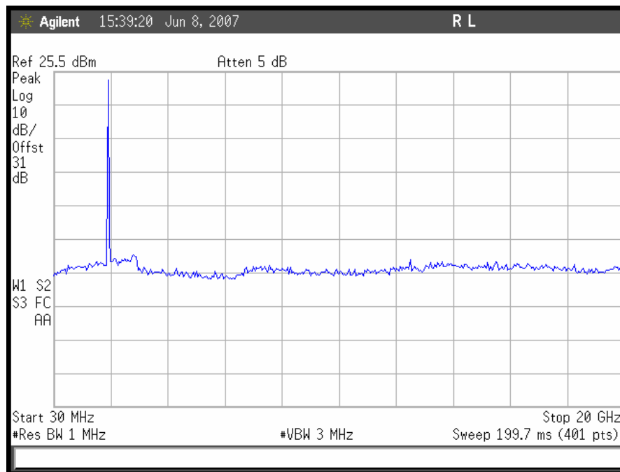
Plot 48. Conducted Spurious Emissions, GSM Low Channel Downlink
