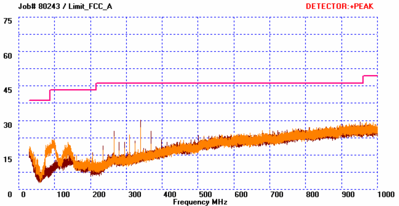
Plot 1. Radiated Emissions Test Plot
