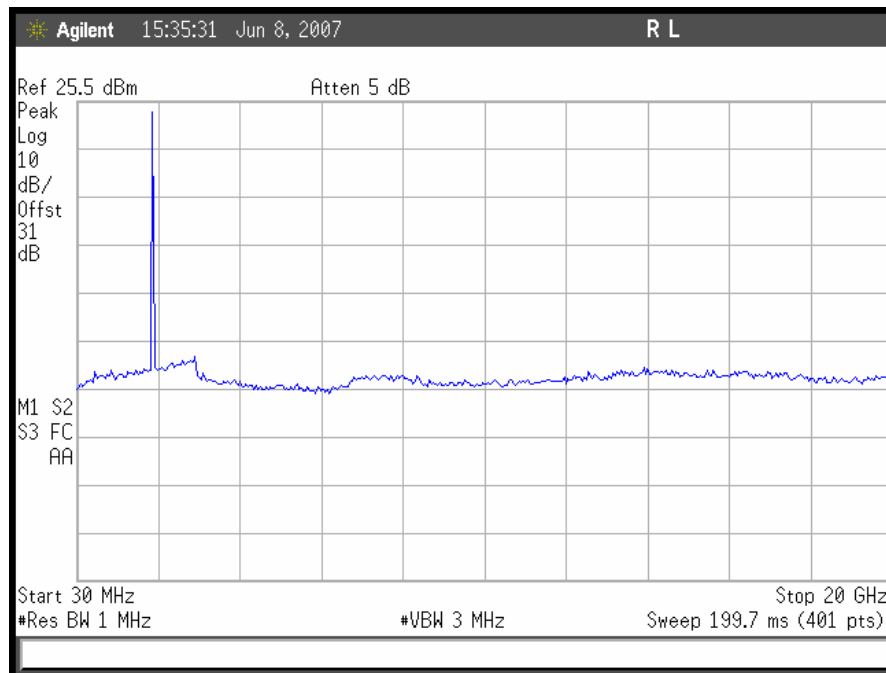
Plot 61. Conducted Spurious Emissions, TDMA Mid Channel Uplink
