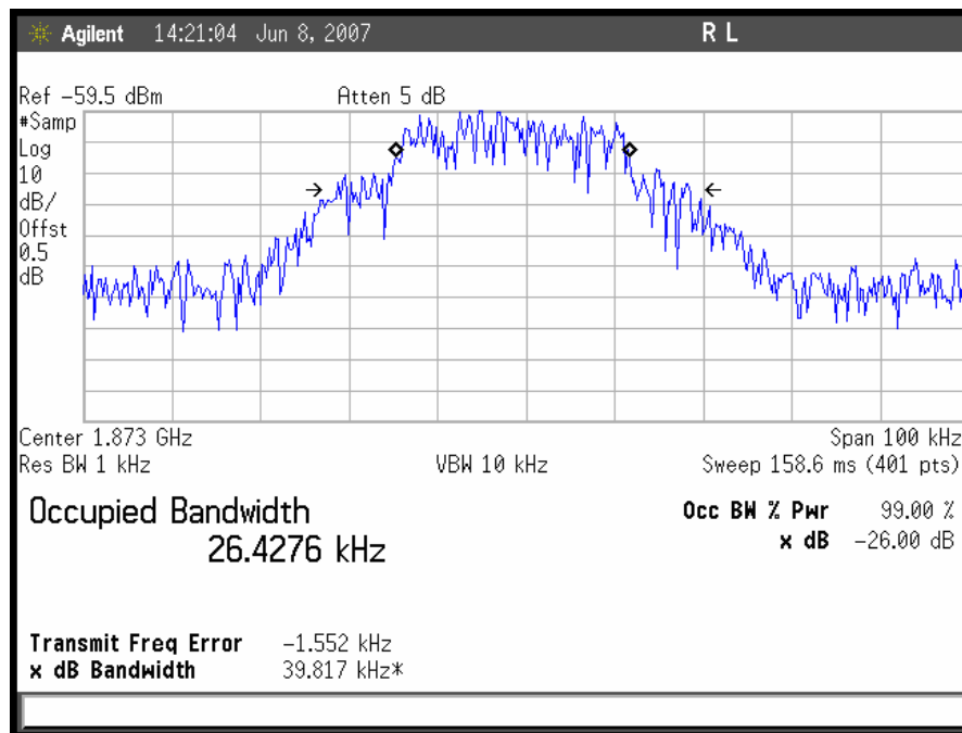
Plot 34. Occupied Bandwidth, TDMA Uplink, Mid Channel Input
