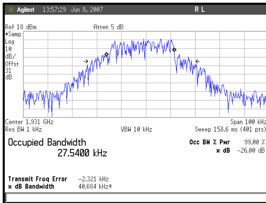
Plot 27. Occupied Bandwidth, TDMA Downlink, Low Channel Output
