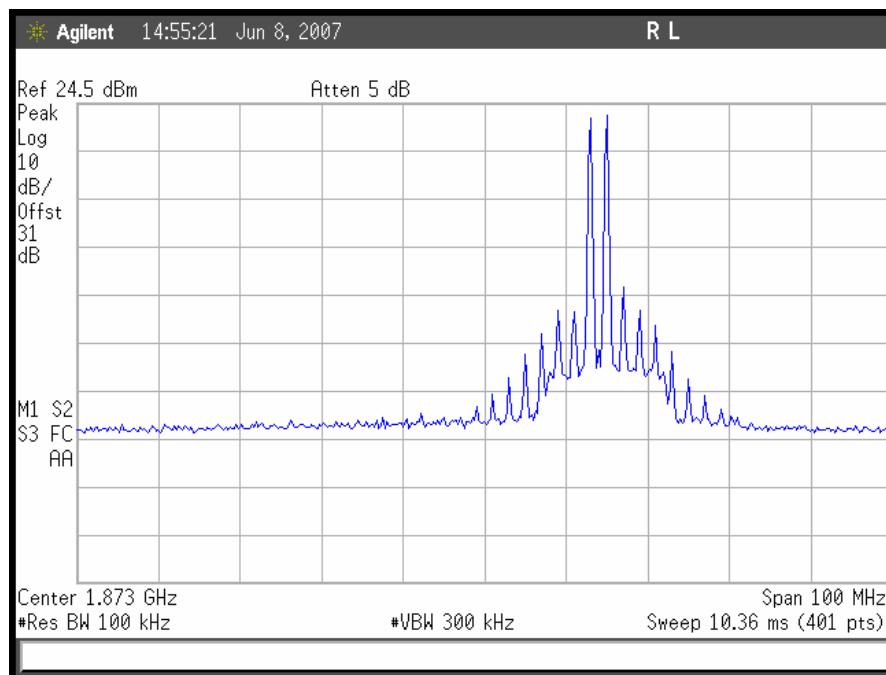
Plot 57. GSM Intermodulation, Uplink High End
