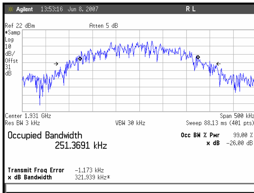
Plot 15. Occupied Bandwidth, GSM Downlink, Low Channel Output
