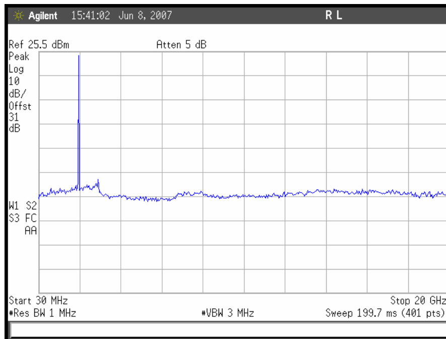
Plot 42. Conducted Spurious Emissions, CDMA High Channel Downlink
