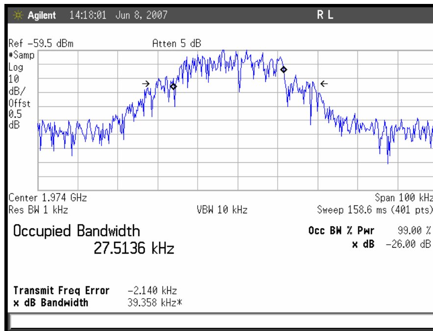
Plot 30. Occupied Bandwidth, TDMA Downlink, High Channel Input
