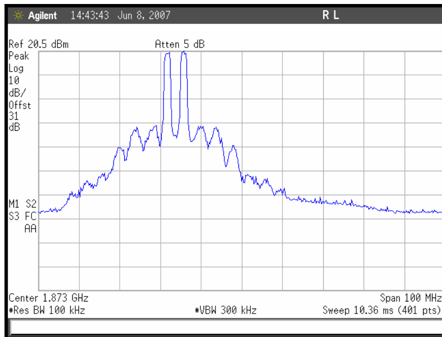
Plot 46. CDMA Intermodulation, Uplink Low End
