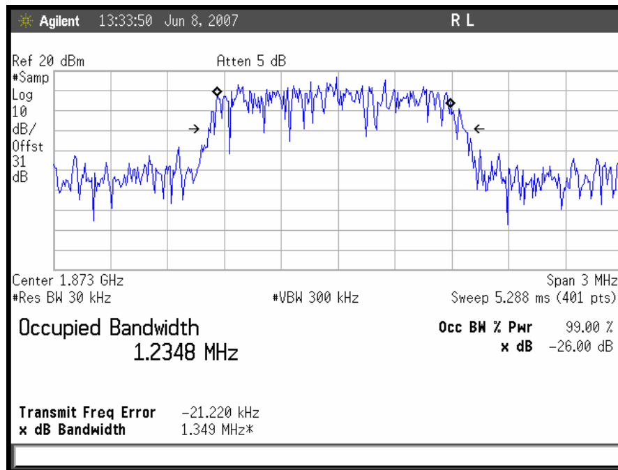
Plot 5. Occupied Bandwidth, CDMA Downlink, Mid Channel Output
