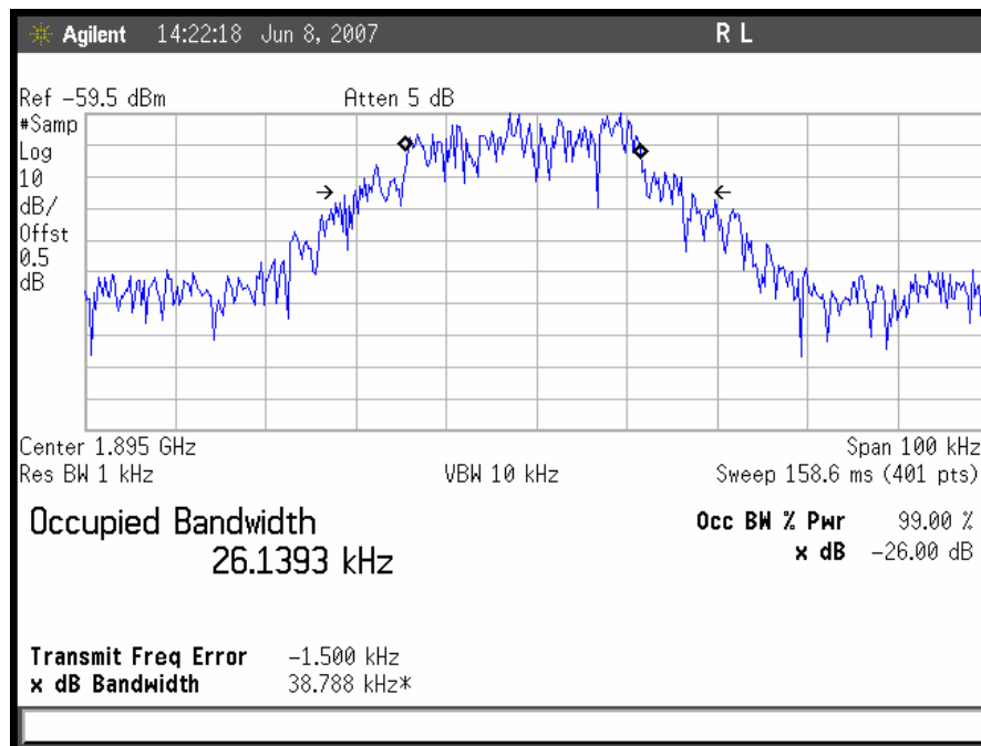
Plot 36. Occupied Bandwidth, TDMA Uplink, High Channel Input
