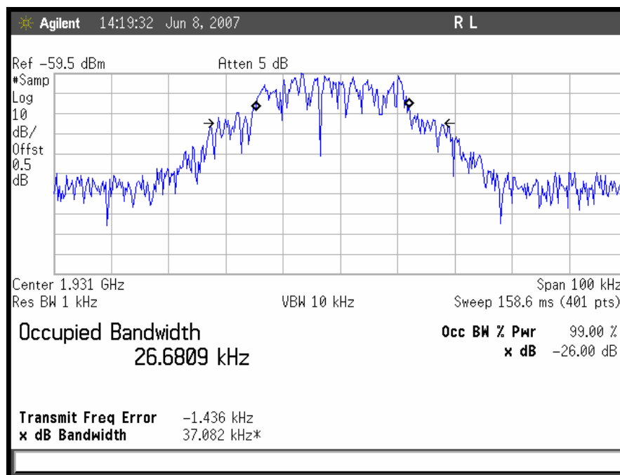
Plot 26. Occupied Bandwidth, TDMA Downlink, Low Channel Input
