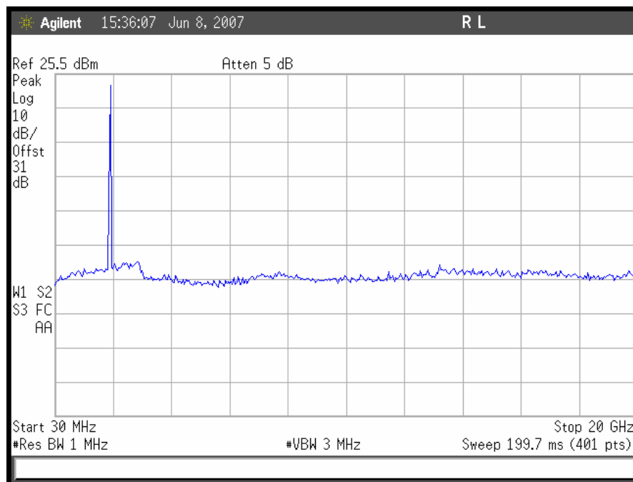
Plot 63. Conducted Spurious Emissions, TDMA High Channel Uplink
