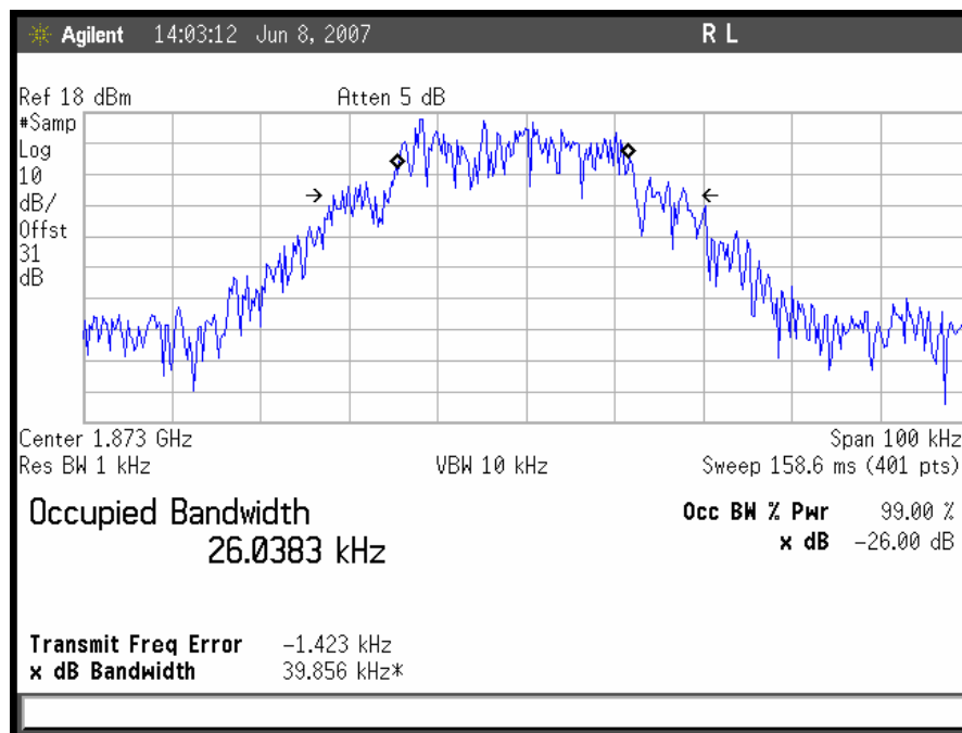
Plot 35. Occupied Bandwidth, TDMA Uplink, Mid Channel Output
