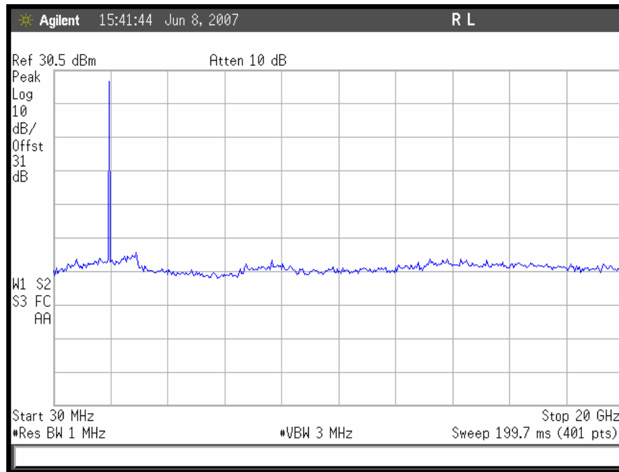
Plot 40. Conducted Spurious Emissions, CDMA Mid Channel Downlink
