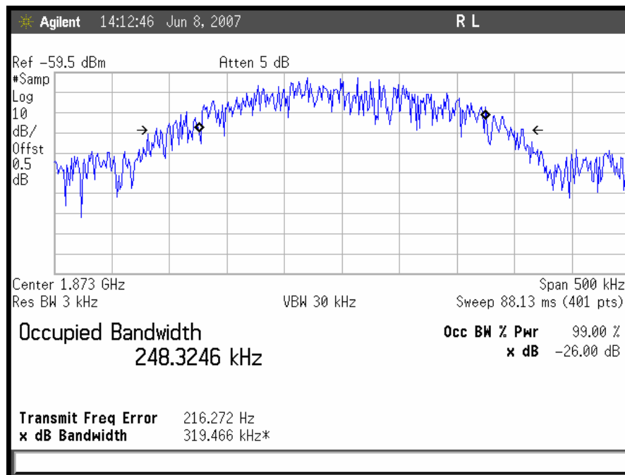
Plot 22. Occupied Bandwidth, GSM Uplink, Mid Channel Input
