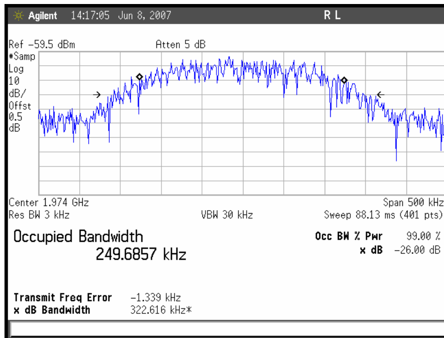
Plot 18. Occupied Bandwidth, GSM Downlink, High Channel Input
