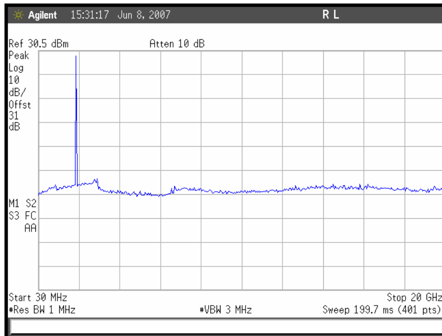
Plot 41. Conducted Spurious Emissions, CDMA Mid Channel Uplink
