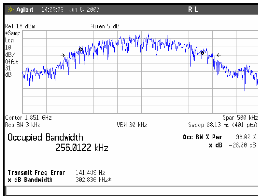
Plot 21. Occupied Bandwidth, GSM Uplink, Low Channel Output
