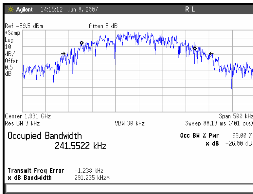
Plot 14. Occupied Bandwidth, GSM Downlink, Low Channel Input
