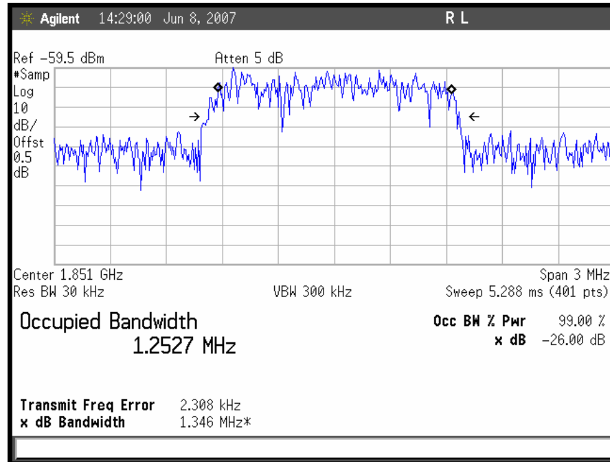
Plot 8. Occupied Bandwidth, CDMA Uplink, Low Channel Input
