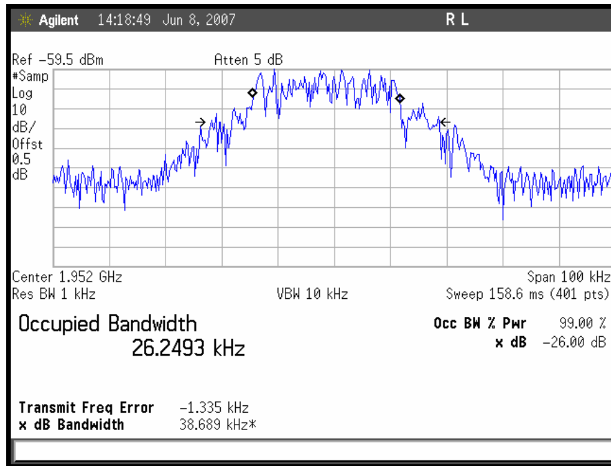
Plot 28. Occupied Bandwidth, TDMA Downlink, Mid Channel Input
