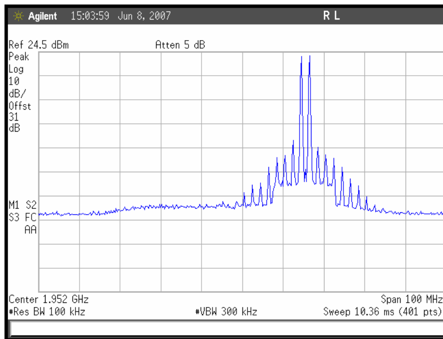
Plot 65. TDMA Intermodulation, Downlink High End
