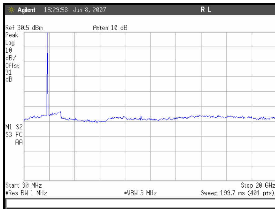
Plot 39. Conducted Spurious Emissions, CDMA Low Channel Uplink
