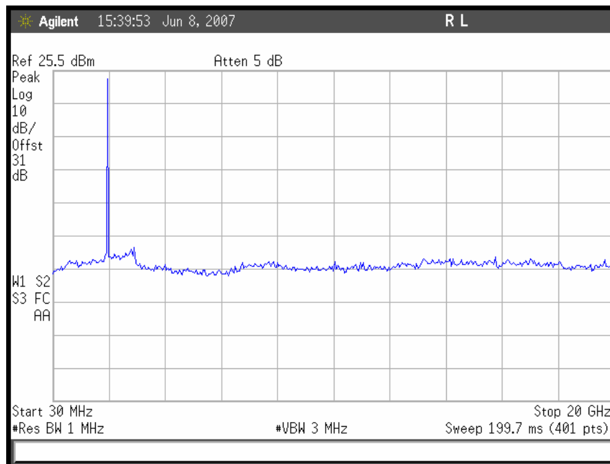
Plot 50. Conducted Spurious Emissions, GSM Mid Channel Downlink
