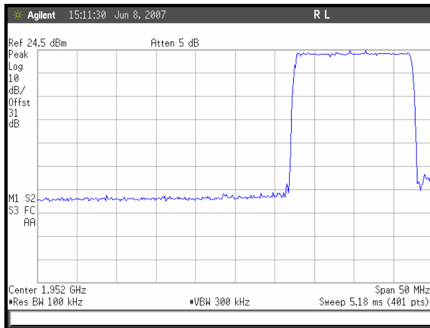
Plot 69. Out of Band Rejection, Downlink High End filter
