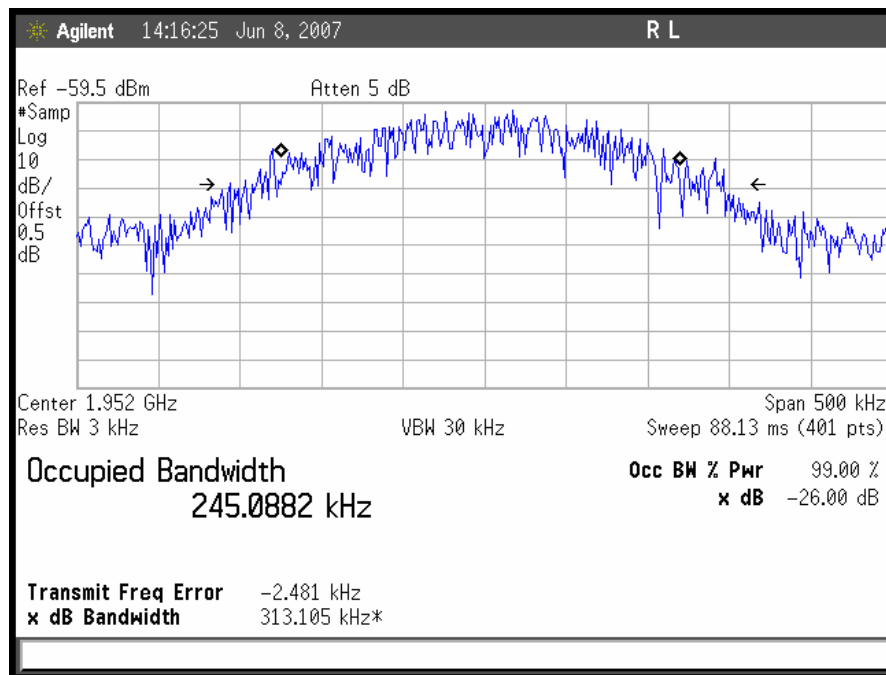
Plot 16. Occupied Bandwidth, GSM Downlink, Mid Channel Input
