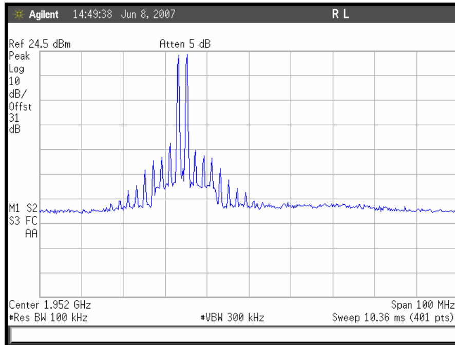
Plot 54. GSM Intermodulation, Downlink Low End
