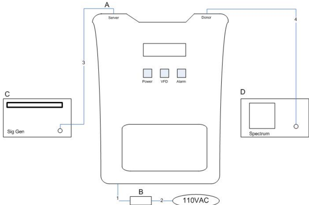
Figure 3. Block Diagram of Test Configuration (Conducted Measurement-Uplink)
