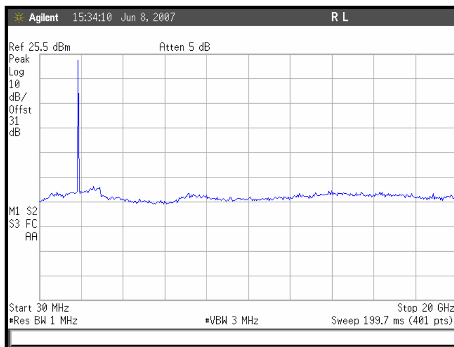
Plot 49. Conducted Spurious Emissions, GSM Low Channel Uplink
