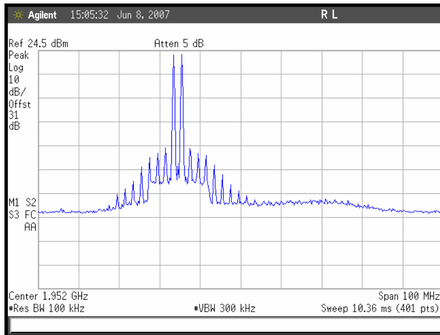
Plot 64. TDMA Intermodulation, Downlink Low End
