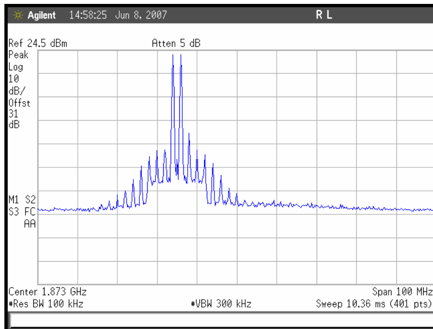
Plot 66. TDMA Intermodulation, Uplink Low End
