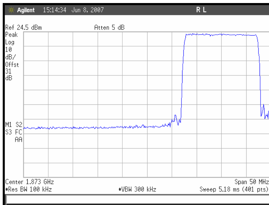
Plot 71. Out of Band Rejection, Uplink High End filter
