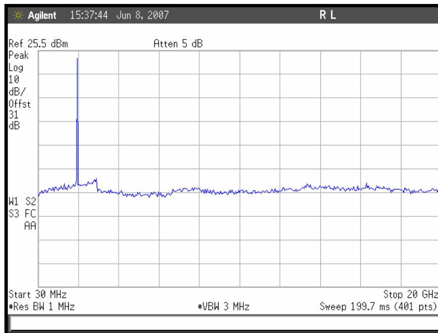
Plot 62. Conducted Spurious Emissions, TDMA High Channel Downlink
