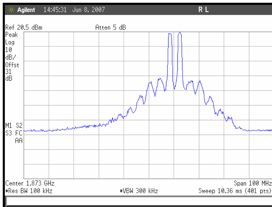
Plot 47. CDMA Intermodulation, Uplink High End
