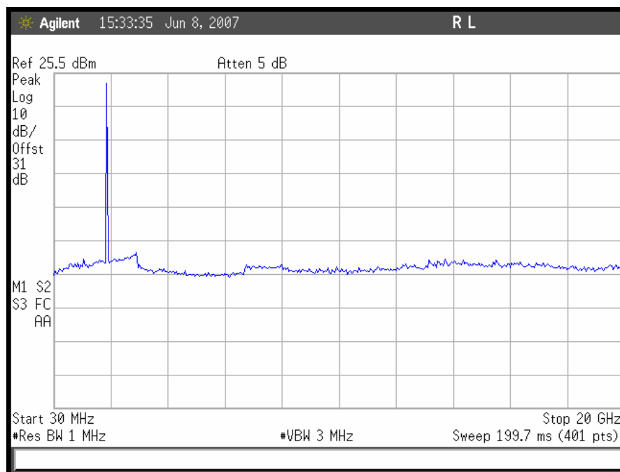
Plot 51. Conducted Spurious Emissions, GSM Mid Channel Uplink
