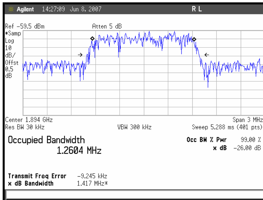
Plot 12. Occupied Bandwidth, CDMA Uplink, High Channel Input
