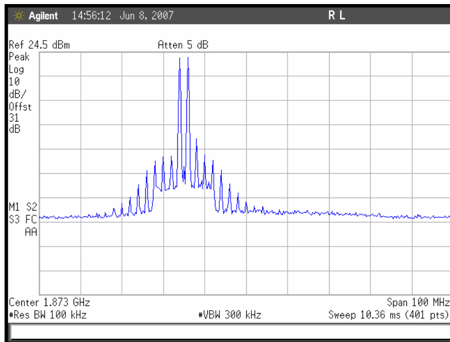
Plot 56. GSM Intermodulation, Uplink Low End
