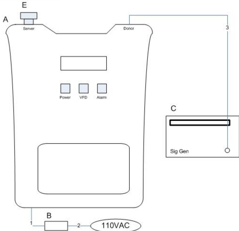
Figure 4. Block Diagram of Test Configuration (Spurious Emission - Downlink)
