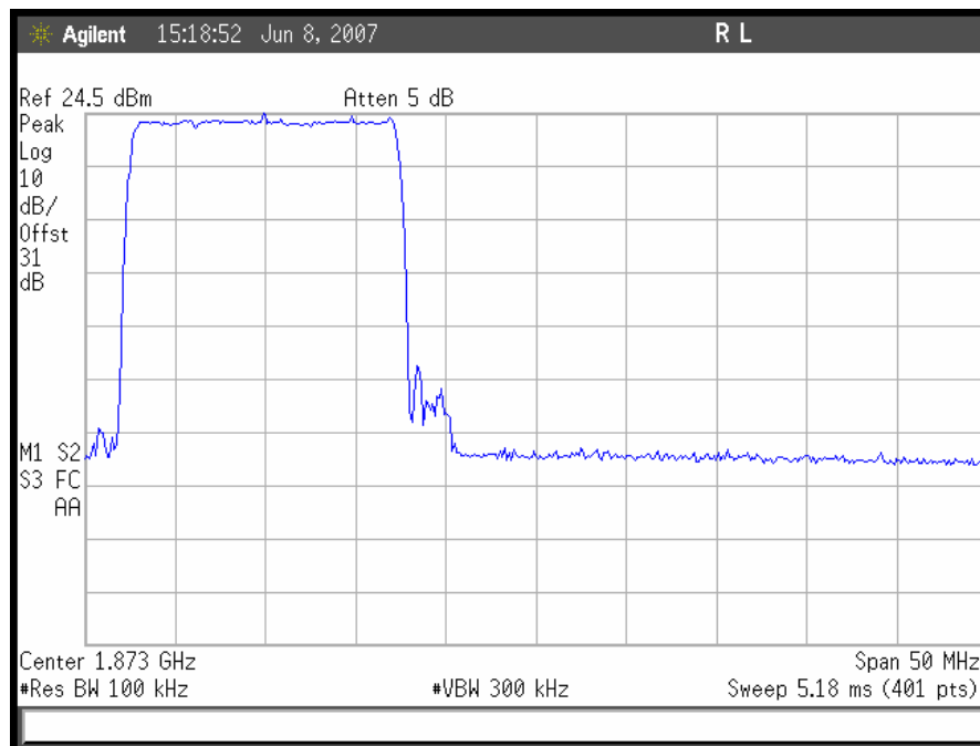
Plot 70. Out of Band Rejection, Uplink Low End filter
