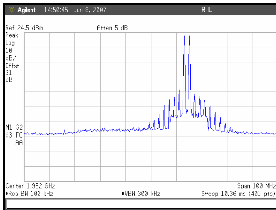
Plot 55. GSM Intermodulation, Downlink High End
