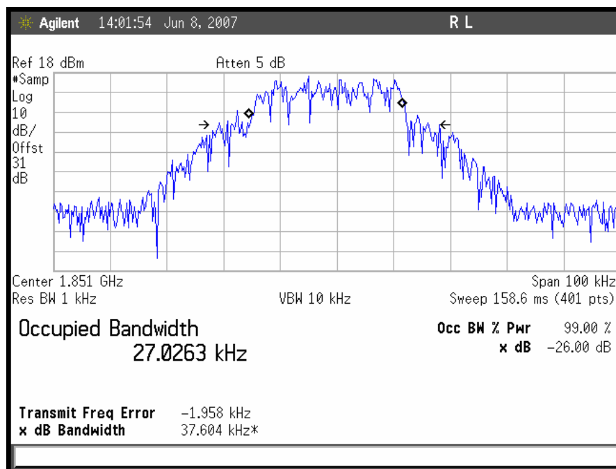
Plot 33. Occupied Bandwidth, TDMA Uplink, Low Channel Output
