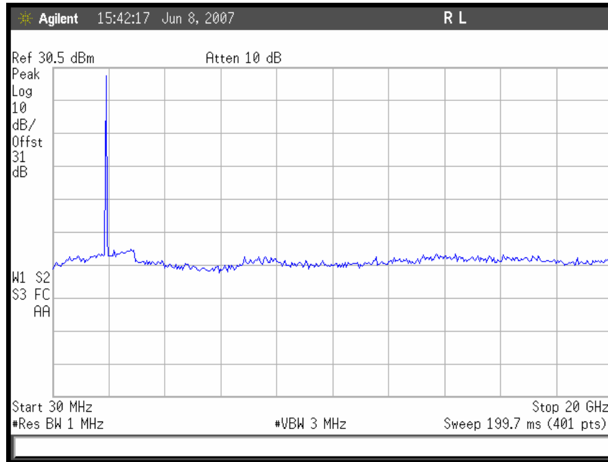
Plot 38. Conducted Spurious Emissions, CDMA Low Channel Downlink
