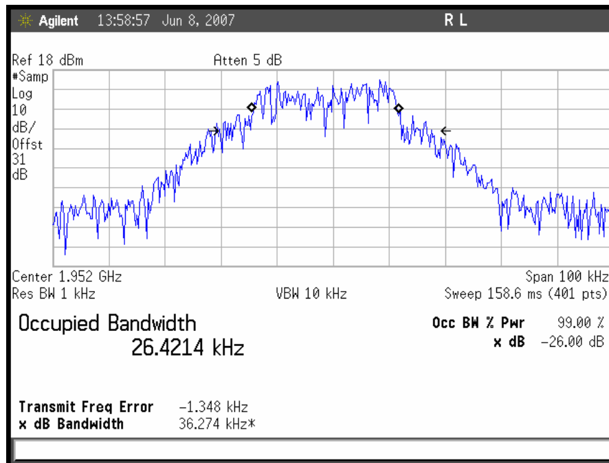
Plot 29. Occupied Bandwidth, TDMA Downlink, Mid Channel Output
