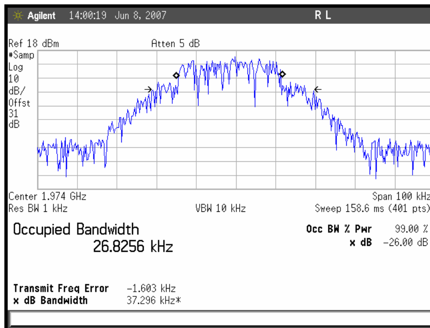
Plot 31. Occupied Bandwidth, TDMA Downlink, High Channel Output
