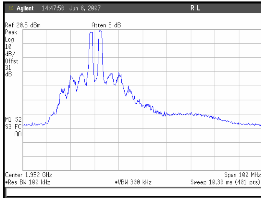
Plot 44. CDMA Intermodulation, Downlink Low End
