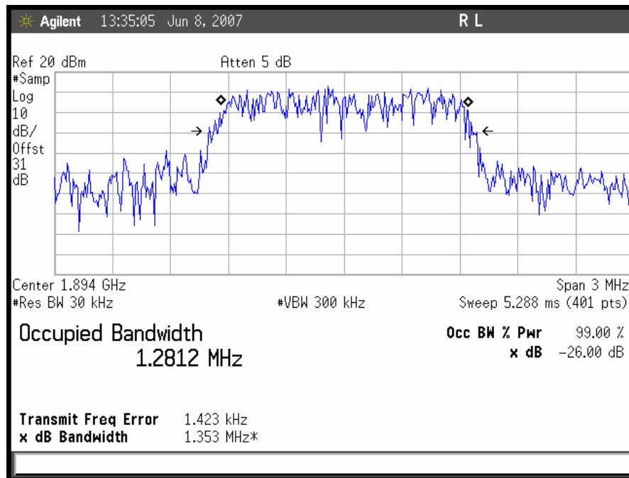
Plot 7. Occupied Bandwidth, CDMA Downlink, High Channel Output
