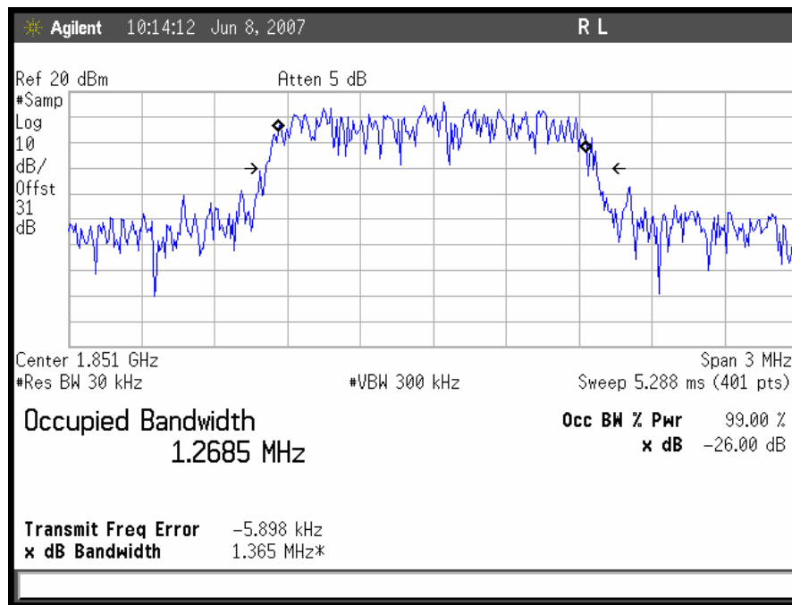
Plot 3. Occupied Bandwidth, CDMA Downlink, Low Channel Output
