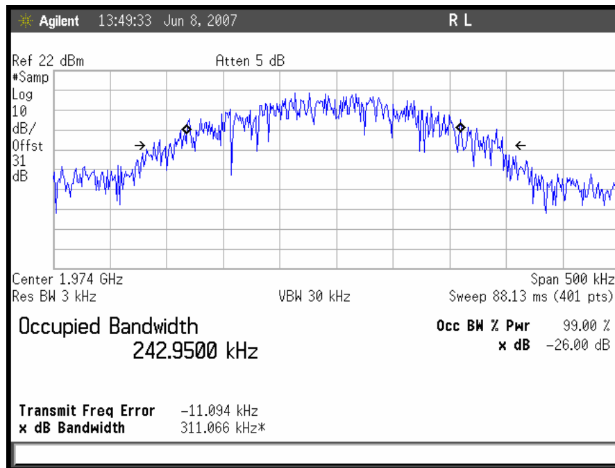
Plot 19. Occupied Bandwidth, GSM Downlink, High Channel Output
