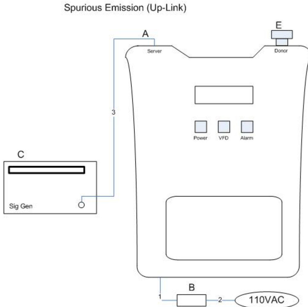
Figure 5. Block Diagram of Test Configuration (Spurious Emission - Uplink)
