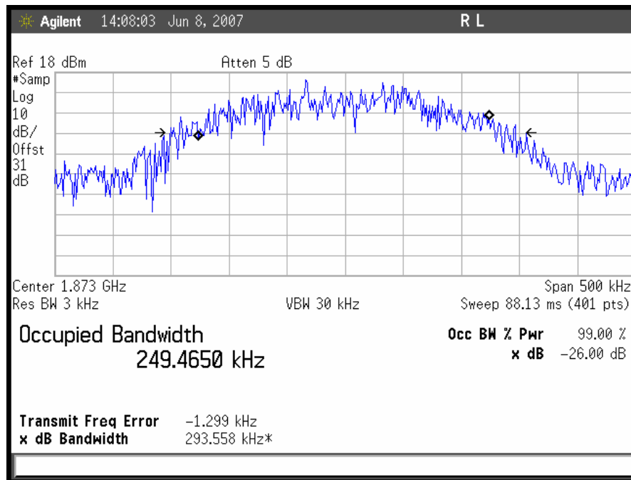
Plot 23. Occupied Bandwidth, GSM Uplink, Mid Channel Output
