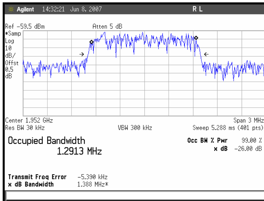
Plot 4. Occupied Bandwidth, CDMA Downlink, Mid Channel Input
