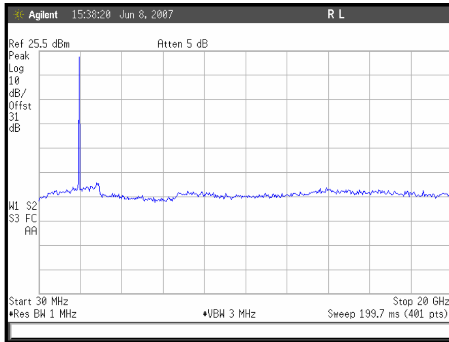
Plot 60. Conducted Spurious Emissions, TDMA Mid Channel Downlink
