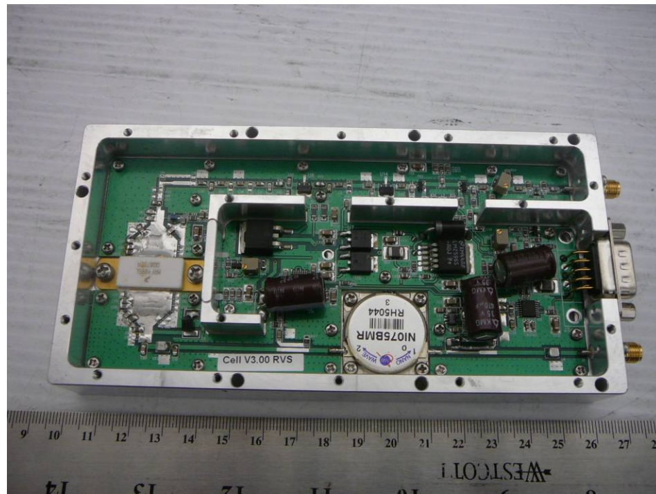
EUT – LTE Band Module PCB-7 Top View
