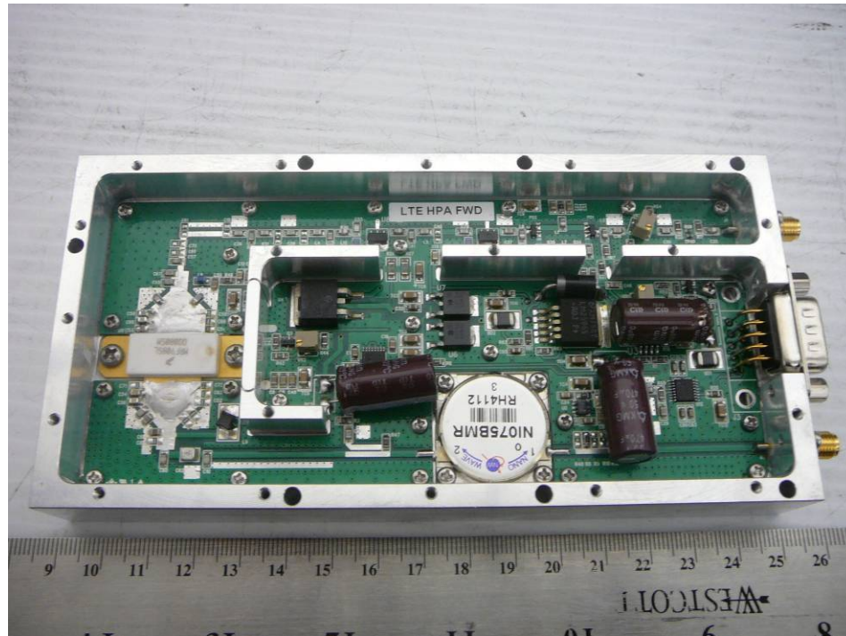
EUT – LTE Band Module PCB-6 Top View
