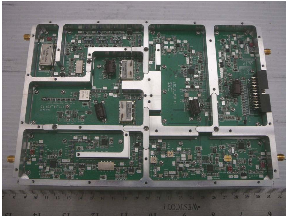
EUT – LTE Band Module PCB-4 Top View
