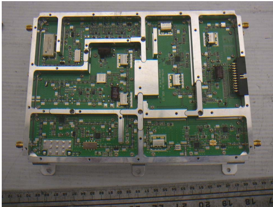
EUT – AWS Band Module PCB-4 Top View
