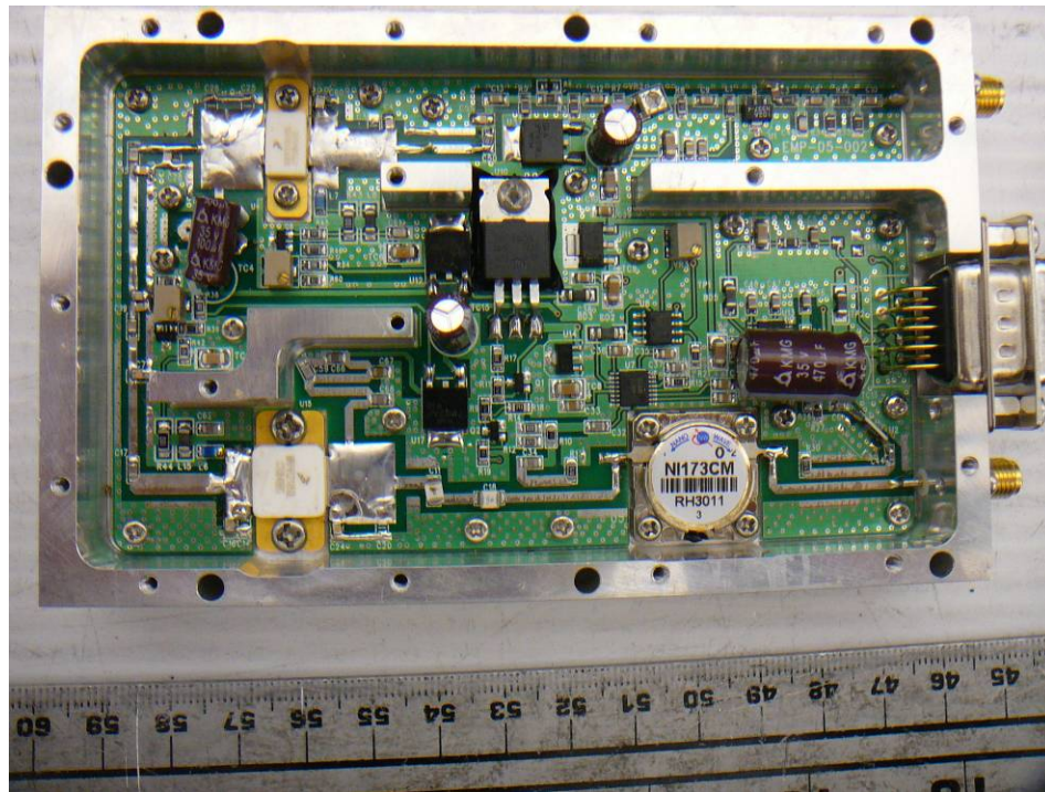
EUT – AWS Band Module PCB-7 Top View
