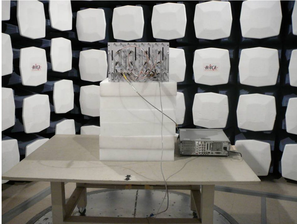
Radiated Emissions 30 MHz to 1GHz- Rear View
