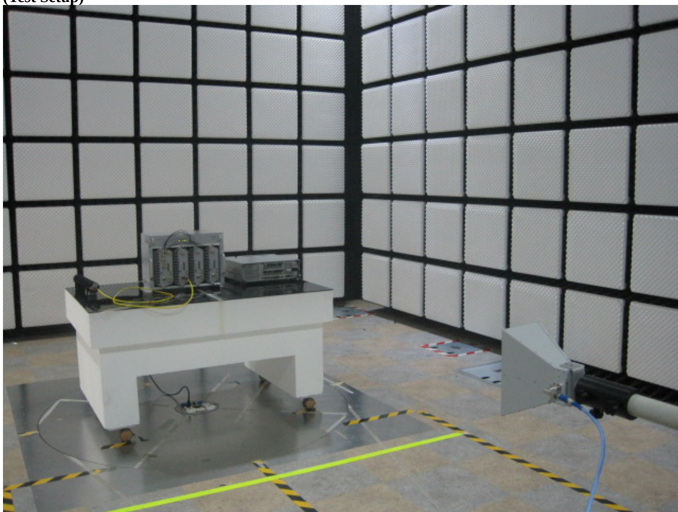
(Test Setup)
