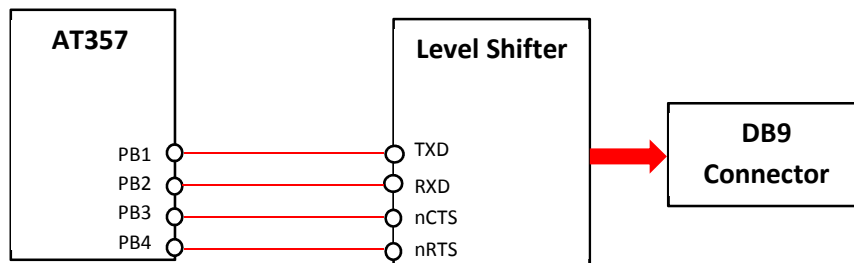
Figure 9b. AT357 module to external UART device
