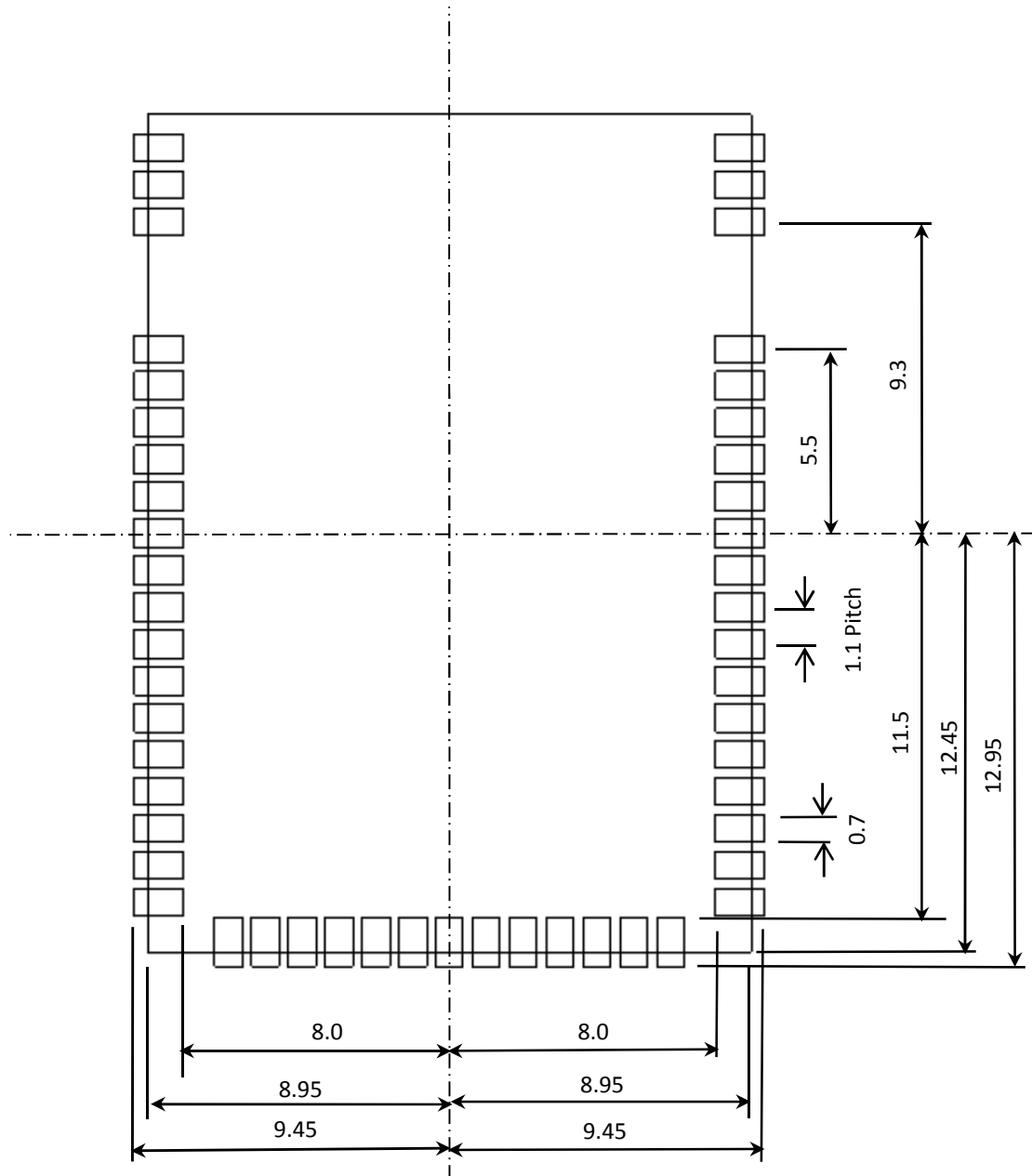
Figure 3: Module Footprint
