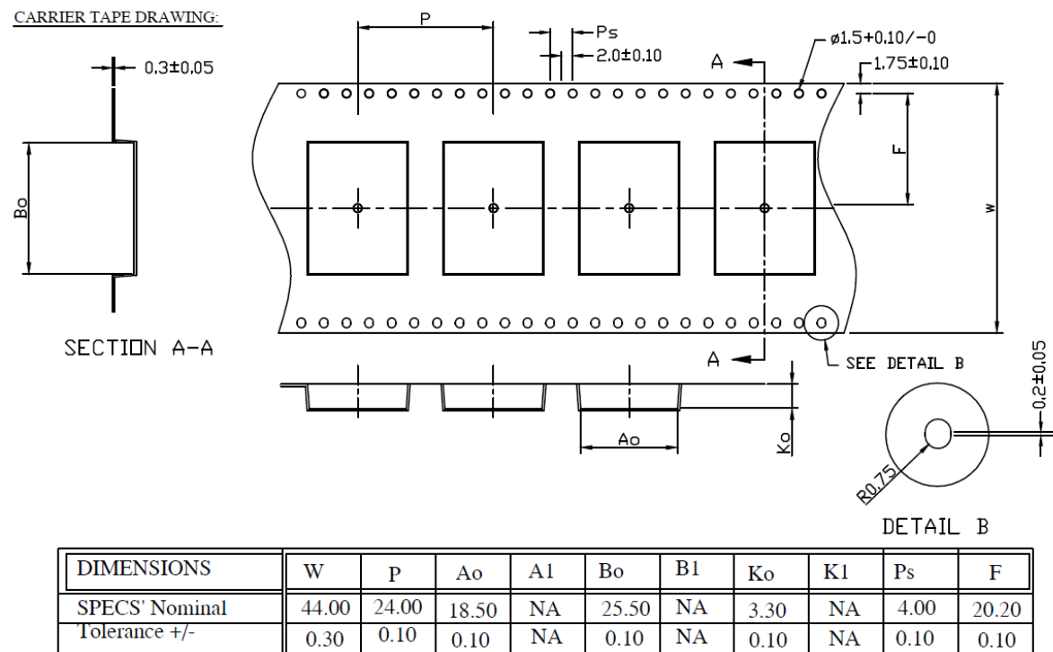
Figure 12: Tape Dimensions
