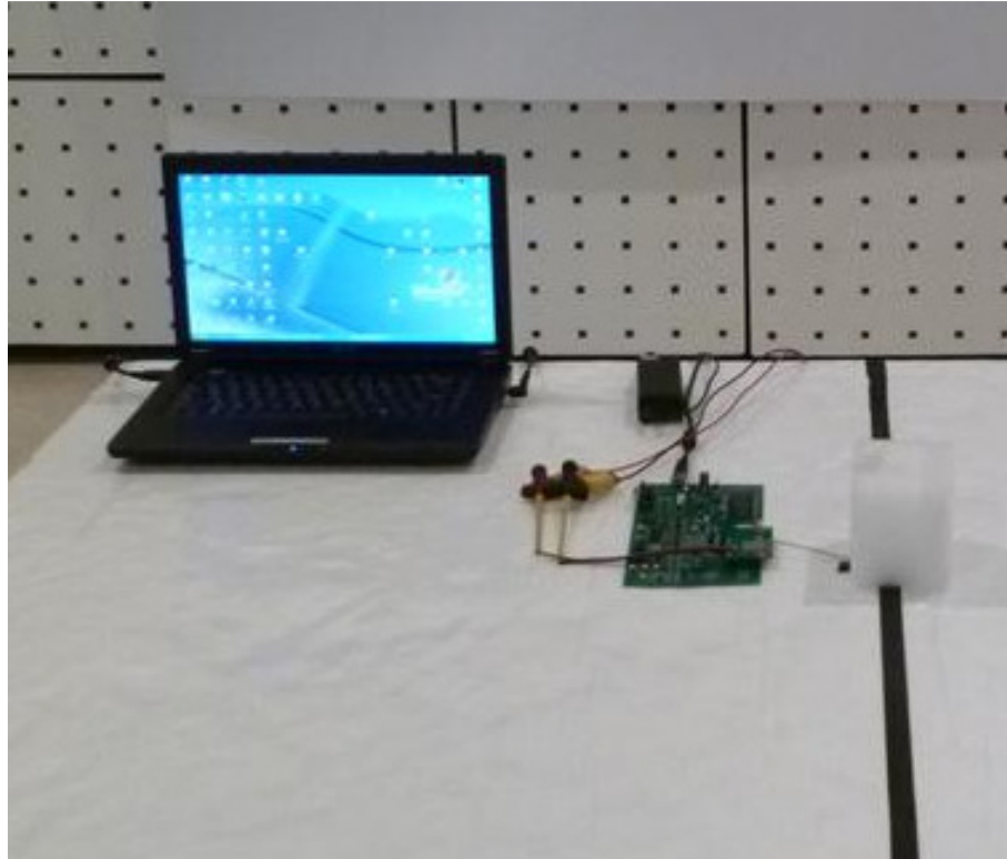
Photograph 5: Set-up for Radiated testing of Module
