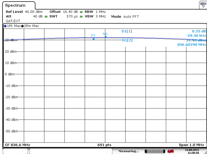
Peak-to-Average Ratio on Channel 190 (836.6 MHz)
