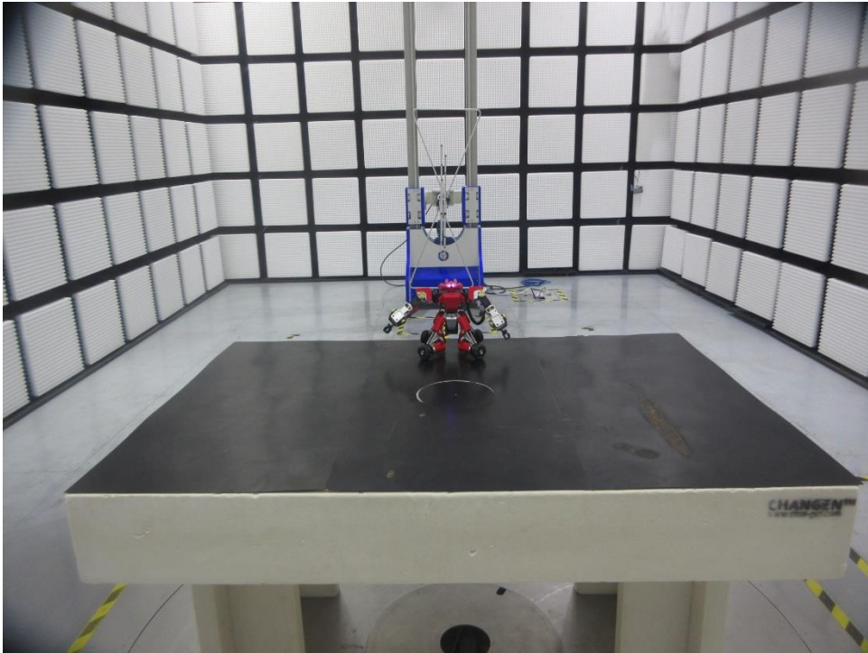
On/TX mode
