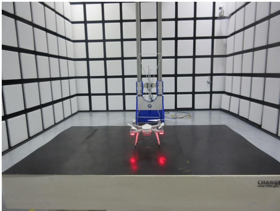
Radiated emission (below 1GHz) Test Setup Photo
