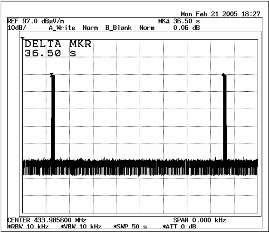
Transmission Period 1
