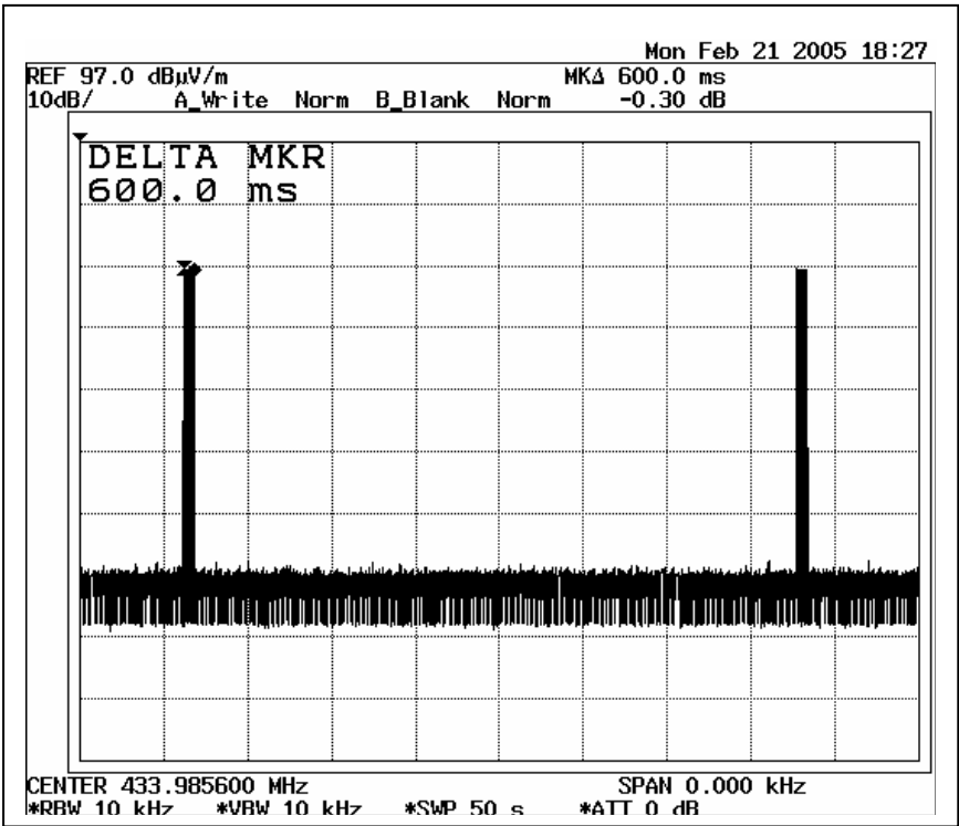
Transmission Period 2
