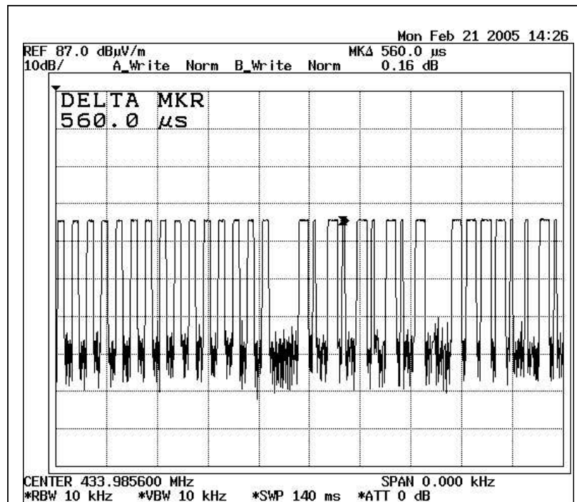
Duty Cycle 4
