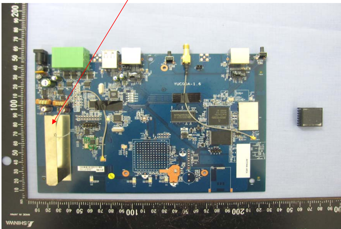
Z-WAVE Antenna
